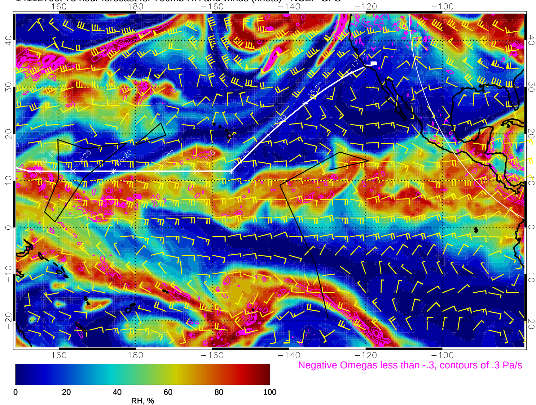
14112706, 78 hour forecast for 700mb RH and winds (knots) - NCEP GFS
