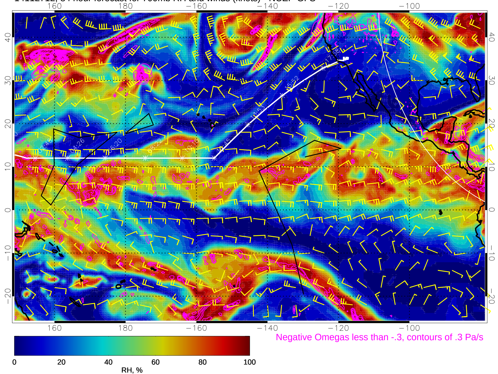
14112712, 84 hour forecast for 700mb RH and winds (knots) - NCEP GFS
