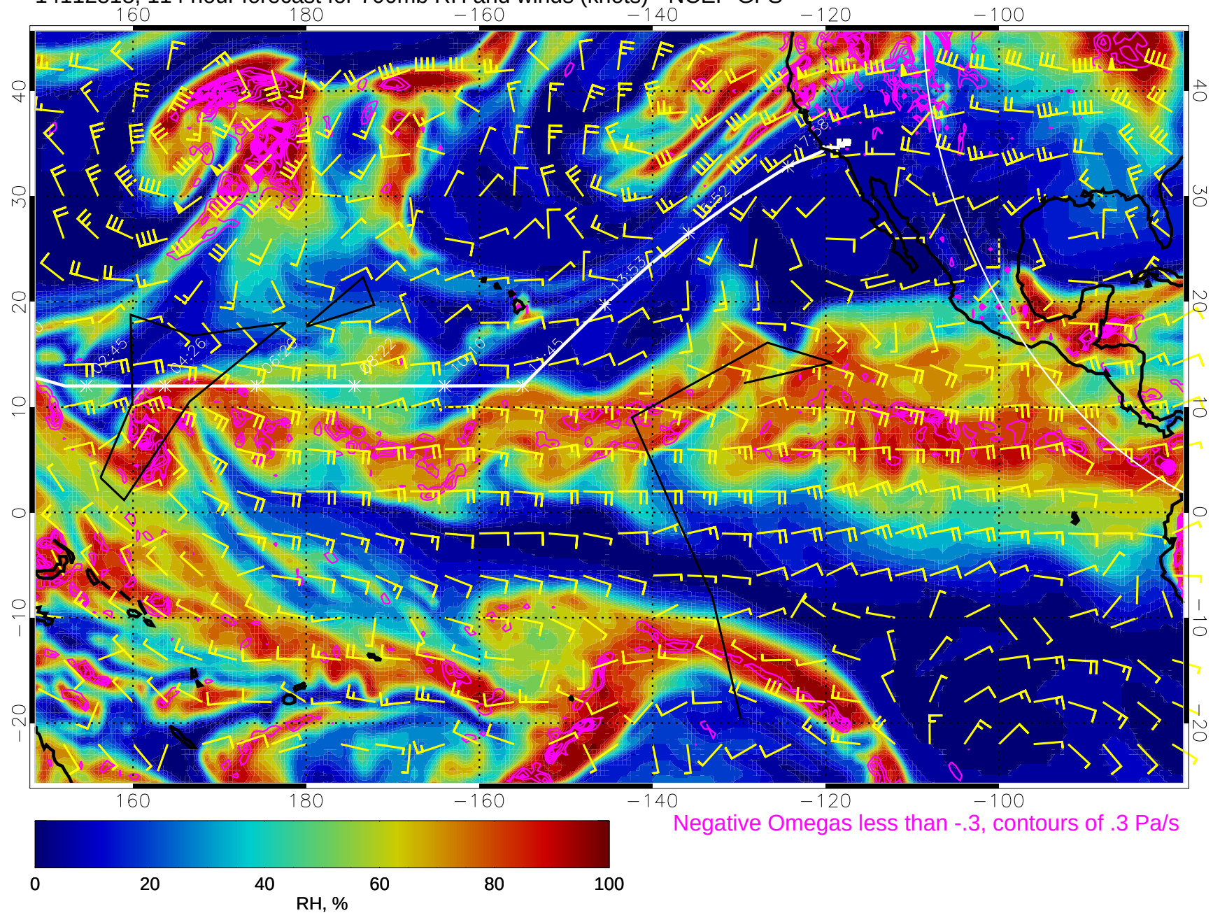
14112818, 114 hour forecast for 700mb RH and winds (knots) - NCEP GFS
