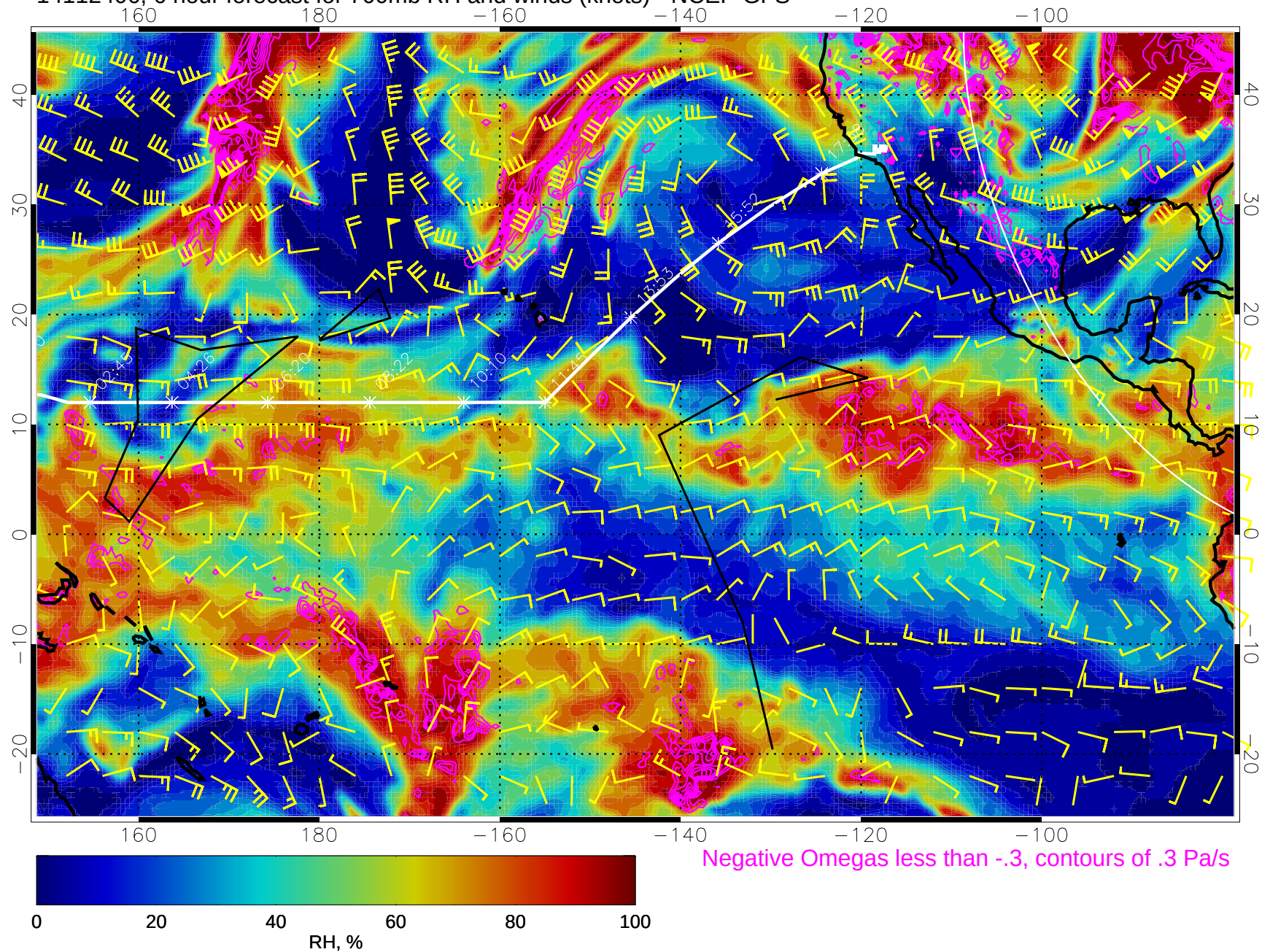
14112406, 6 hour forecast for 700mb RH and winds (knots) - NCEP GFS
