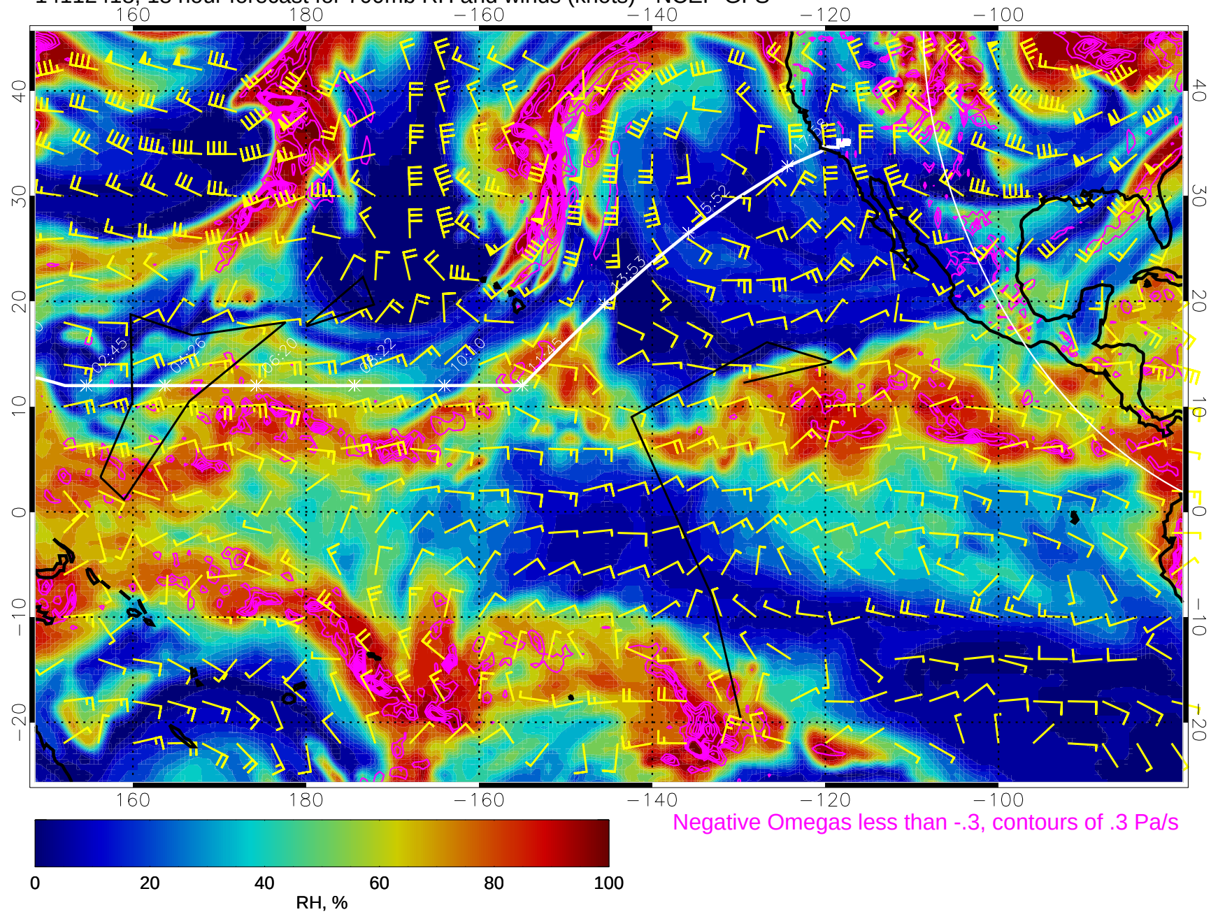
14112418, 18 hour forecast for 700mb RH and winds (knots) - NCEP GFS
