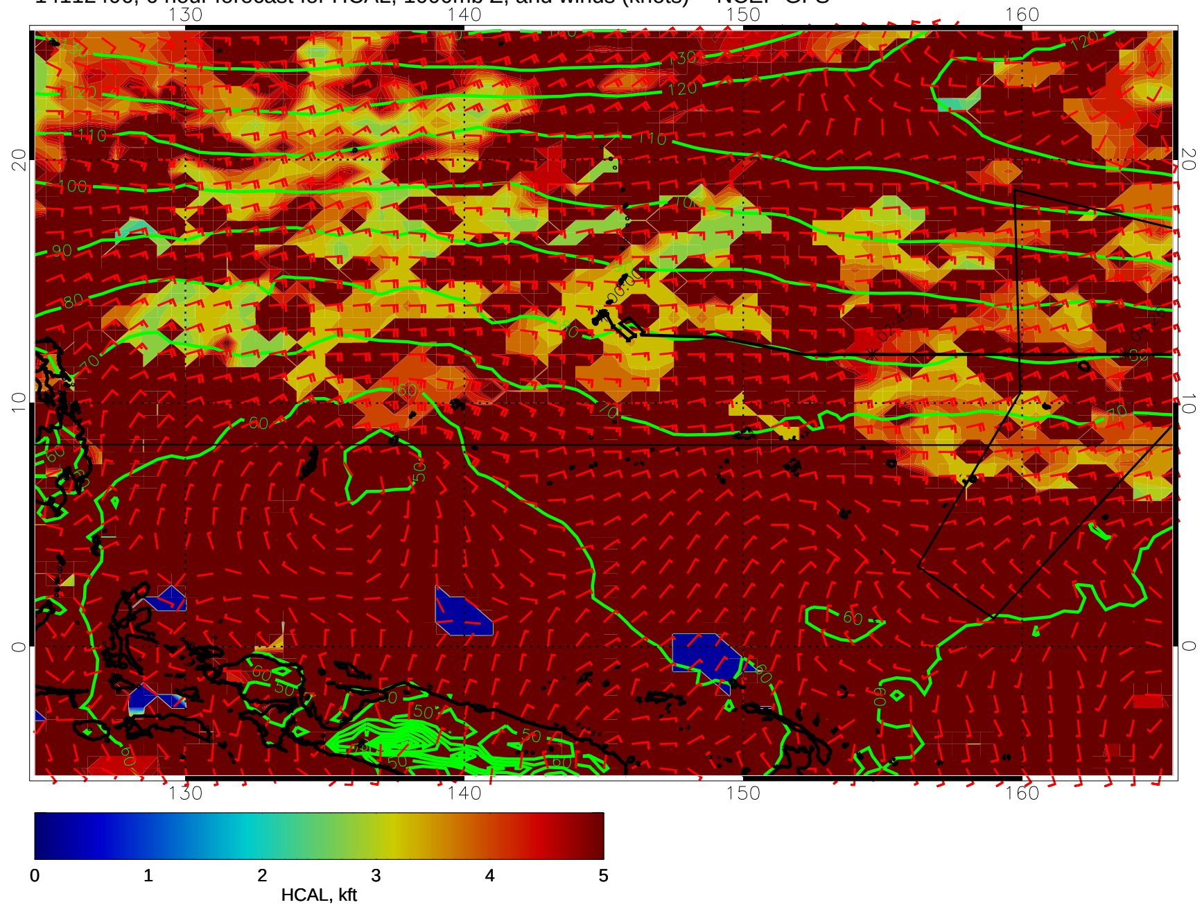
14112406, 6 hour forecast for HCAL, 1000mb Z, and winds (knots) -- NCEP GFS
