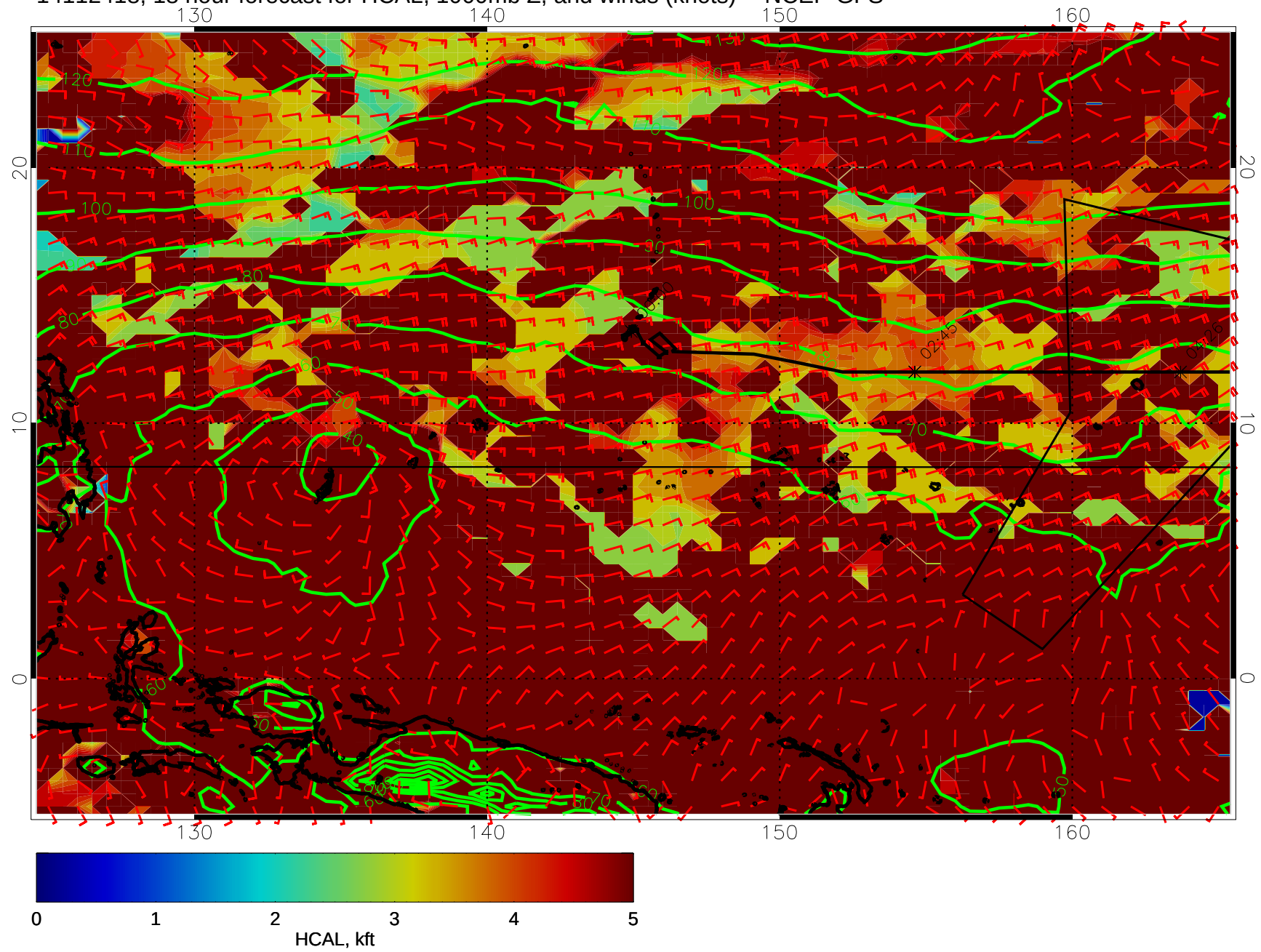
14112418, 18 hour forecast for HCAL, 1000mb Z, and winds (knots) -- NCEP GFS
