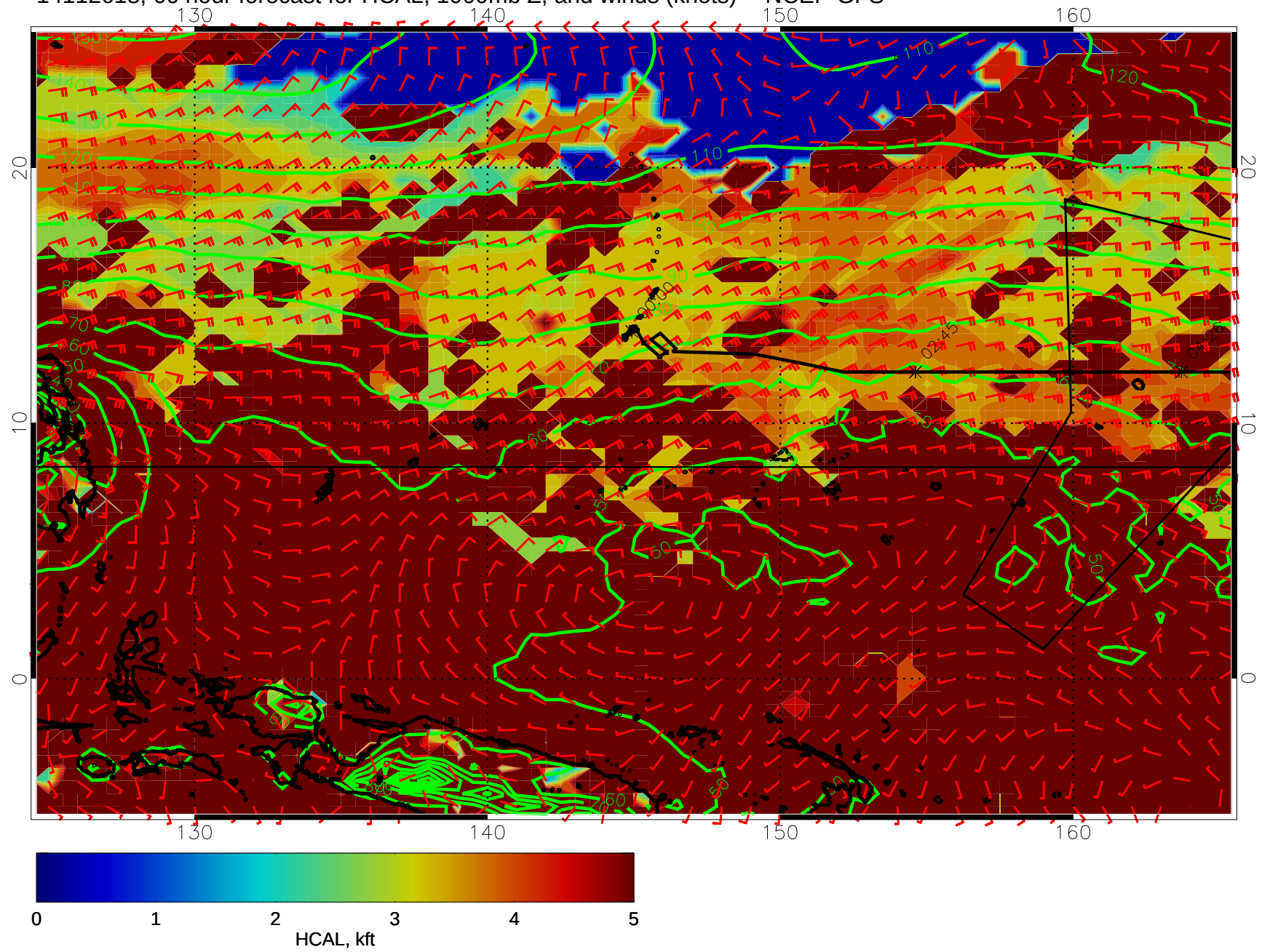
14112618, 66 hour forecast for HCAL, 1000mb Z, and winds (knots) -- NCEP GFS
