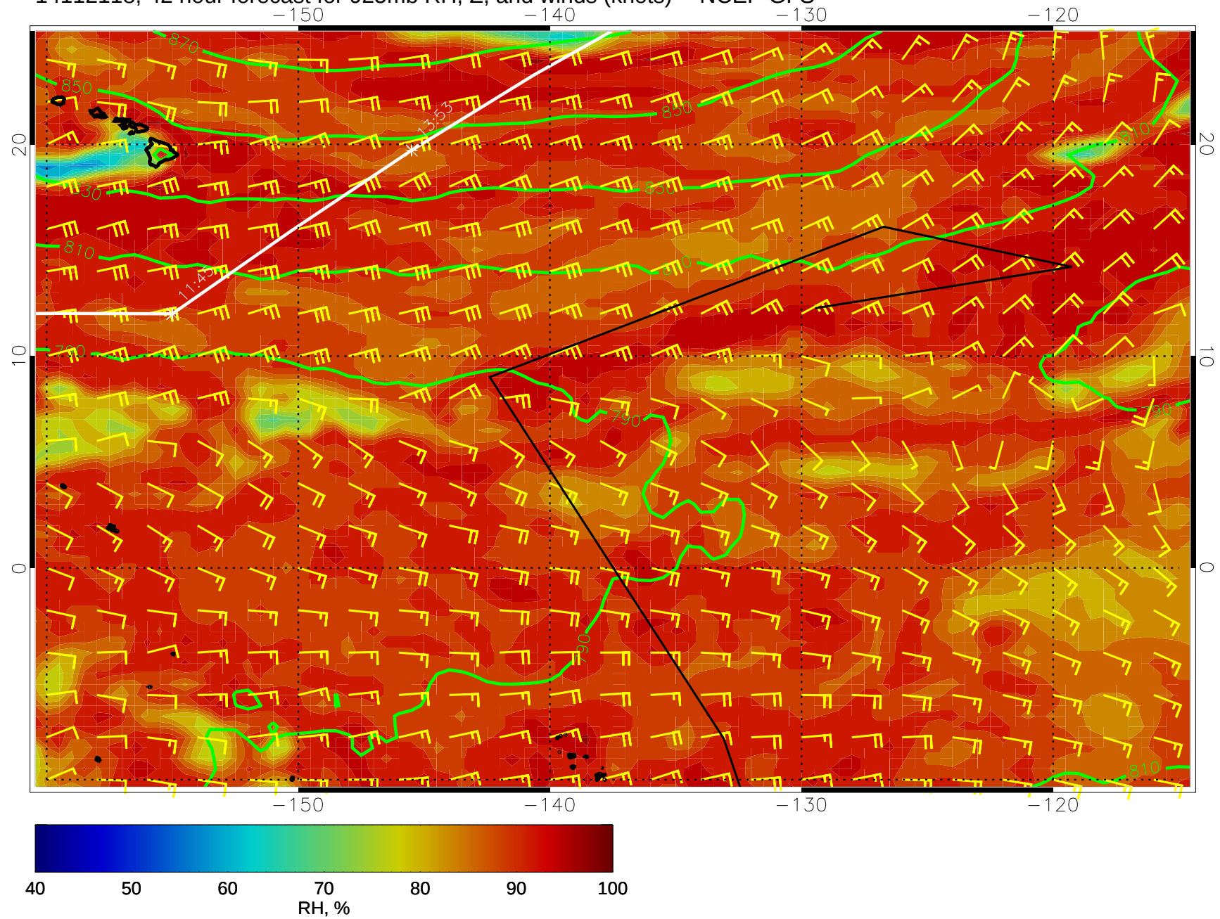
14112118, 42 hour forecast for 925mb RH, Z, and winds (knots) -- NCEP GFS
