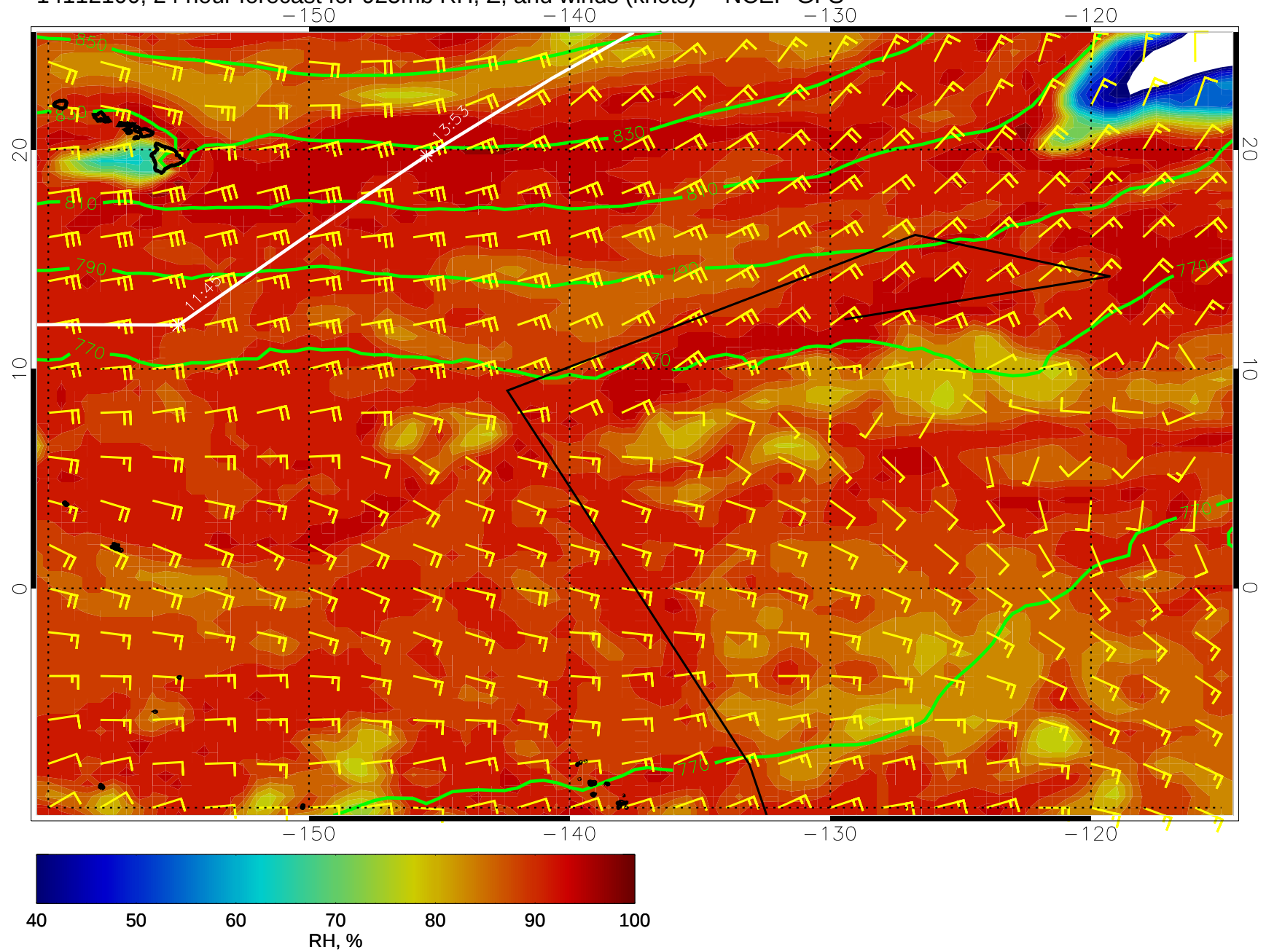
14112100, 24 hour forecast for 925mb RH, Z, and winds (knots) -- NCEP GFS
