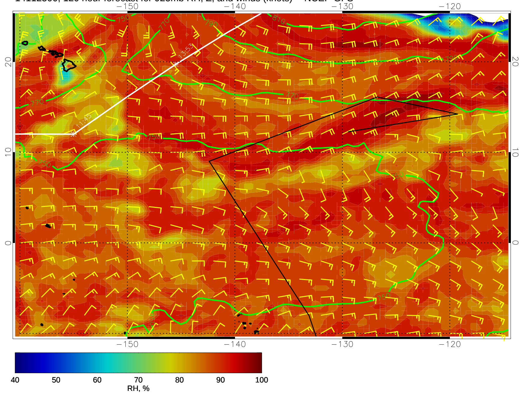
14112500, 120 hour forecast for 925mb RH, Z, and winds (knots) -- NCEP GFS
