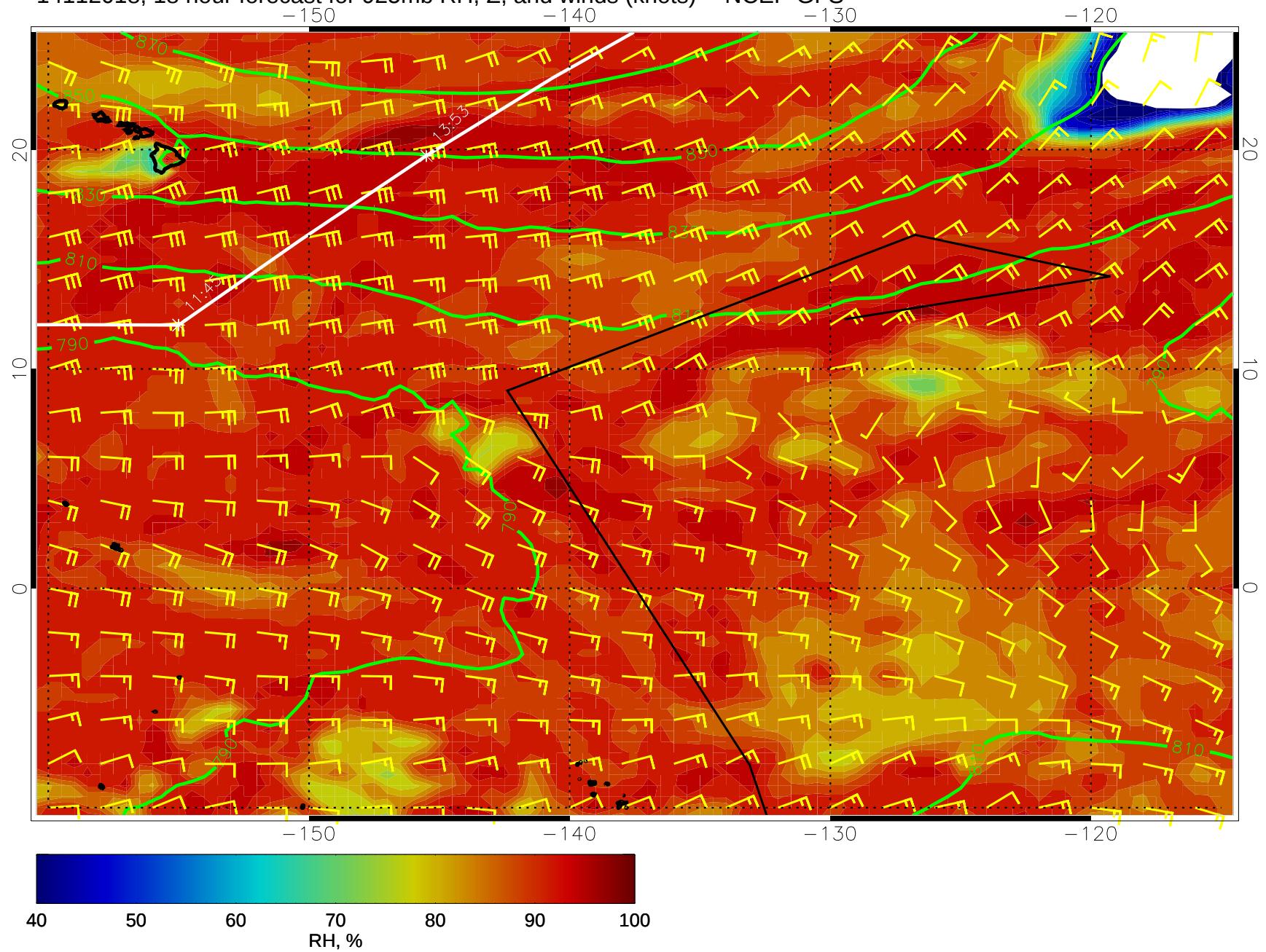
14112018, 18 hour forecast for 925mb RH, Z, and winds (knots) -- NCEP GFS
