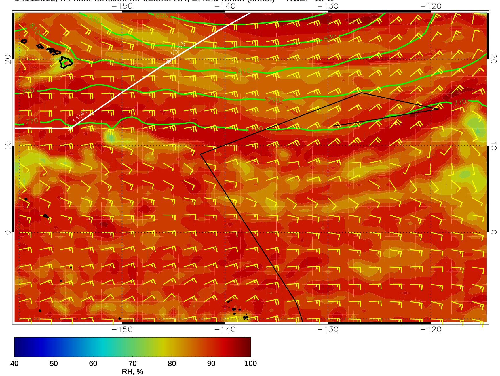
14112312, 84 hour forecast for 925mb RH, Z, and winds (knots) -- NCEP GFS
