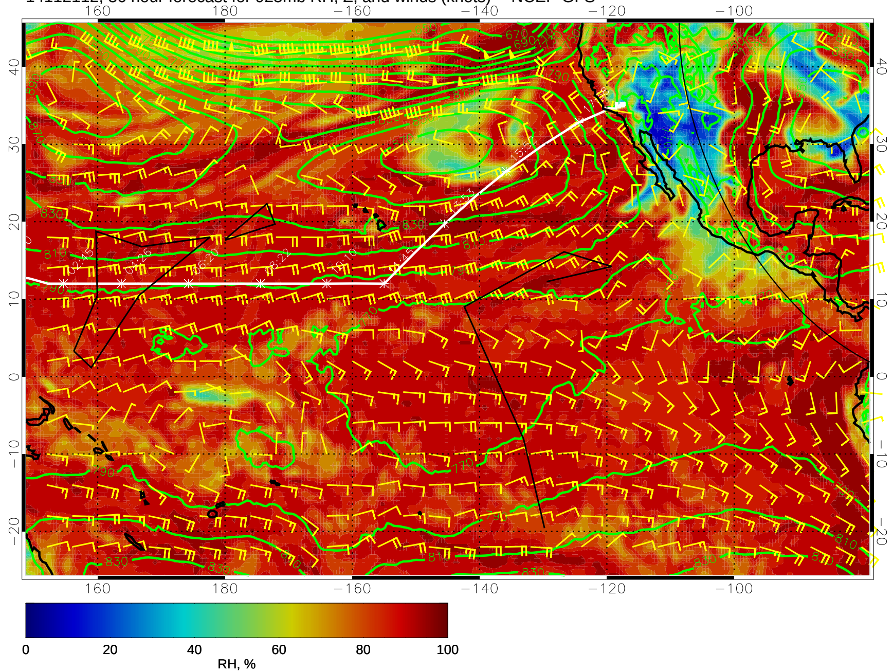
14112112, 36 hour forecast for 925mb RH, Z, and winds (knots) -- NCEP GFS
