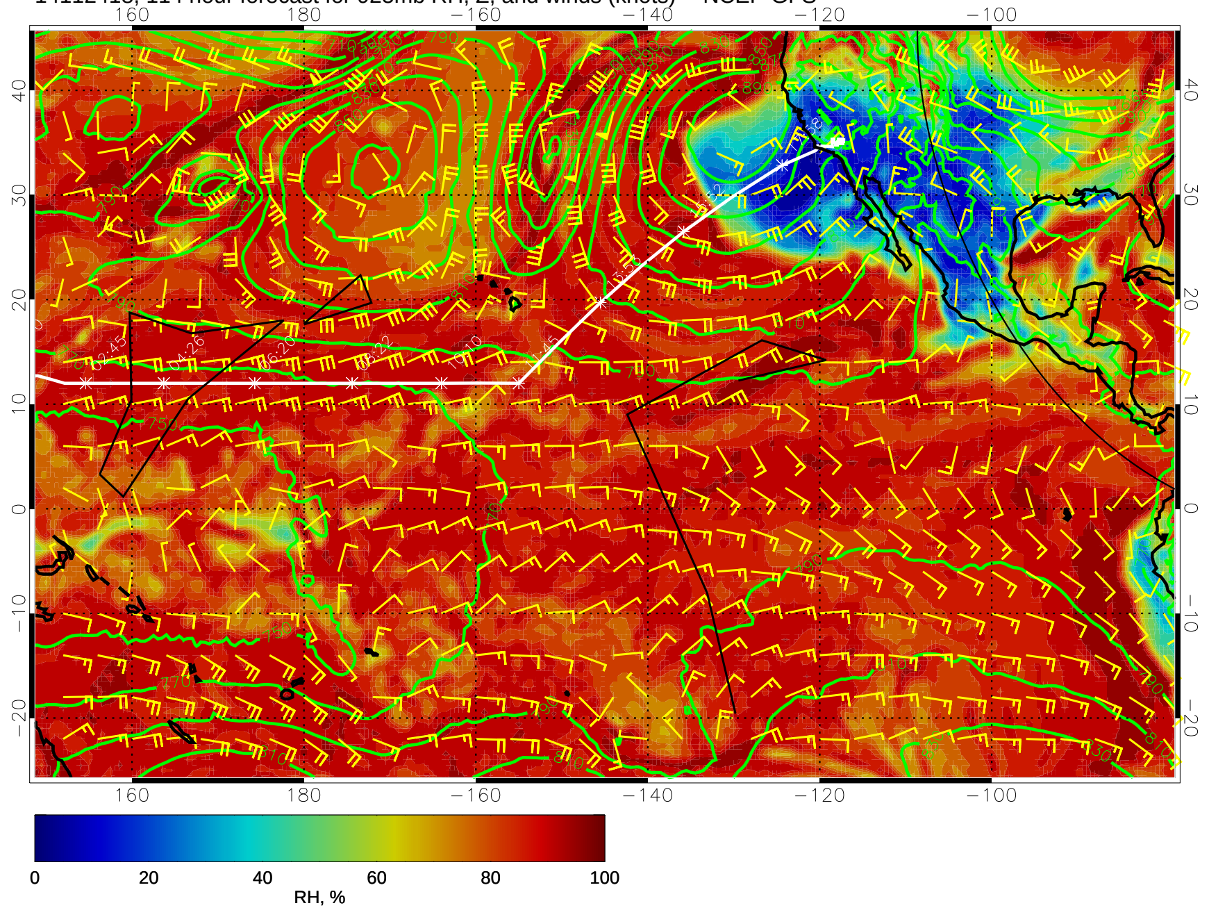
14112418, 114 hour forecast for 925mb RH, Z, and winds (knots) -- NCEP GFS
