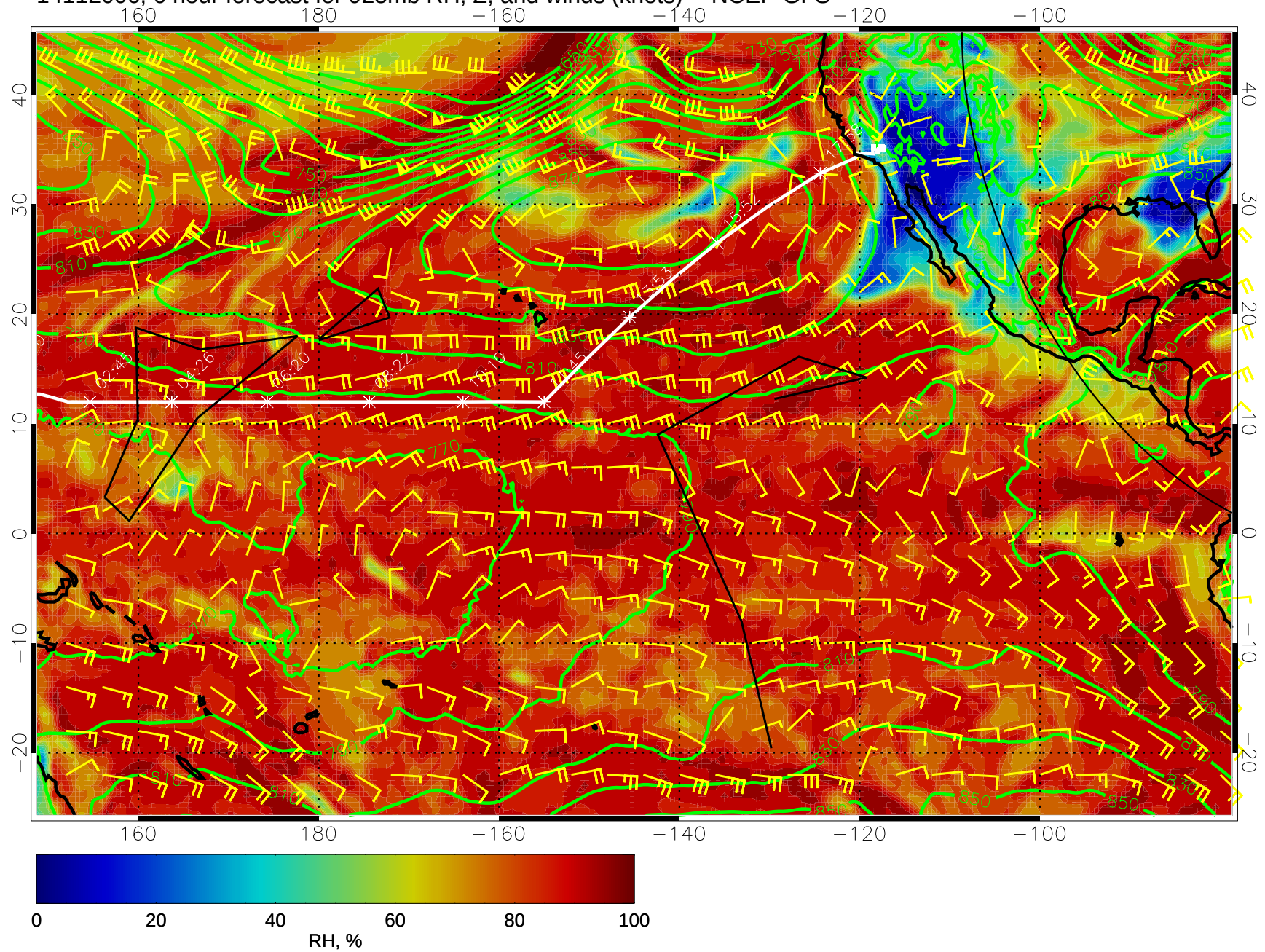
14112006, 6 hour forecast for 925mb RH, Z, and winds (knots) -- NCEP GFS
