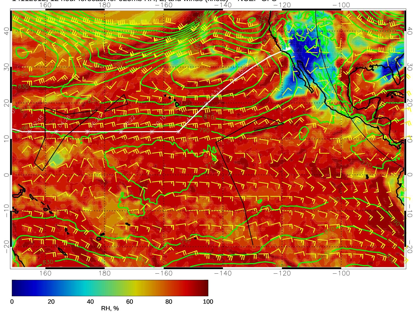
14112012, 12 hour forecast for 925mb RH, Z, and winds (knots) -- NCEP GFS
