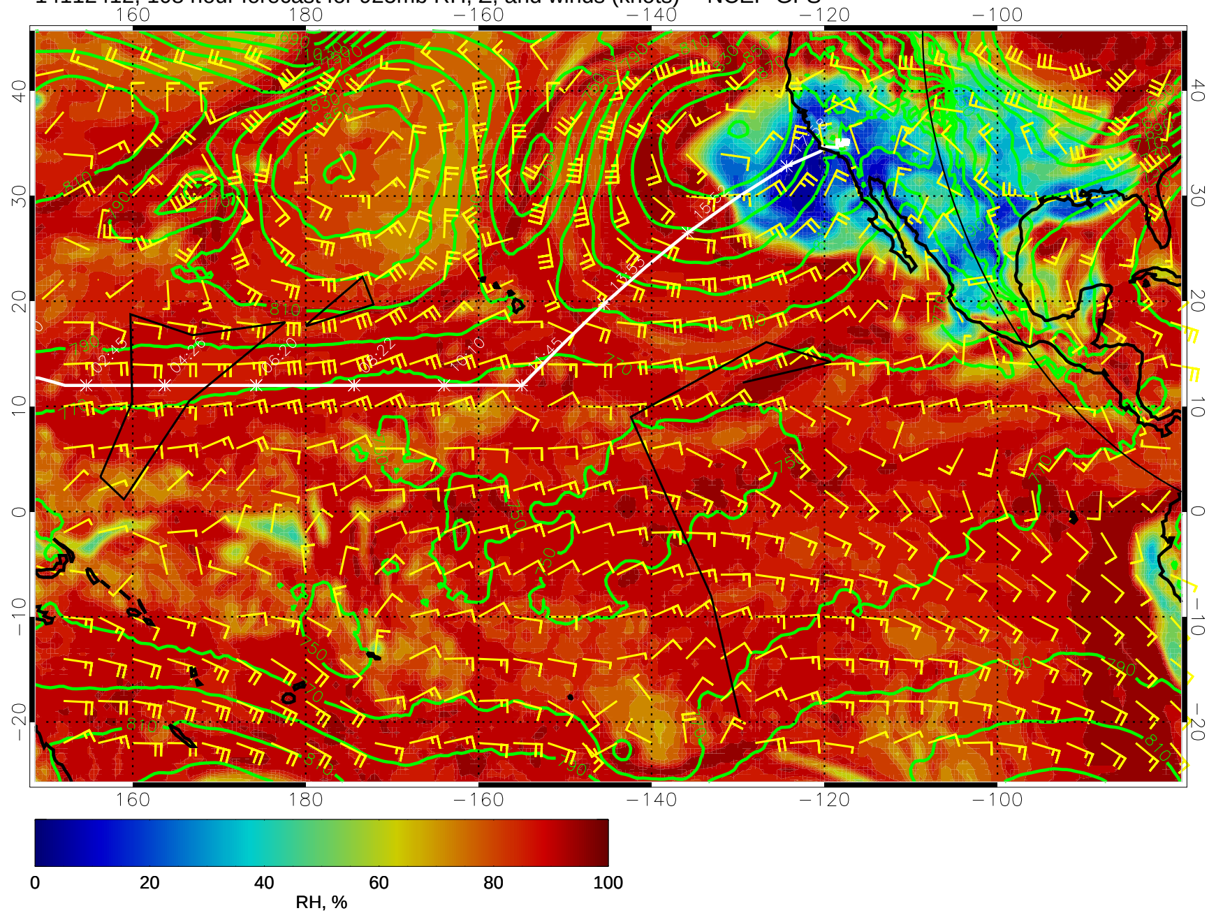
14112412, 108 hour forecast for 925mb RH, Z, and winds (knots) -- NCEP GFS
