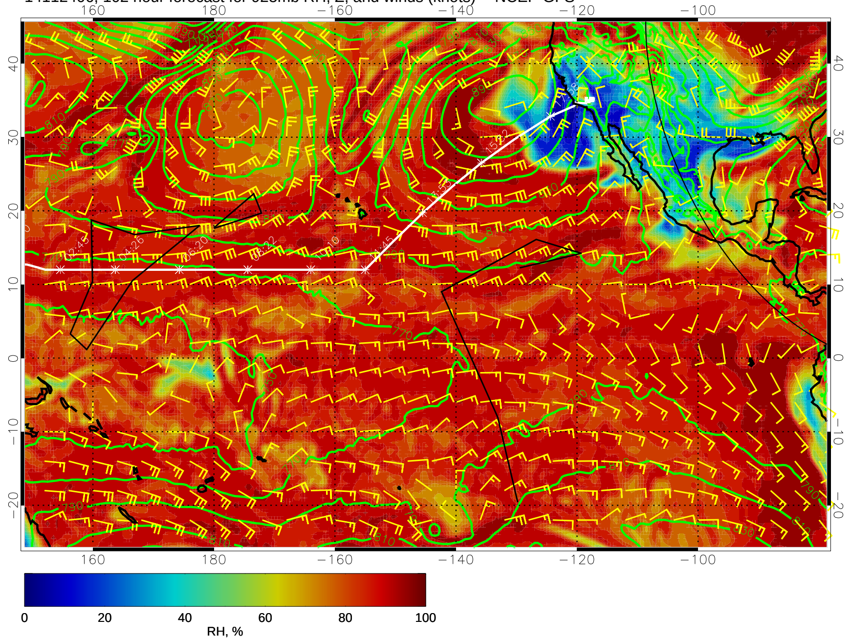
14112406, 102 hour forecast for 925mb RH, Z, and winds (knots) -- NCEP GFS
