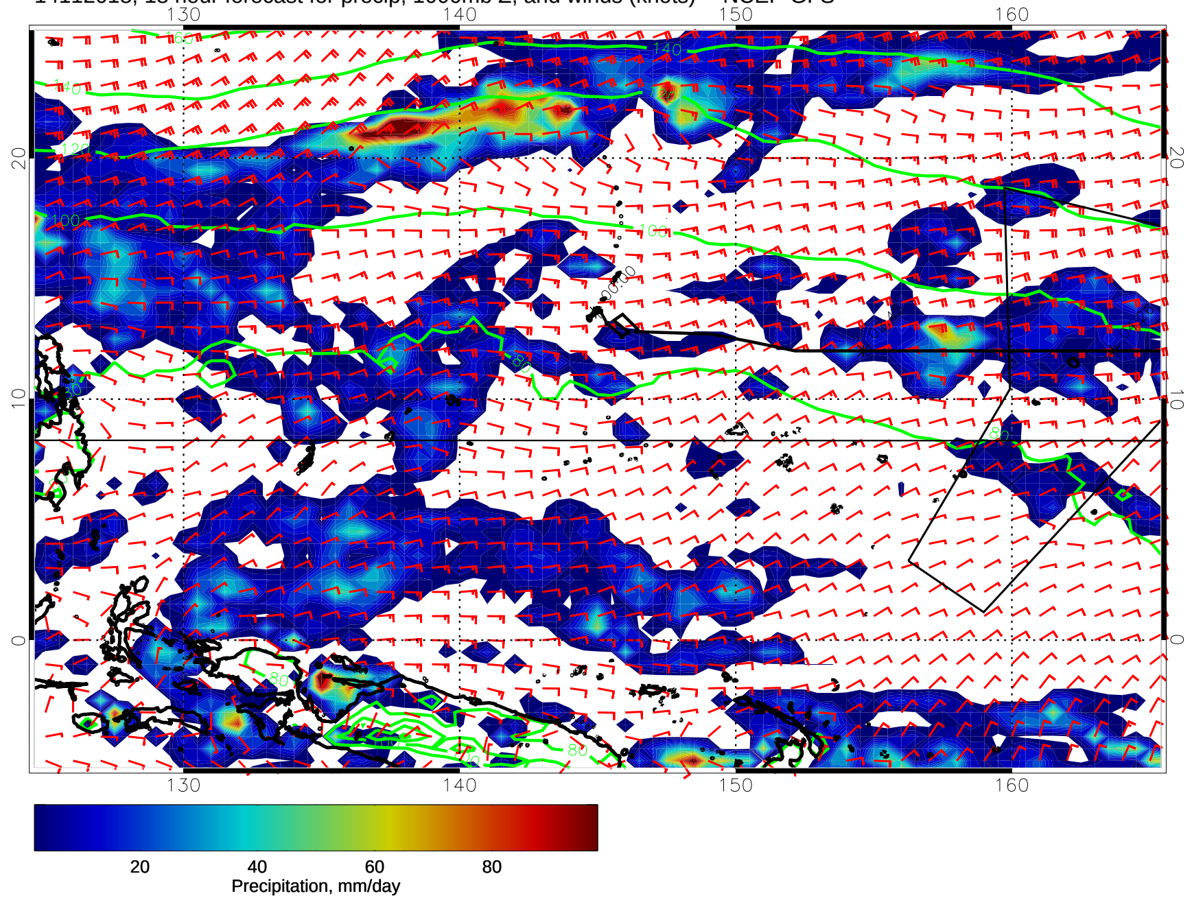
14112018, 18 hour forecast for precip, 1000mb Z, and winds (knots) -- NCEP GFS
