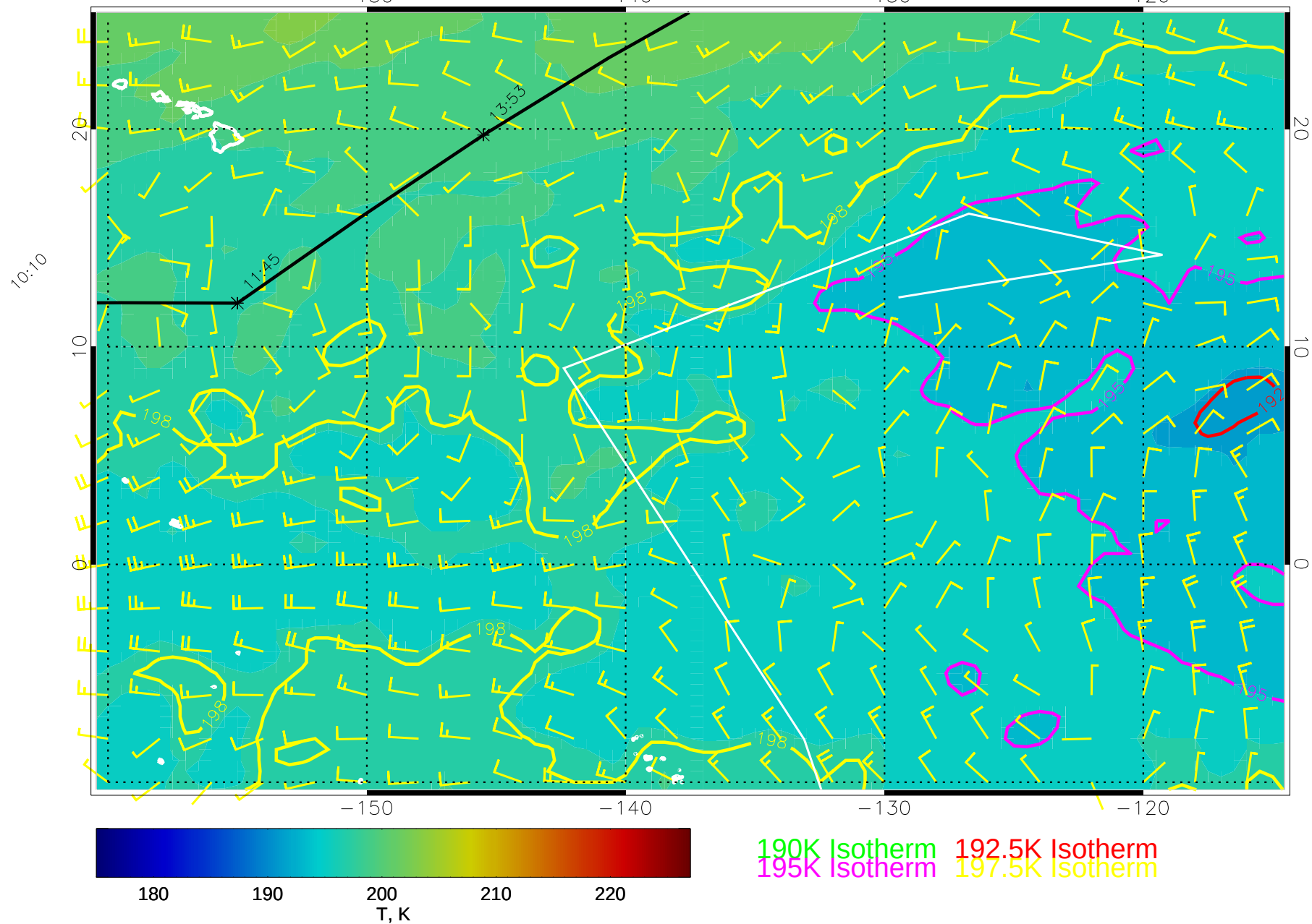
14112406, 102 hour forecast for 70mb T and winds (knots) -- NCEP GFS
