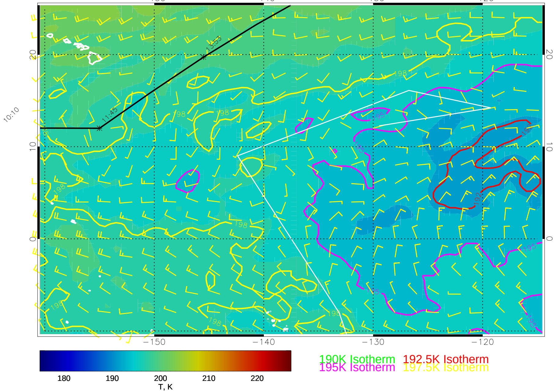
14112500, 120 hour forecast for 70mb T and winds (knots) -- NCEP GFS
