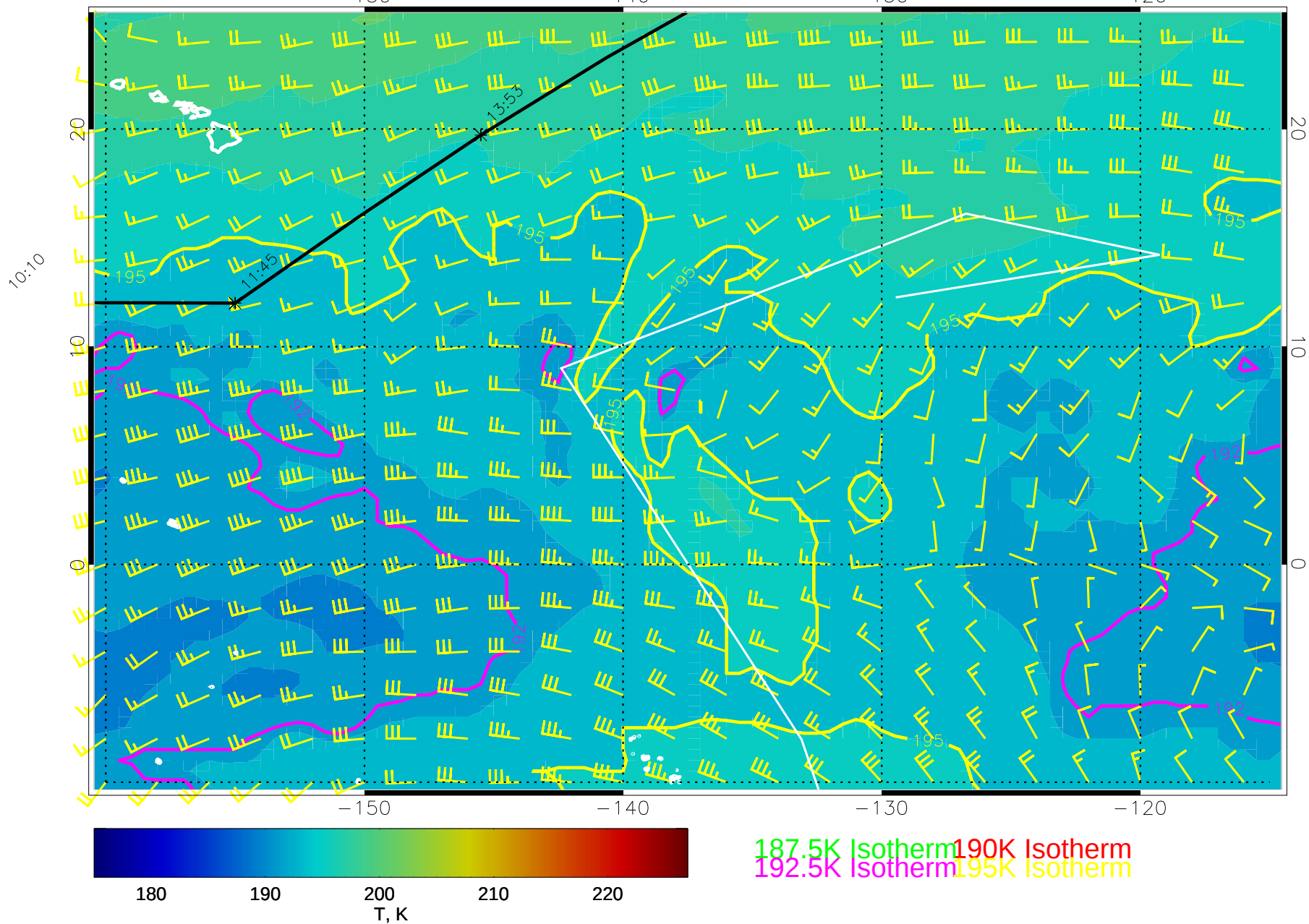
14112012, 12 hour forecast for 100mb T and winds (knots) -- NCEP GFS
