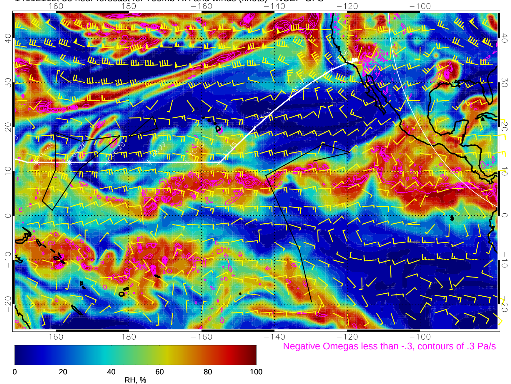
14112112, 36 hour forecast for 700mb RH and winds (knots) - NCEP GFS
