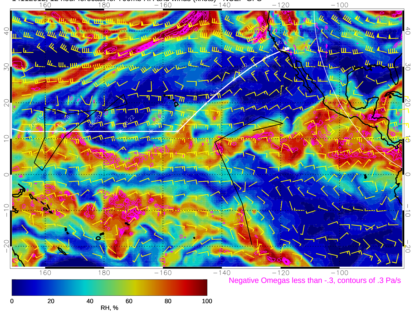
14112012, 12 hour forecast for 700mb RH and winds (knots) - NCEP GFS
