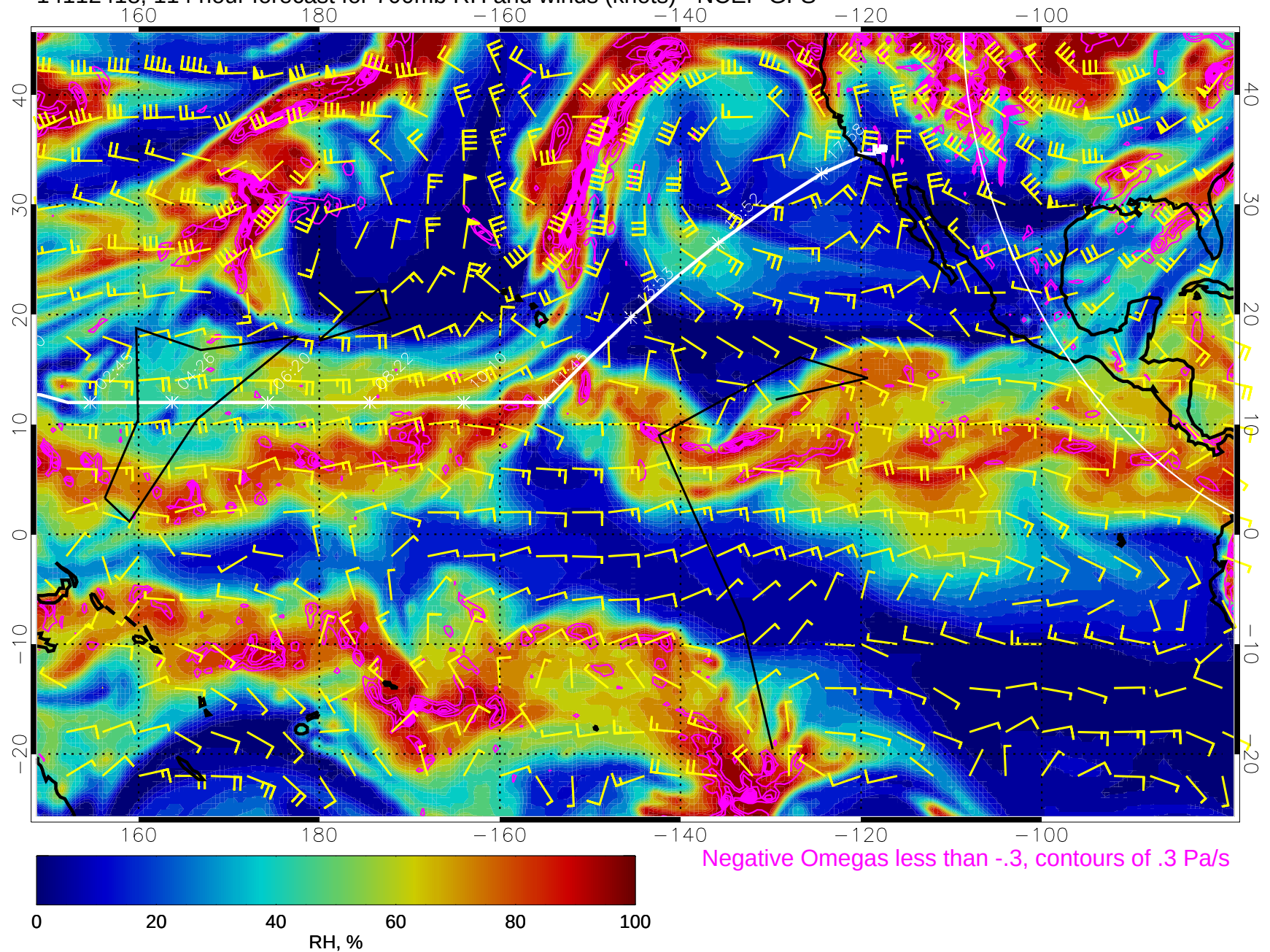
14112418, 114 hour forecast for 700mb RH and winds (knots) - NCEP GFS
