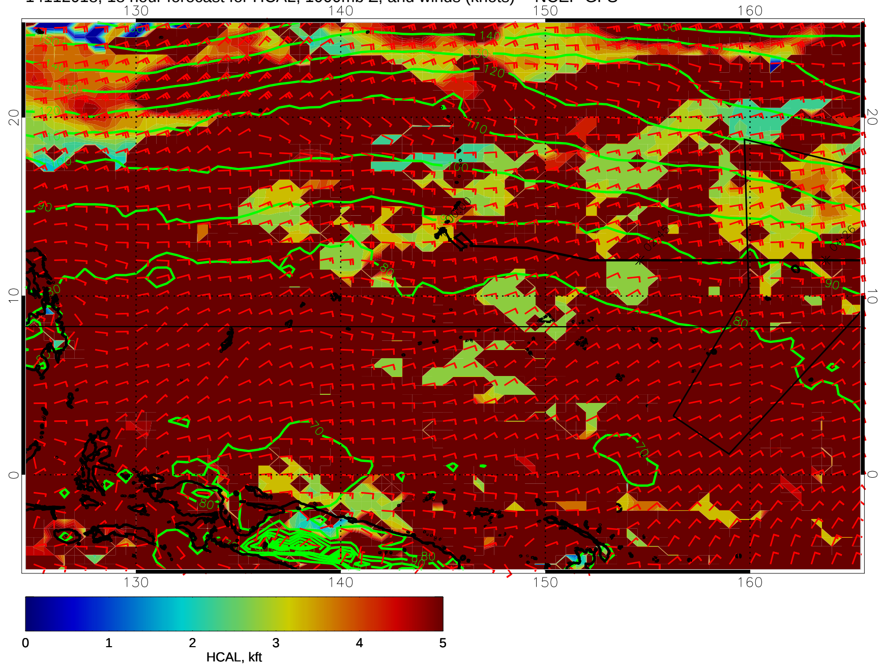
14112018, 18 hour forecast for HCAL, 1000mb Z, and winds (knots) -- NCEP GFS
