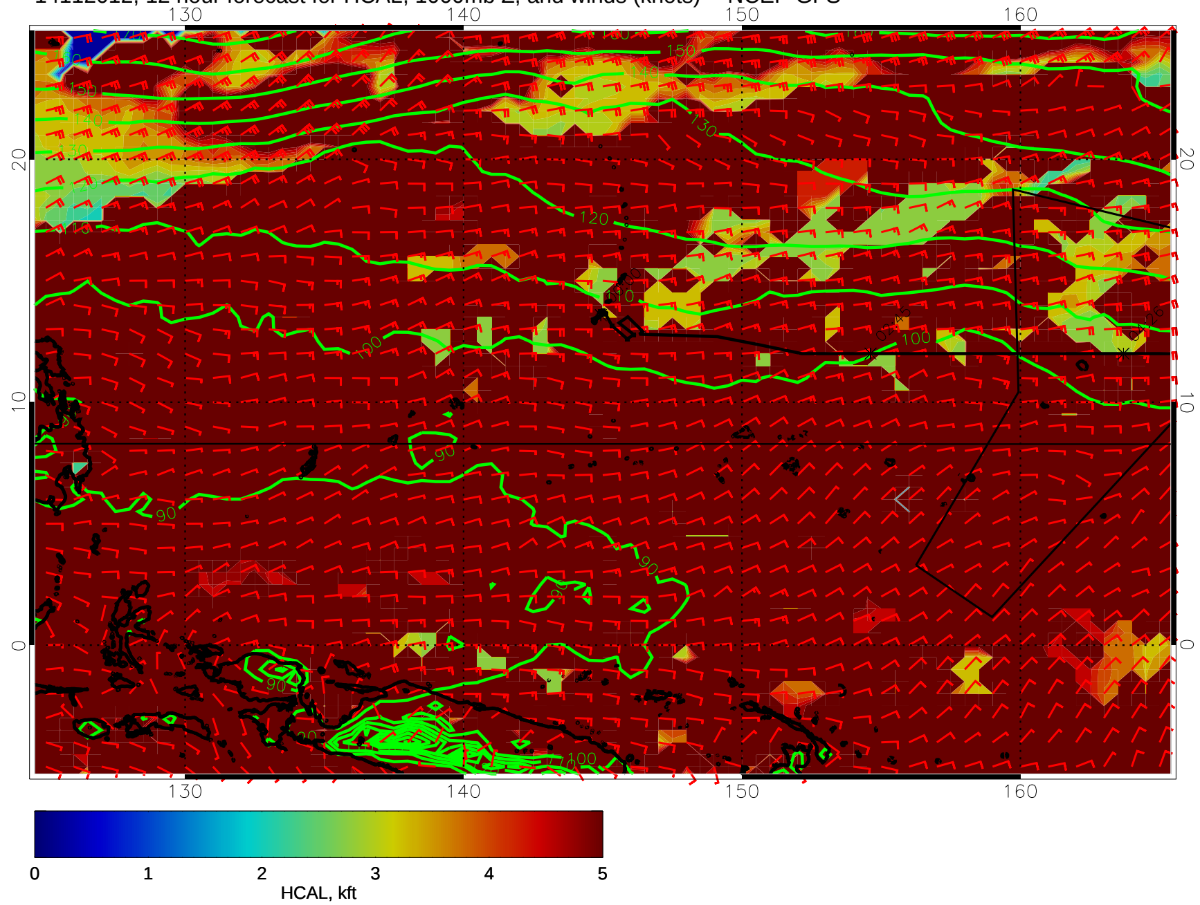
14112012, 12 hour forecast for HCAL, 1000mb Z, and winds (knots) -- NCEP GFS
