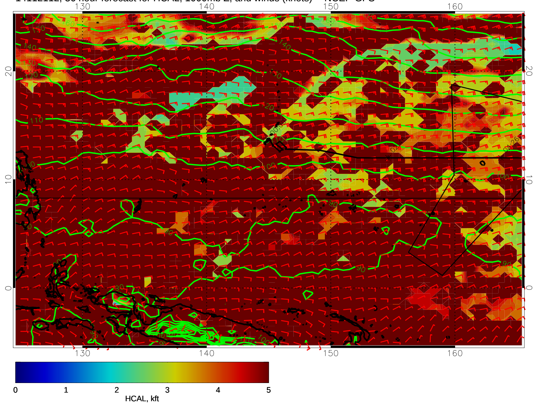
14112112, 36 hour forecast for HCAL, 1000mb Z, and winds (knots) -- NCEP GFS
