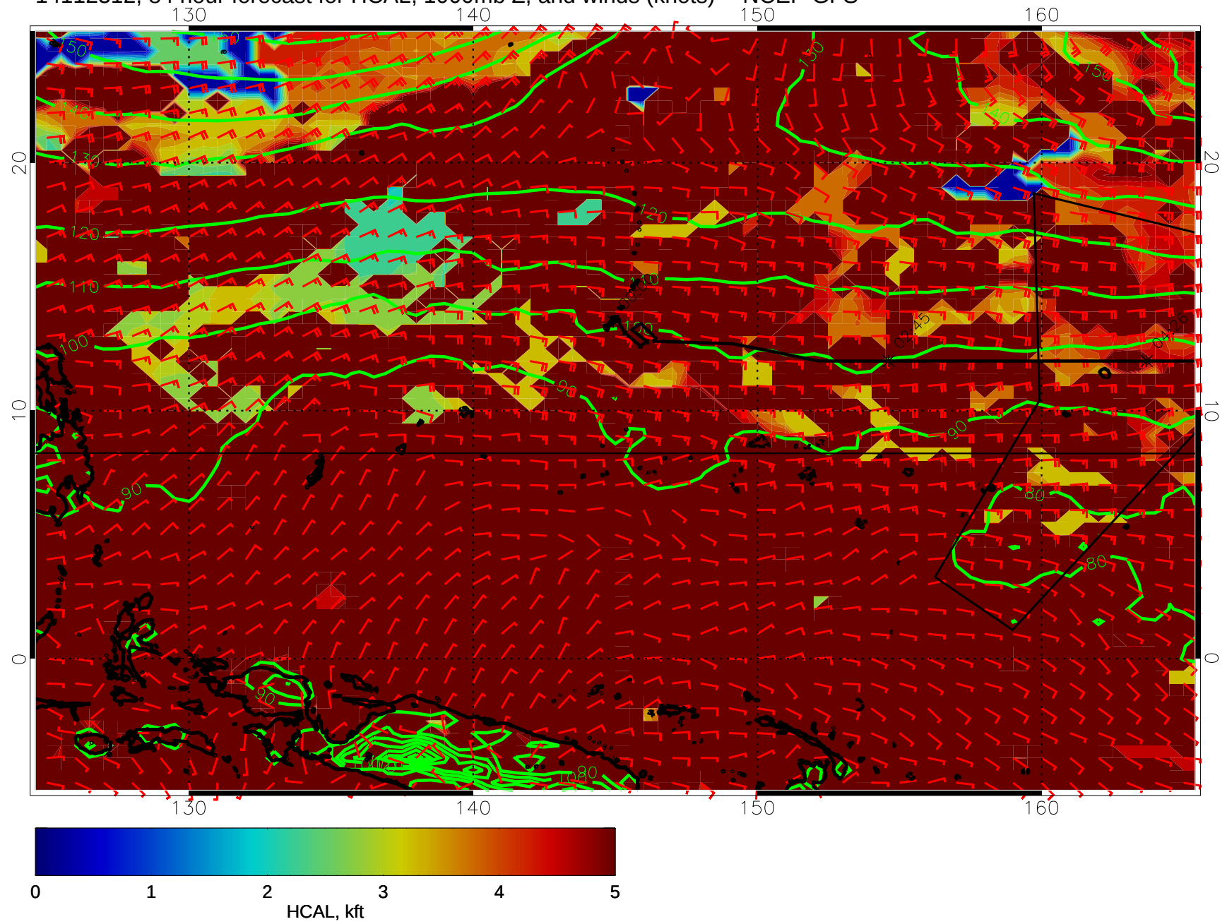
14112312, 84 hour forecast for HCAL, 1000mb Z, and winds (knots) -- NCEP GFS
