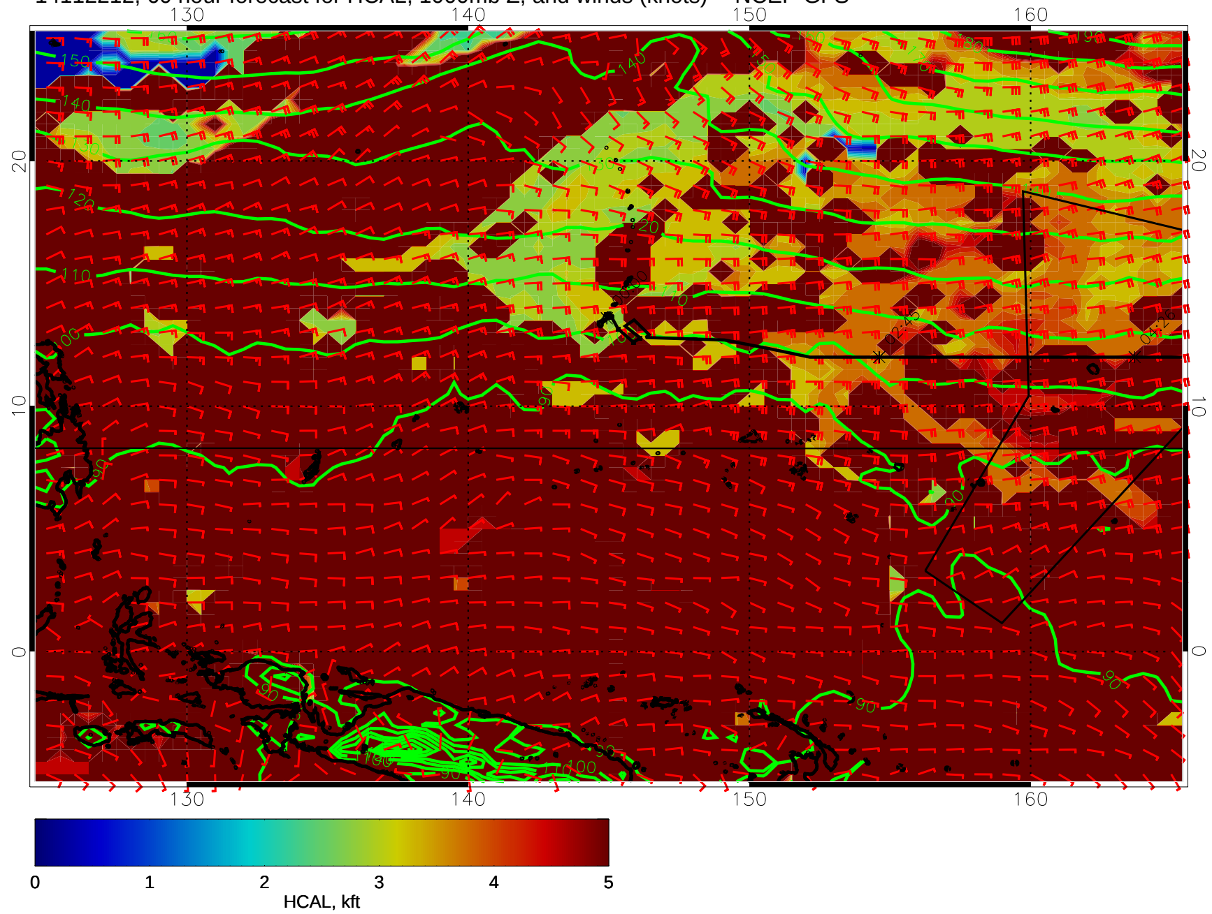
14112212, 60 hour forecast for HCAL, 1000mb Z, and winds (knots) -- NCEP GFS
