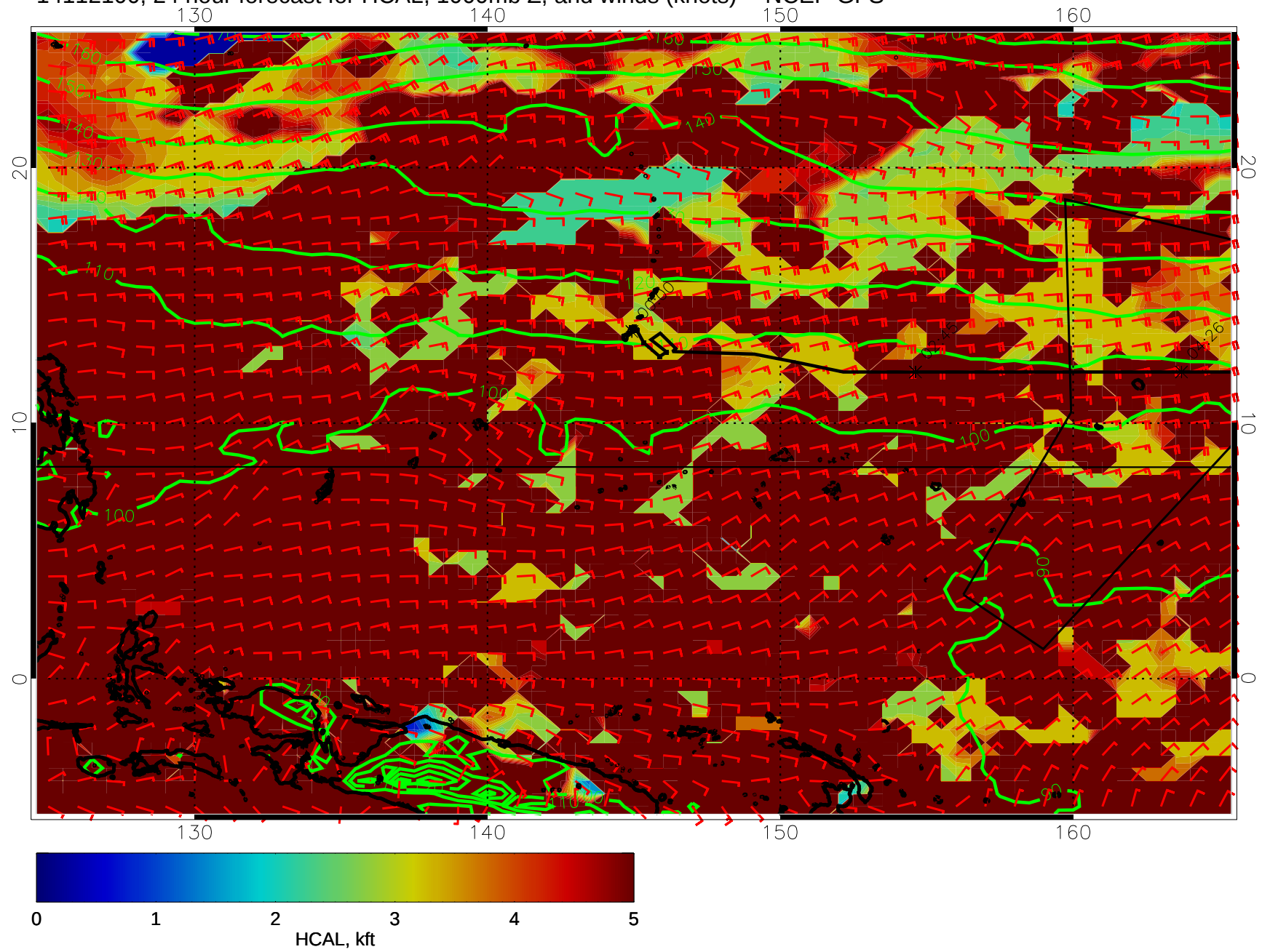
14112100, 24 hour forecast for HCAL, 1000mb Z, and winds (knots) -- NCEP GFS
