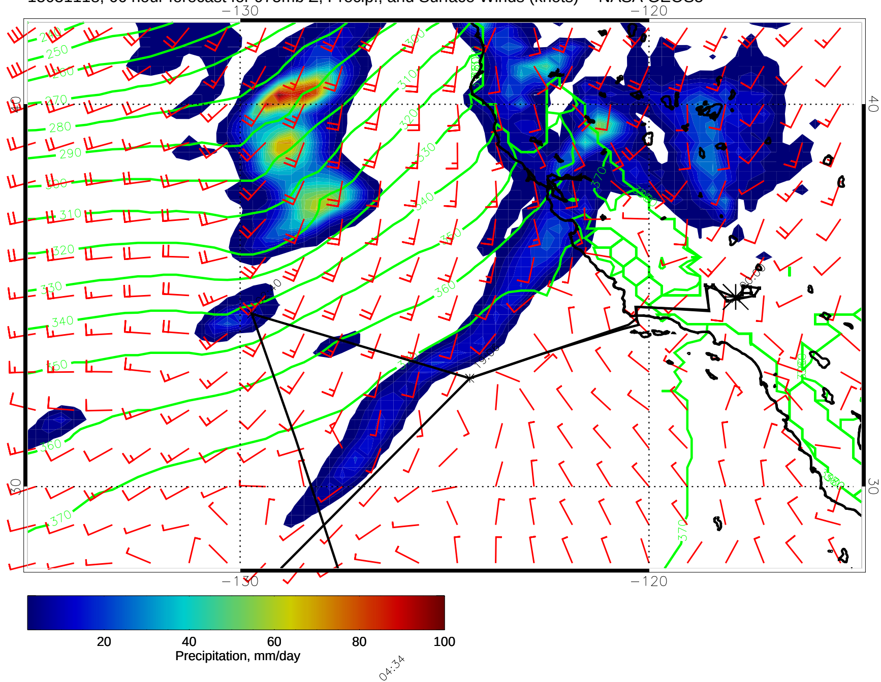
15031118, 66 hour forecast for 975mb Z, Precip., and Surface Winds (knots) -- NASA GEOS5
