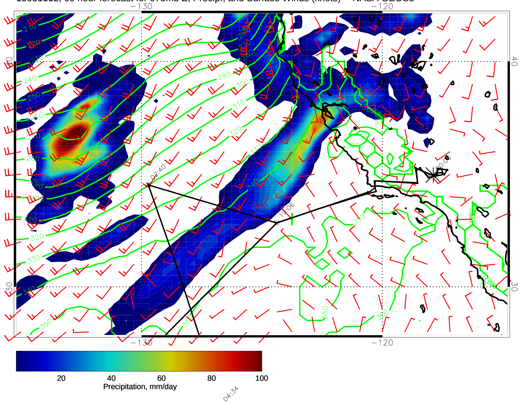
15031112, 60 hour forecast for 975mb Z, Precip., and Surface Winds (knots) -- NASA GEOS5
