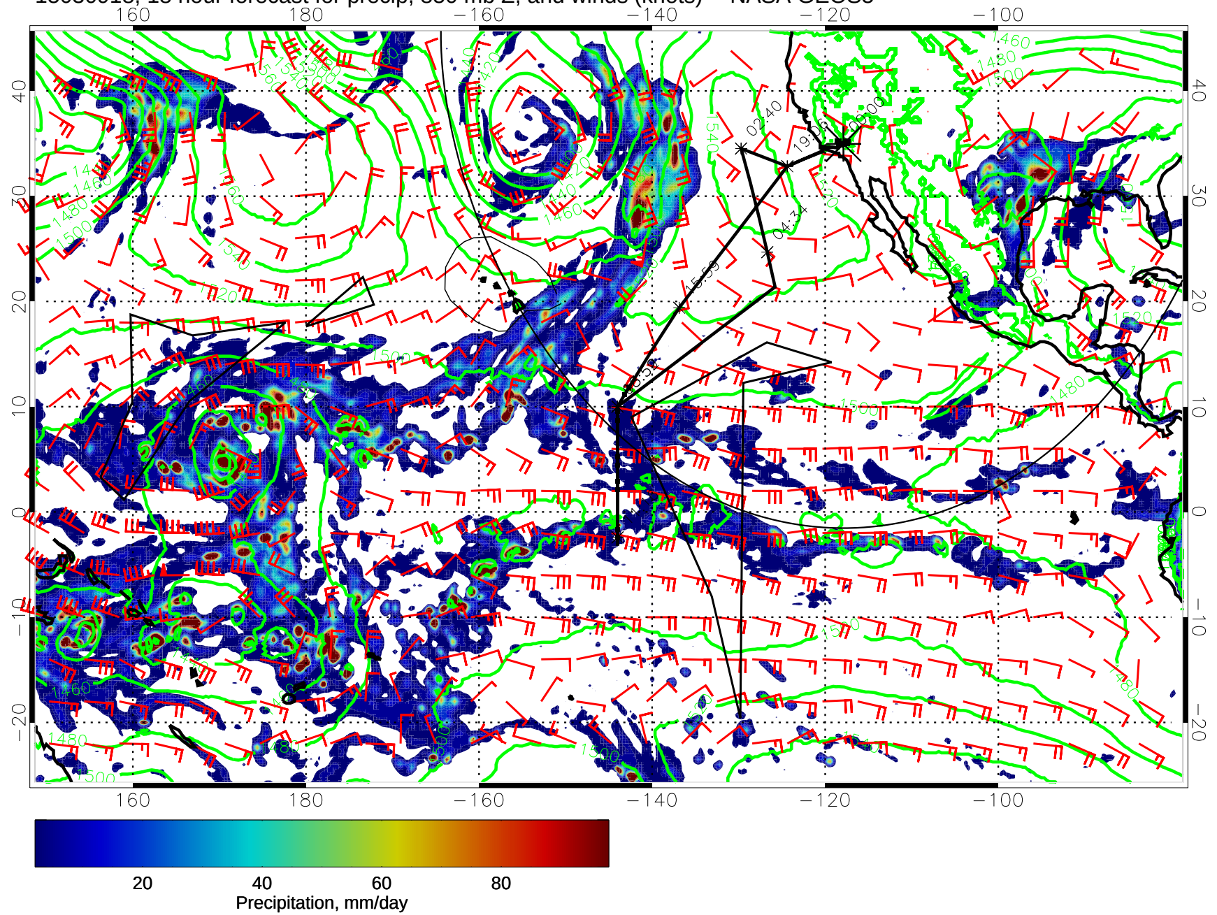
15030918, 18 hour forecast for precip, 850 mb Z, and winds (knots) -- NASA GEOS5
