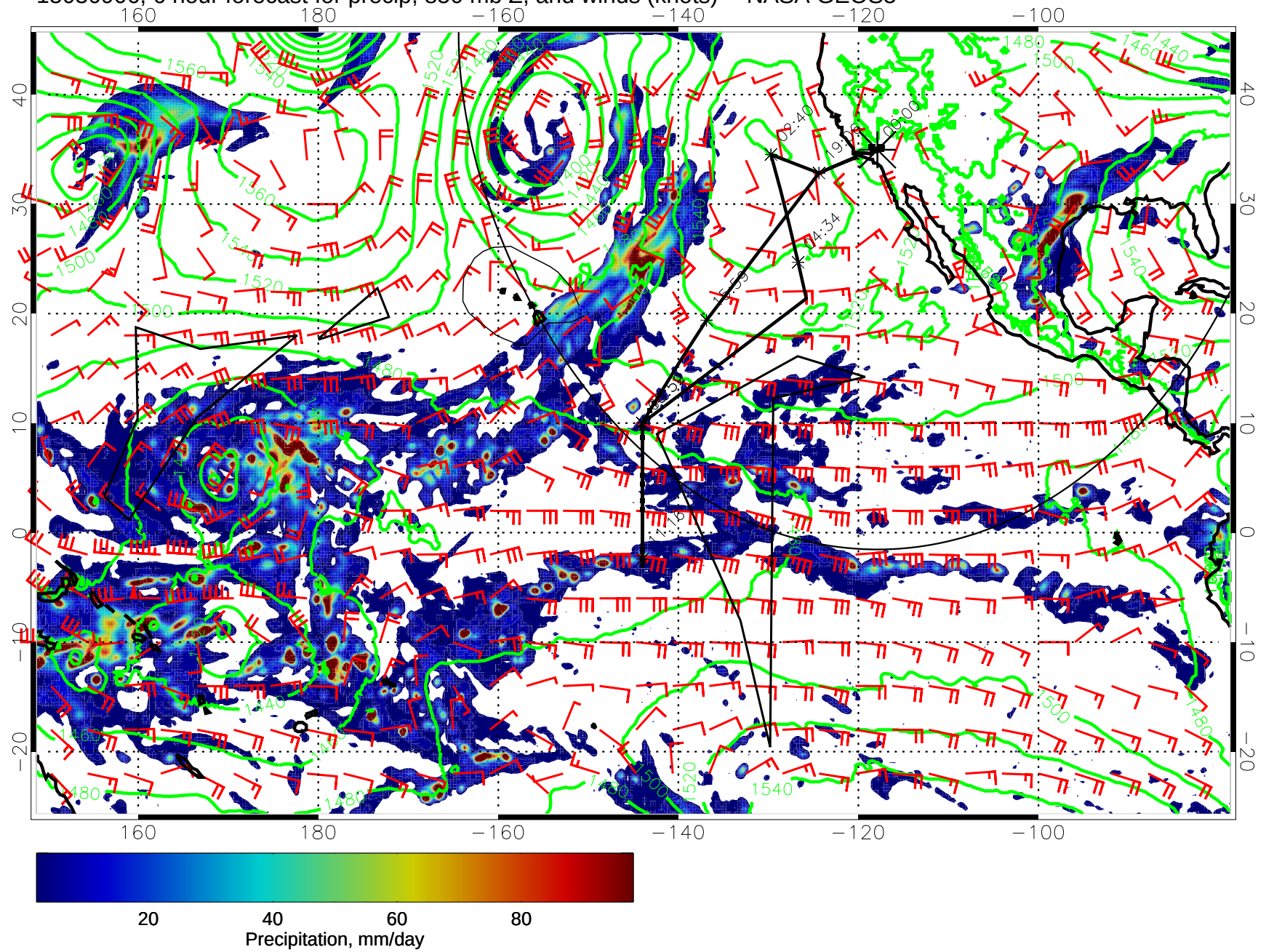
15030906, 6 hour forecast for precip, 850 mb Z, and winds (knots) -- NASA GEOS5
