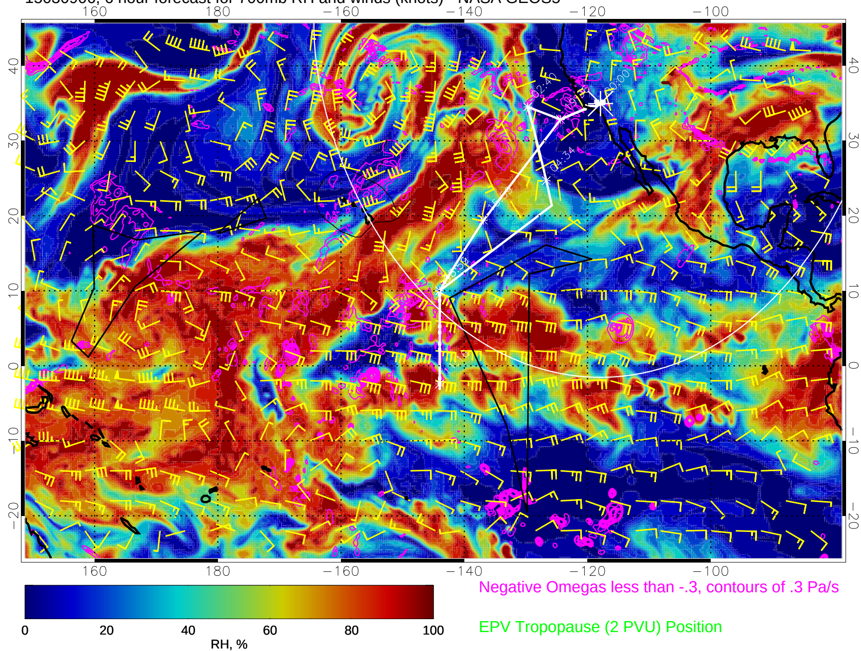
15030906, 6 hour forecast for 700mb RH and winds (knots) - NASA GEOS5
