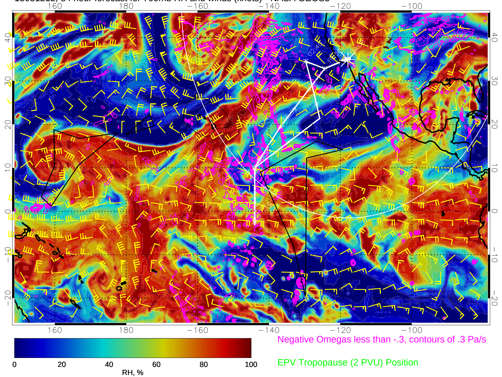
15031212, 84 hour forecast for 700mb RH and winds (knots) - NASA GEOS5
