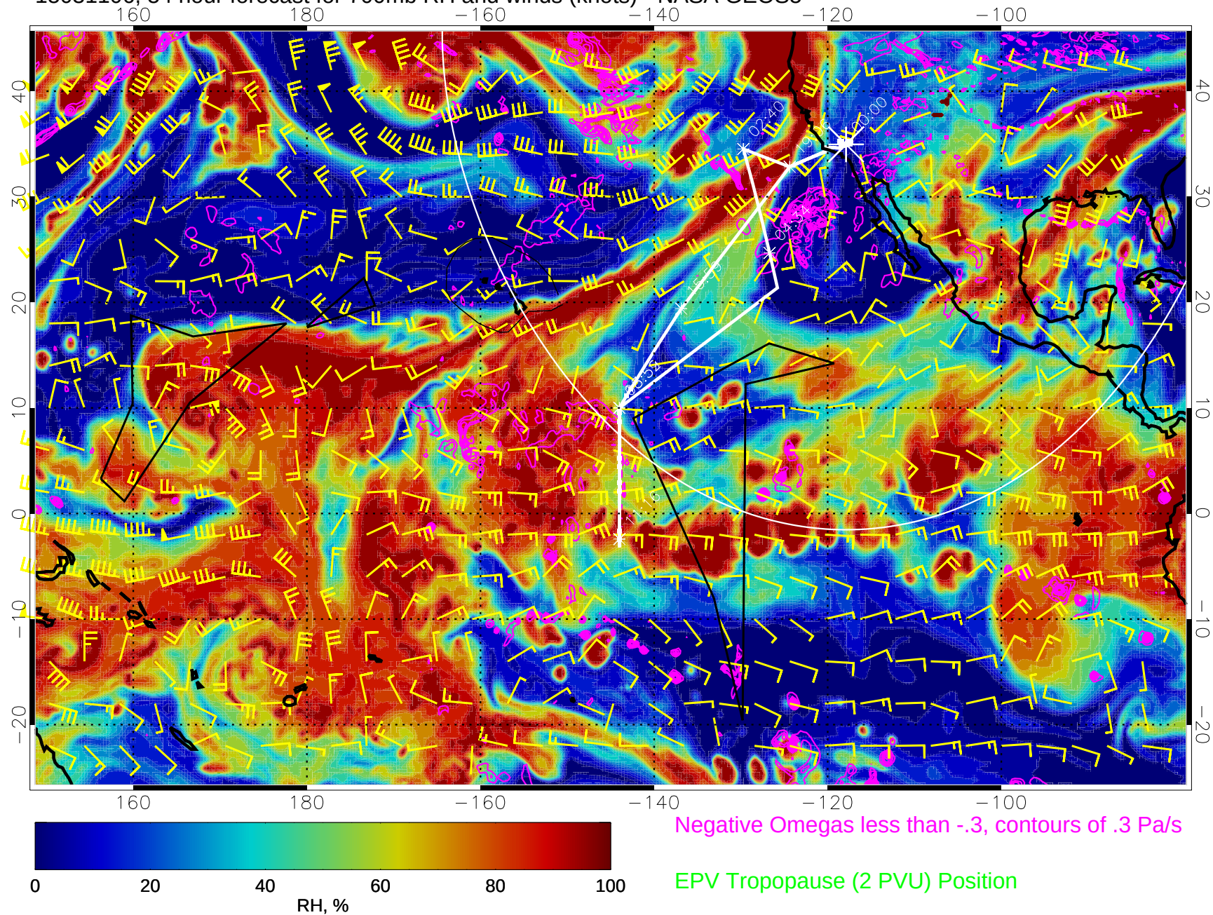
15031106, 54 hour forecast for 700mb RH and winds (knots) - NASA GEOS5
