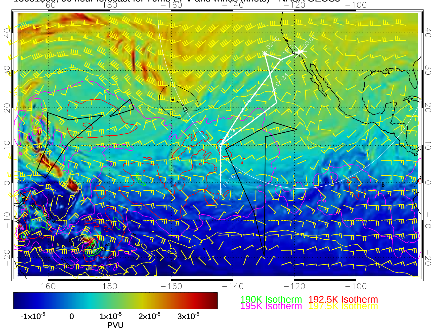
15031300, 96 hour forecast for 70mb EPV and winds (knots)-- NASA GEOS5
