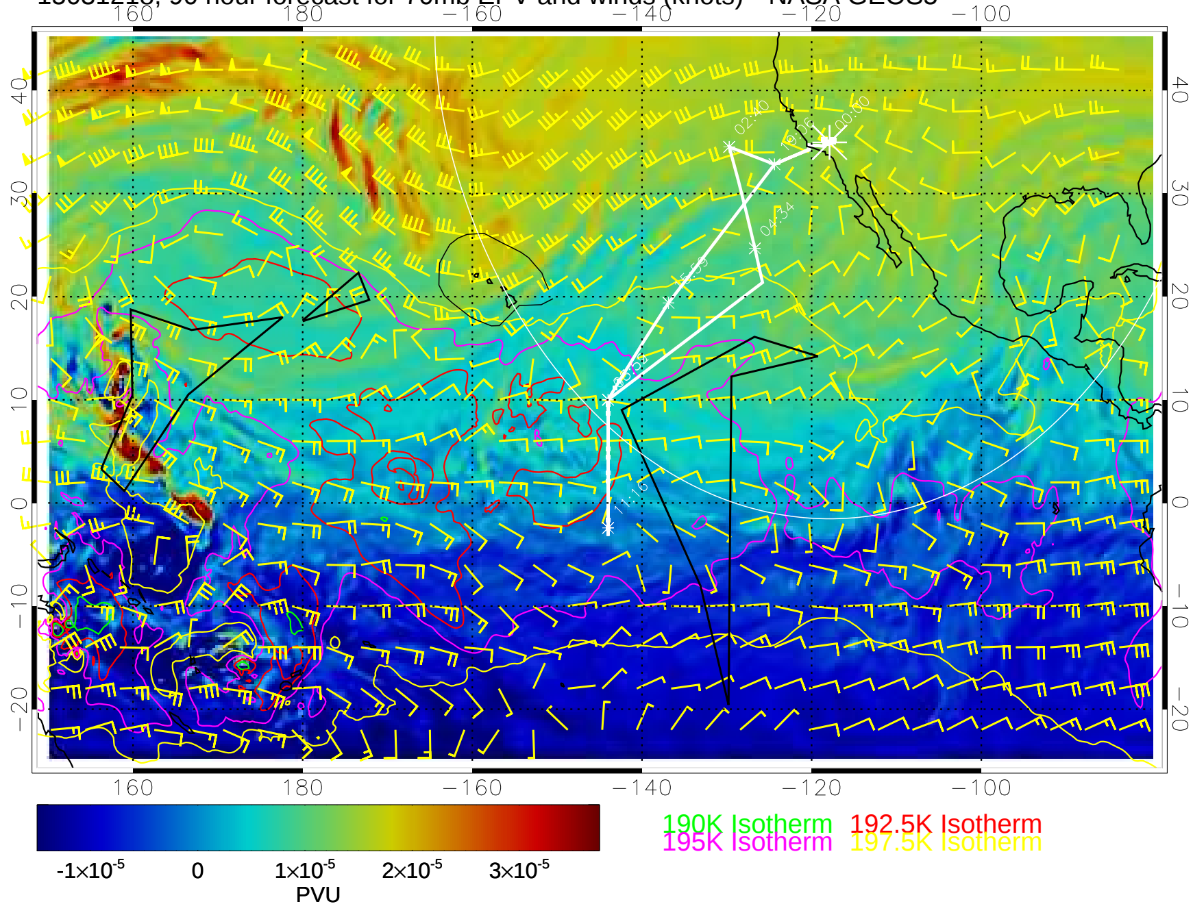
15031218, 90 hour forecast for 70mb EPV and winds (knots)-- NASA GEOS5
