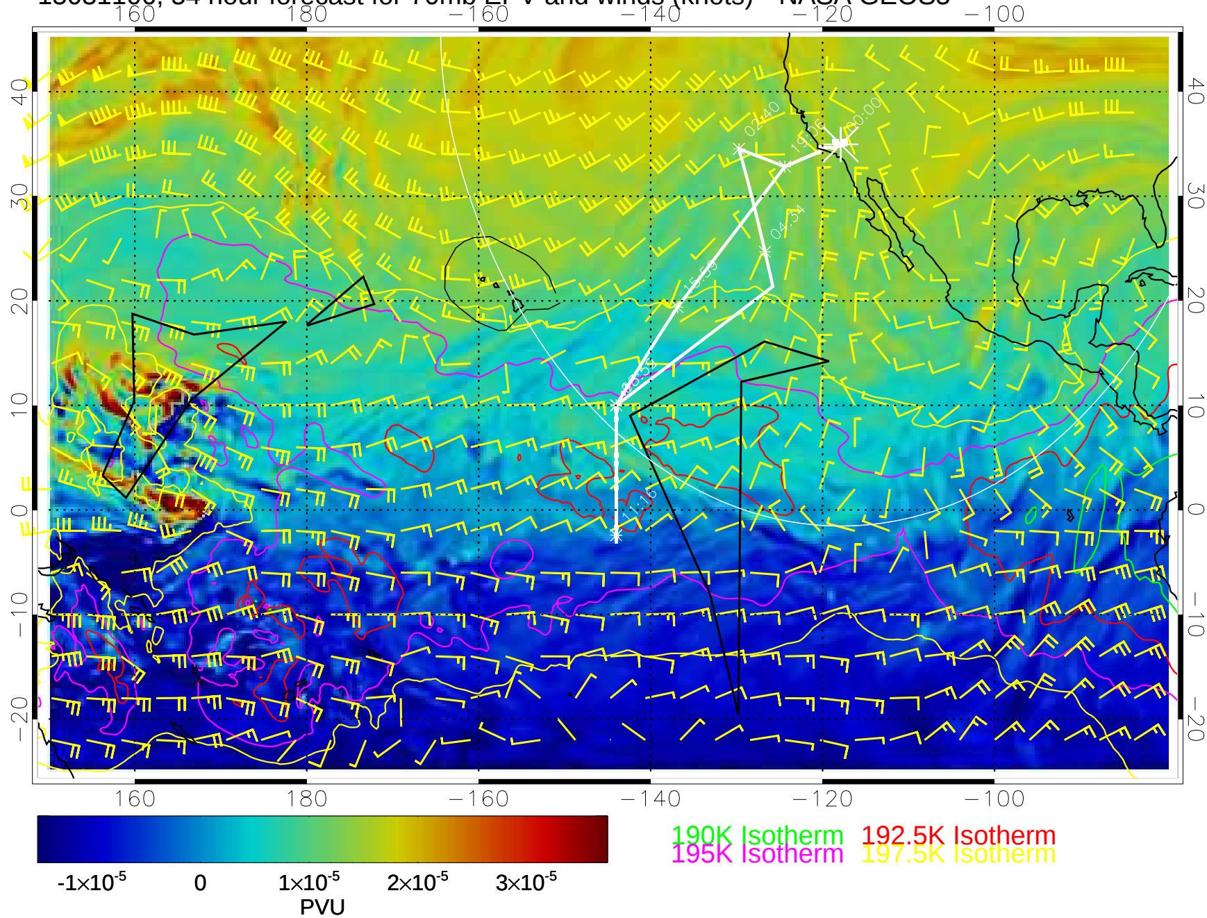
15031106, 54 hour forecast for 70mb EPV and winds (knots)-- NASA GEOS5
