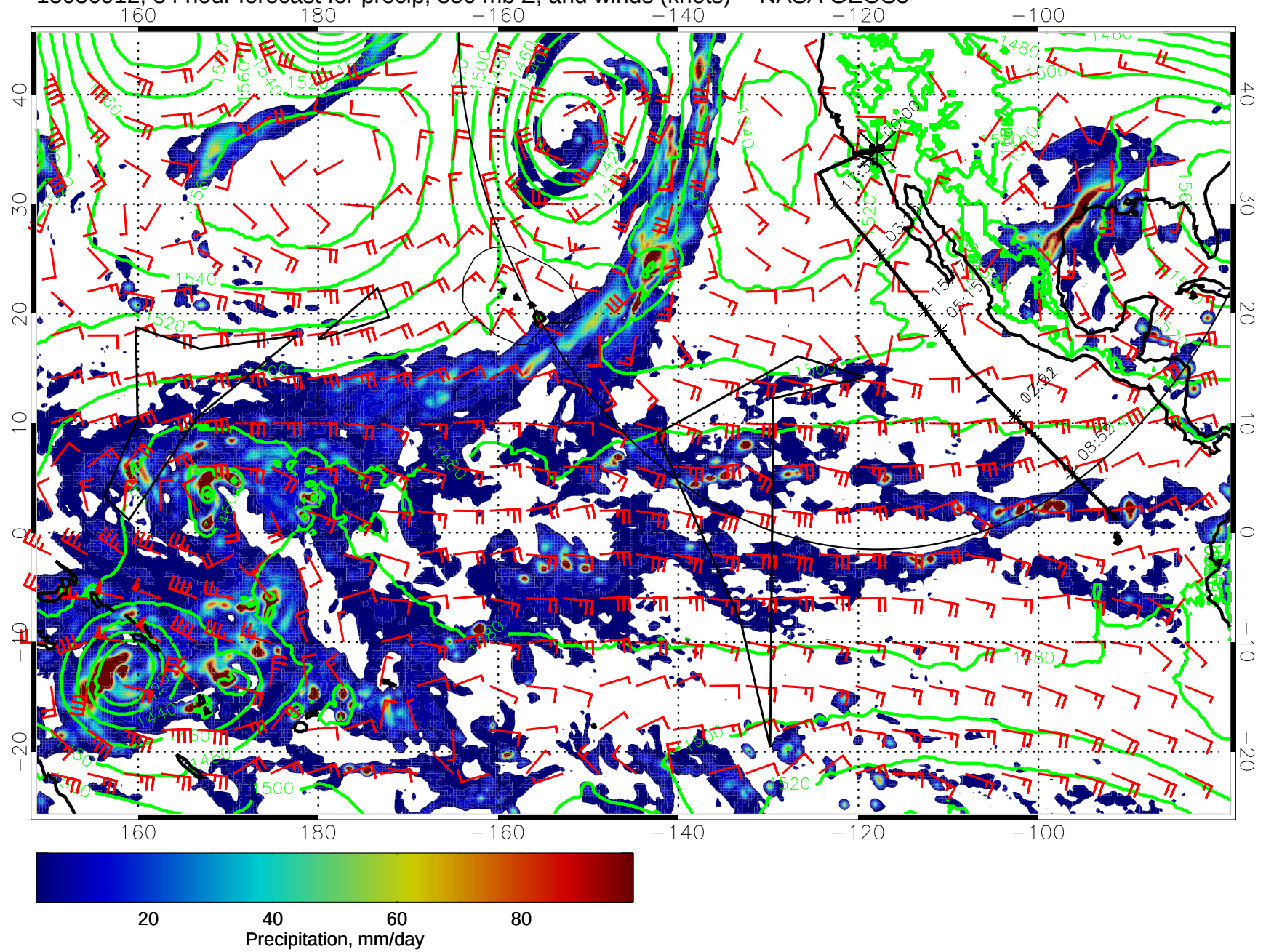
15030912, 84 hour forecast for precip, 850 mb Z, and winds (knots) -- NASA GEOS5
