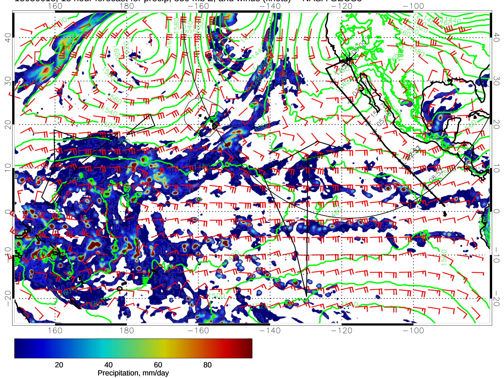
15030618, 18 hour forecast for precip, 850 mb Z, and winds (knots) -- NASA GEOS5
