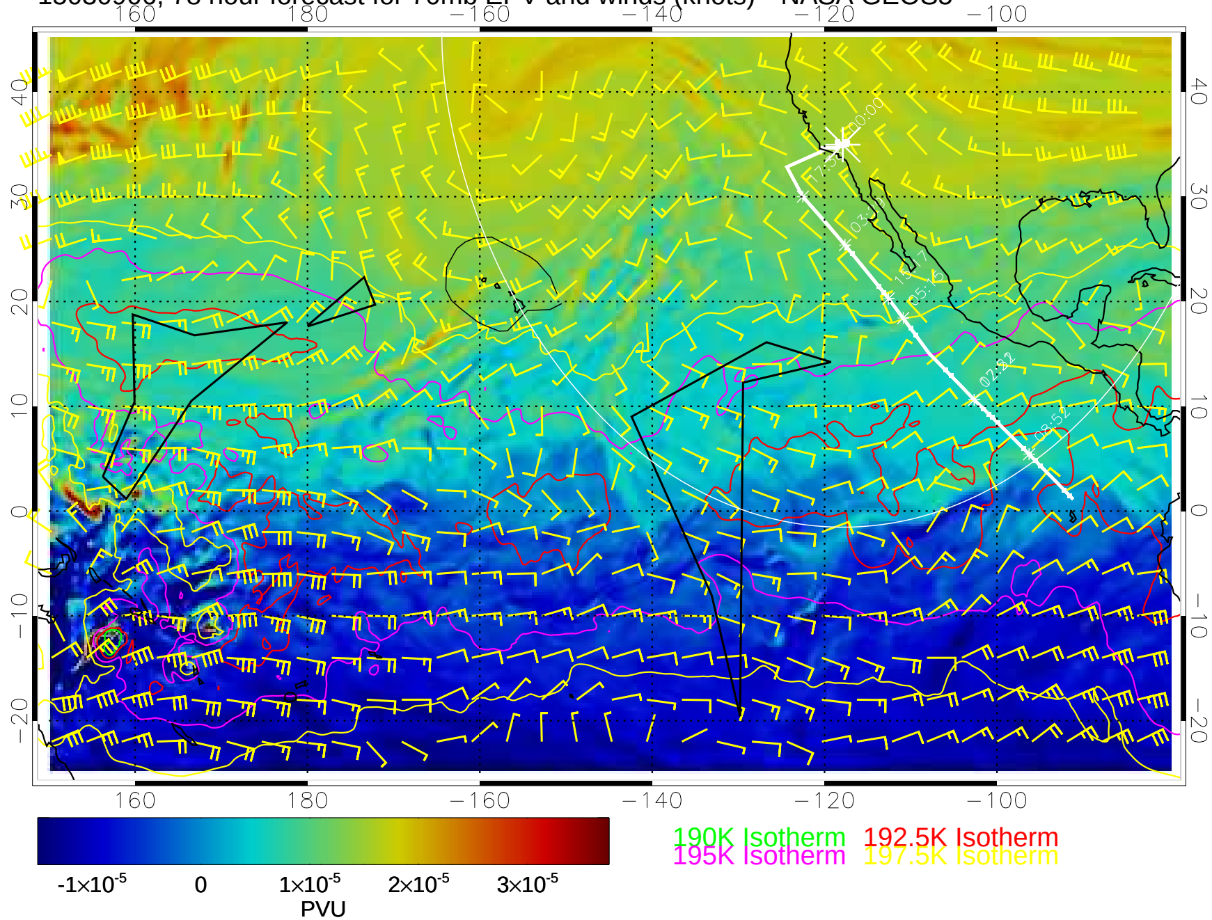
15030906, 78 hour forecast for 70mb EPV and winds (knots)-- NASA GEOS5
