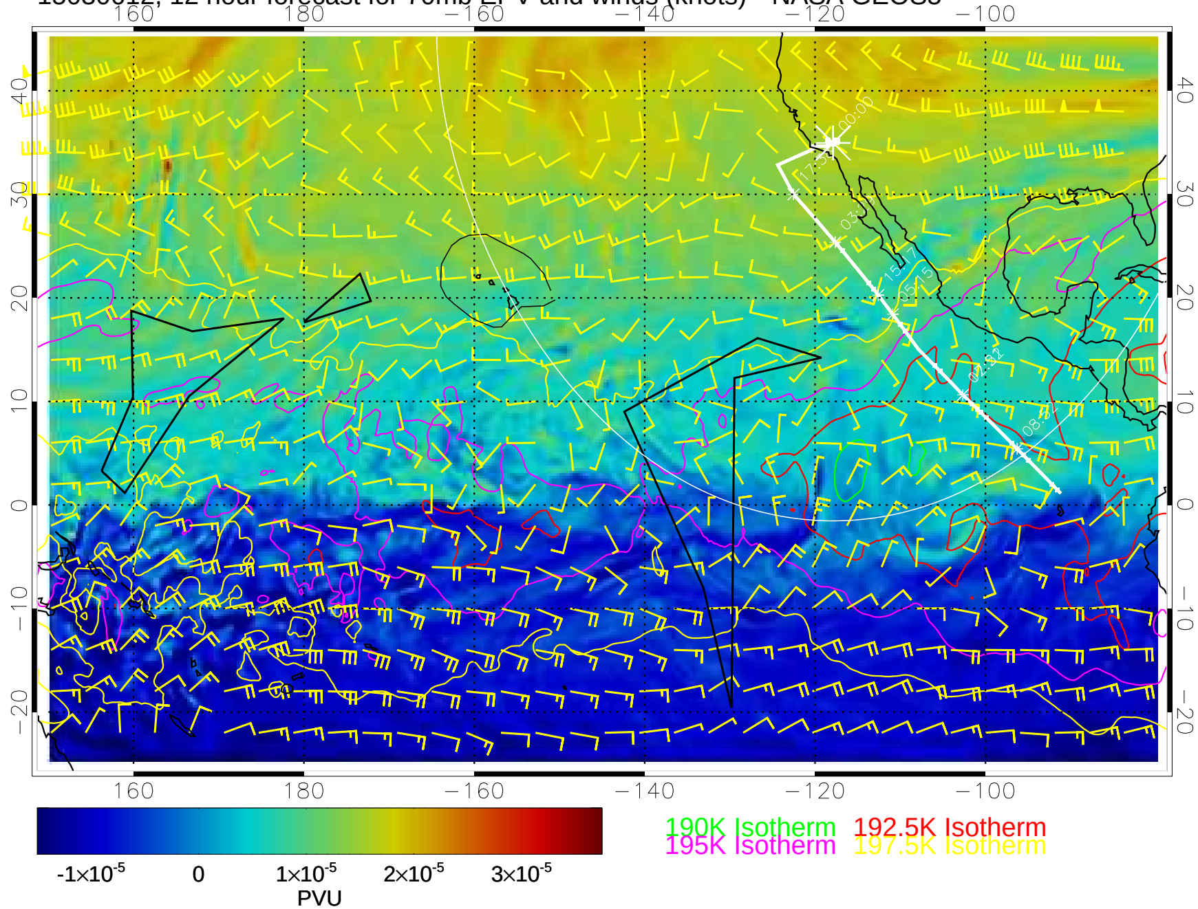
15030612, 12 hour forecast for 70mb EPV and winds (knots)-- NASA GEOS5
