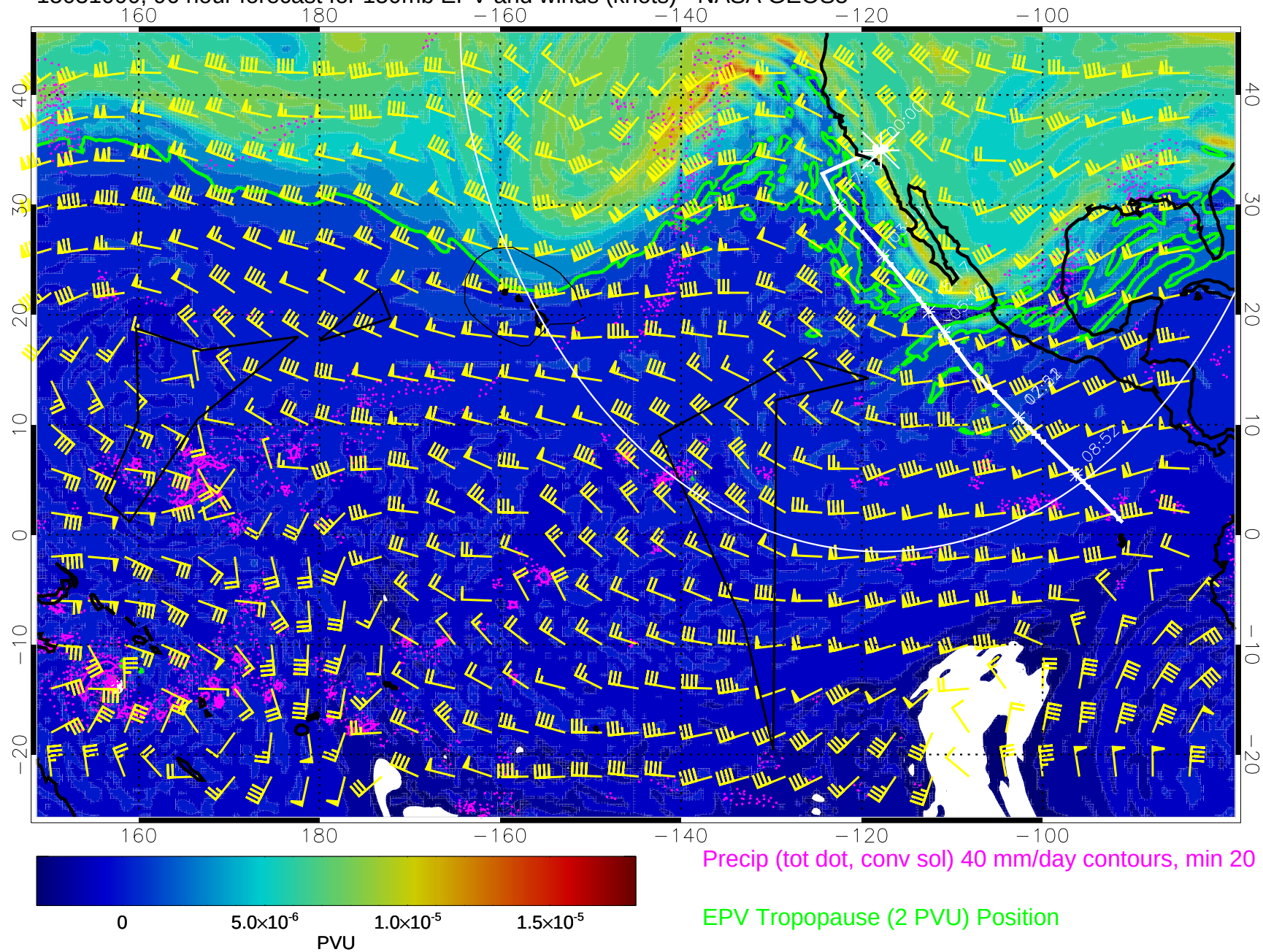
15031000, 96 hour forecast for 150mb EPV and winds (knots) - NASA GEOS5
