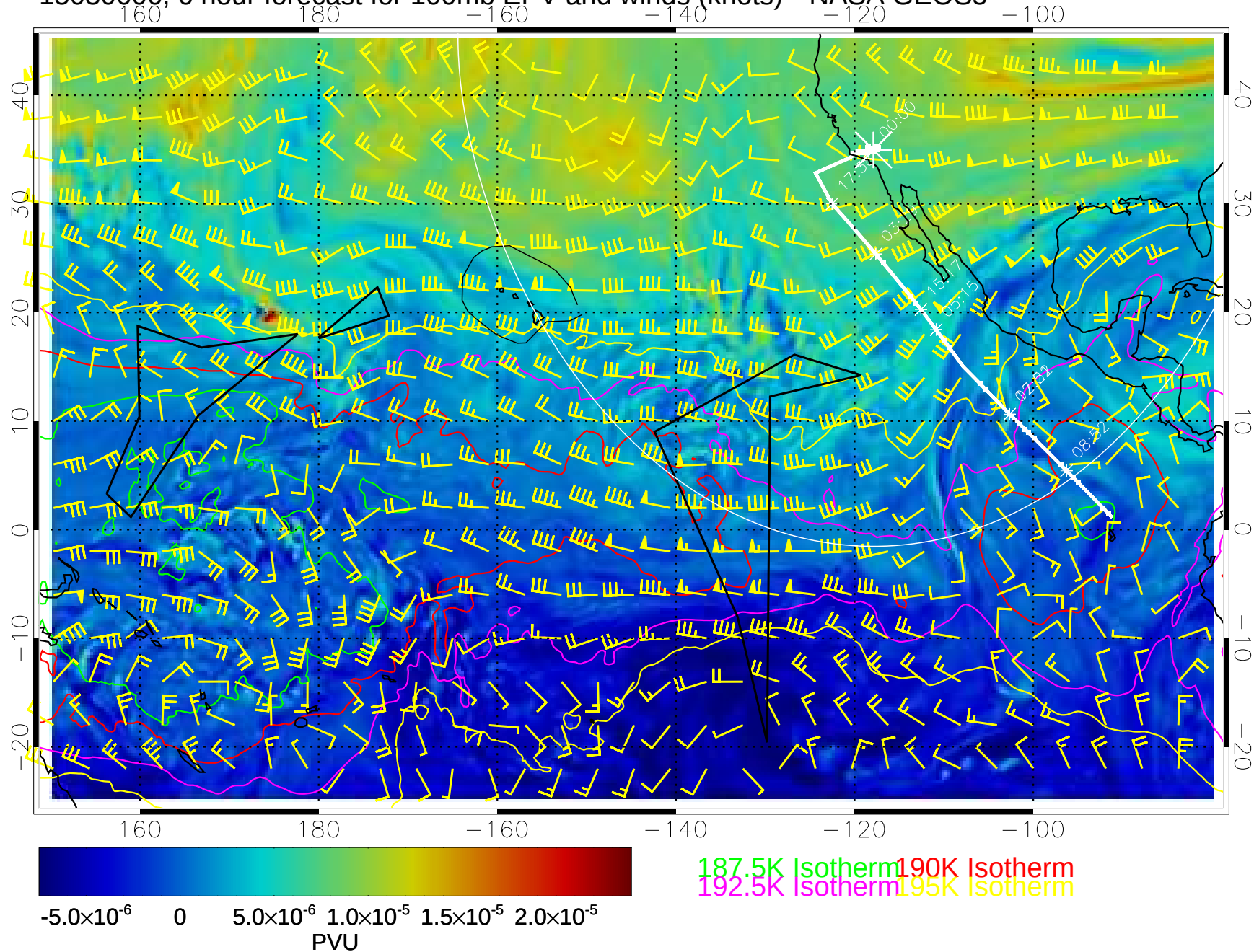
15030606, 6 hour forecast for 100mb EPV and winds (knots)-- NASA GEOS5
