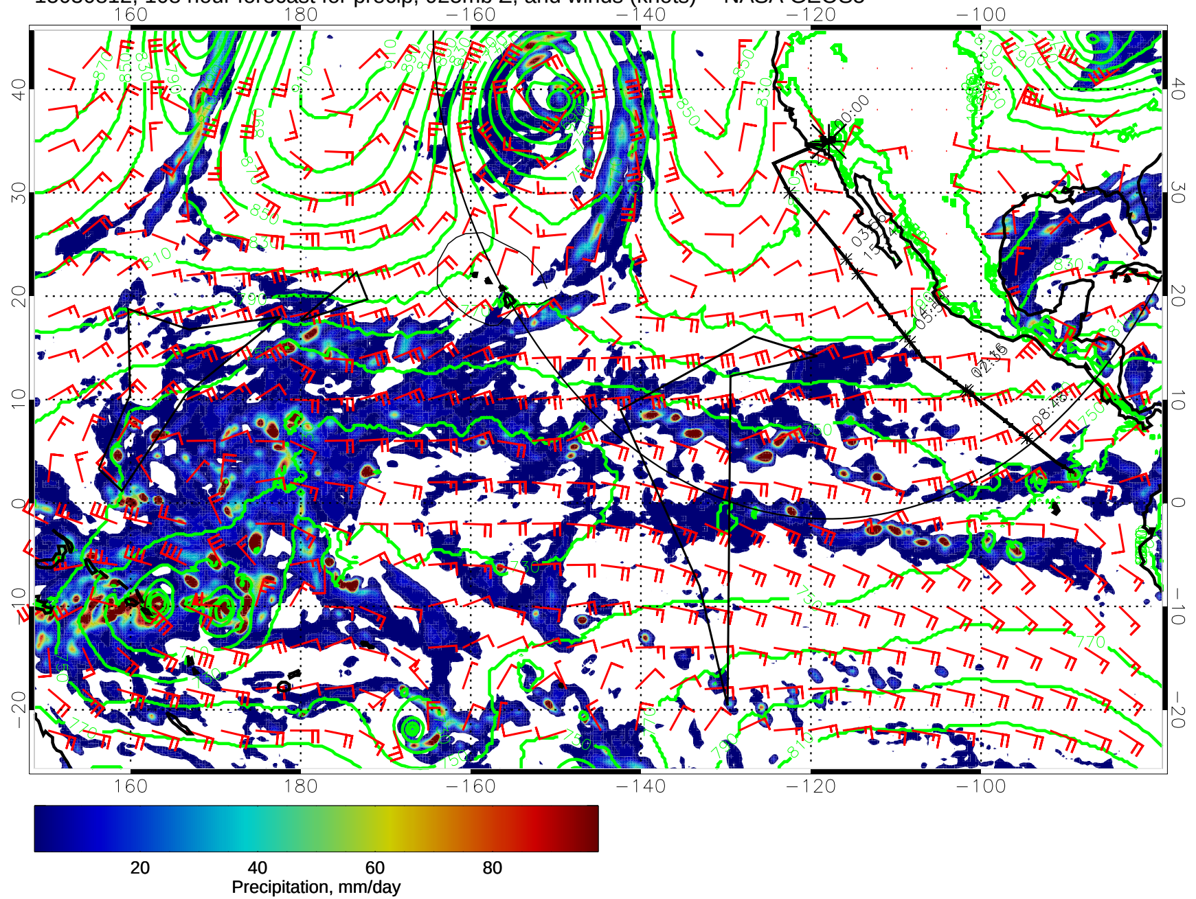
15030812, 108 hour forecast for precip, 925mb Z, and winds (knots) -- NASA GEOS5
