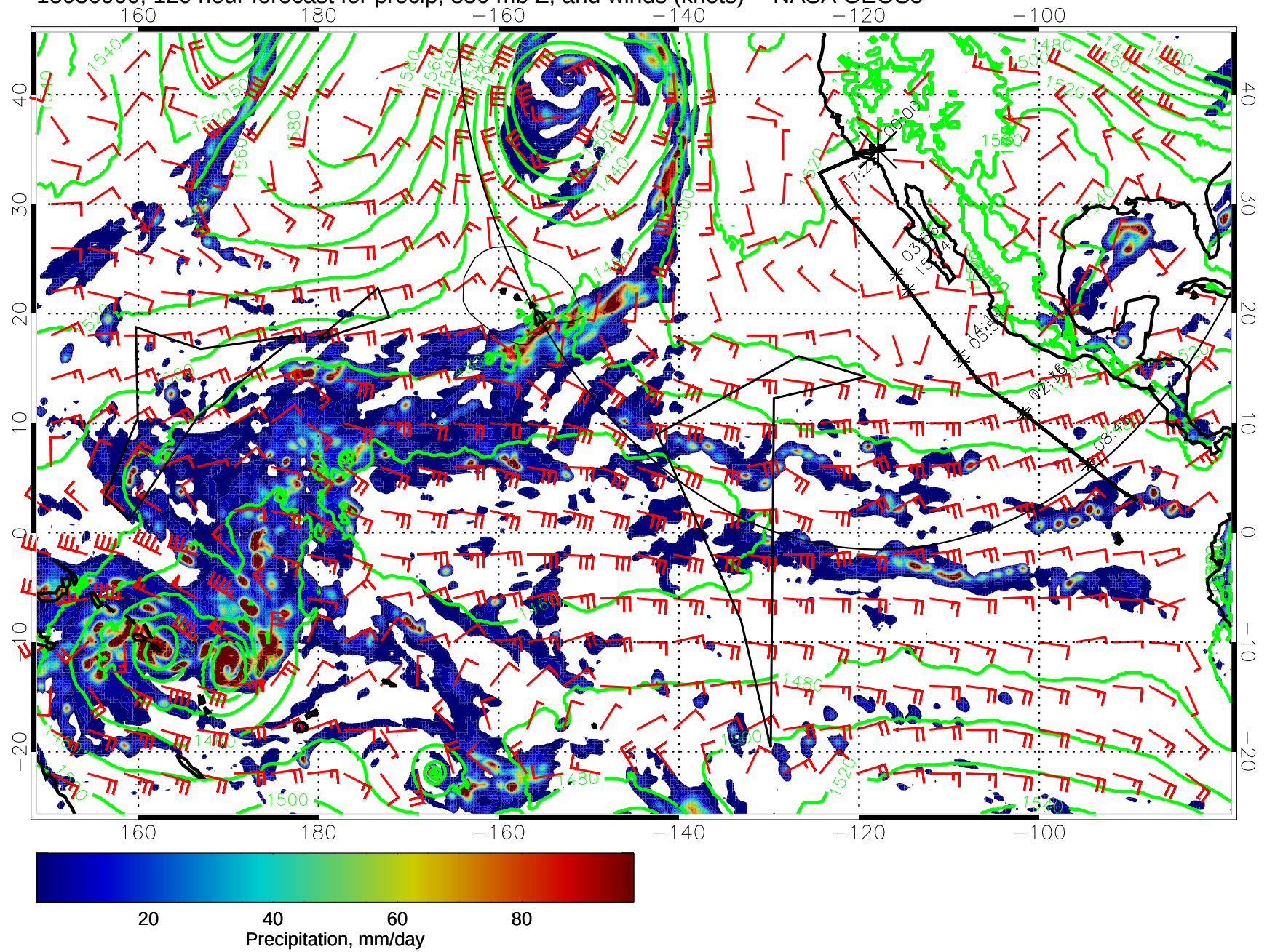
15030900, 120 hour forecast for precip, 850 mb Z, and winds (knots) -- NASA GEOS5
