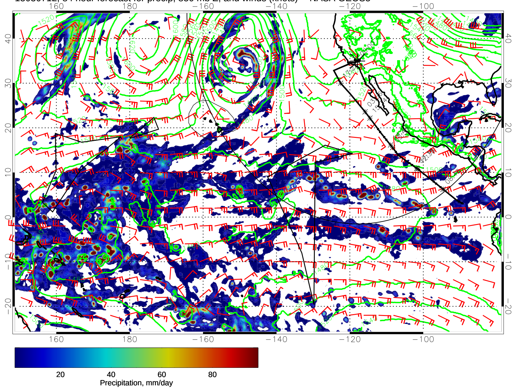
15030712, 84 hour forecast for precip, 850 mb Z, and winds (knots) -- NASA GEOS5
