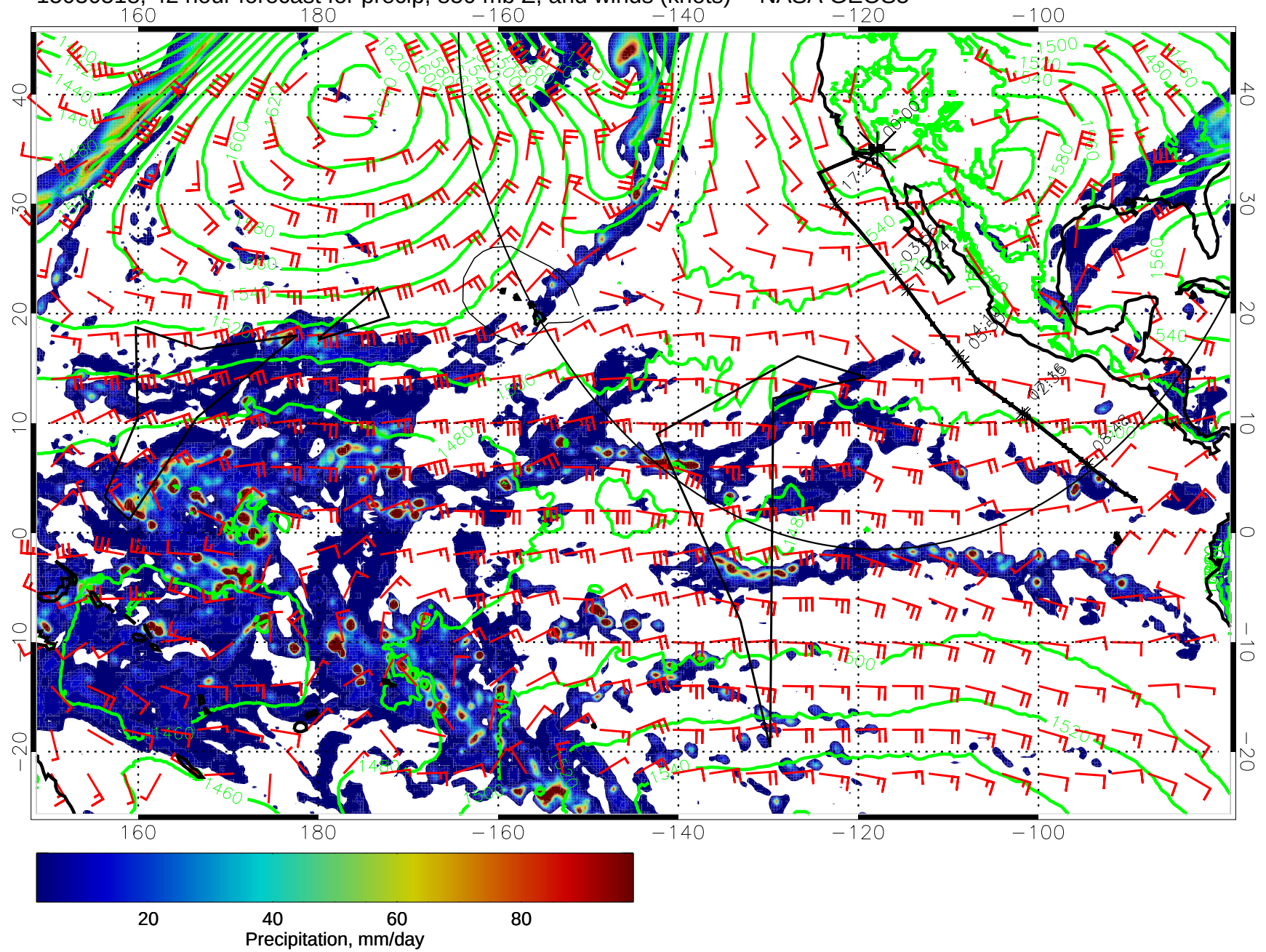
15030518, 42 hour forecast for precip, 850 mb Z, and winds (knots) -- NASA GEOS5
