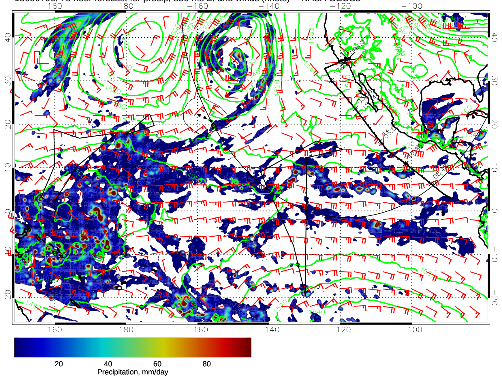
15030706, 78 hour forecast for precip, 850 mb Z, and winds (knots) -- NASA GEOS5
