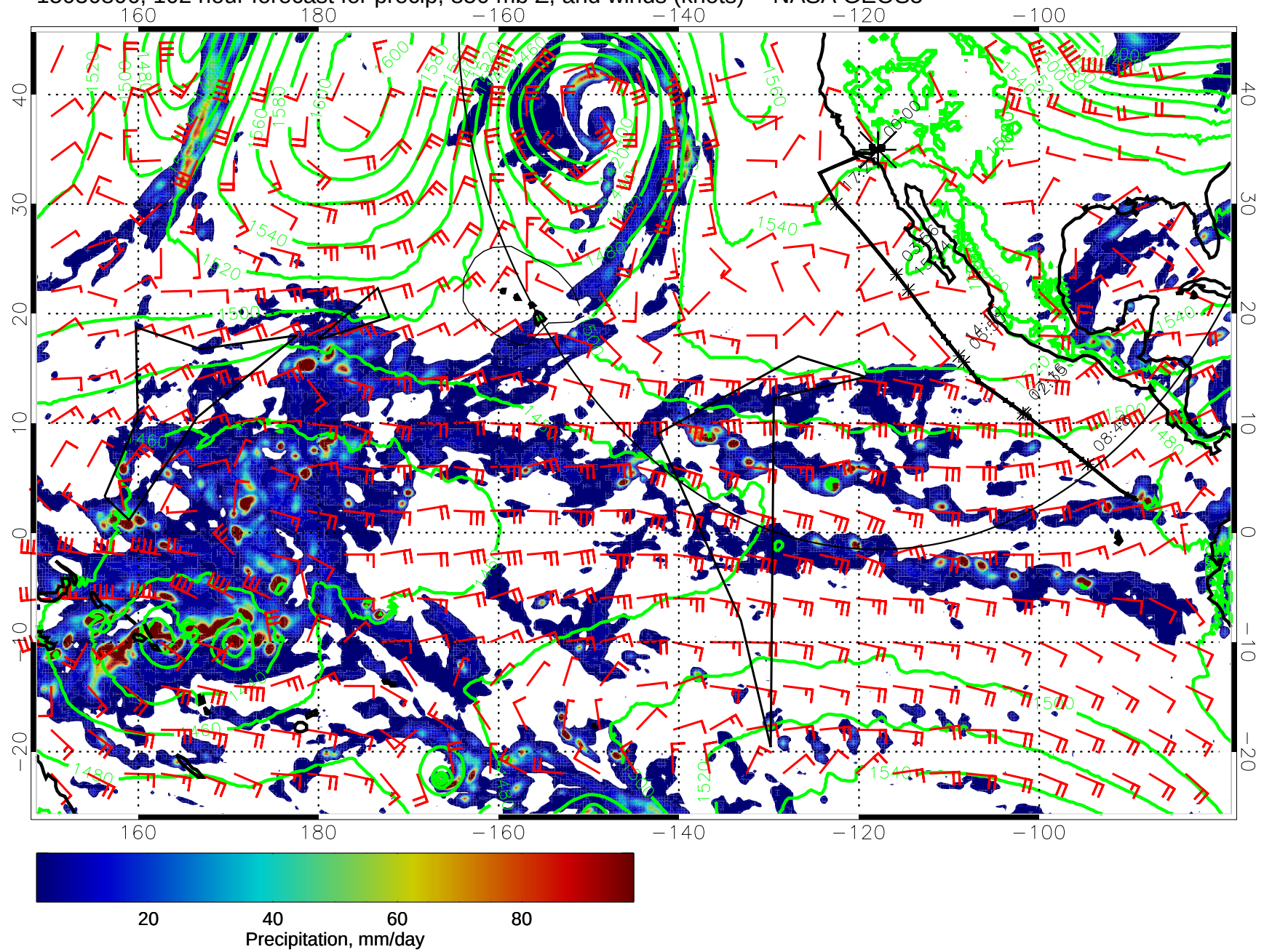
15030806, 102 hour forecast for precip, 850 mb Z, and winds (knots) -- NASA GEOS5
