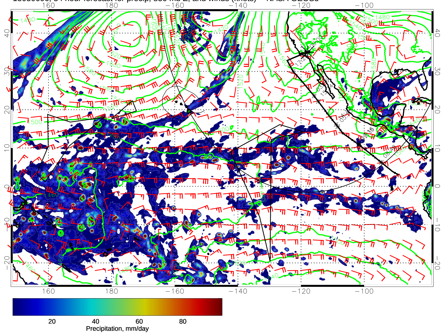
15030606, 54 hour forecast for precip, 850 mb Z, and winds (knots) -- NASA GEOS5
