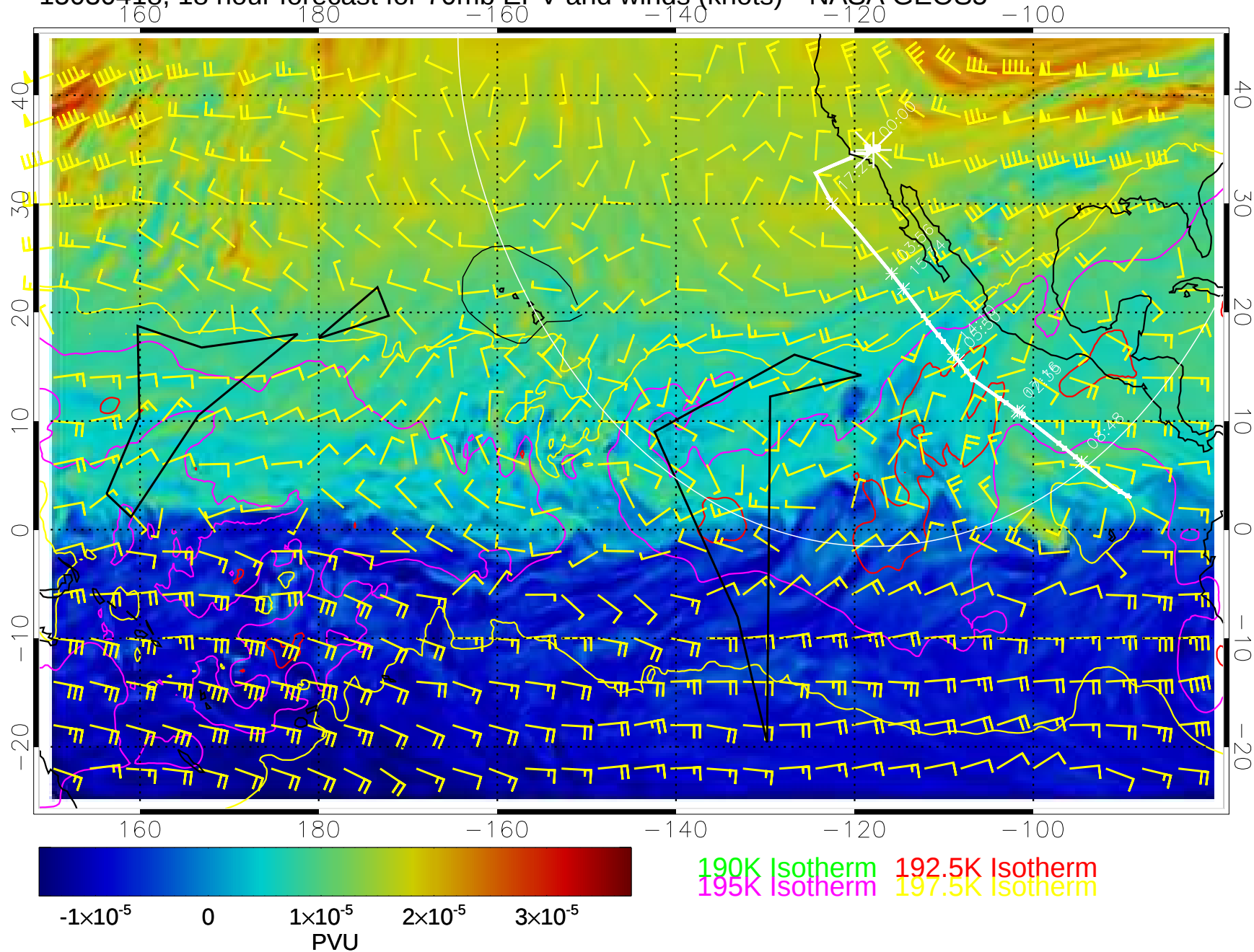
15030418, 18 hour forecast for 70mb EPV and winds (knots)-- NASA GEOS5
