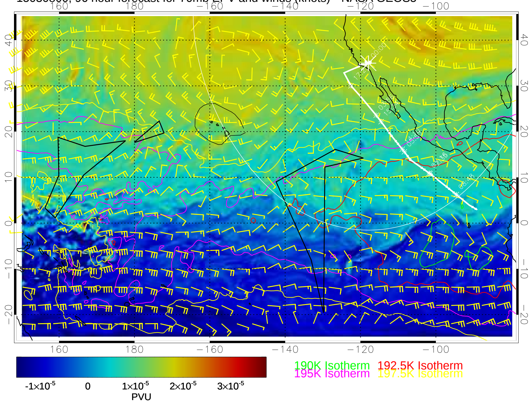
15030800, 96 hour forecast for 70mb EPV and winds (knots)-- NASA GEOS5
