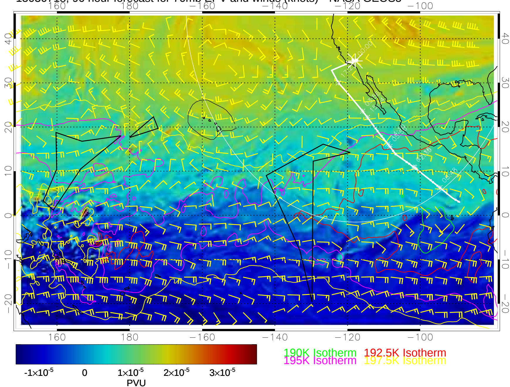
15030718, 90 hour forecast for 70mb EPV and winds (knots)-- NASA GEOS5
