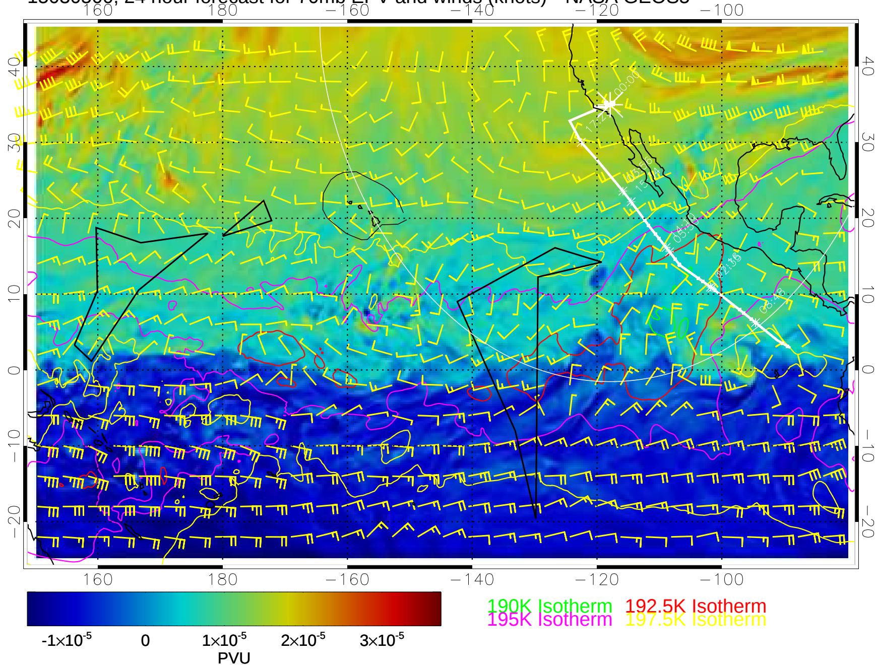
15030500, 24 hour forecast for 70mb EPV and winds (knots)-- NASA GEOS5
