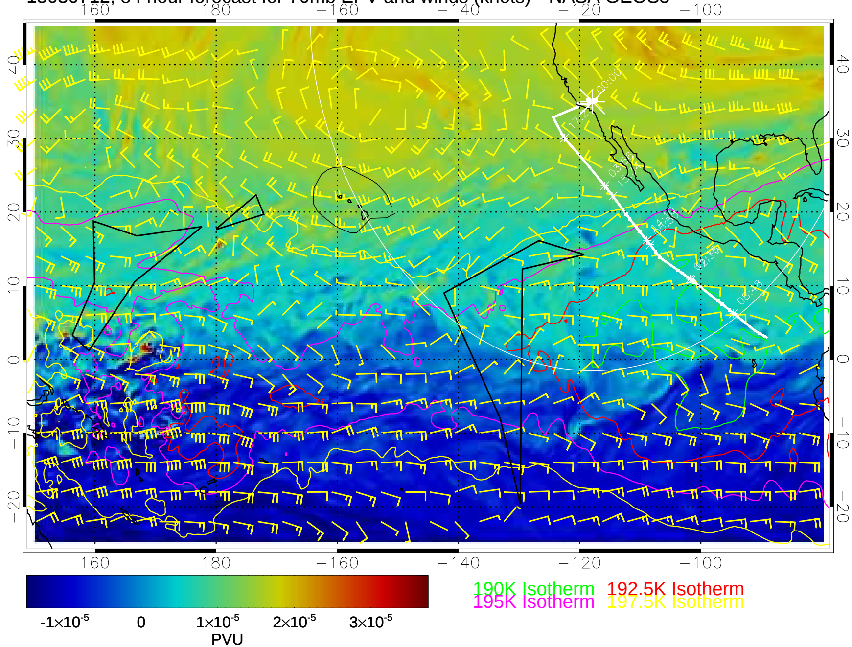
15030712, 84 hour forecast for 70mb EPV and winds (knots)-- NASA GEOS5
