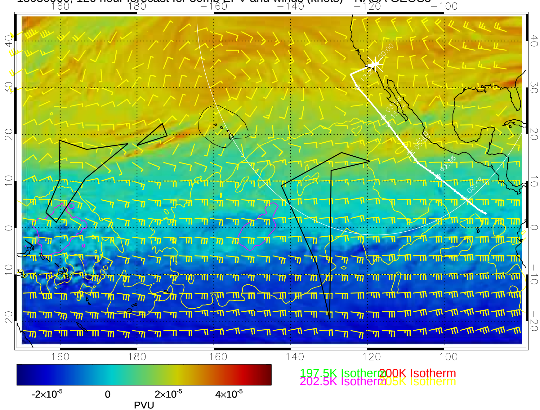
15030900, 120 hour forecast for 50mb EPV and winds (knots)-- NASA GEOS5
