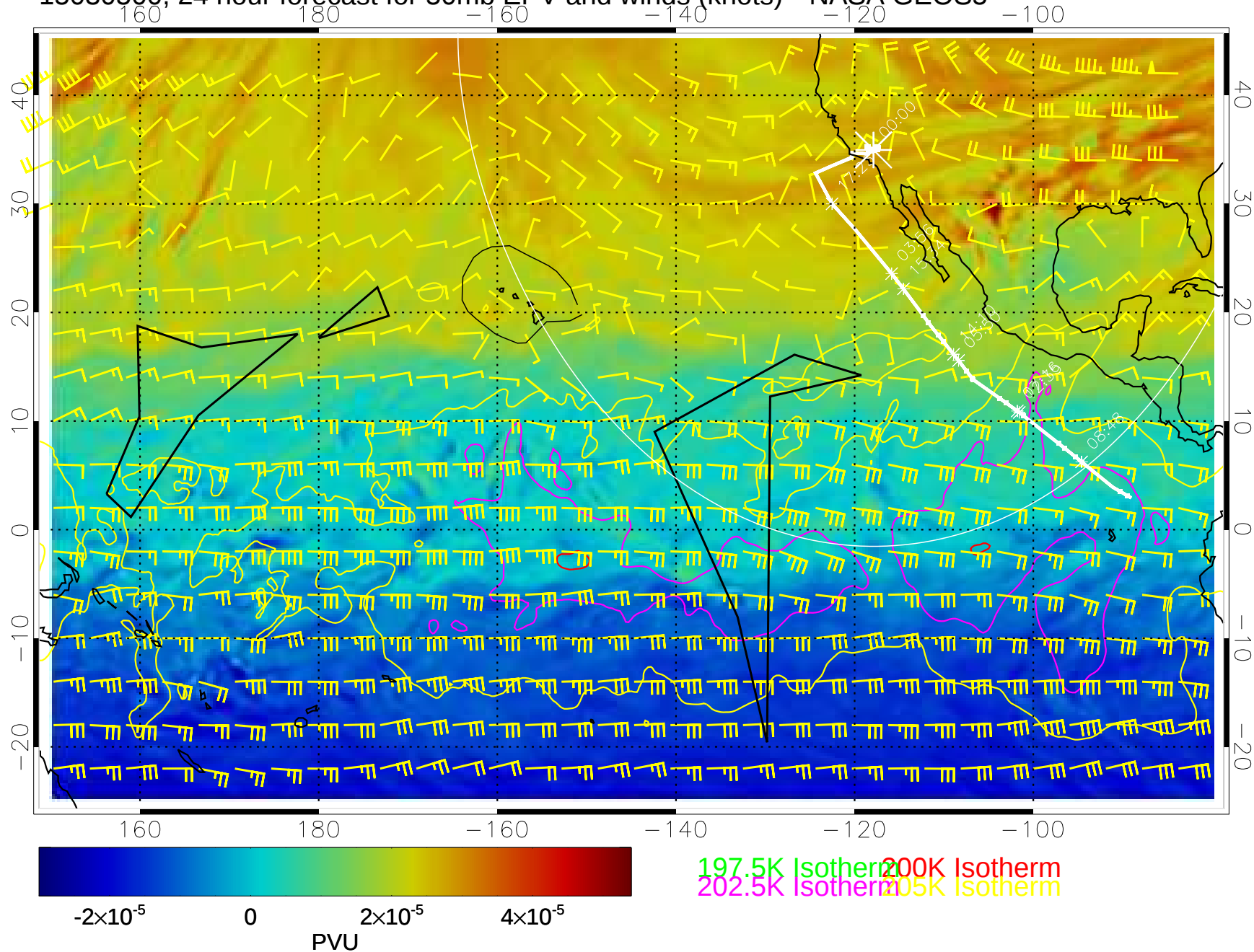
15030500, 24 hour forecast for 50mb EPV and winds (knots)-- NASA GEOS5
