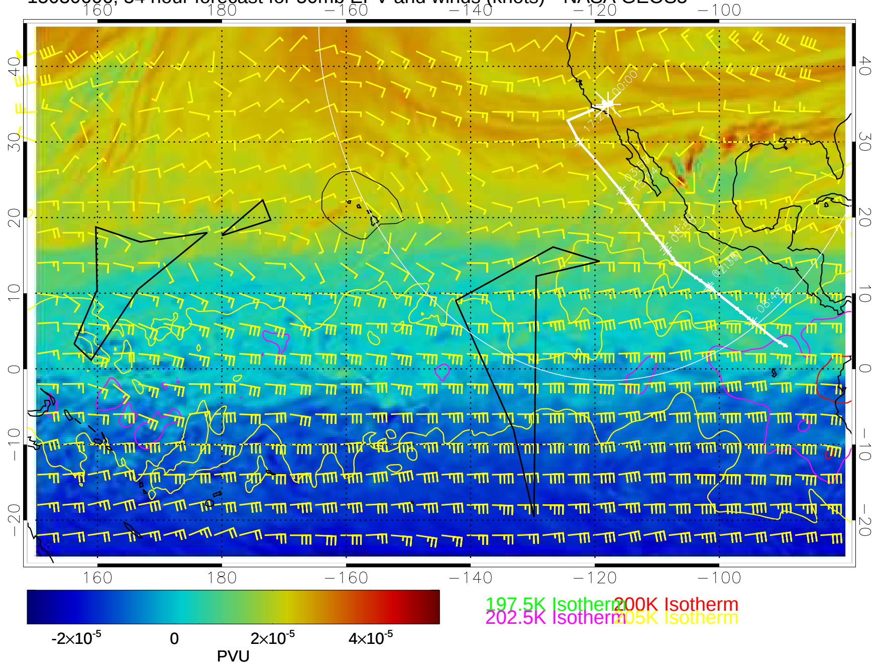
15030606, 54 hour forecast for 50mb EPV and winds (knots)-- NASA GEOS5
