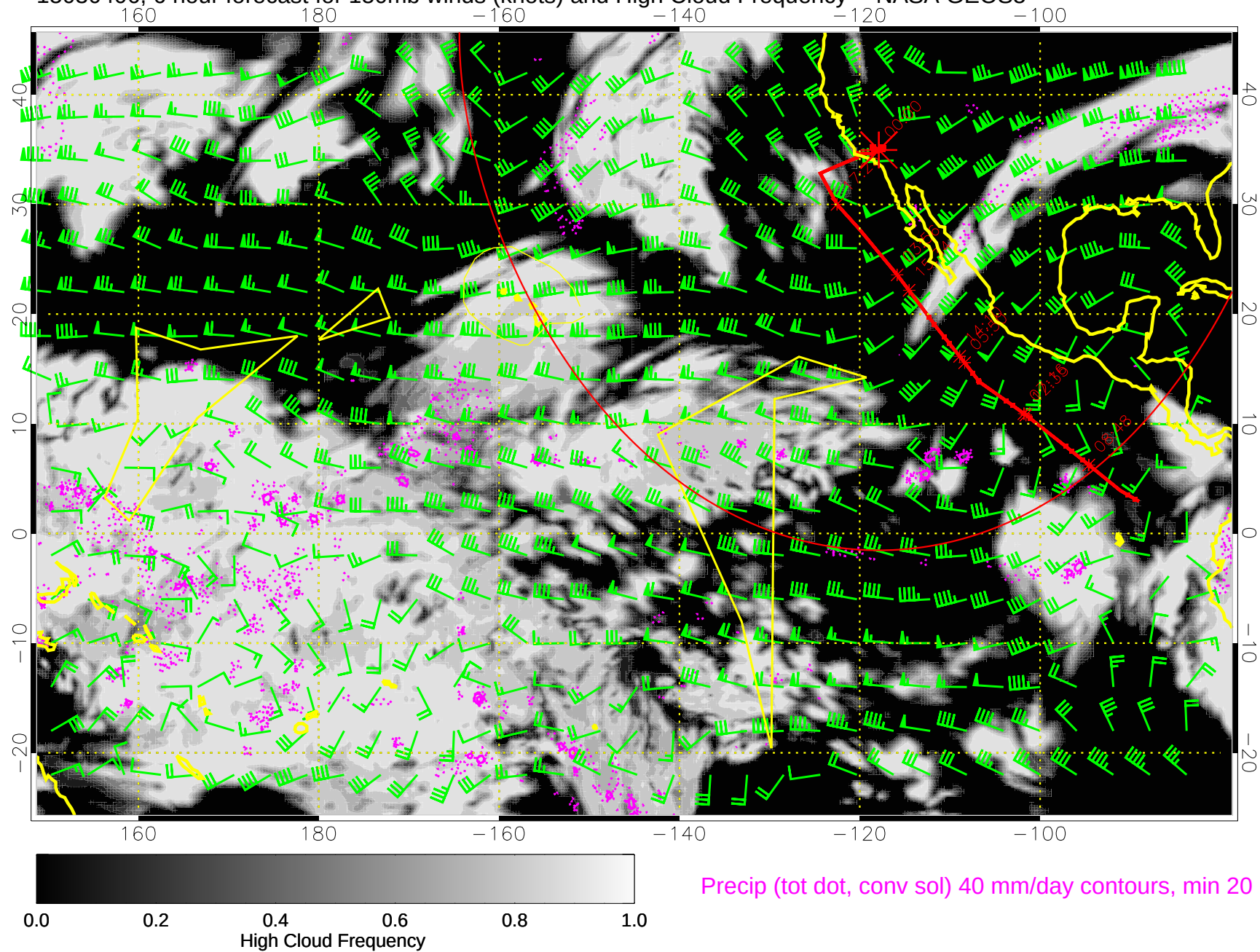
15030406, 6 hour forecast for 150mb winds (knots) and High Cloud Frequency -- NASA GEOS5
