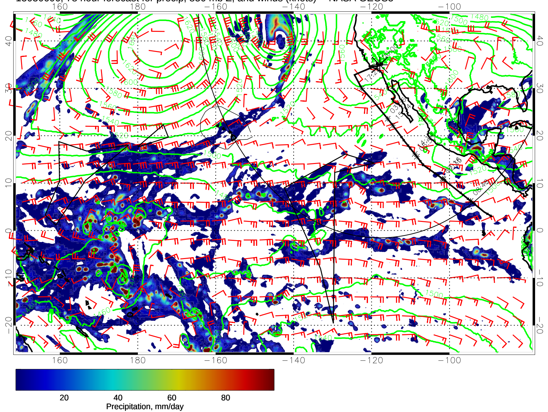
15030606, 78 hour forecast for precip, 850 mb Z, and winds (knots) -- NASA GEOS5
