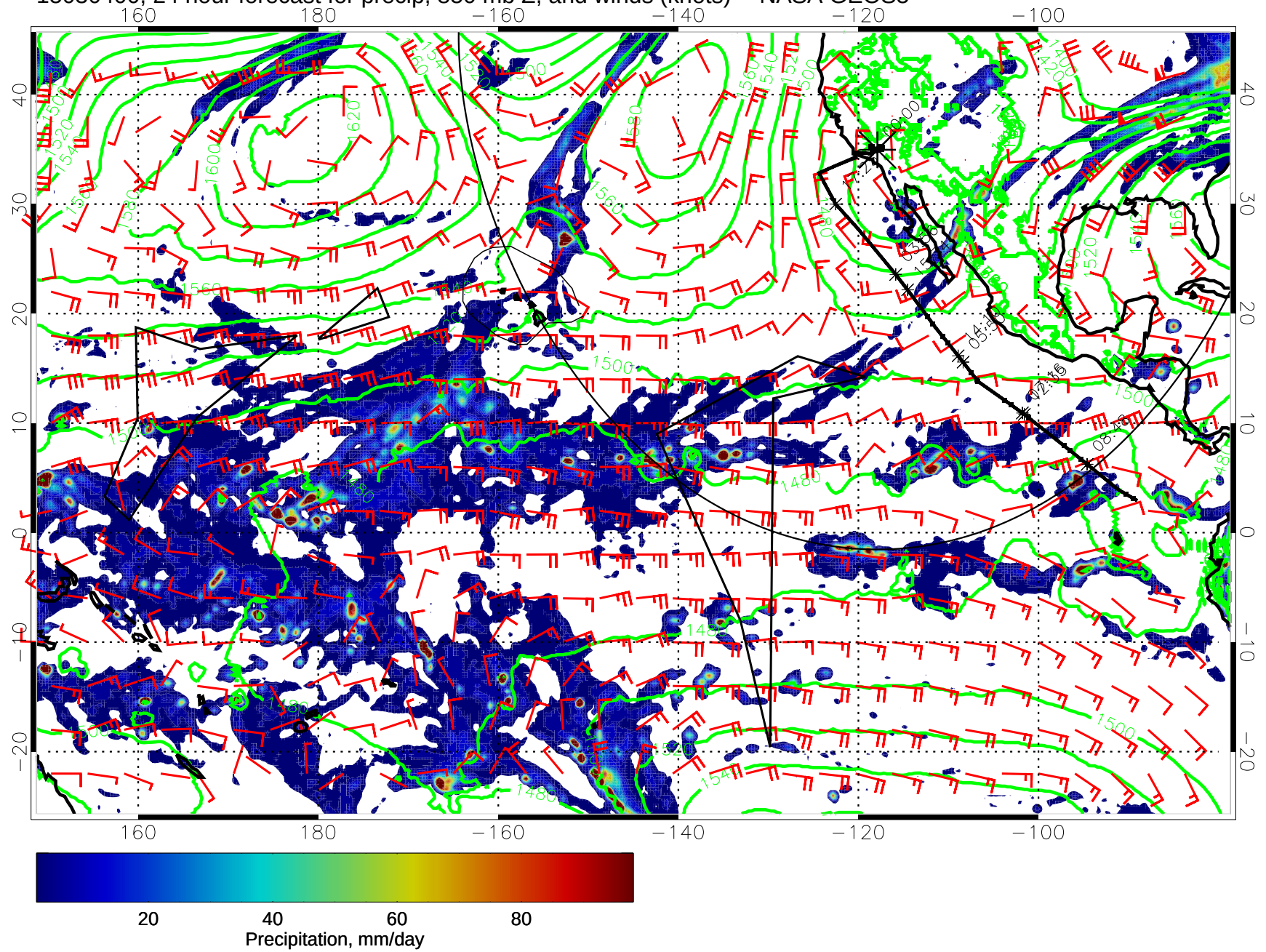
15030400, 24 hour forecast for precip, 850 mb Z, and winds (knots) -- NASA GEOS5
