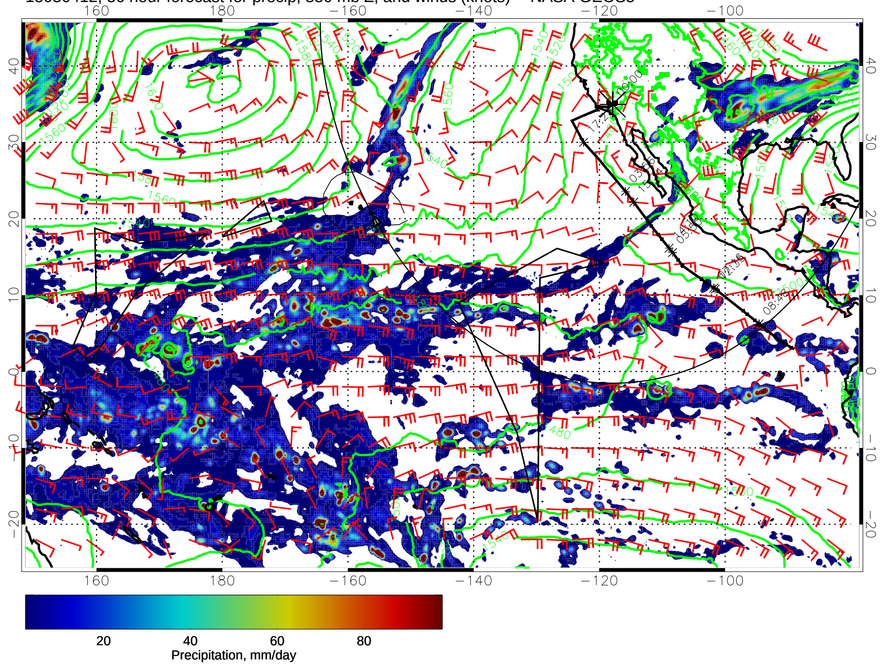
15030412, 36 hour forecast for precip, 850 mb Z, and winds (knots) -- NASA GEOS5
