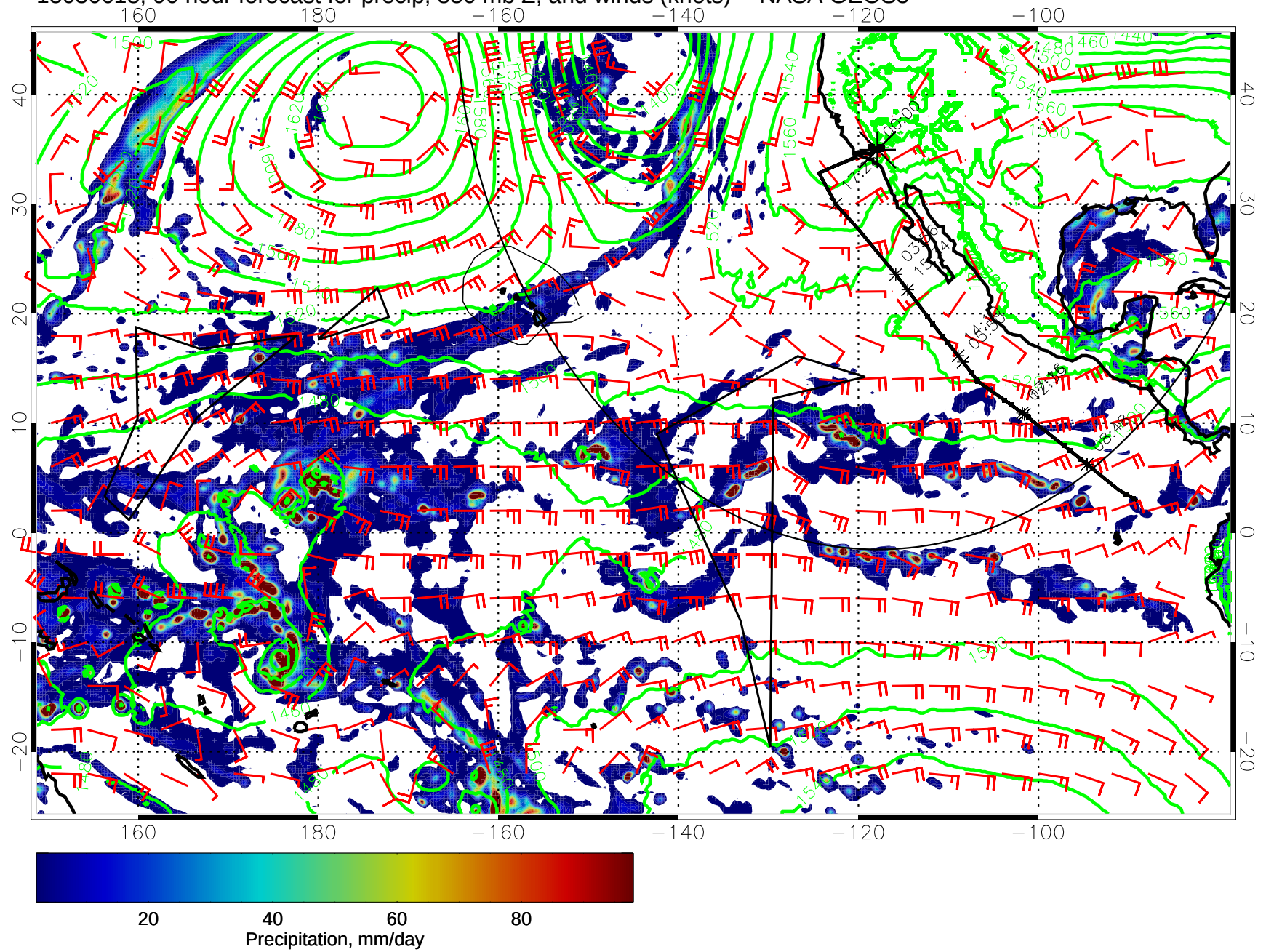
15030618, 90 hour forecast for precip, 850 mb Z, and winds (knots) -- NASA GEOS5
