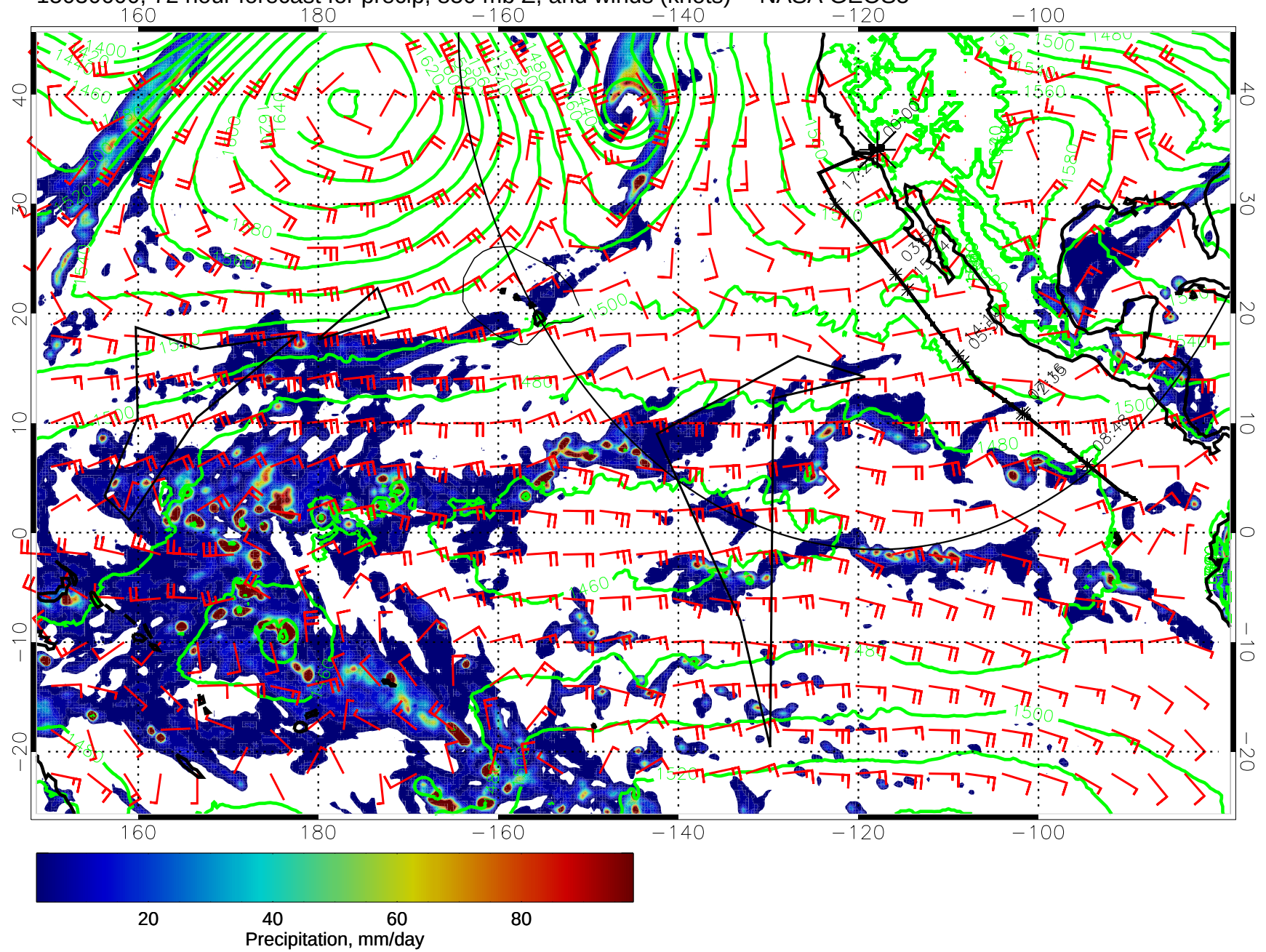
15030600, 72 hour forecast for precip, 850 mb Z, and winds (knots) -- NASA GEOS5
