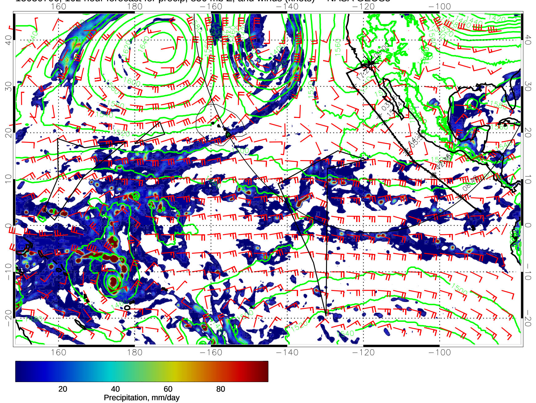
15030706, 102 hour forecast for precip, 850 mb Z, and winds (knots) -- NASA GEOS5
