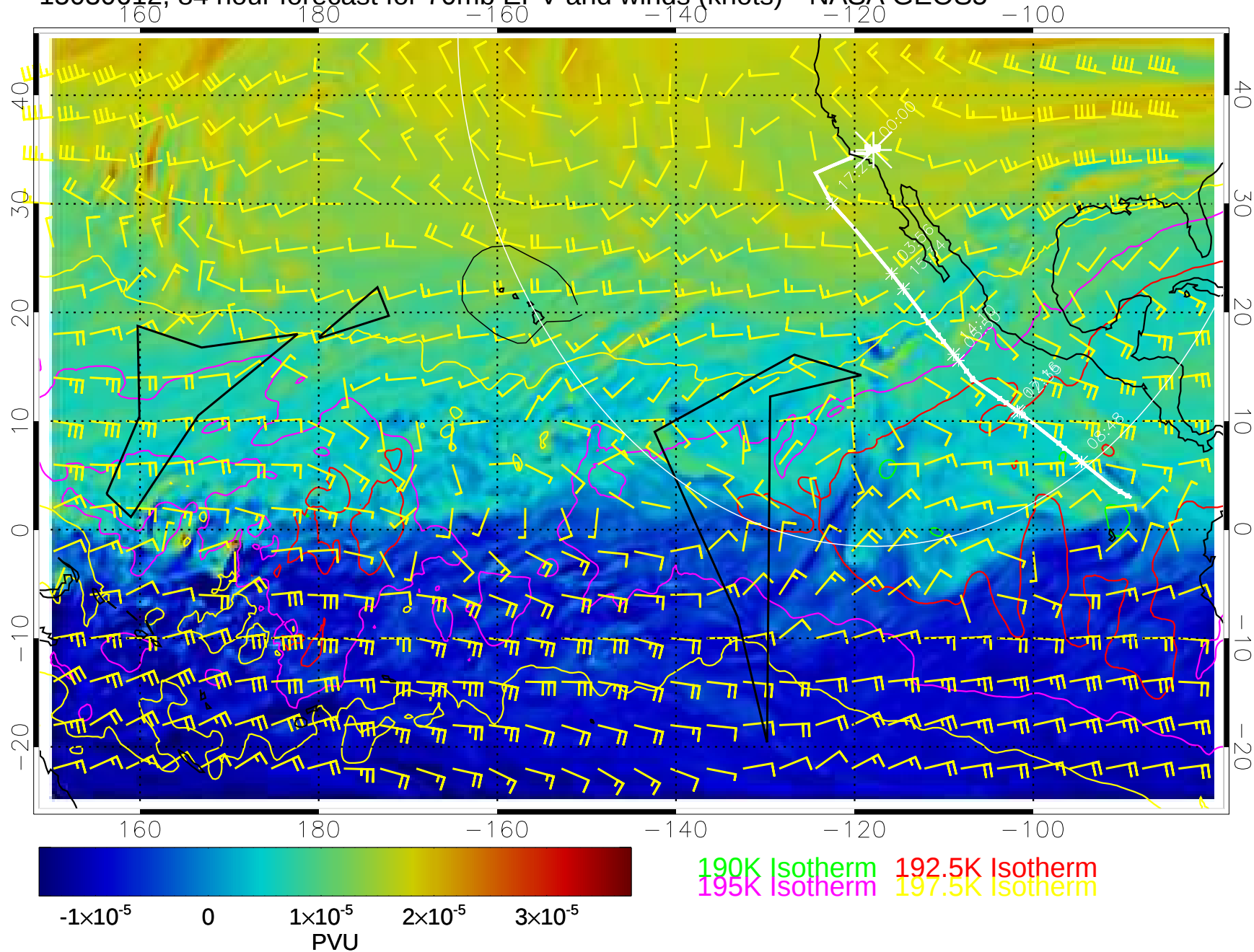
15030612, 84 hour forecast for 70mb EPV and winds (knots)-- NASA GEOS5
