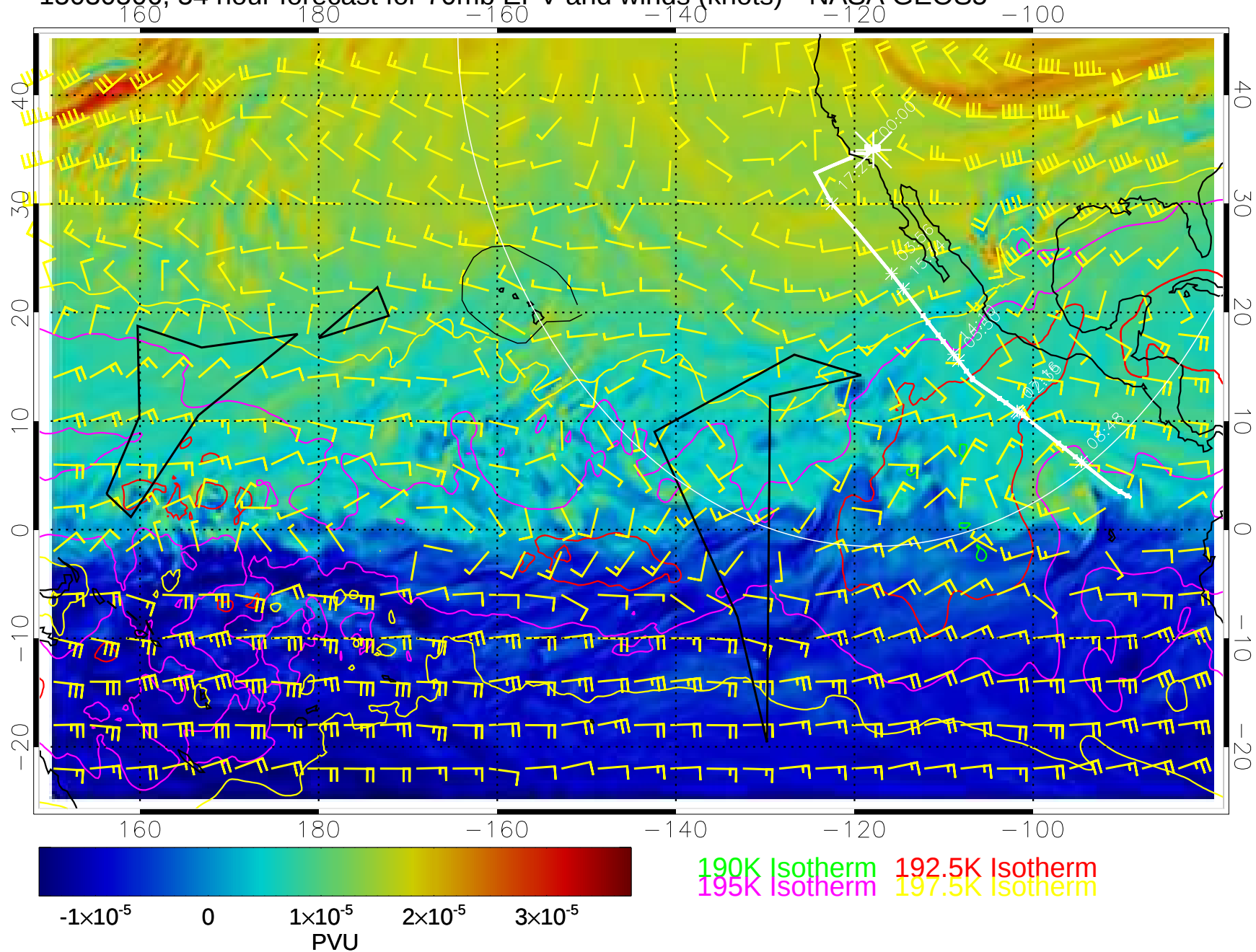
15030506, 54 hour forecast for 70mb EPV and winds (knots)-- NASA GEOS5
