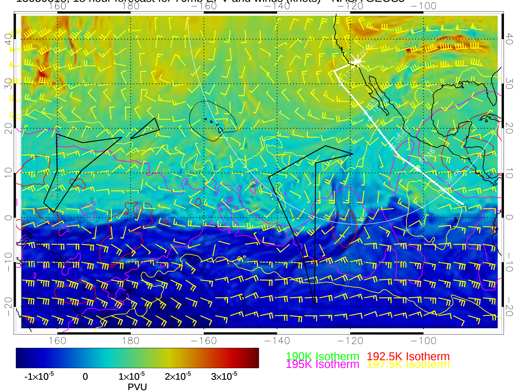
15030318, 18 hour forecast for 70mb EPV and winds (knots)-- NASA GEOS5
