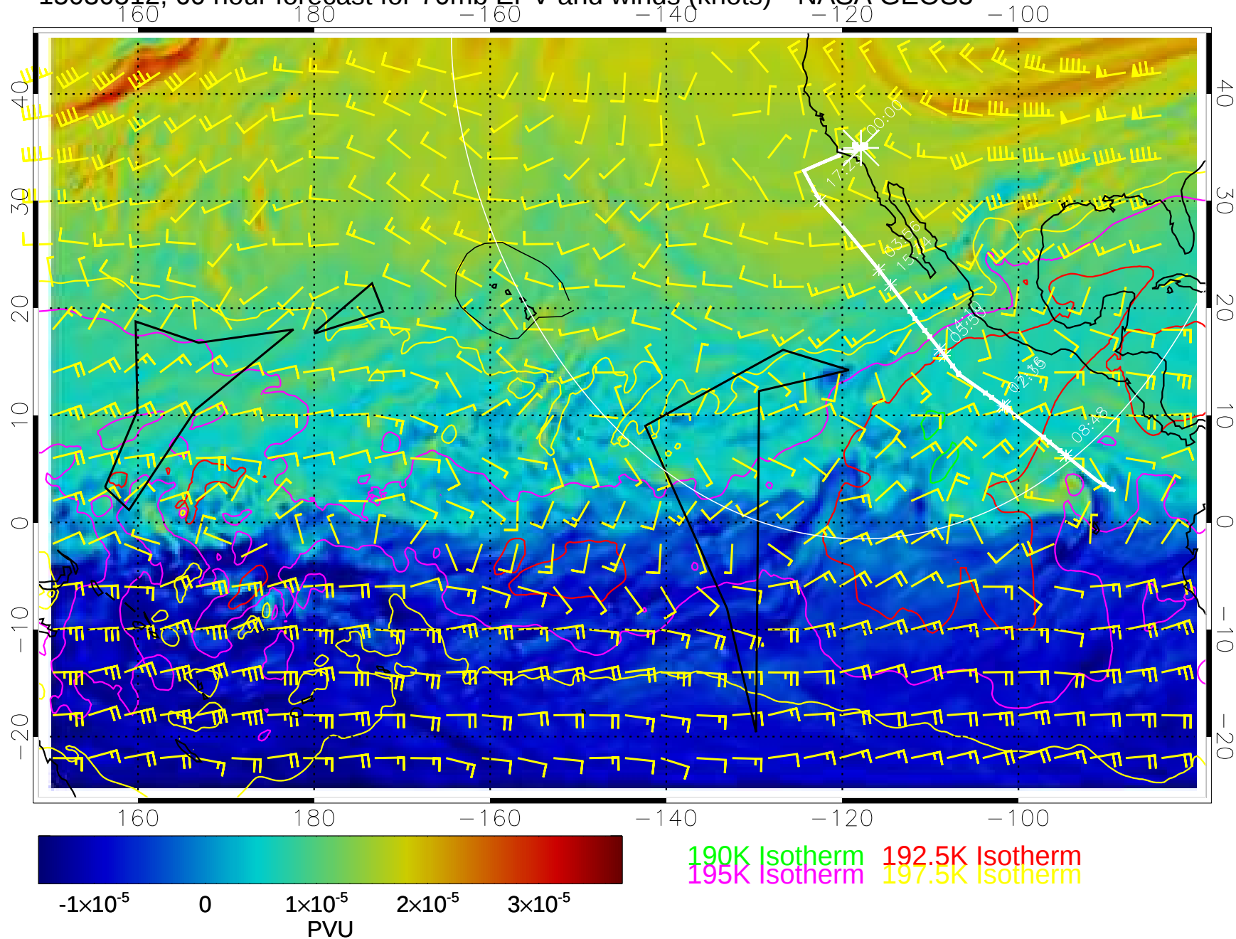
15030512, 60 hour forecast for 70mb EPV and winds (knots)-- NASA GEOS5
