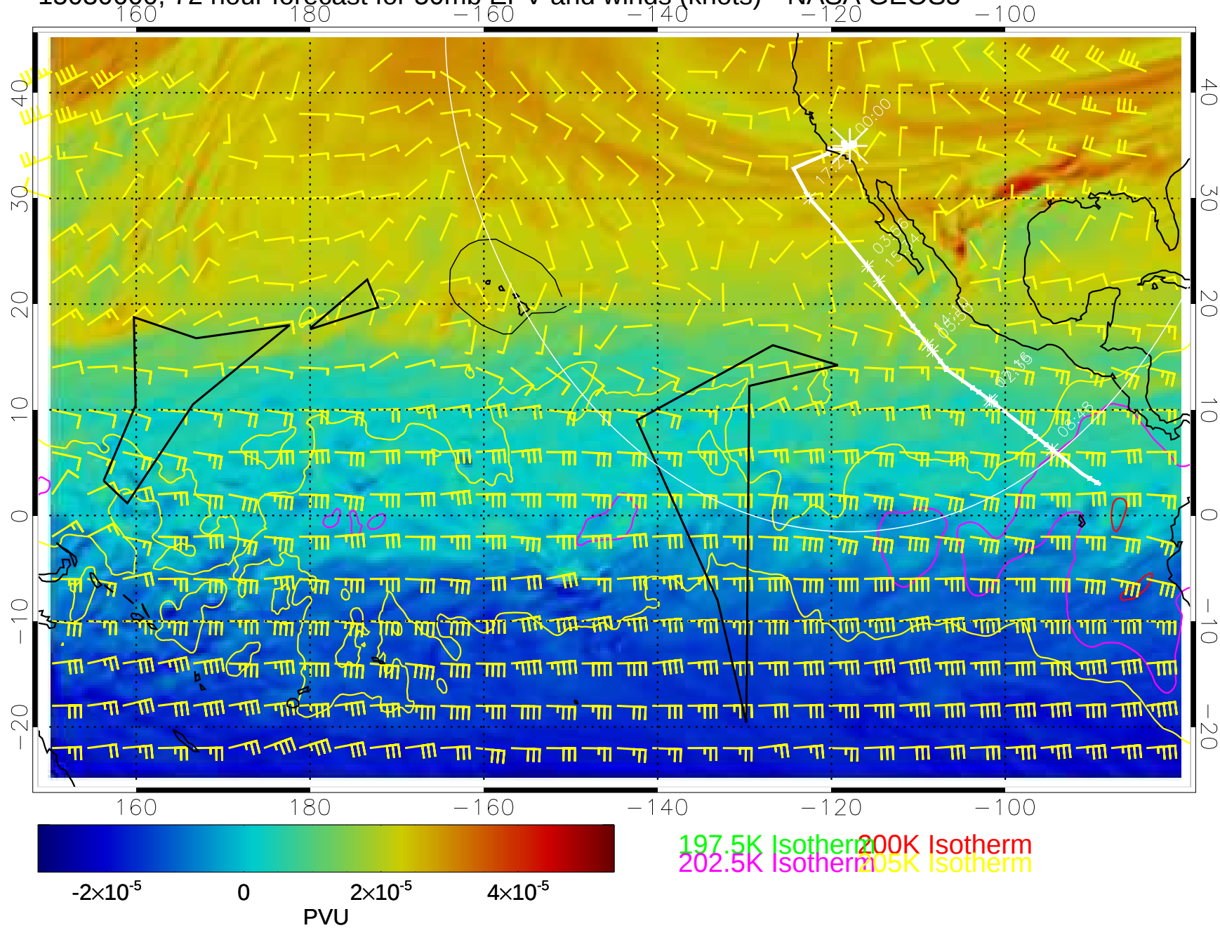
15030600, 72 hour forecast for 50mb EPV and winds (knots)-- NASA GEOS5
