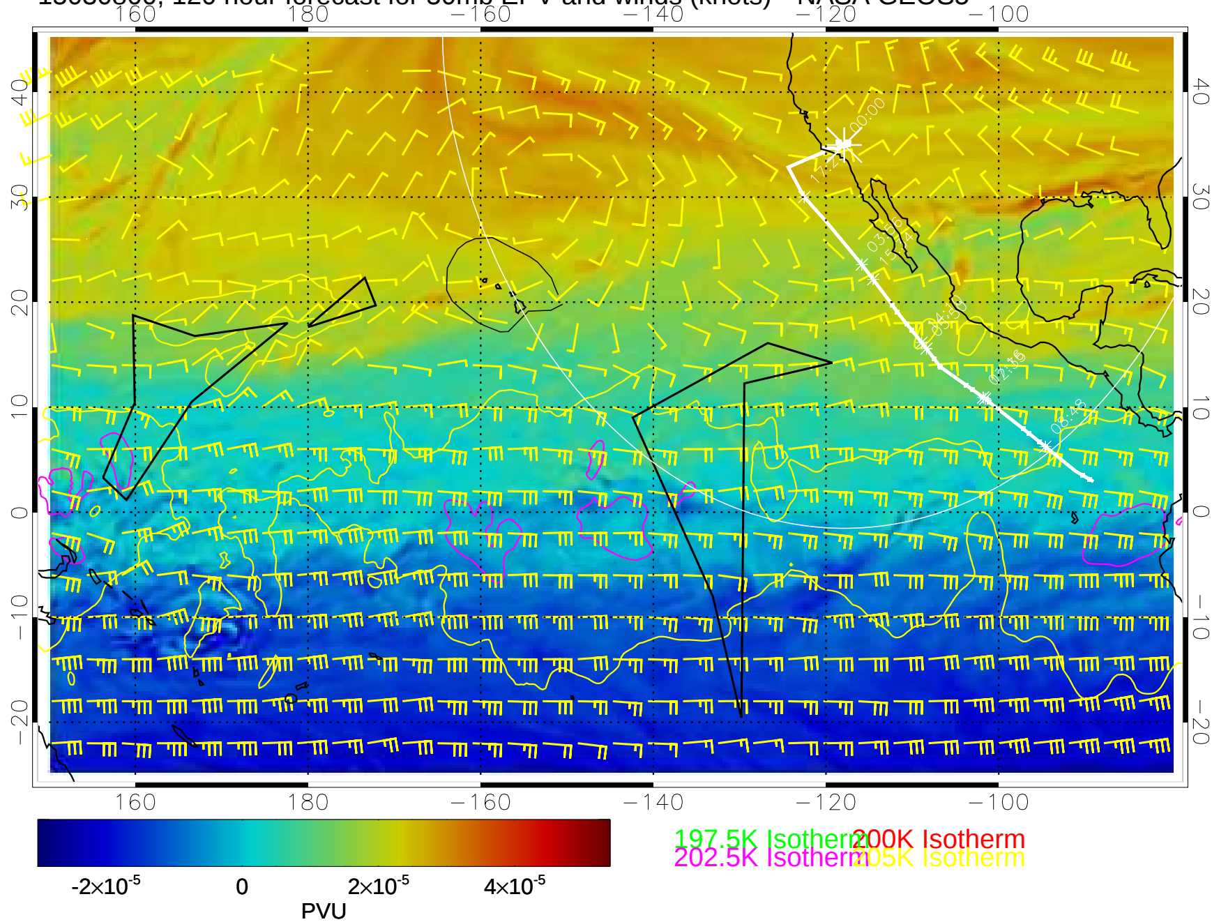
15030800, 120 hour forecast for 50mb EPV and winds (knots)-- NASA GEOS5
