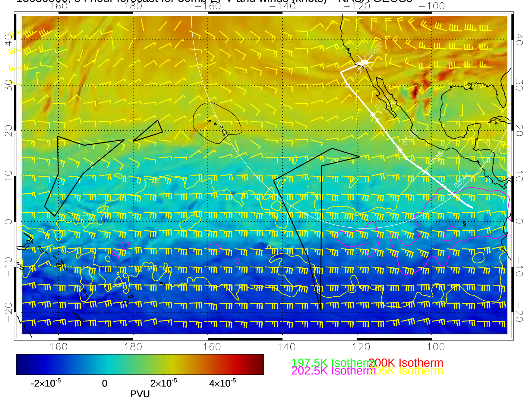
15030506, 54 hour forecast for 50mb EPV and winds (knots)-- NASA GEOS5
