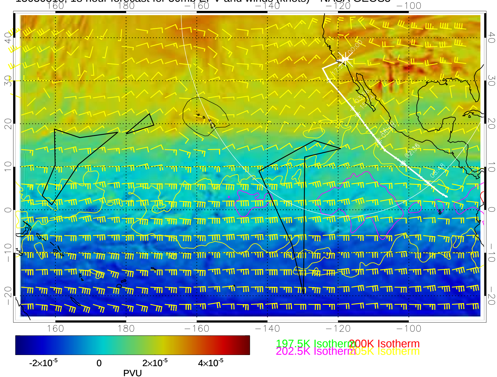
15030318, 18 hour forecast for 50mb EPV and winds (knots)-- NASA GEOS5
