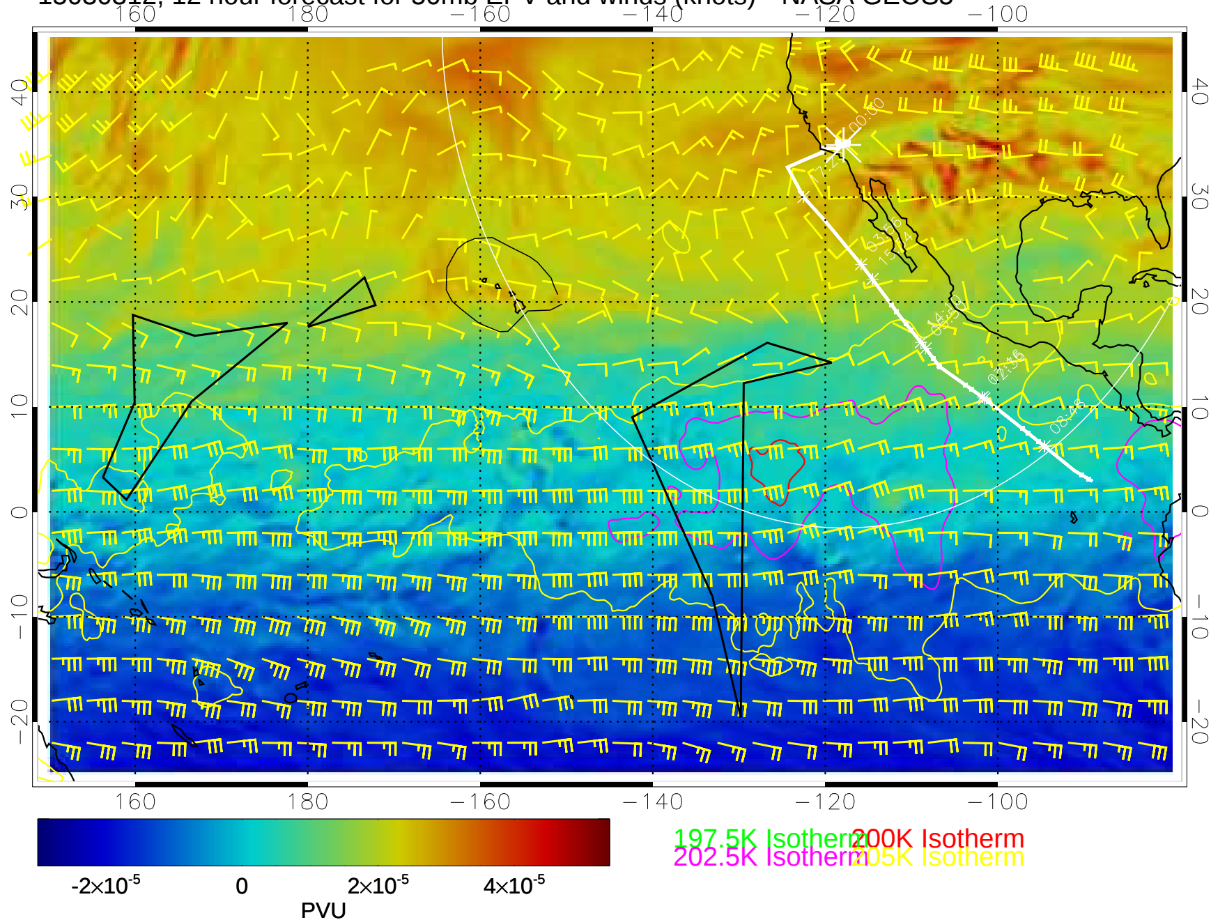
15030312, 12 hour forecast for 50mb EPV and winds (knots)-- NASA GEOS5
