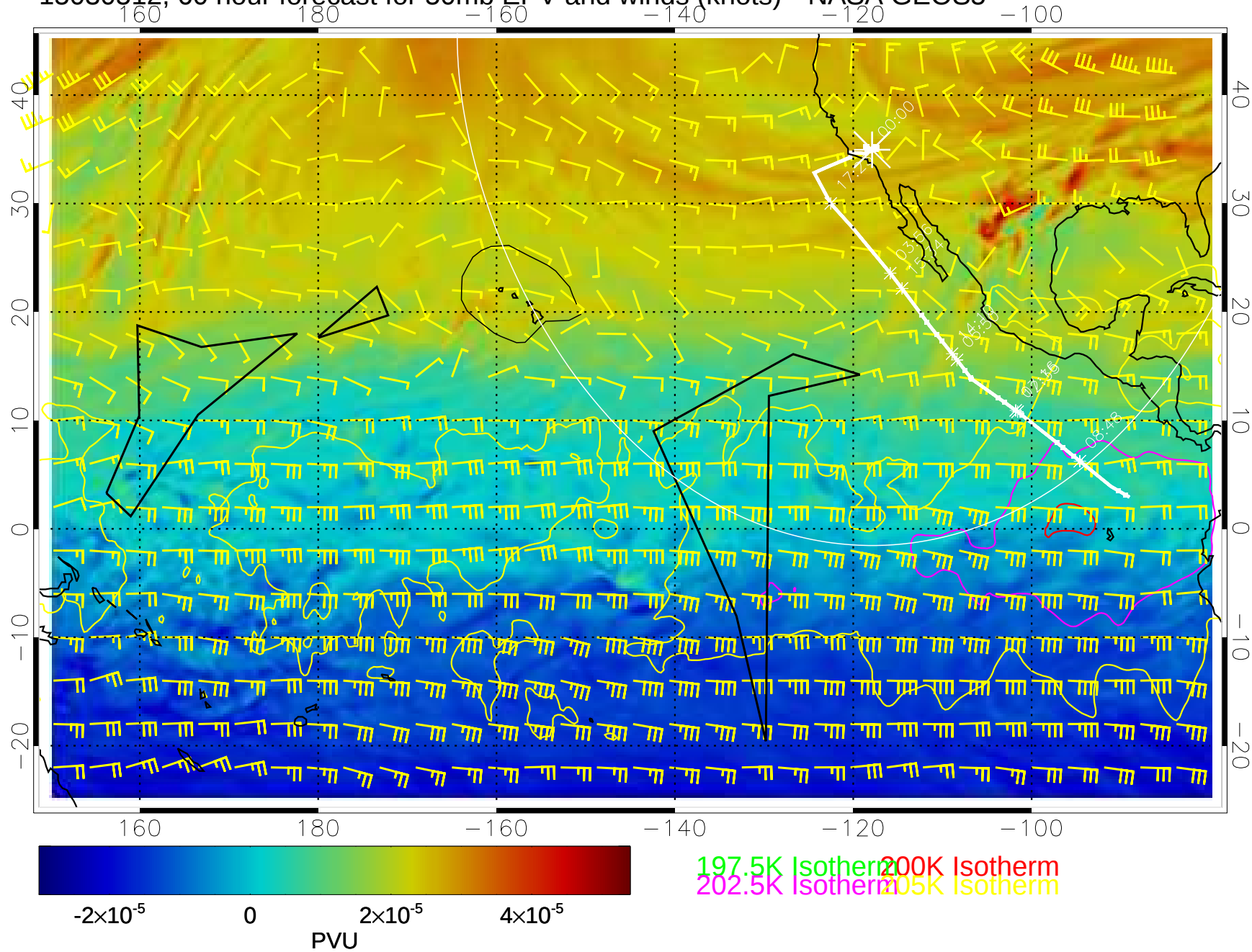
15030512, 60 hour forecast for 50mb EPV and winds (knots)-- NASA GEOS5
