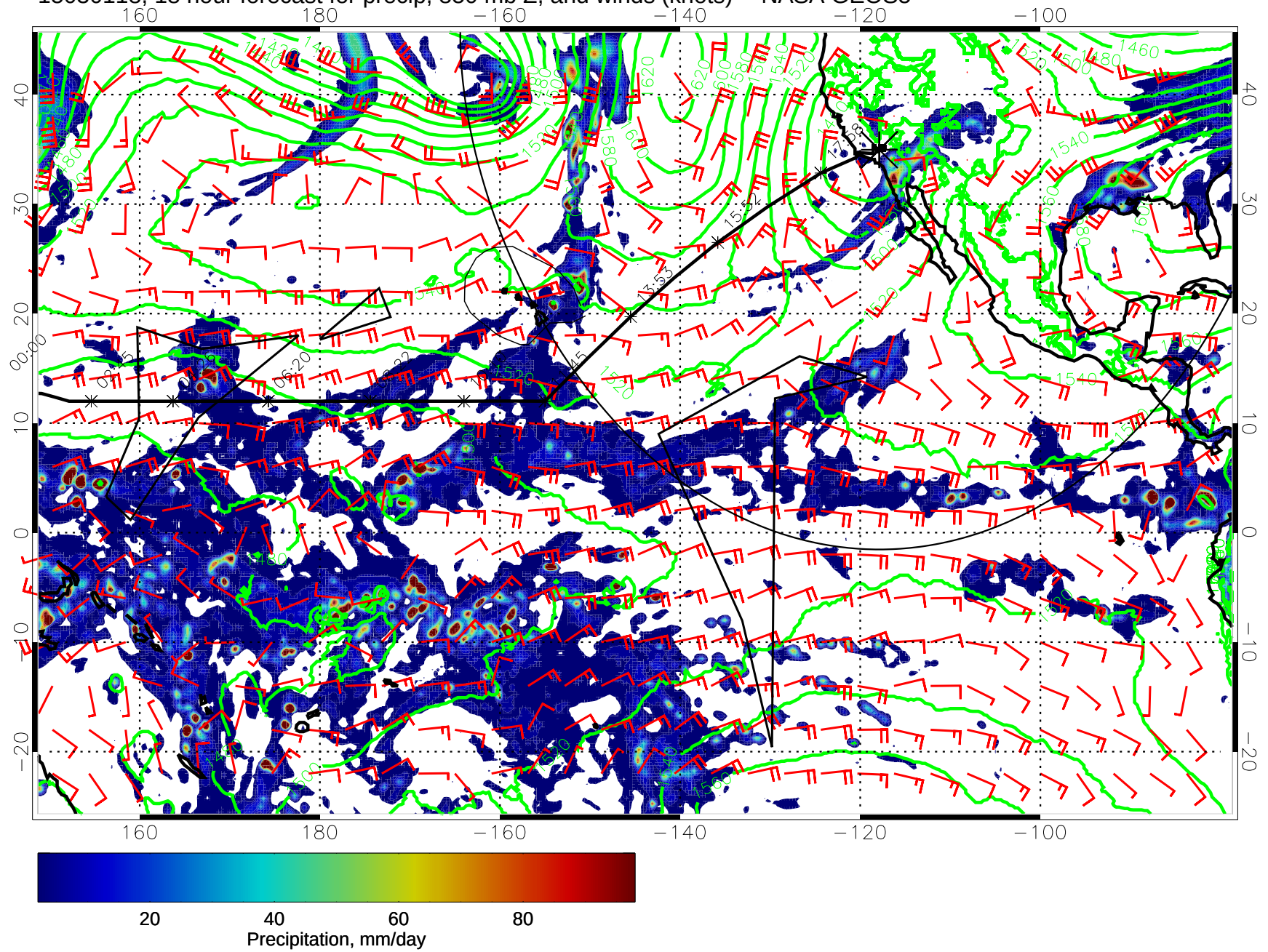
15030118, 18 hour forecast for precip, 850 mb Z, and winds (knots) -- NASA GEOS5
