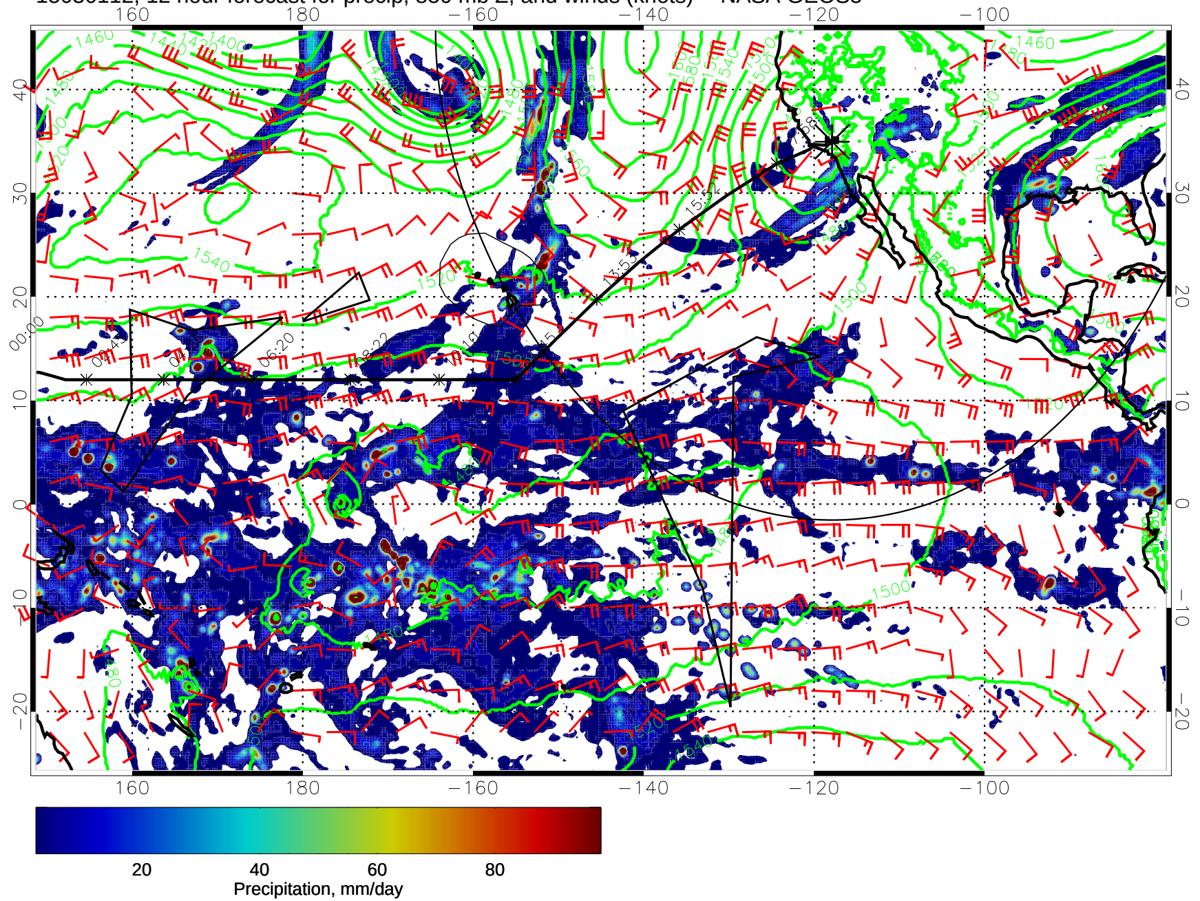
15030112, 12 hour forecast for precip, 850 mb Z, and winds (knots) -- NASA GEOS5
