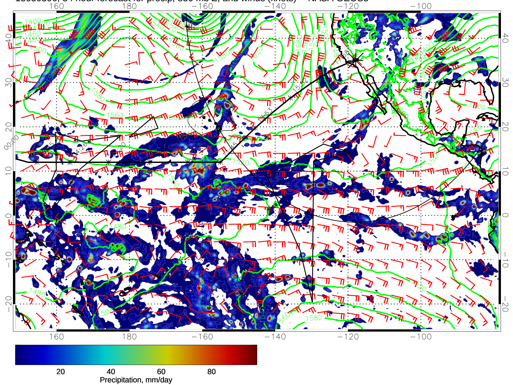
15030306, 54 hour forecast for precip, 850 mb Z, and winds (knots) -- NASA GEOS5
