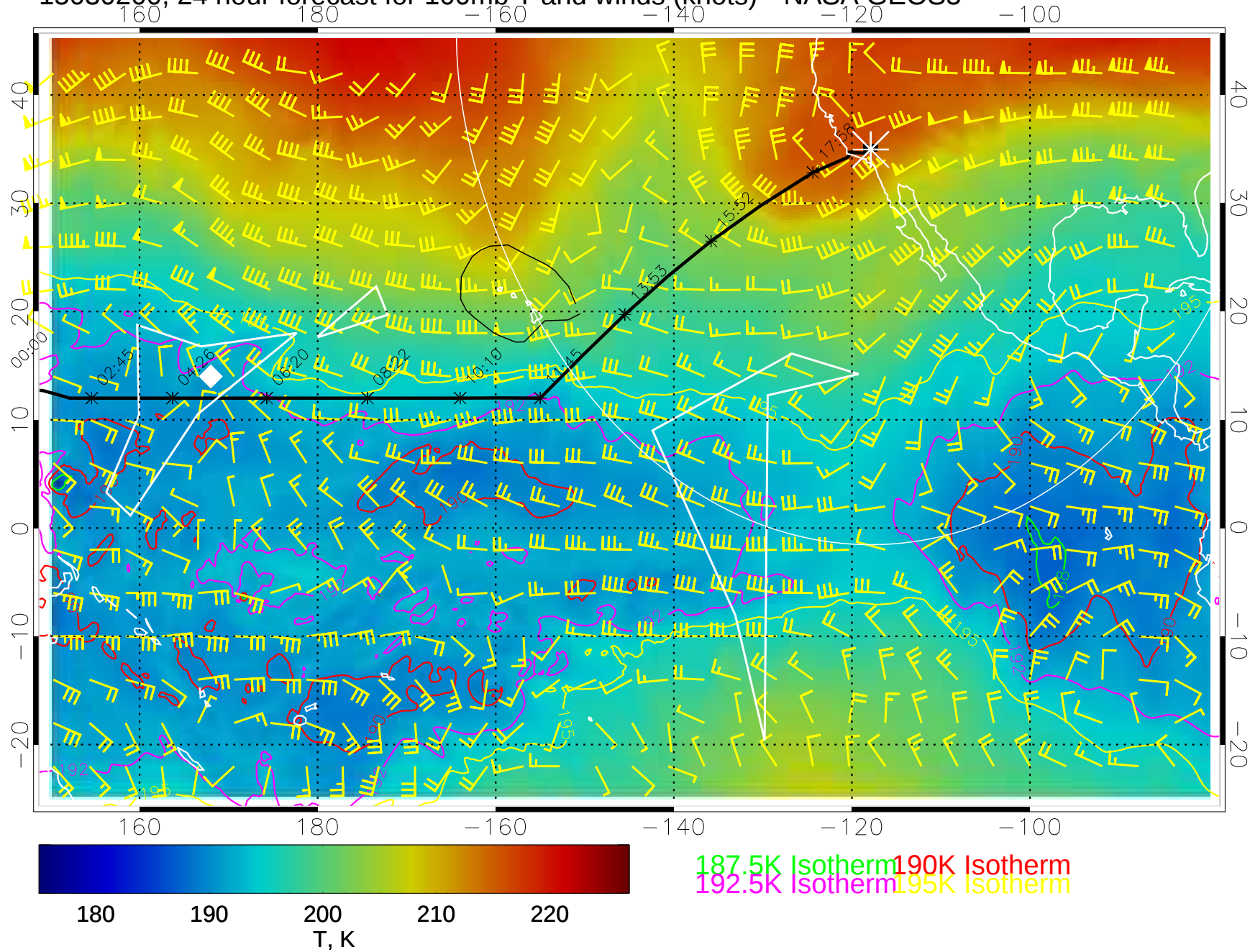
15030200, 24 hour forecast for 100mb T and winds (knots)-- NASA GEOS5
