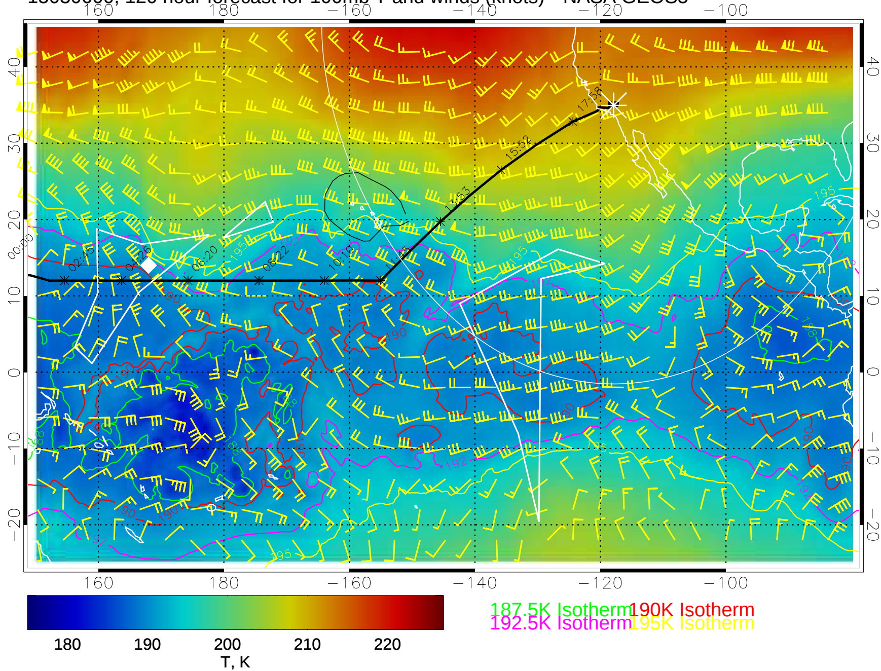
15030600, 120 hour forecast for 100mb T and winds (knots)-- NASA GEOS5
