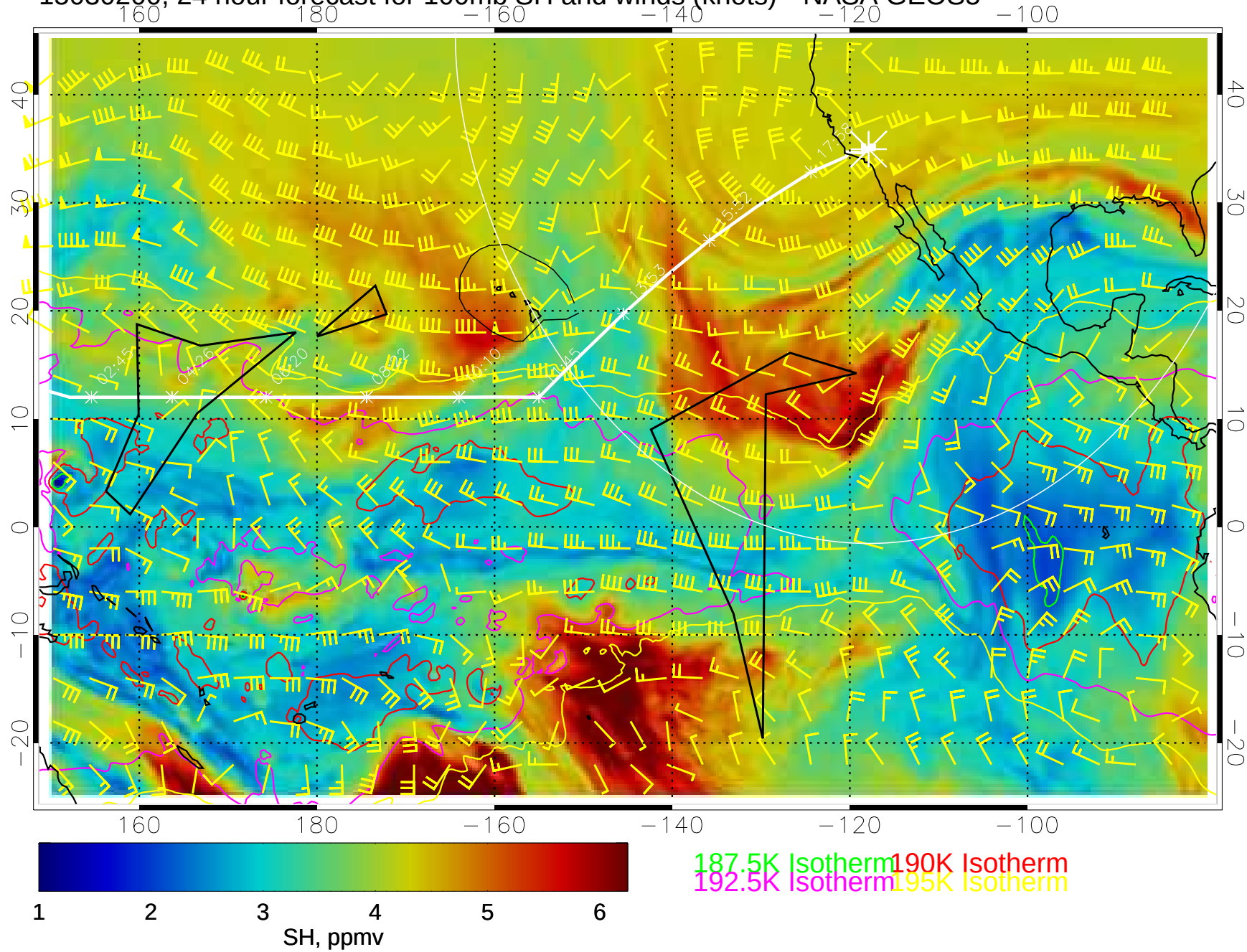
15030200, 24 hour forecast for 100mb SH and winds (knots)-- NASA GEOS5
