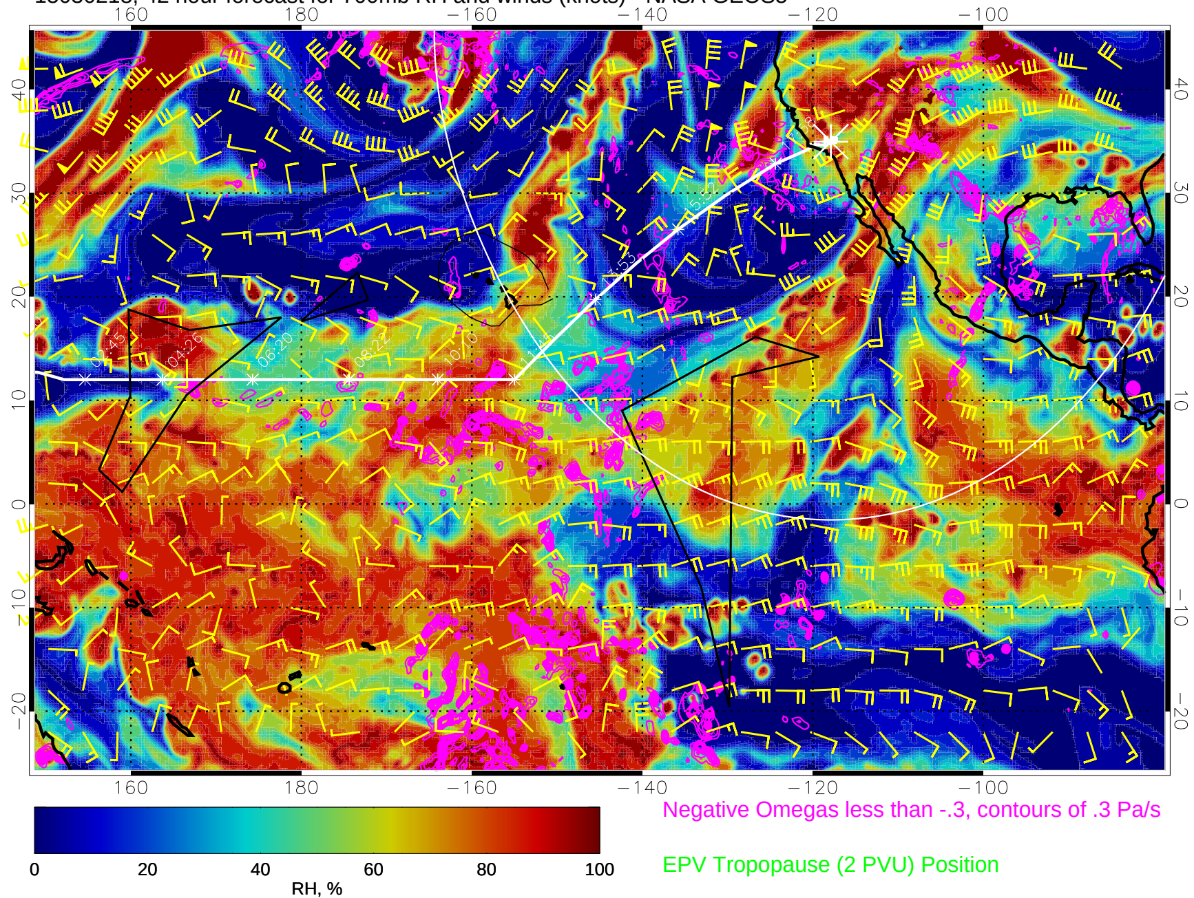
15030218, 42 hour forecast for 700mb RH and winds (knots) - NASA GEOS5
