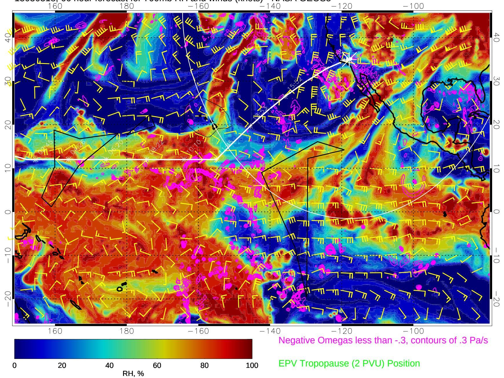
15030318, 66 hour forecast for 700mb RH and winds (knots) - NASA GEOS5
