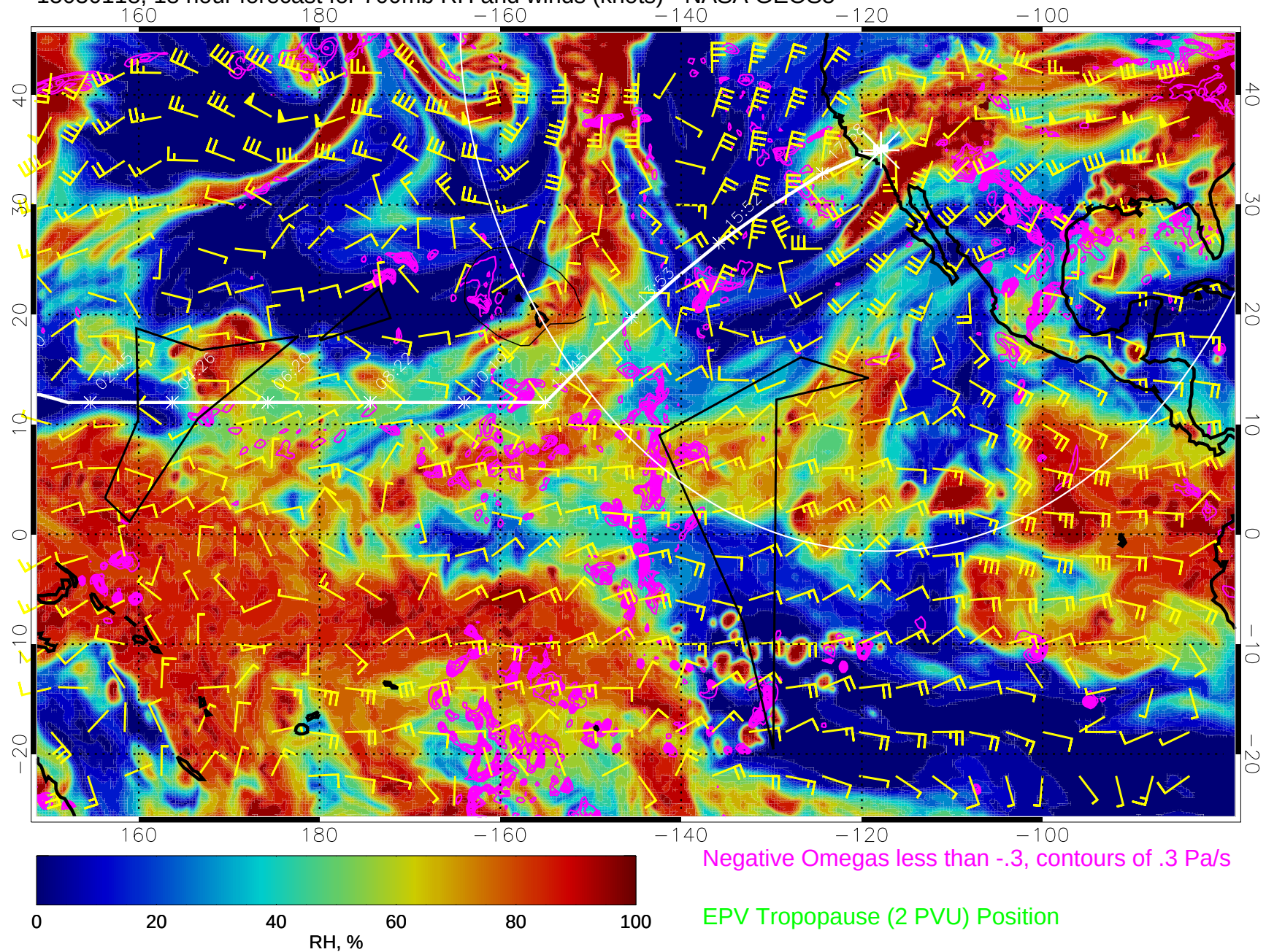
15030118, 18 hour forecast for 700mb RH and winds (knots) - NASA GEOS5
