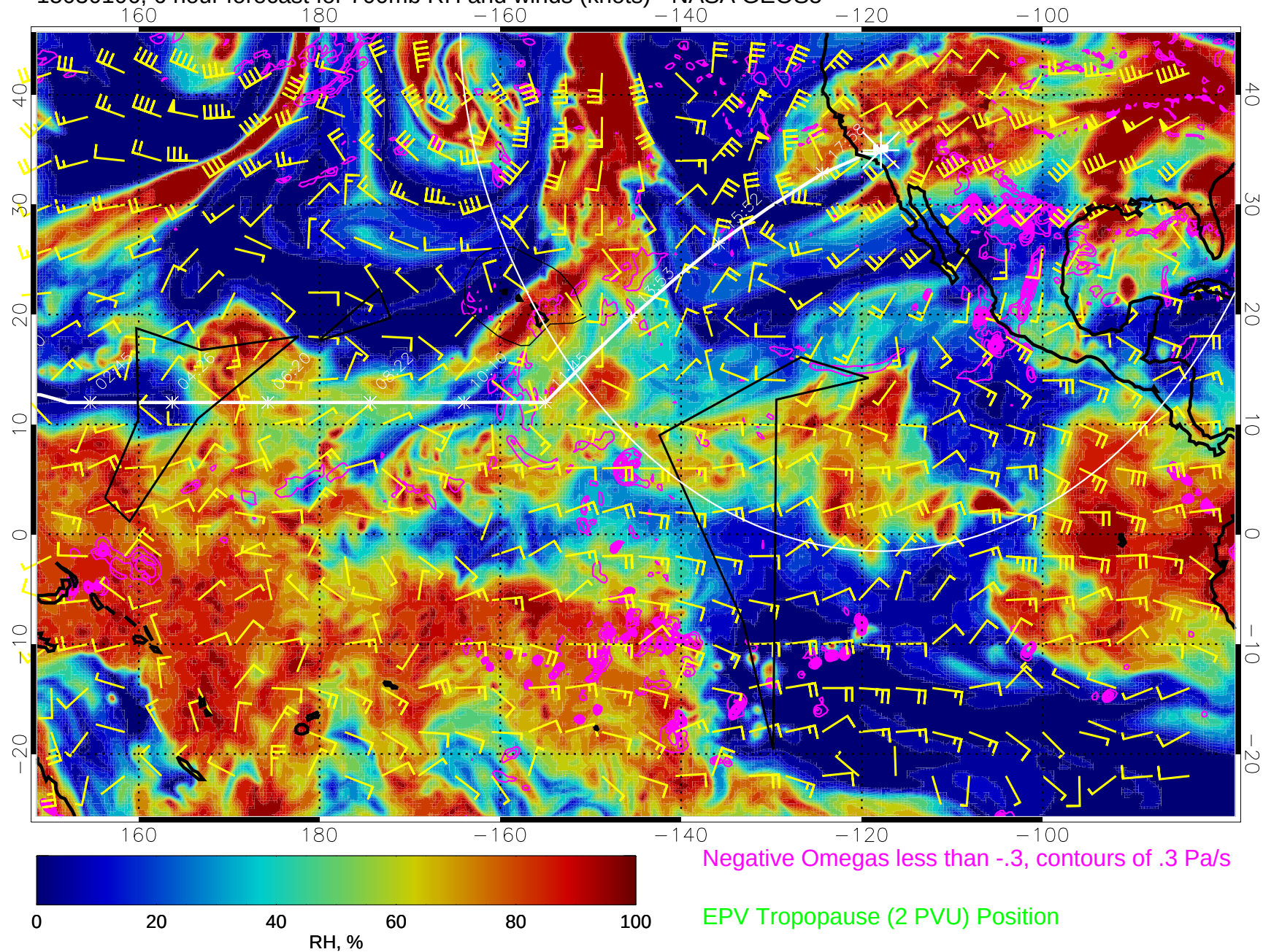
15030106, 6 hour forecast for 700mb RH and winds (knots) - NASA GEOS5
