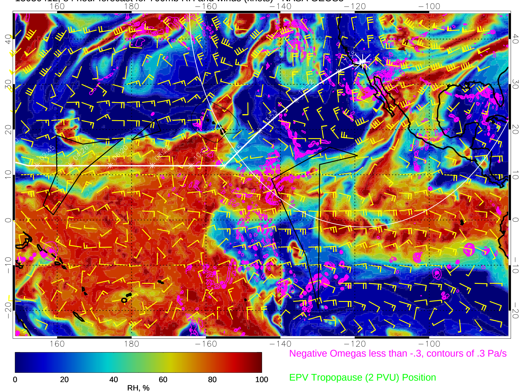
15030412, 84 hour forecast for 700mb RH and winds (knots) - NASA GEOS5
