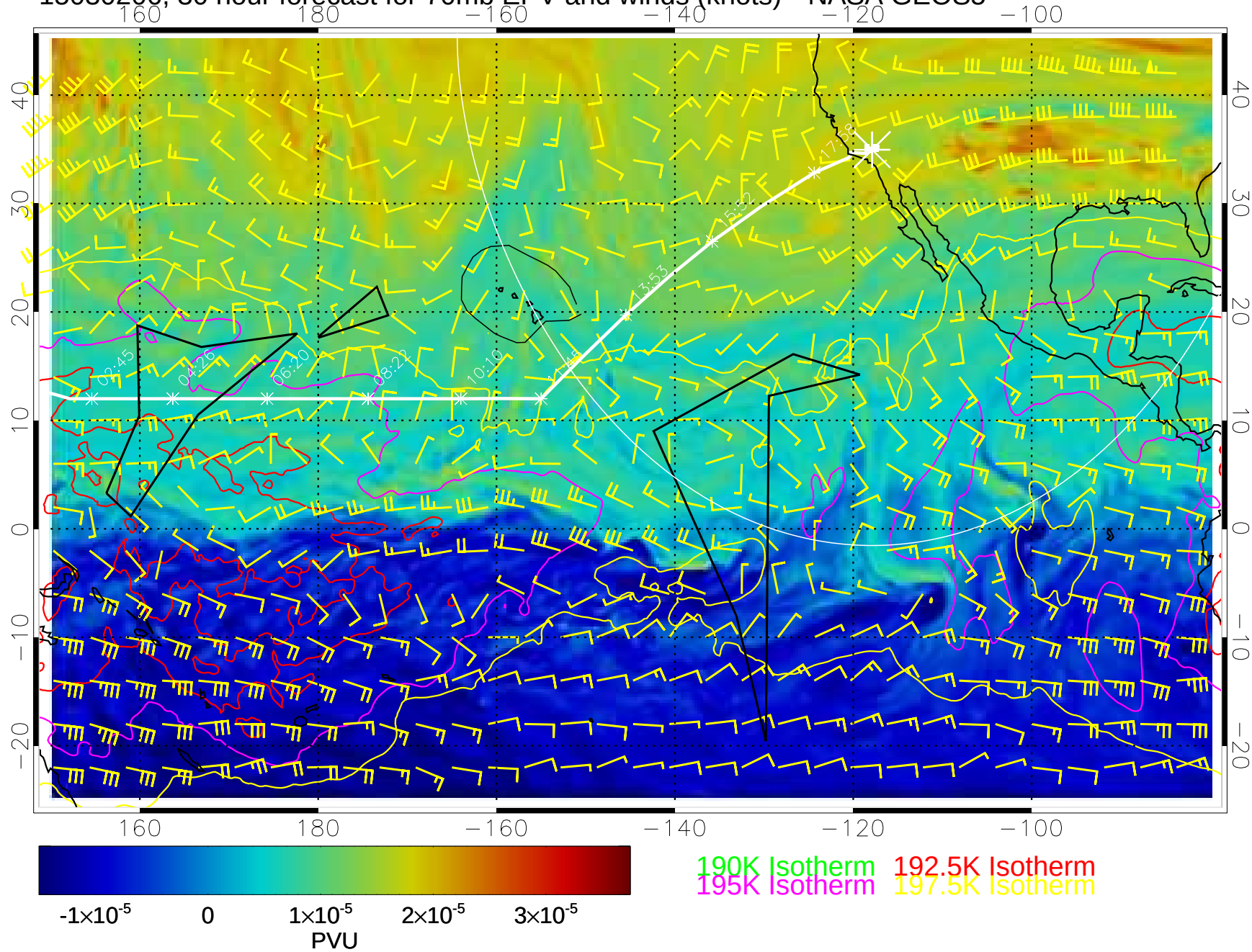
15030206, 30 hour forecast for 70mb EPV and winds (knots)-- NASA GEOS5
