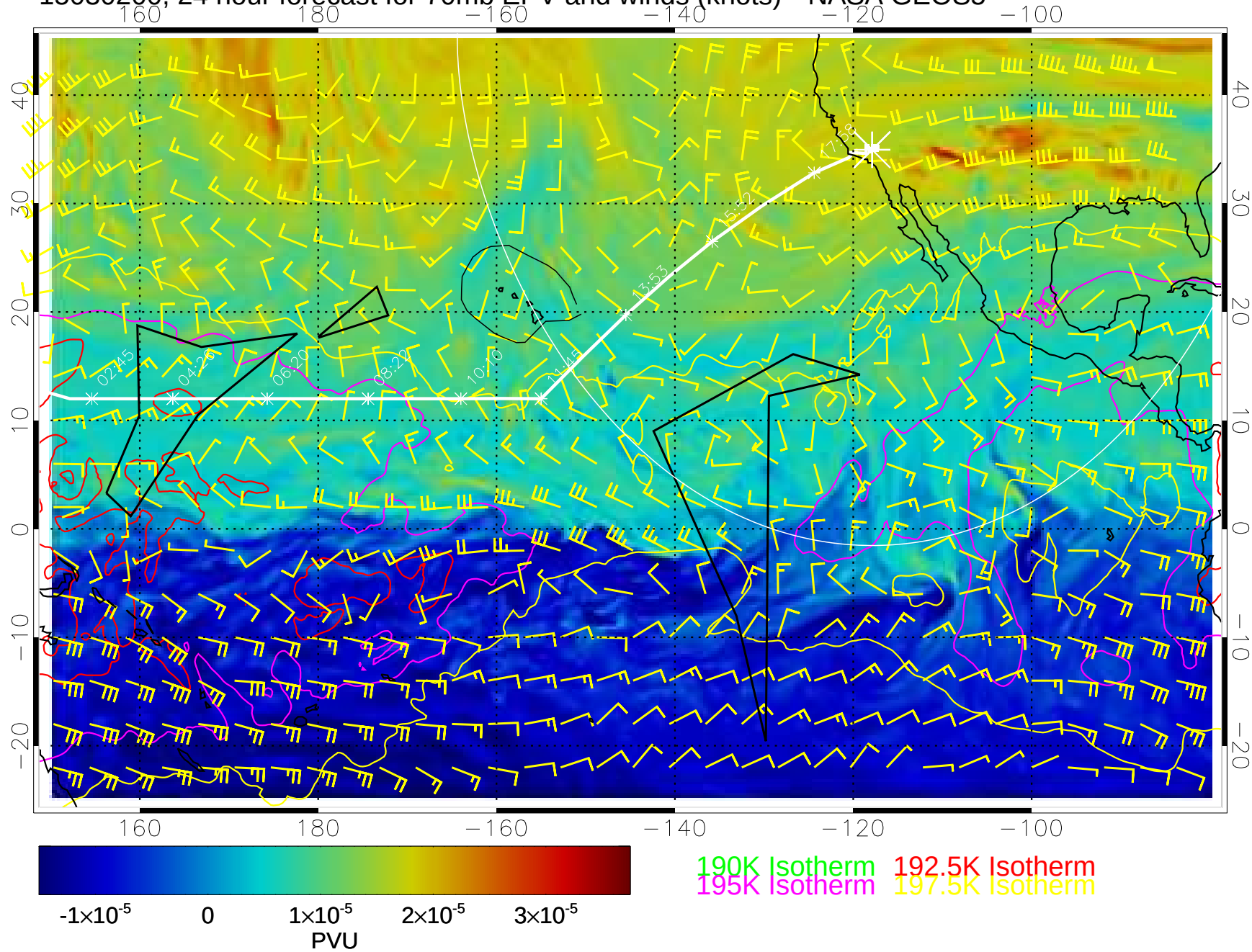
15030200, 24 hour forecast for 70mb EPV and winds (knots)-- NASA GEOS5
