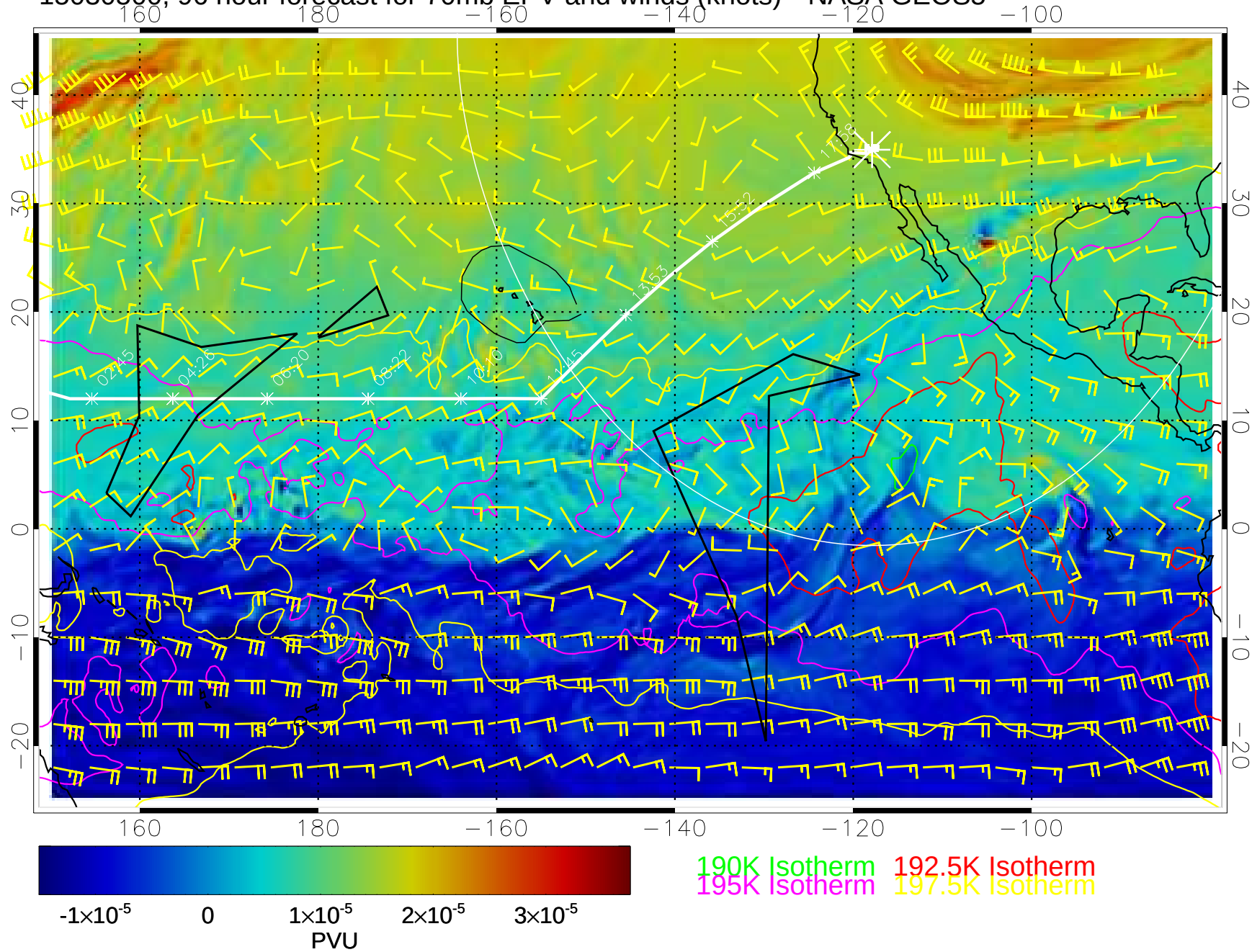
15030500, 96 hour forecast for 70mb EPV and winds (knots)-- NASA GEOS5
