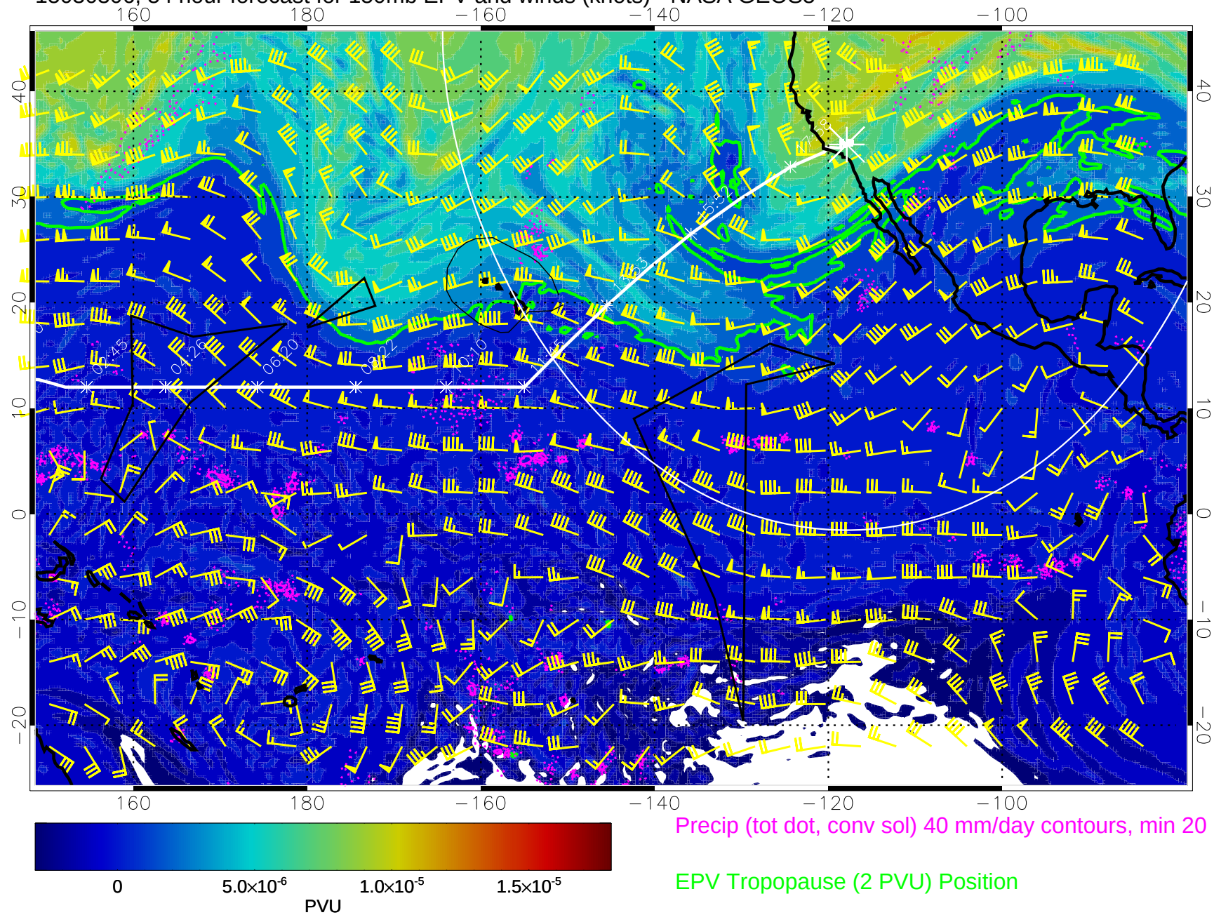
15030306, 54 hour forecast for 150mb EPV and winds (knots) - NASA GEOS5
