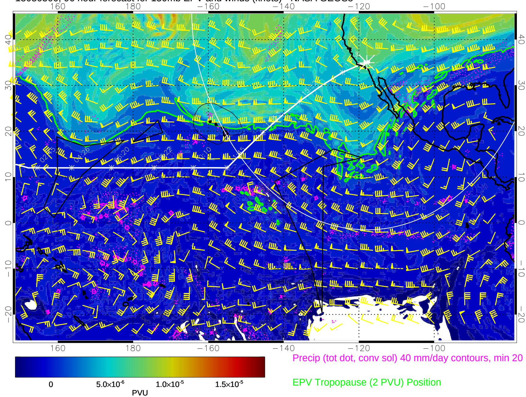
15030500, 96 hour forecast for 150mb EPV and winds (knots) - NASA GEOS5
