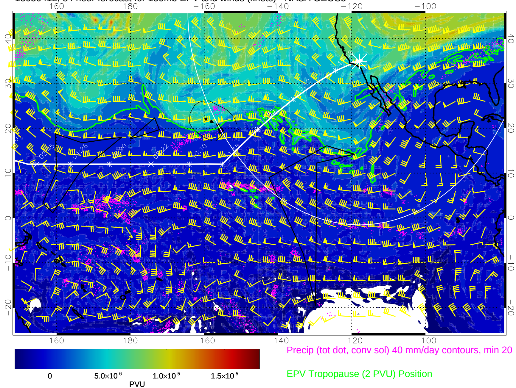
15030412, 84 hour forecast for 150mb EPV and winds (knots) - NASA GEOS5
