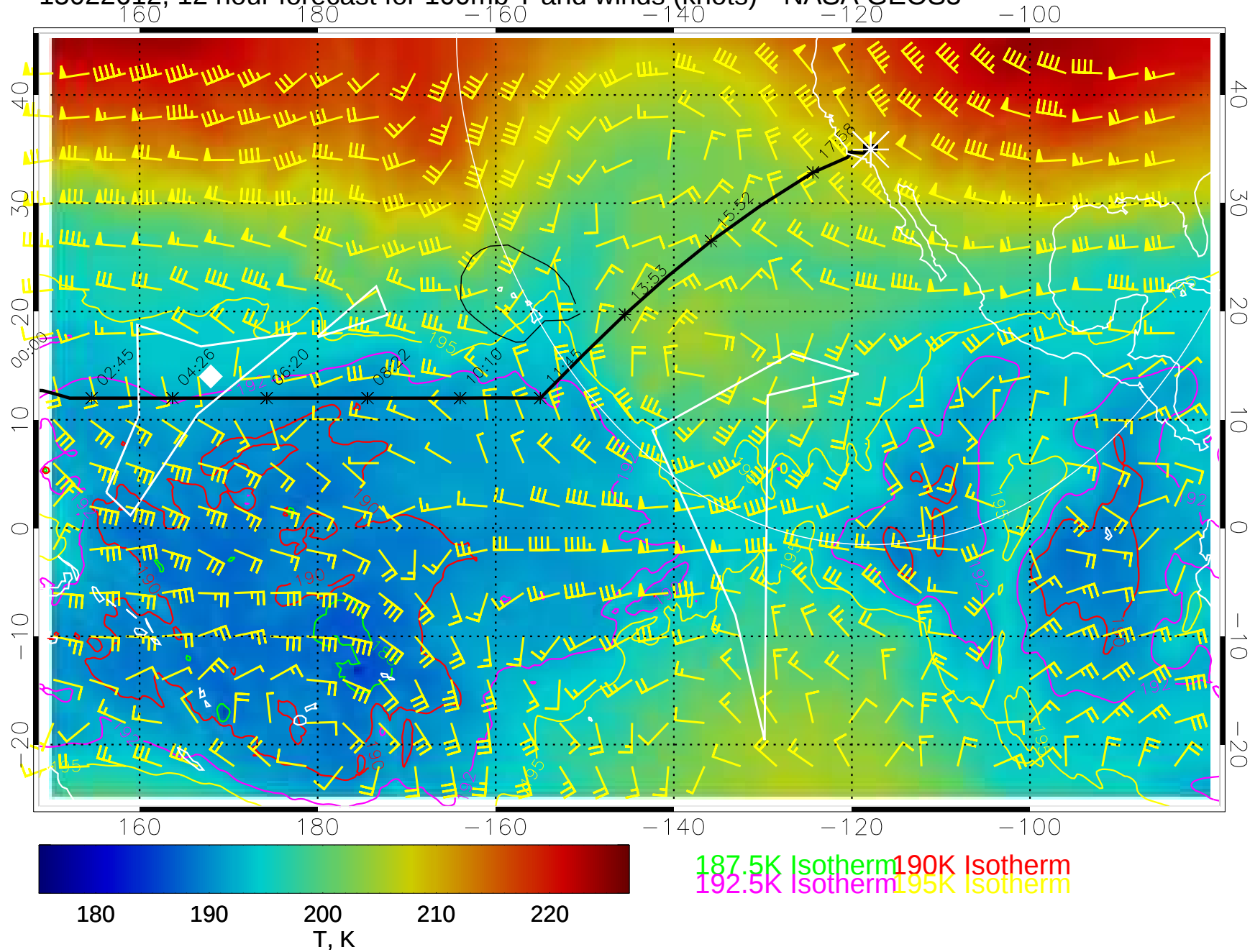
15022612, 12 hour forecast for 100mb T and winds (knots)-- NASA GEOS5
