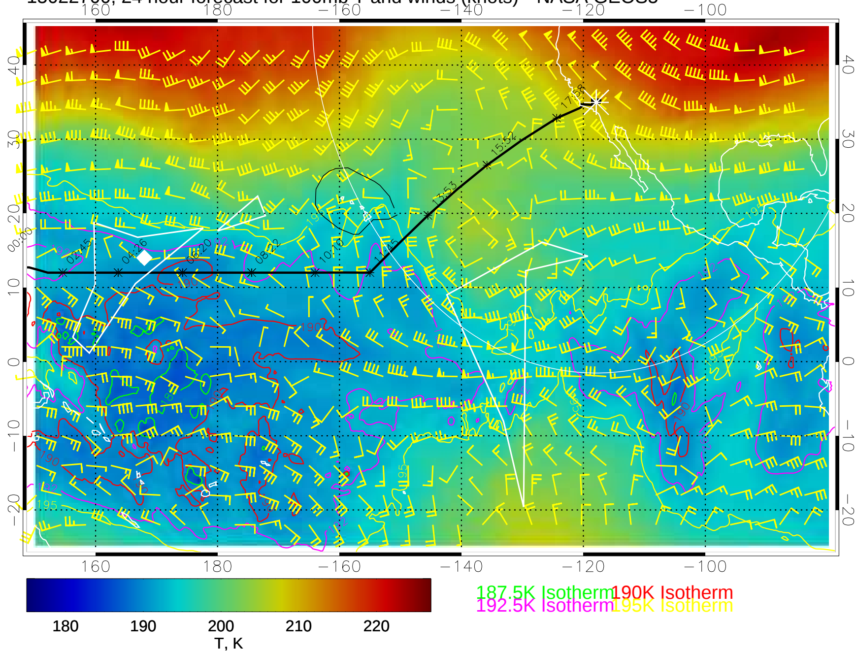
15022700, 24 hour forecast for 100mb T and winds (knots)-- NASA GEOS5
