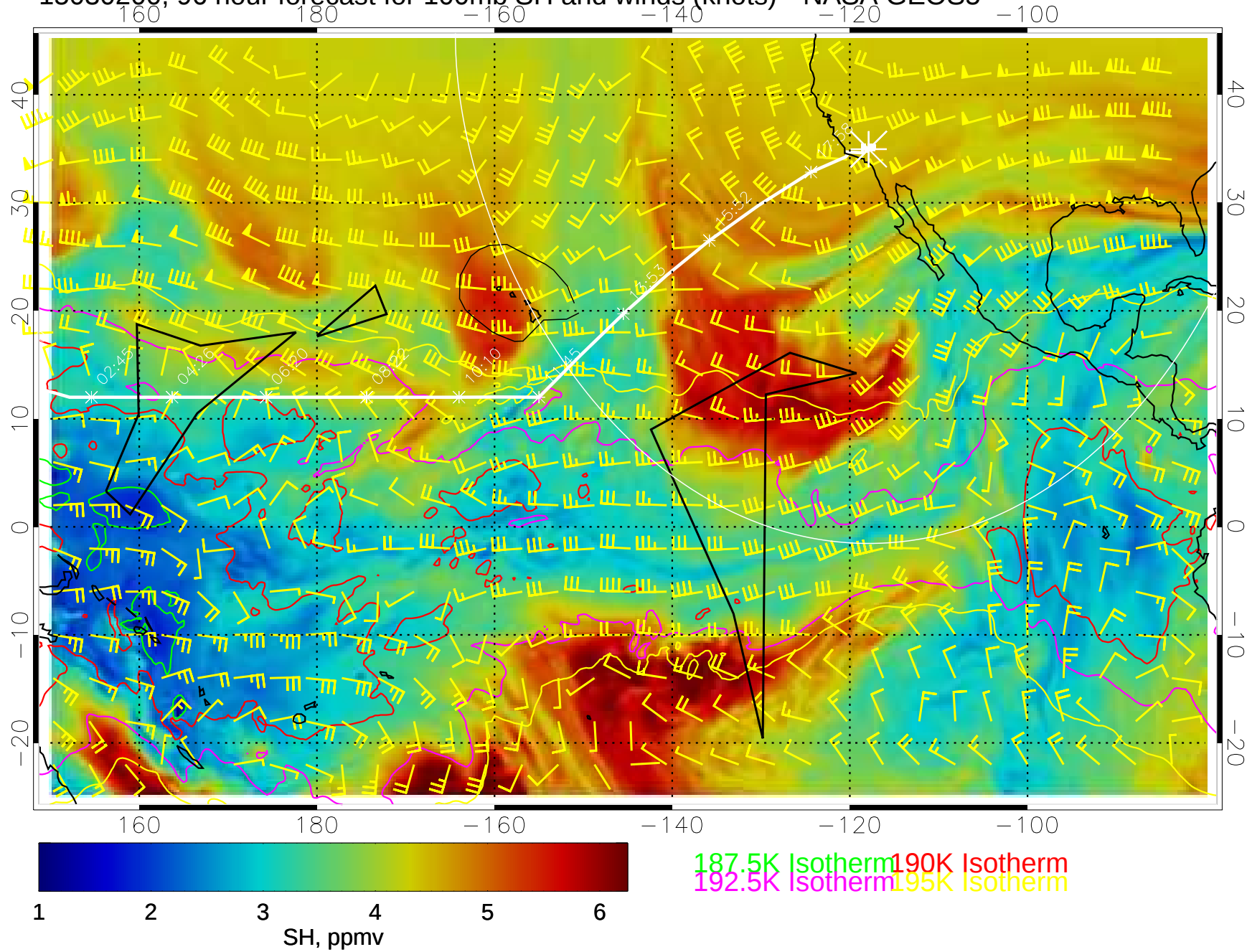
15030200, 96 hour forecast for 100mb SH and winds (knots)-- NASA GEOS5
