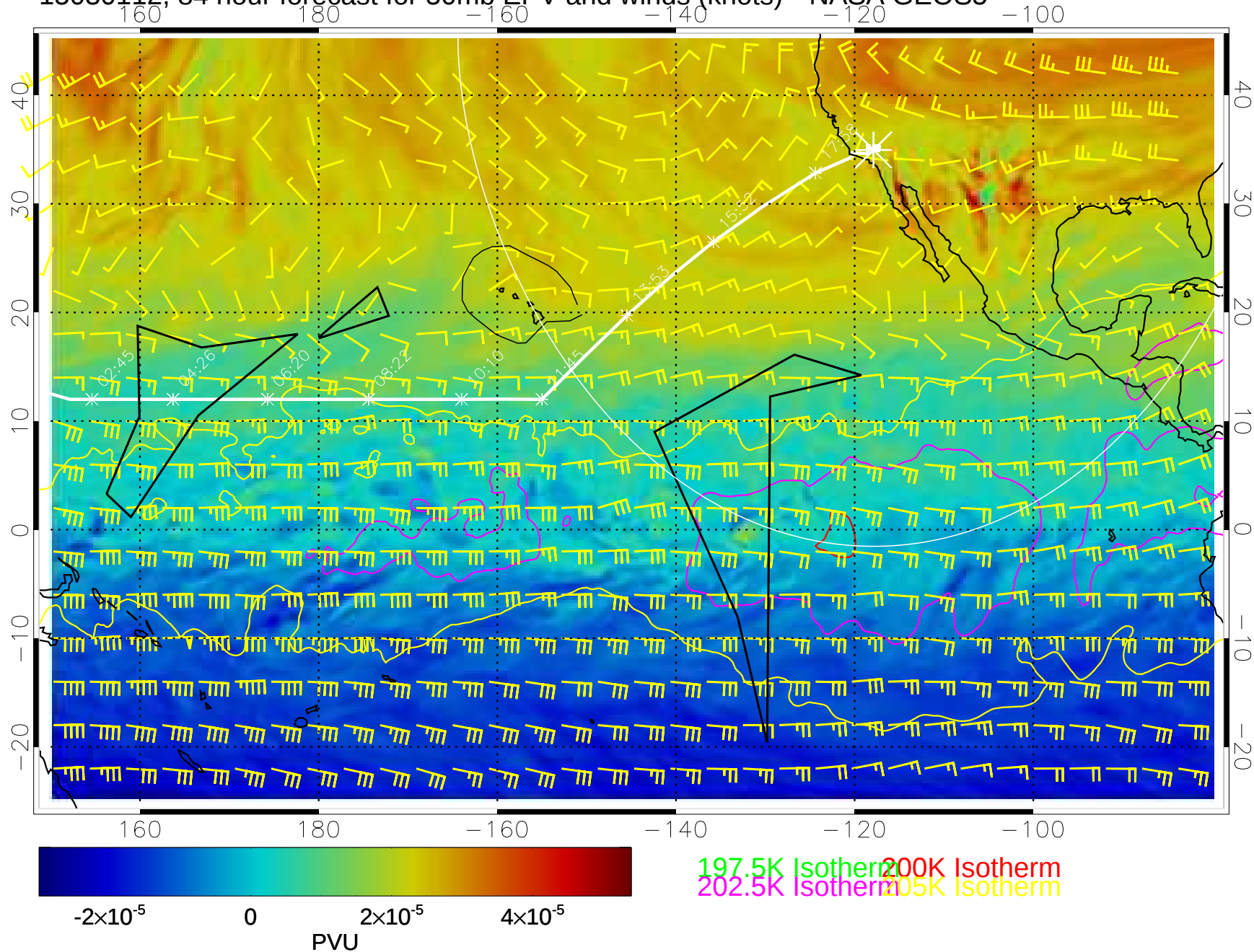
15030112, 84 hour forecast for 50mb EPV and winds (knots)-- NASA GEOS5
