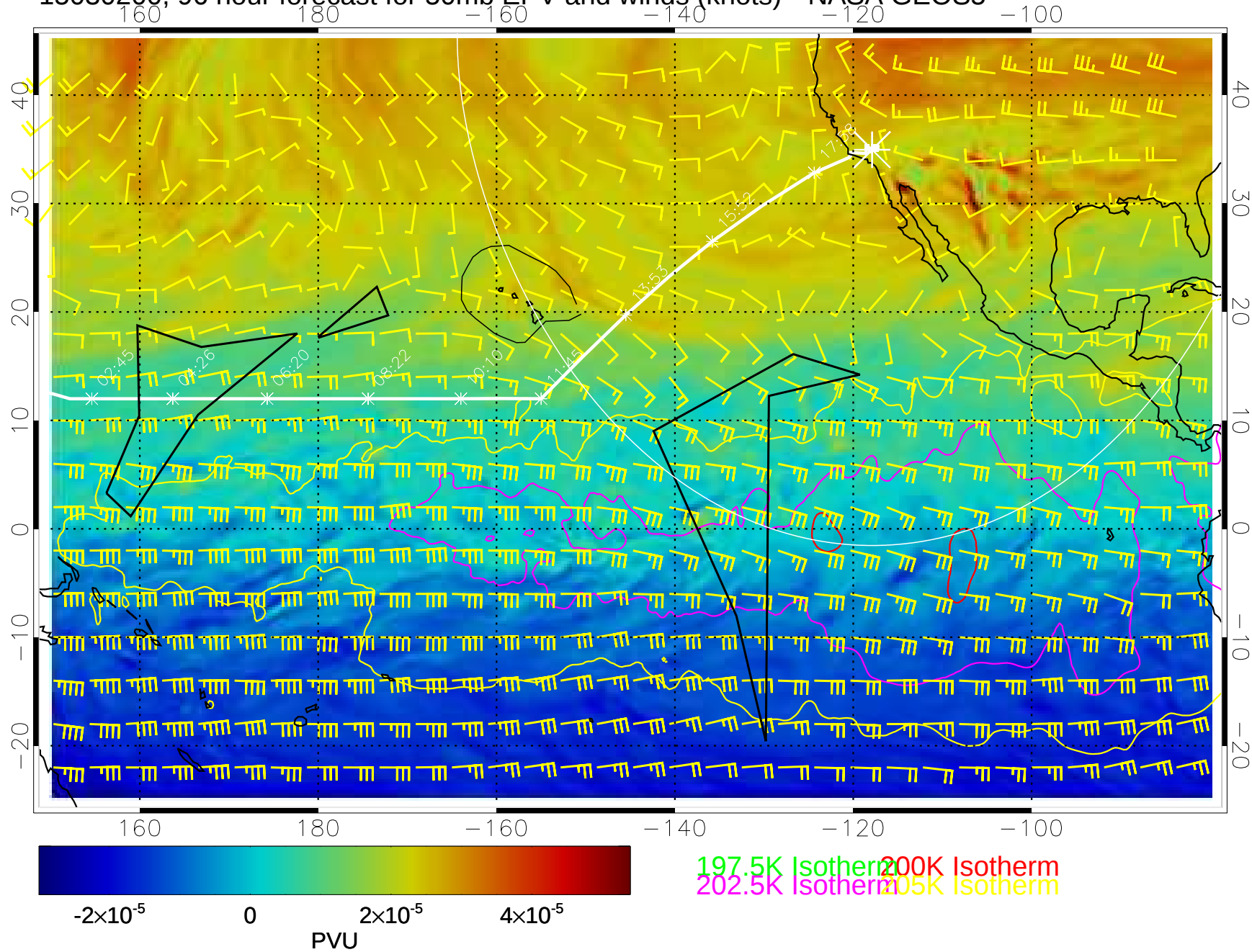
15030200, 96 hour forecast for 50mb EPV and winds (knots)-- NASA GEOS5
