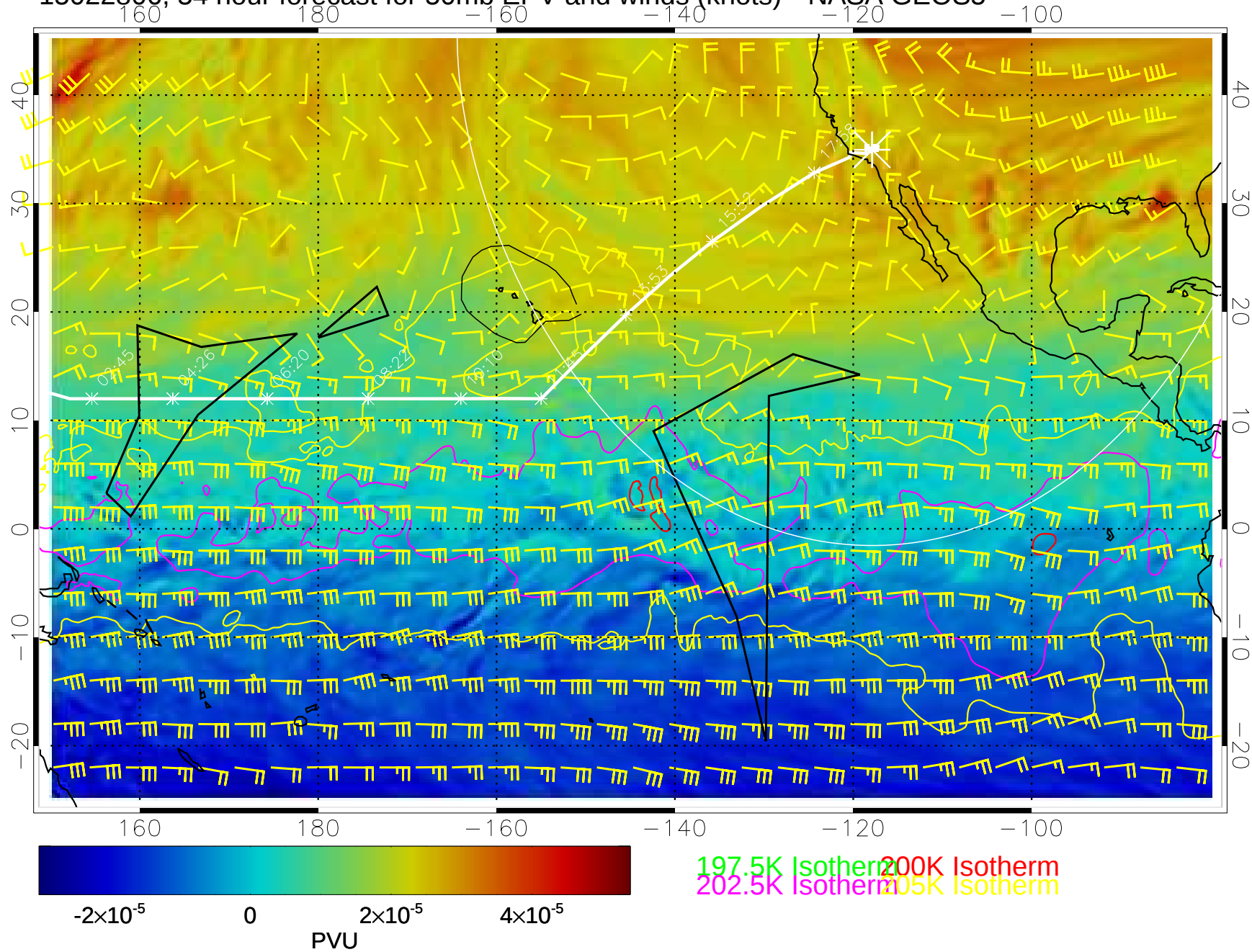
15022806, 54 hour forecast for 50mb EPV and winds (knots)-- NASA GEOS5
