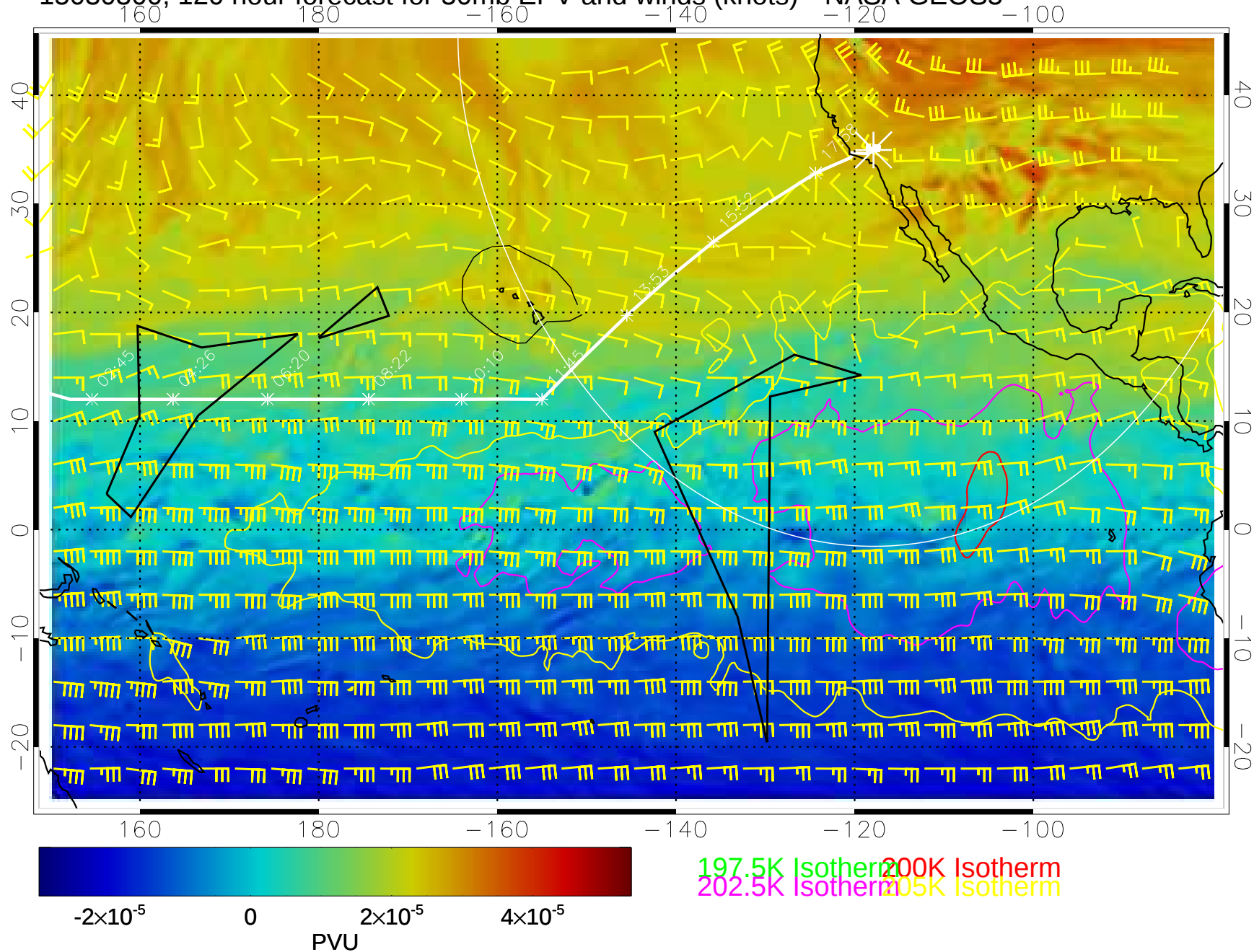
15030300, 120 hour forecast for 50mb EPV and winds (knots)-- NASA GEOS5
