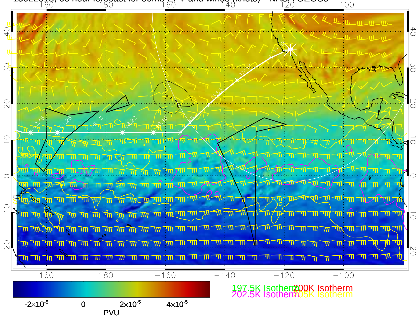
15022818, 66 hour forecast for 50mb EPV and winds (knots)-- NASA GEOS5
