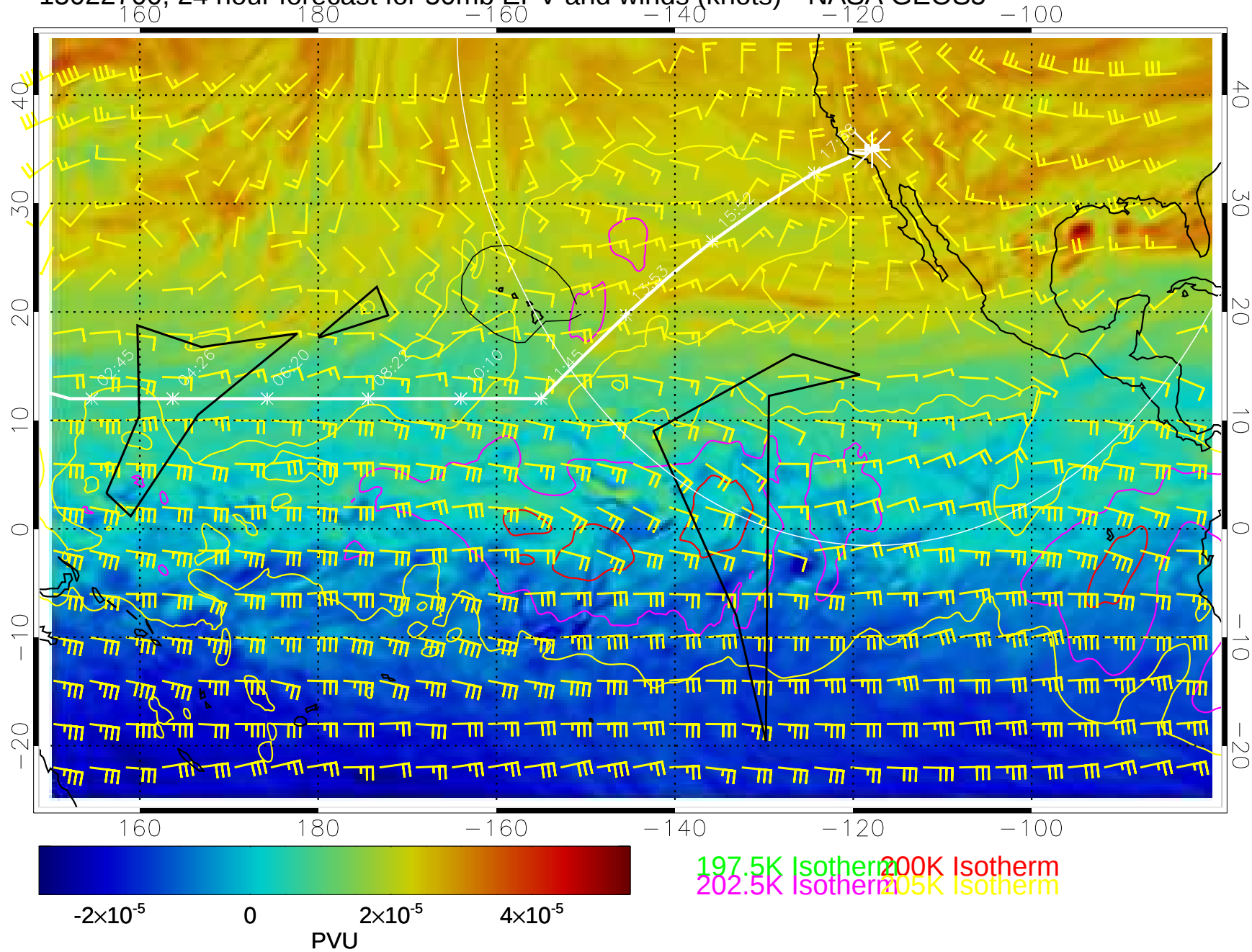
15022700, 24 hour forecast for 50mb EPV and winds (knots)-- NASA GEOS5
