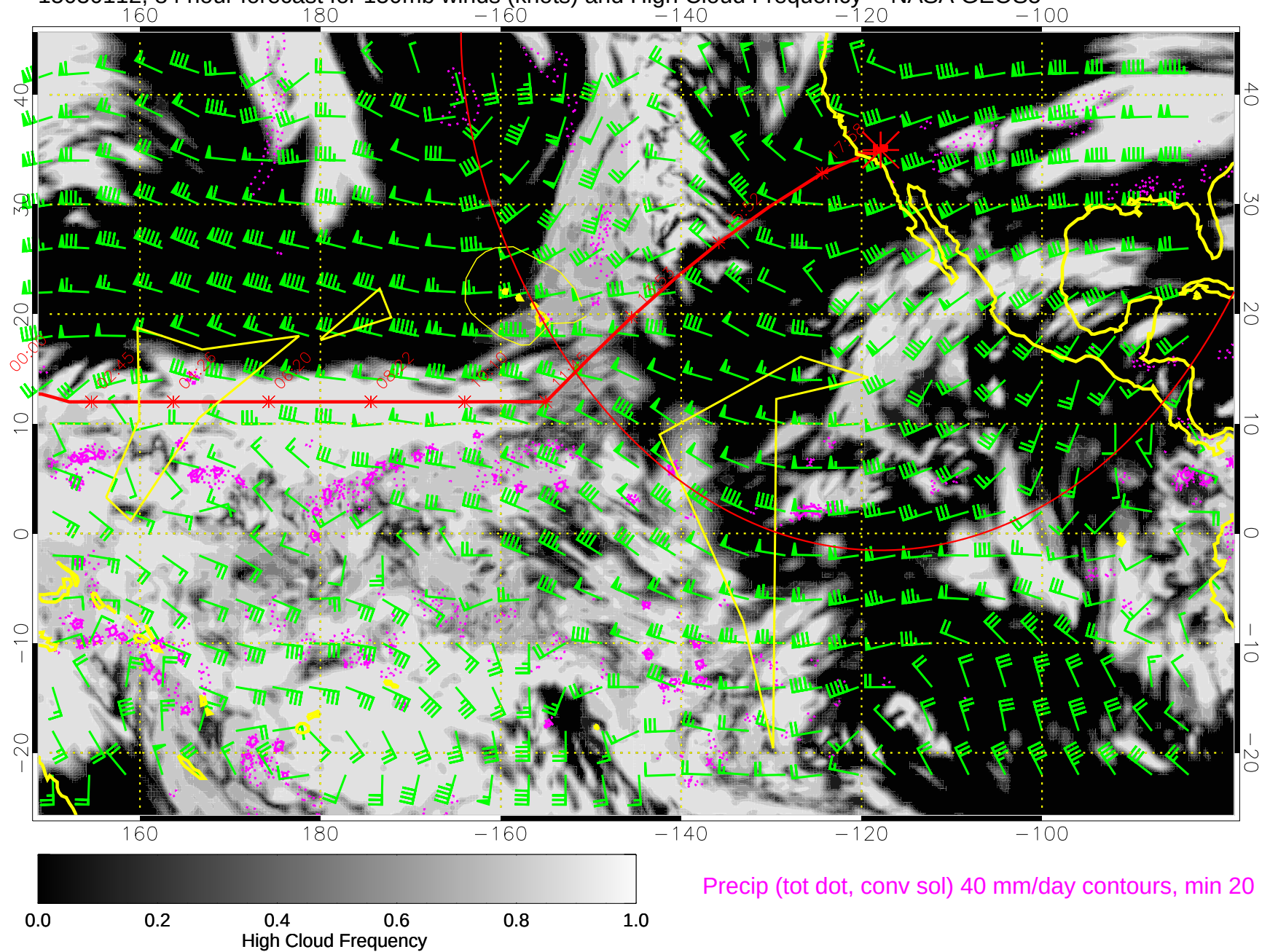
15030112, 84 hour forecast for 150mb winds (knots) and High Cloud Frequency -- NASA GEOS5
