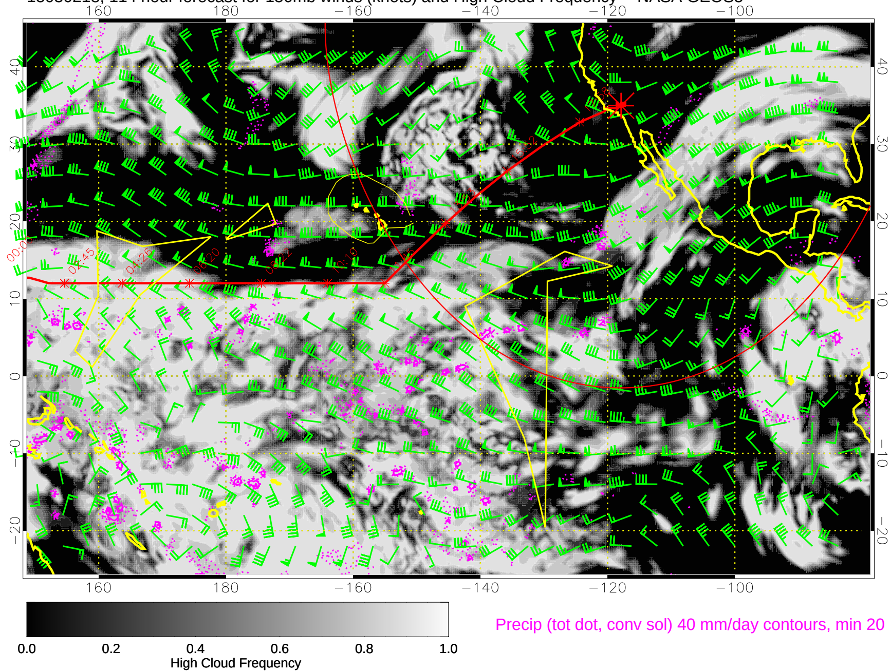
15030218, 114 hour forecast for 150mb winds (knots) and High Cloud Frequency -- NASA GEOS5
