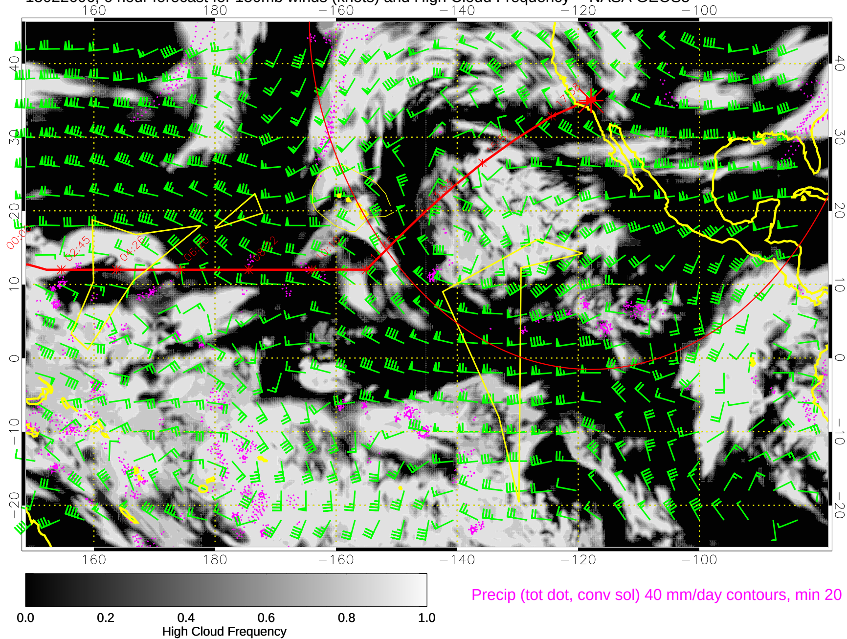
15022606, 6 hour forecast for 150mb winds (knots) and High Cloud Frequency -- NASA GEOS5
