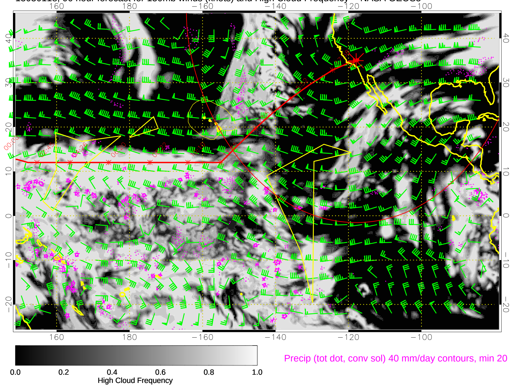
15030118, 90 hour forecast for 150mb winds (knots) and High Cloud Frequency -- NASA GEOS5
