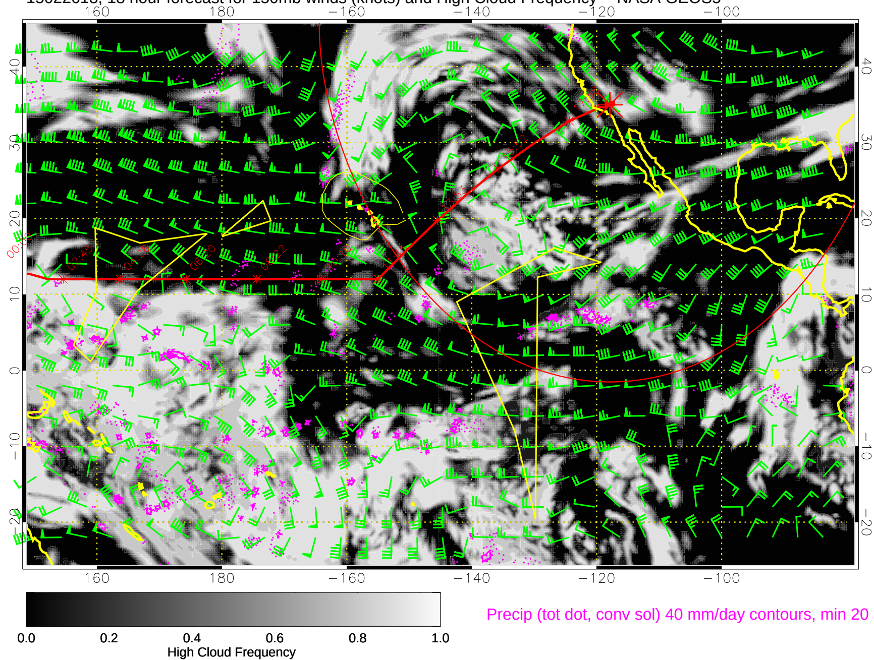
15022618, 18 hour forecast for 150mb winds (knots) and High Cloud Frequency -- NASA GEOS5
