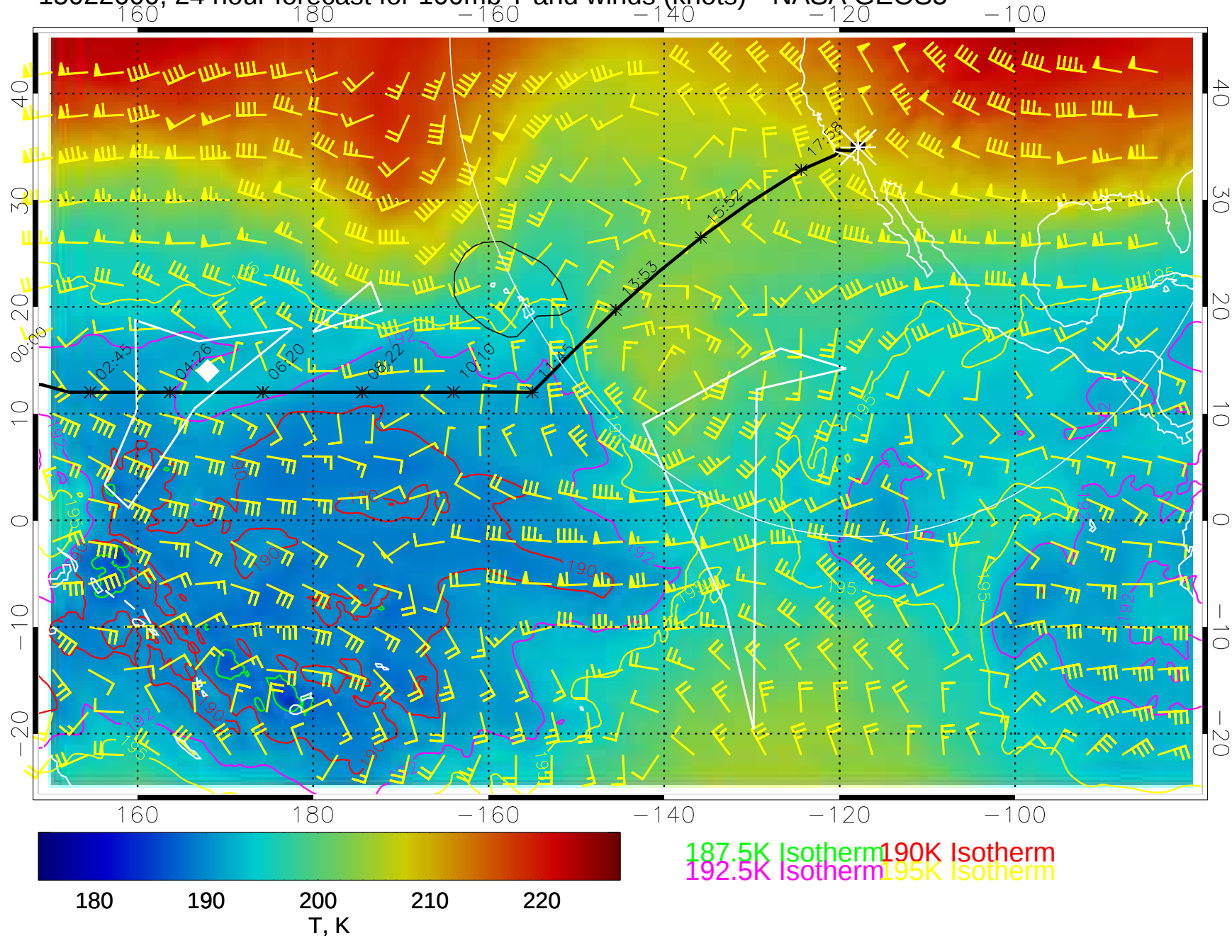
15022600, 24 hour forecast for 100mb T and winds (knots)-- NASA GEOS5
