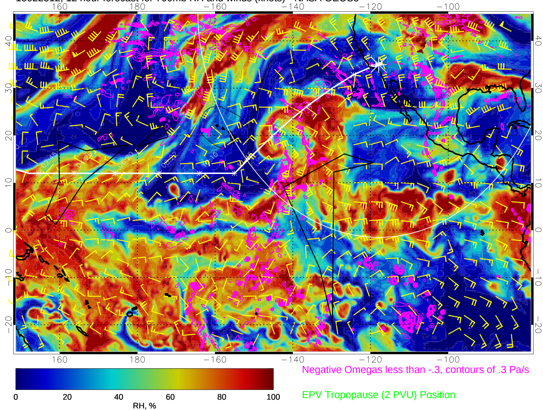
15022512, 12 hour forecast for 700mb RH and winds (knots) - NASA GEOS5
