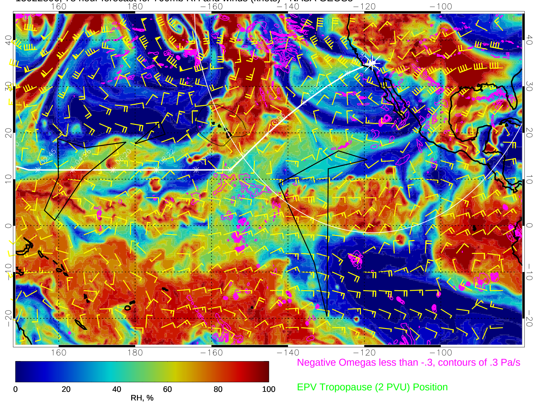
15022806, 78 hour forecast for 700mb RH and winds (knots) - NASA GEOS5
