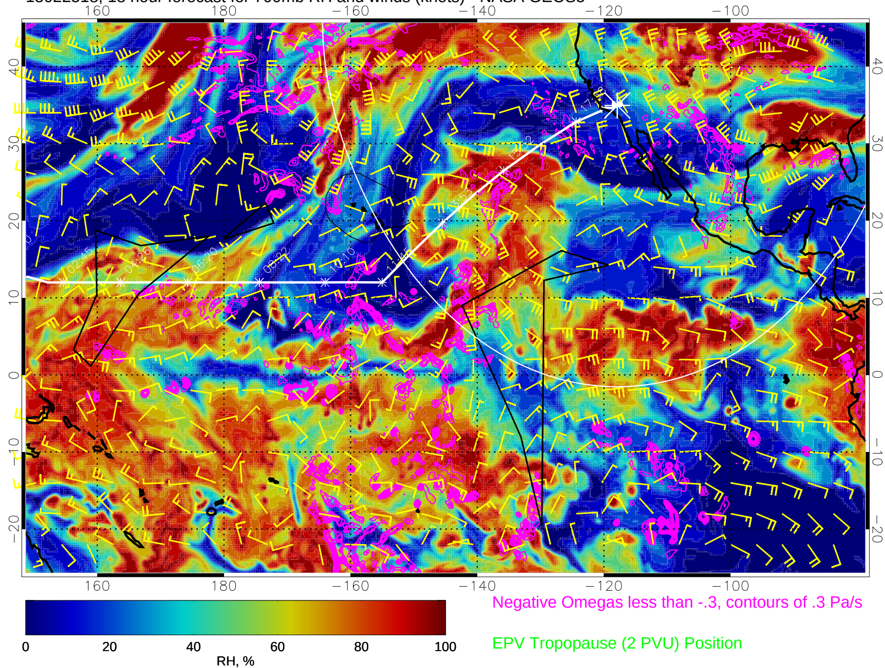
15022518, 18 hour forecast for 700mb RH and winds (knots) - NASA GEOS5
