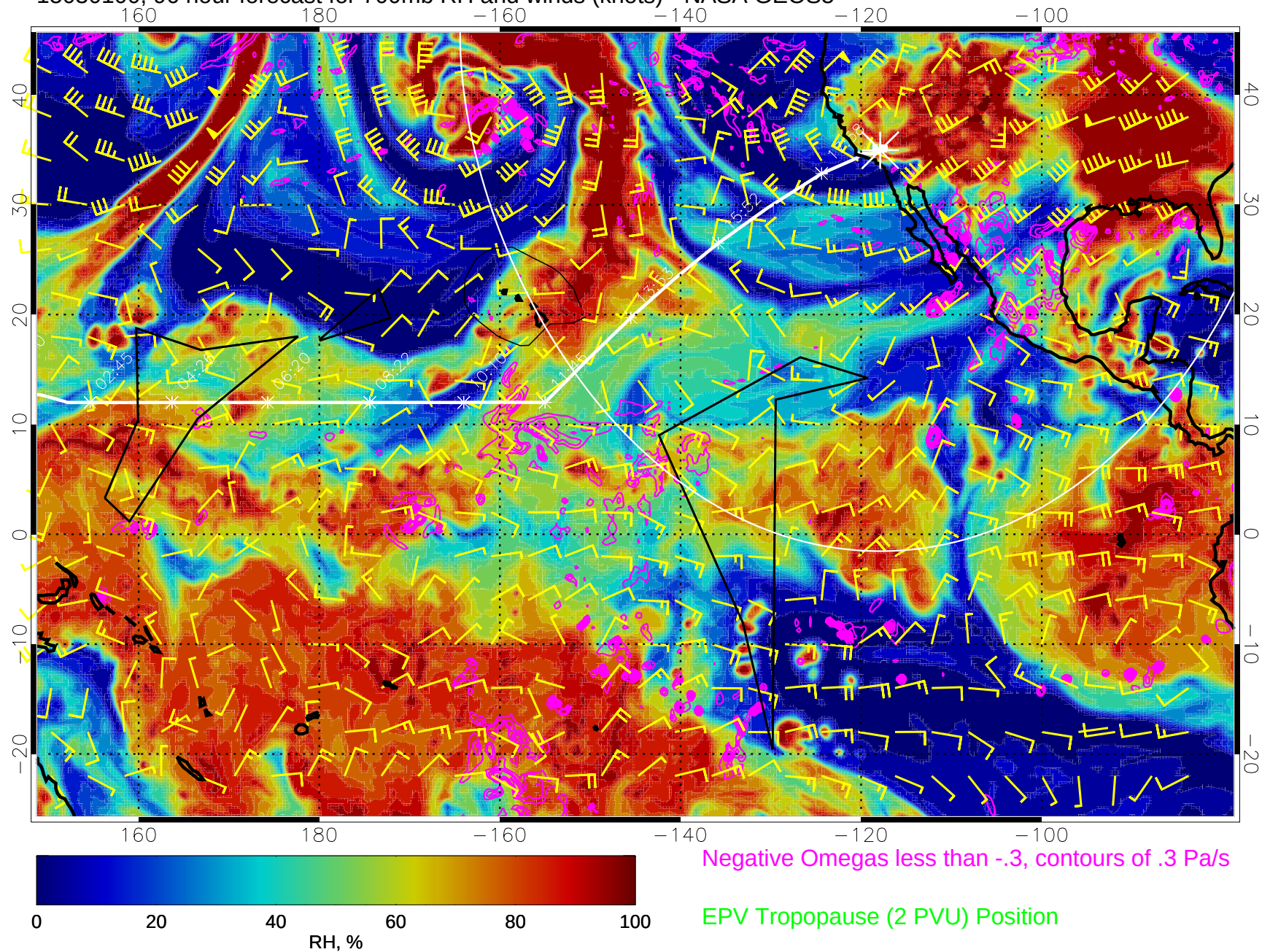
15030100, 96 hour forecast for 700mb RH and winds (knots) - NASA GEOS5
