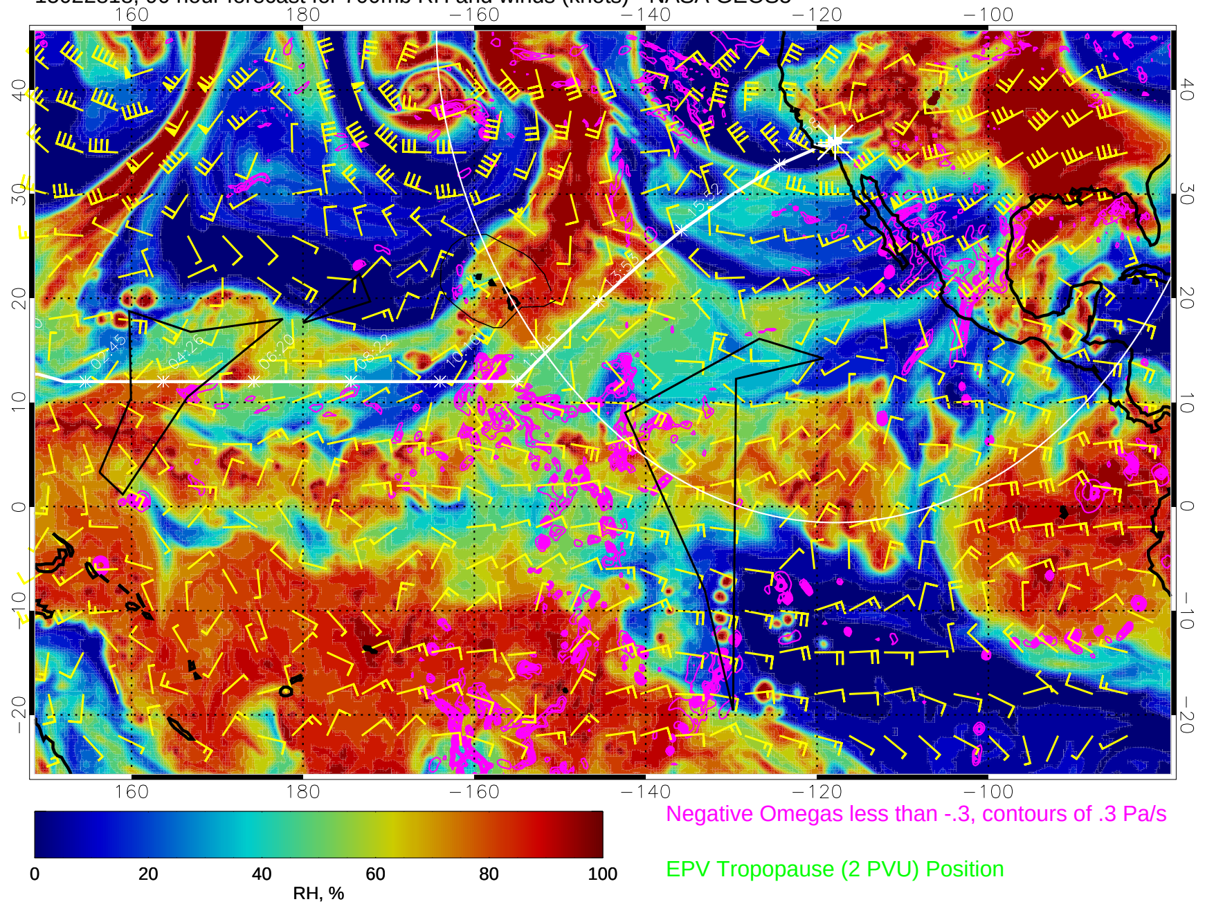
15022818, 90 hour forecast for 700mb RH and winds (knots) - NASA GEOS5
