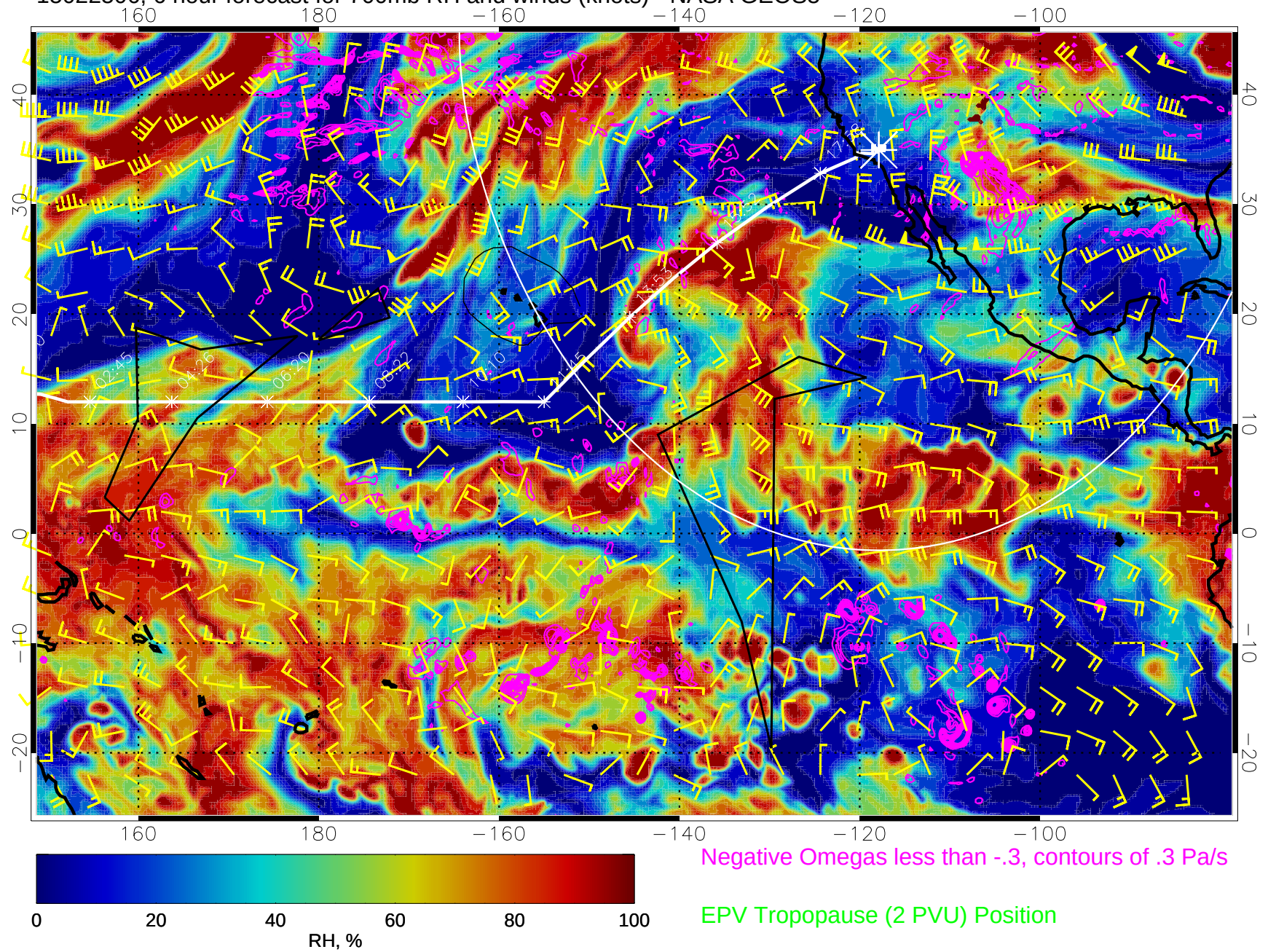
15022506, 6 hour forecast for 700mb RH and winds (knots) - NASA GEOS5
