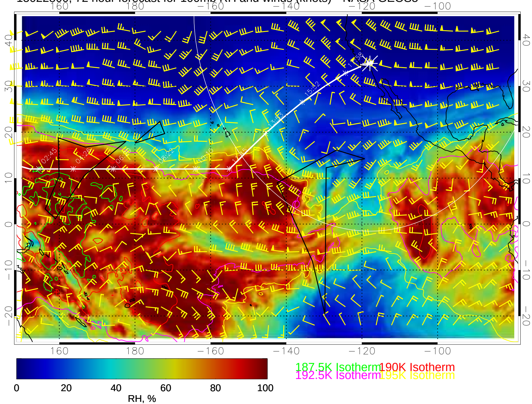
15022800, 72 hour forecast for 100mb RH and winds (knots)-- NASA GEOS5
