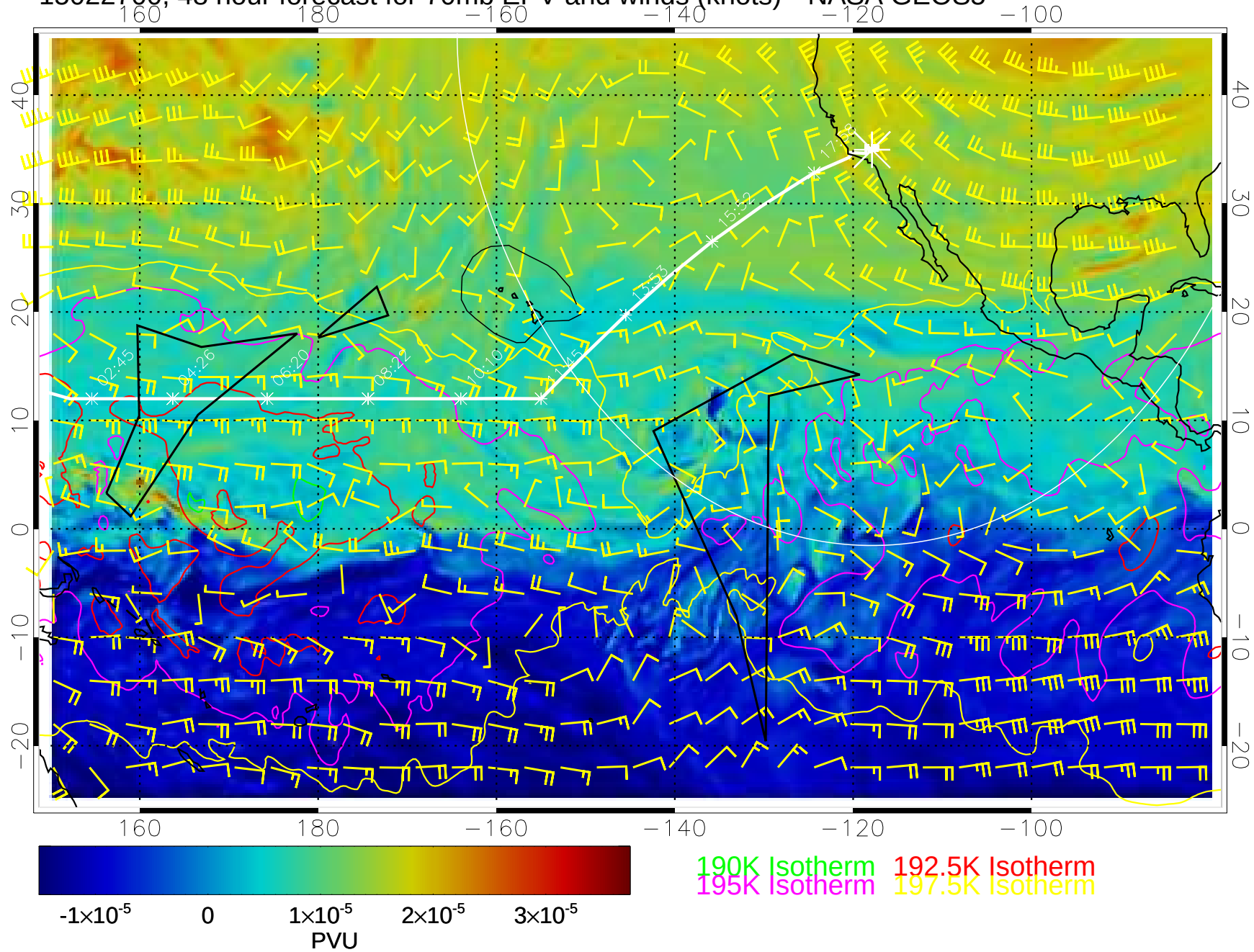
15022700, 48 hour forecast for 70mb EPV and winds (knots)-- NASA GEOS5
