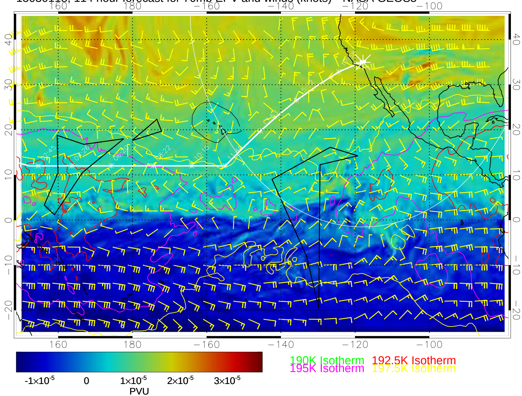
15030118, 114 hour forecast for 70mb EPV and winds (knots)-- NASA GEOS5
