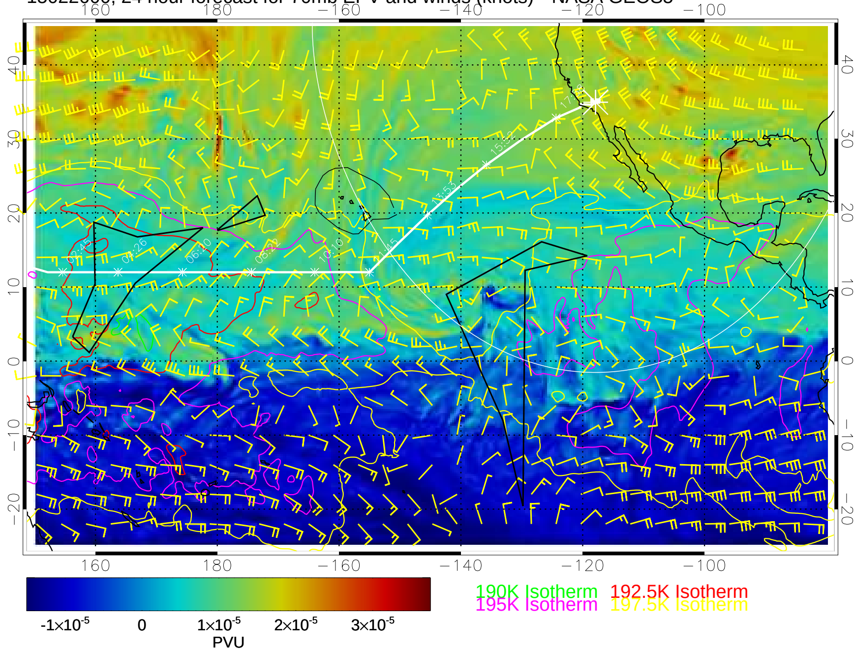
15022600, 24 hour forecast for 70mb EPV and winds (knots)-- NASA GEOS5
