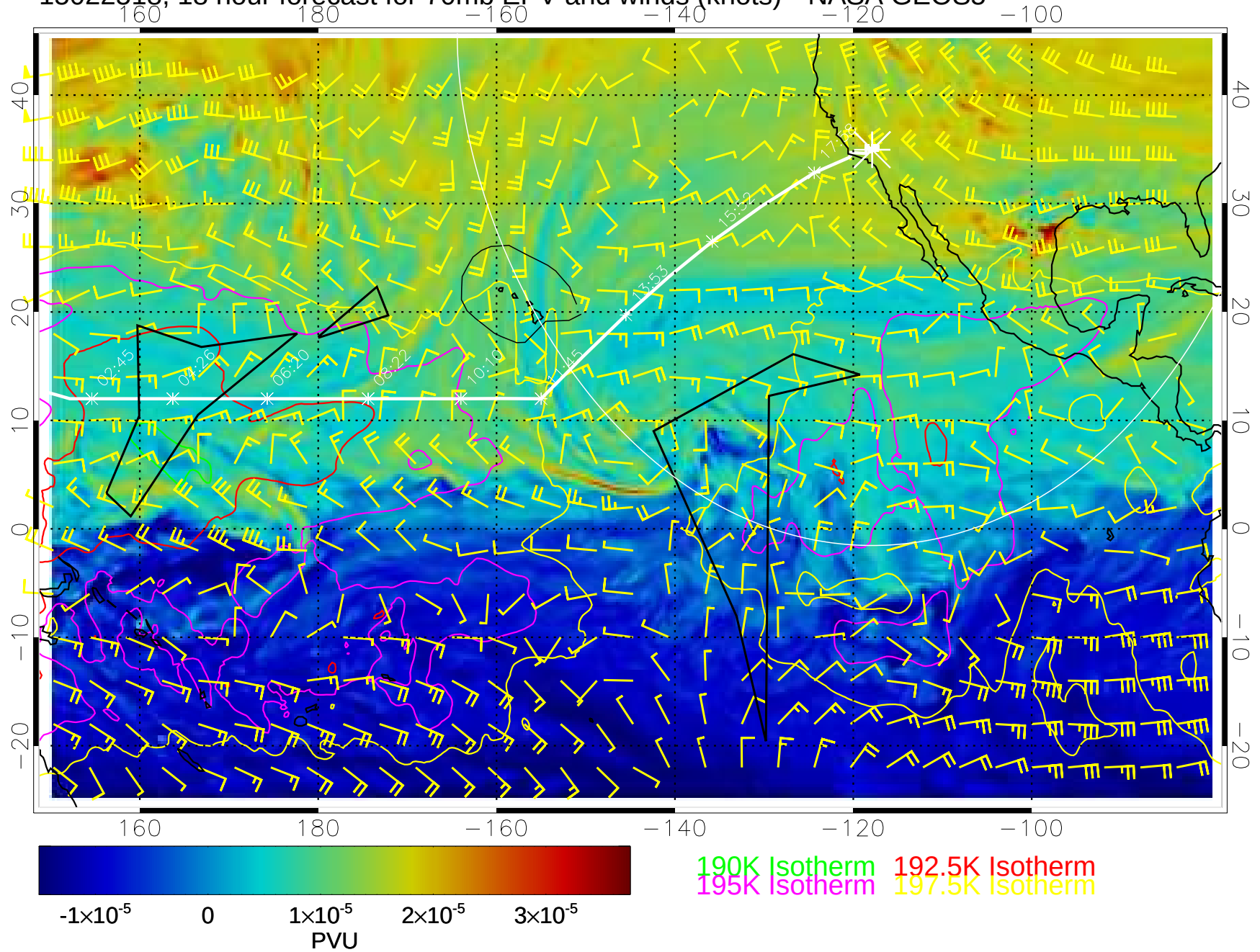
15022518, 18 hour forecast for 70mb EPV and winds (knots)-- NASA GEOS5
