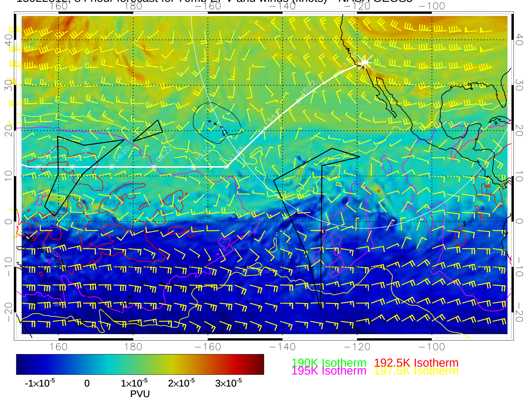
15022812, 84 hour forecast for 70mb EPV and winds (knots)-- NASA GEOS5
