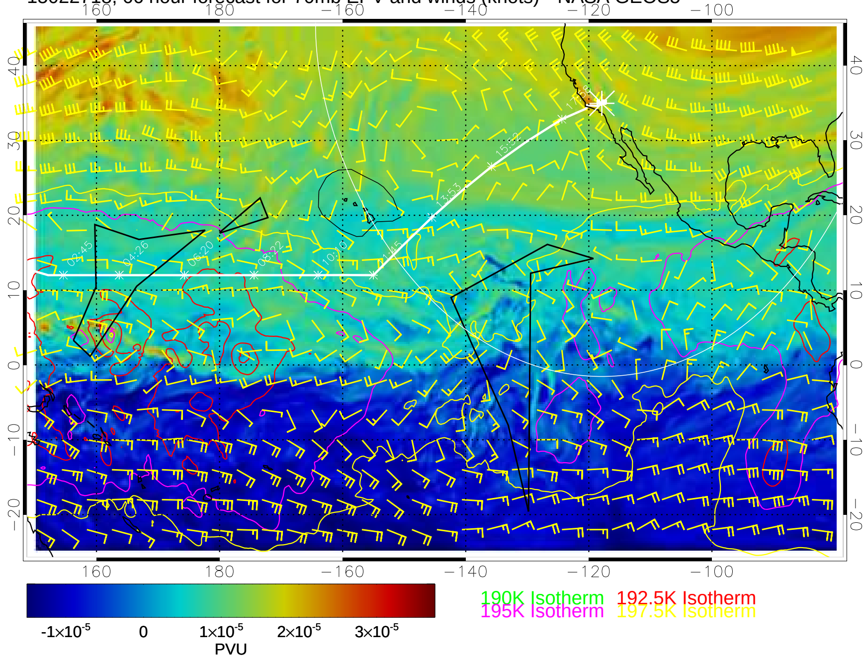
15022718, 66 hour forecast for 70mb EPV and winds (knots)-- NASA GEOS5
