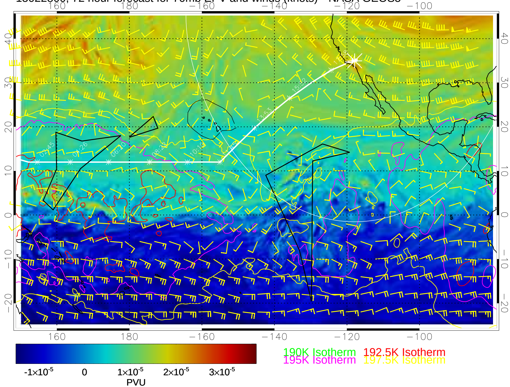
15022800, 72 hour forecast for 70mb EPV and winds (knots)-- NASA GEOS5
