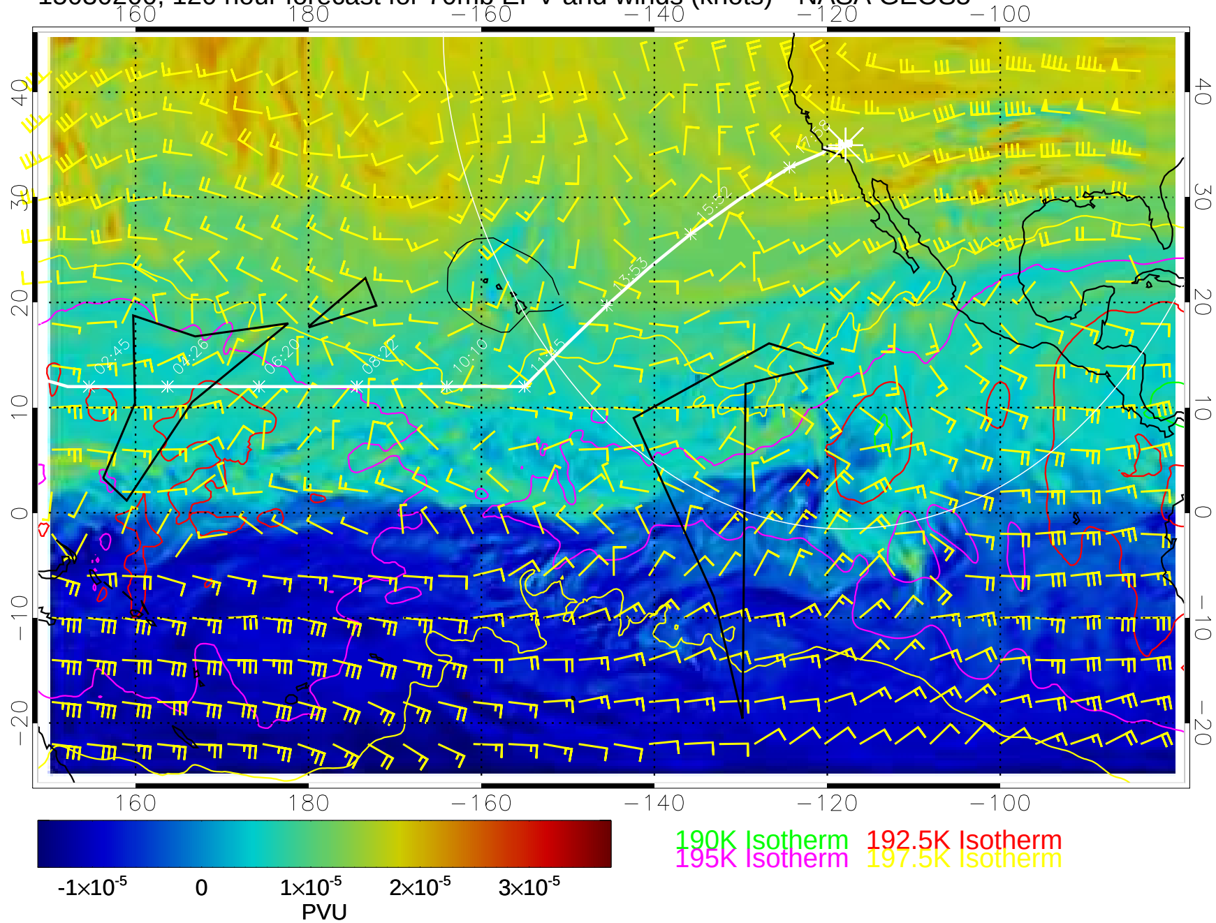
15030200, 120 hour forecast for 70mb EPV and winds (knots)-- NASA GEOS5
