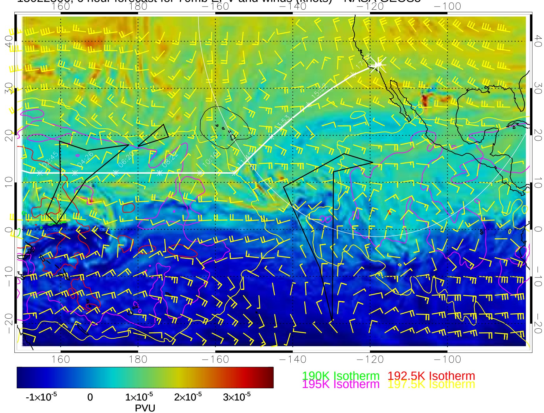
15022506, 6 hour forecast for 70mb EPV and winds (knots)-- NASA GEOS5
