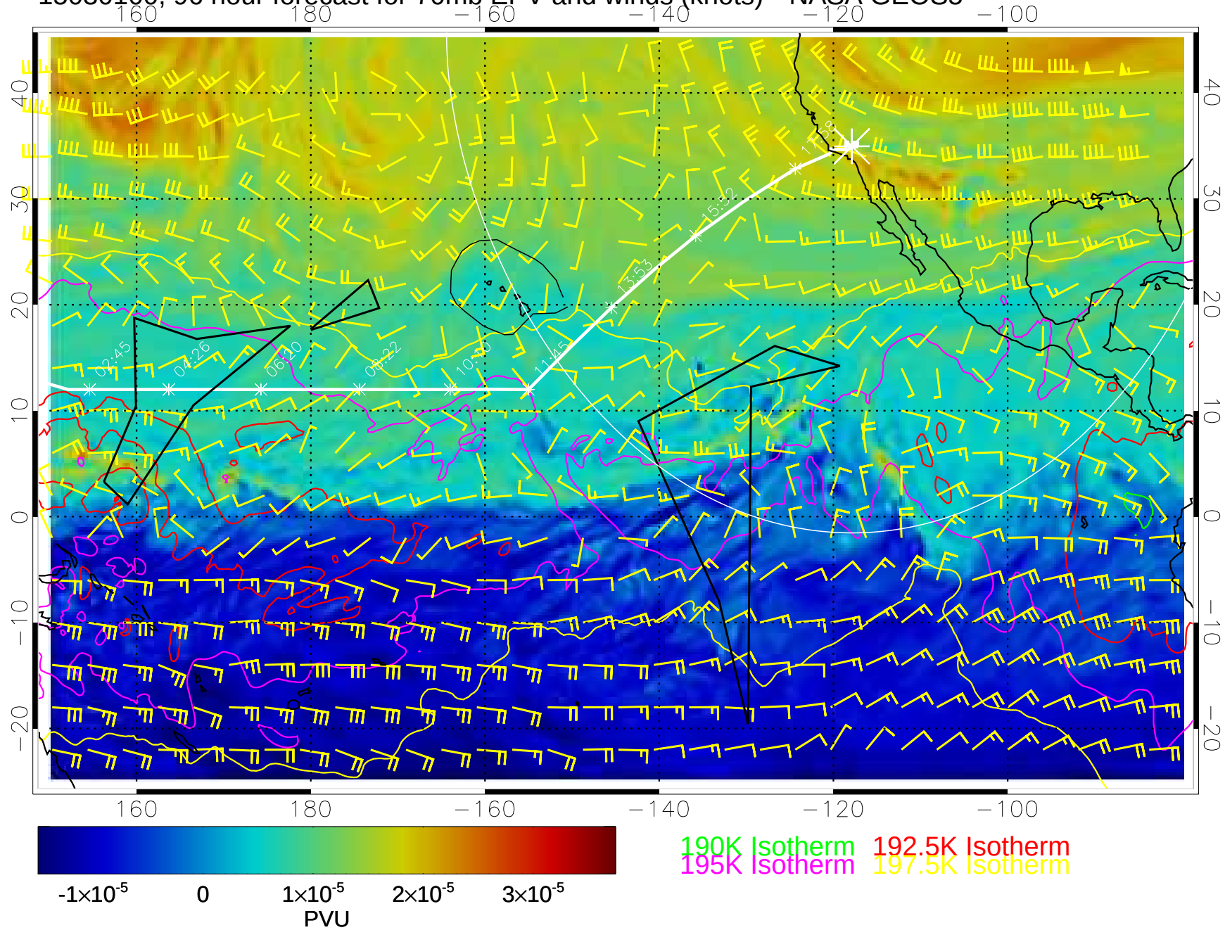
15030100, 96 hour forecast for 70mb EPV and winds (knots)-- NASA GEOS5
