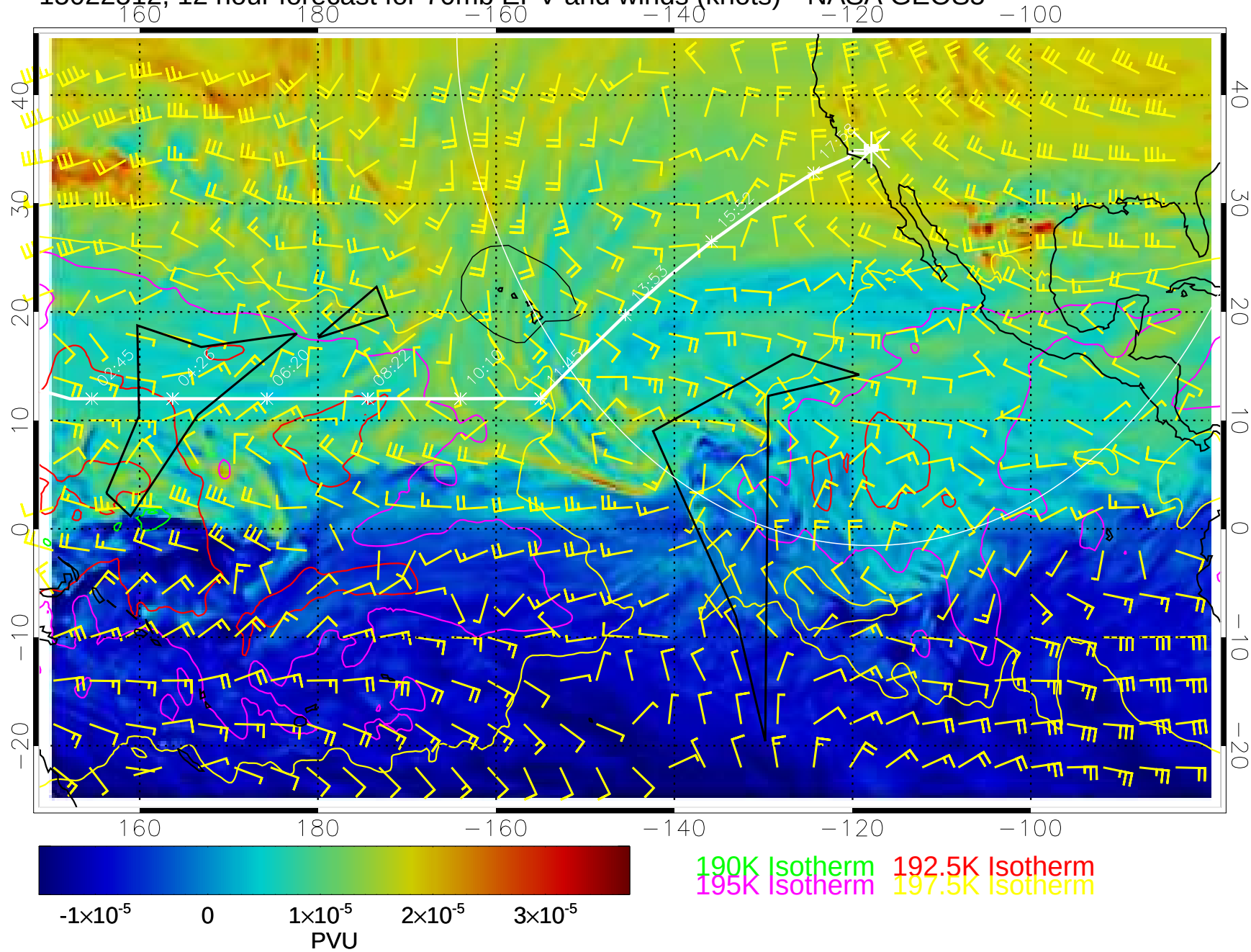
15022512, 12 hour forecast for 70mb EPV and winds (knots)-- NASA GEOS5
