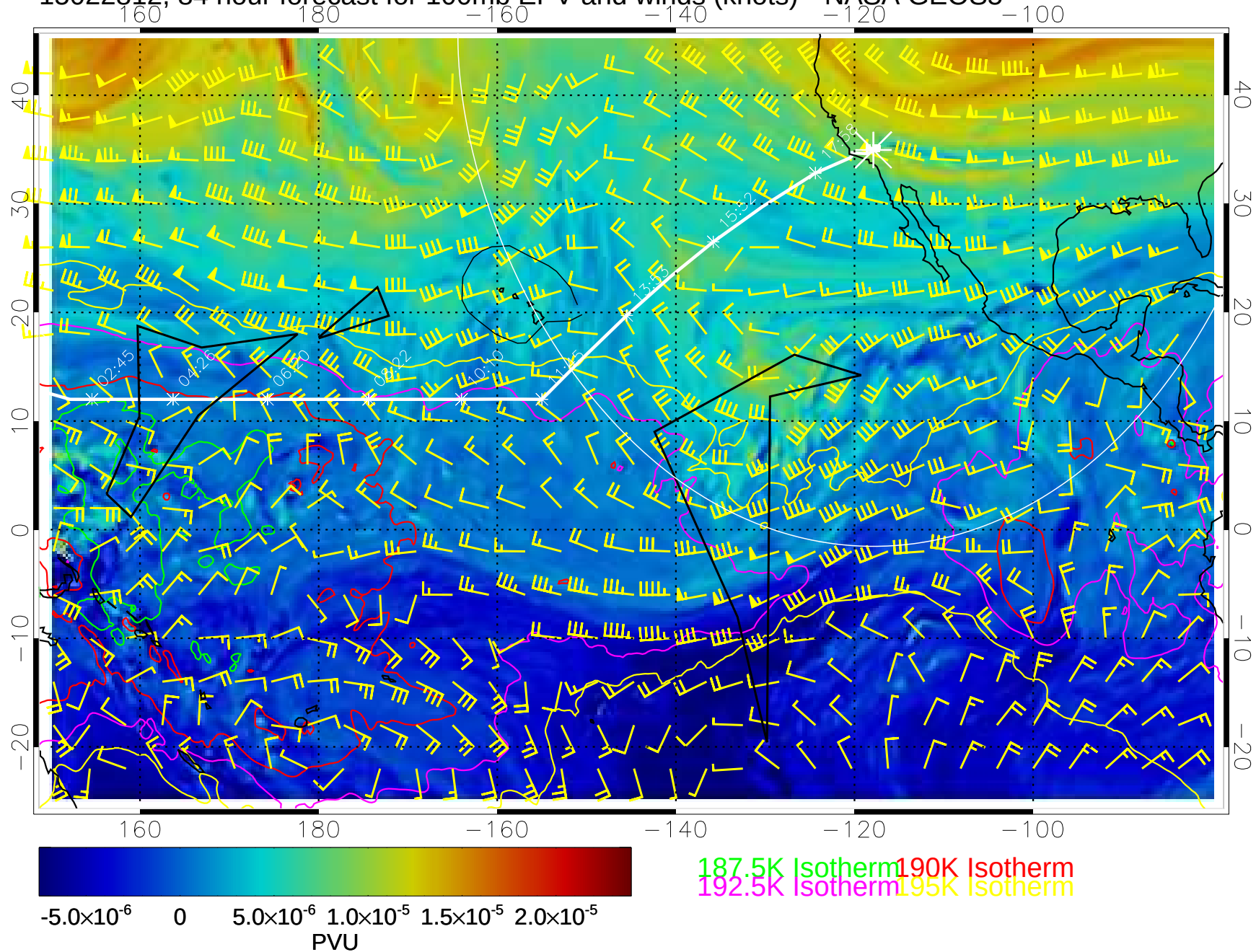
15022812, 84 hour forecast for 100mb EPV and winds (knots)-- NASA GEOS5
