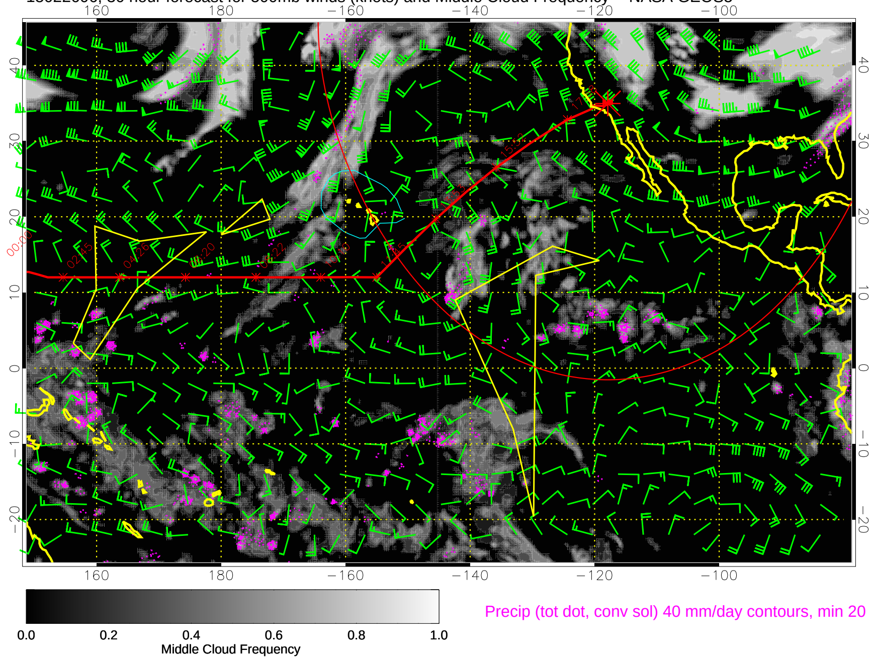
15022606, 30 hour forecast for 500mb winds (knots) and Middle Cloud Frequency -- NASA GEOS5
