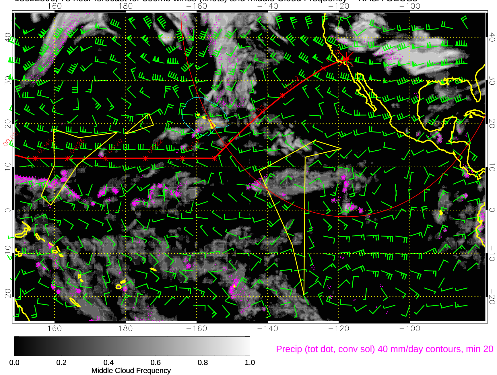
15022806, 78 hour forecast for 500mb winds (knots) and Middle Cloud Frequency -- NASA GEOS5
