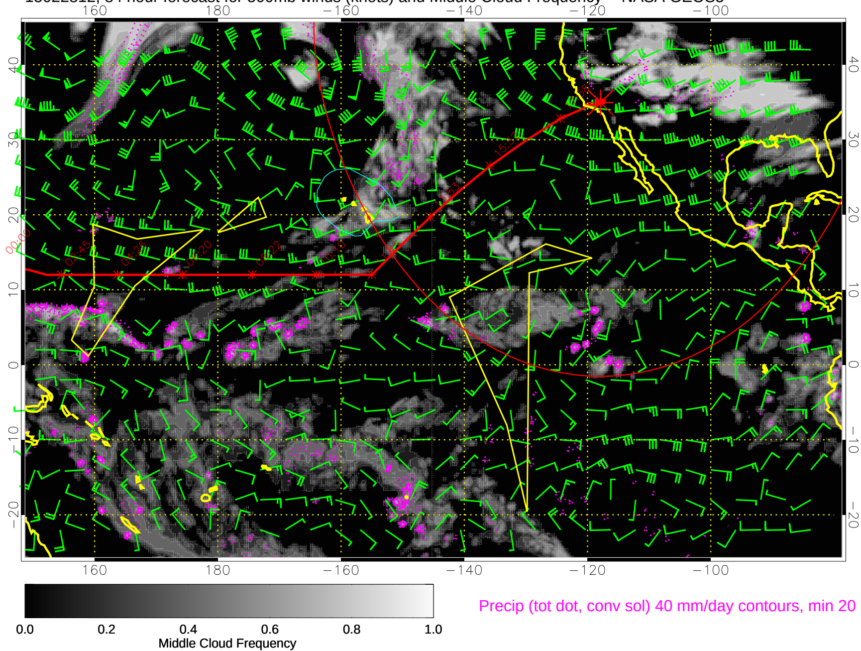
15022812, 84 hour forecast for 500mb winds (knots) and Middle Cloud Frequency -- NASA GEOS5
