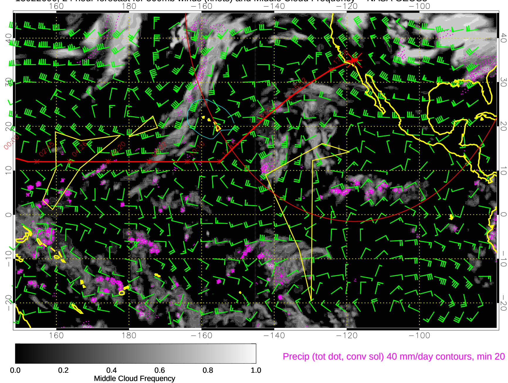
15022600, 24 hour forecast for 500mb winds (knots) and Middle Cloud Frequency -- NASA GEOS5
