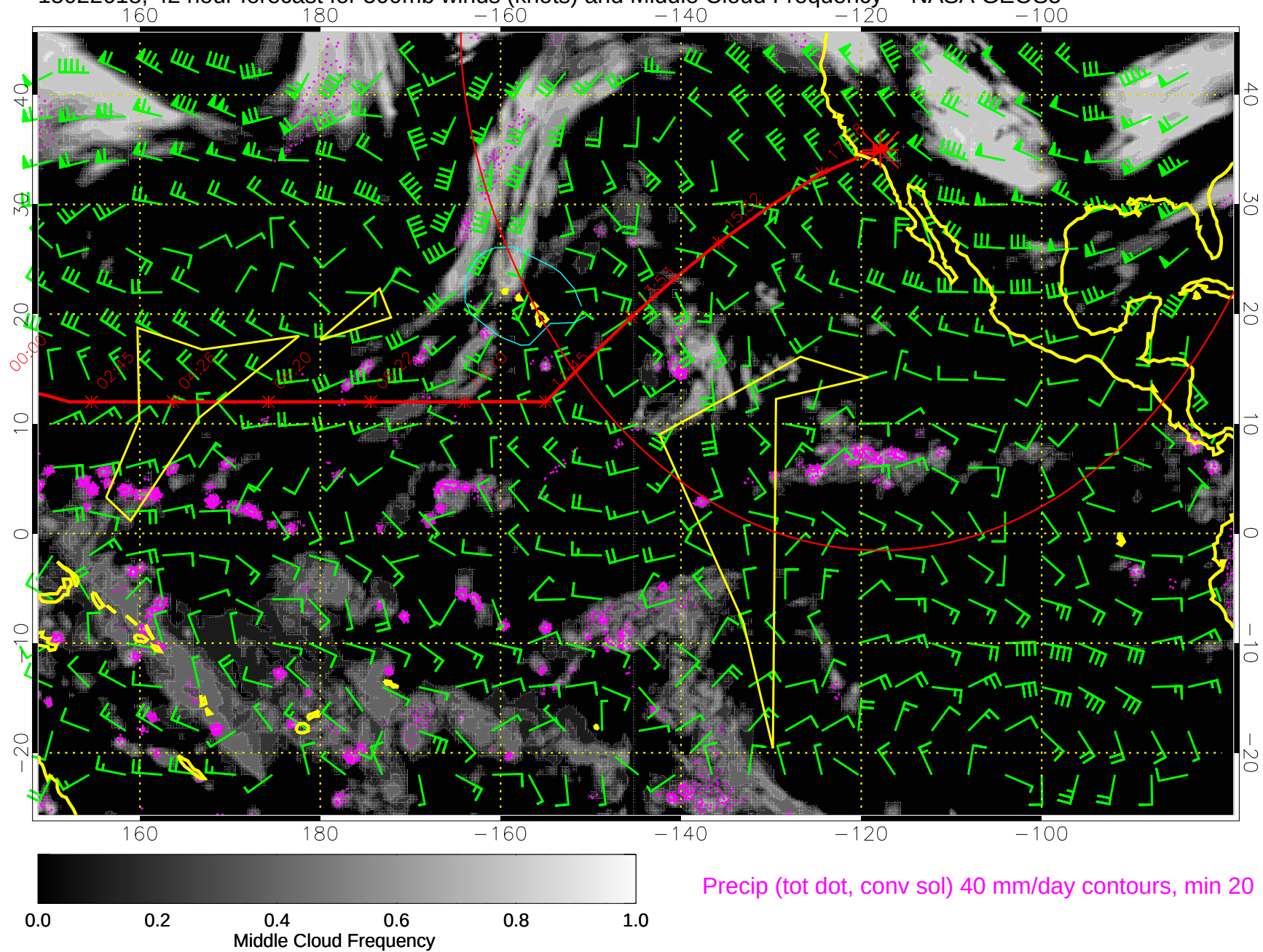
15022618, 42 hour forecast for 500mb winds (knots) and Middle Cloud Frequency -- NASA GEOS5
