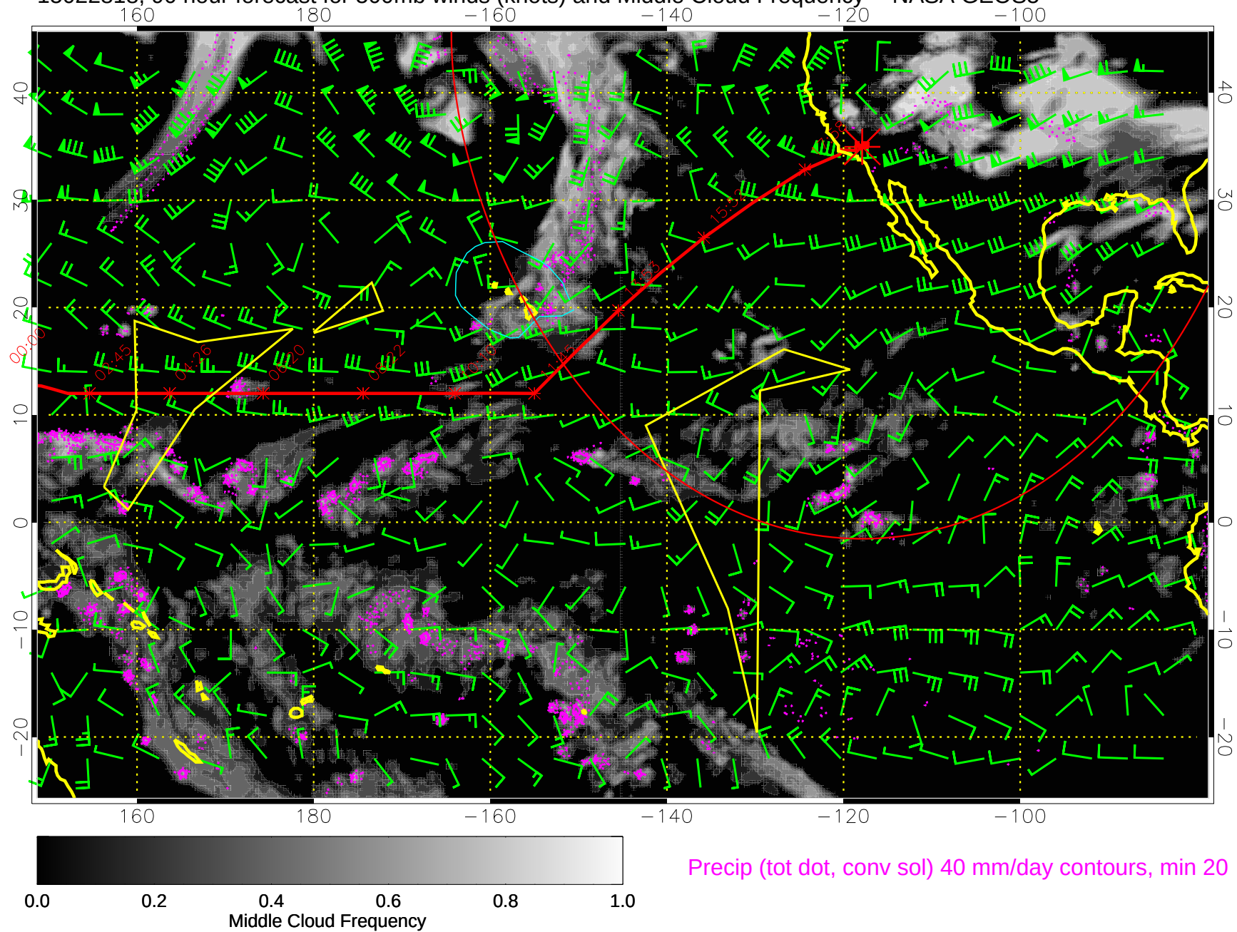
15022818, 90 hour forecast for 500mb winds (knots) and Middle Cloud Frequency -- NASA GEOS5
