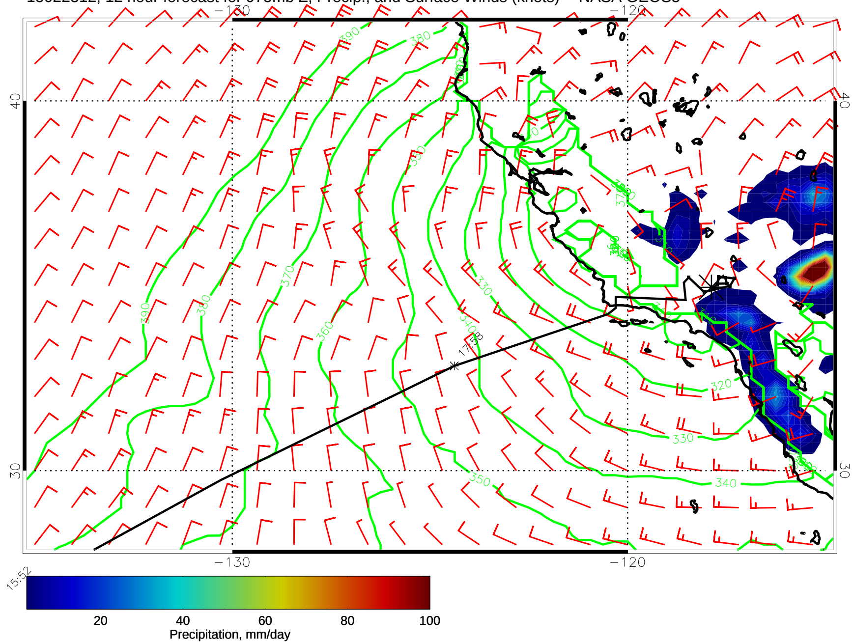
15022312, 12 hour forecast for 975mb Z, Precip., and Surface Winds (knots) -- NASA GEOS5
