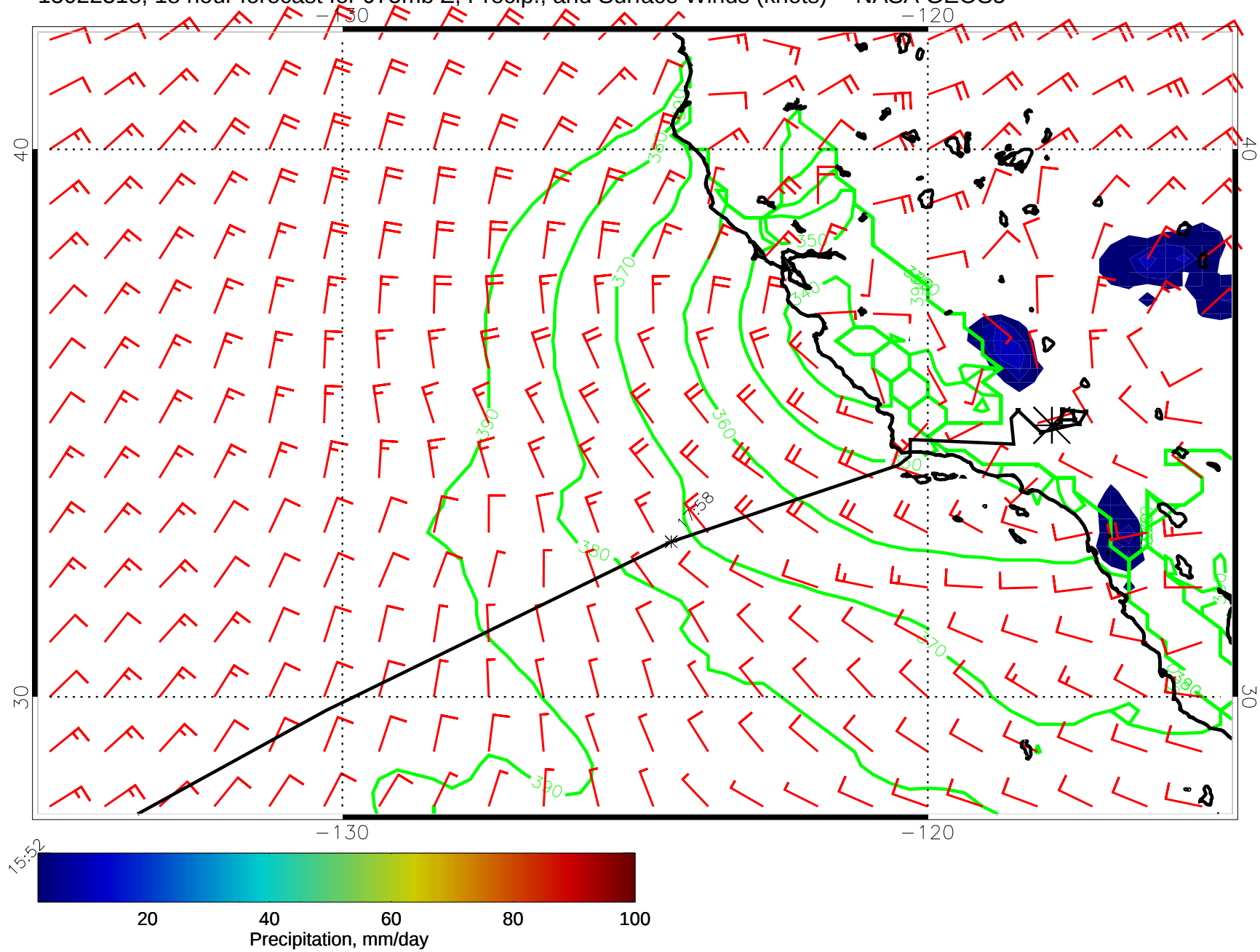
15022318, 18 hour forecast for 975mb Z, Precip., and Surface Winds (knots) -- NASA GEOS5
