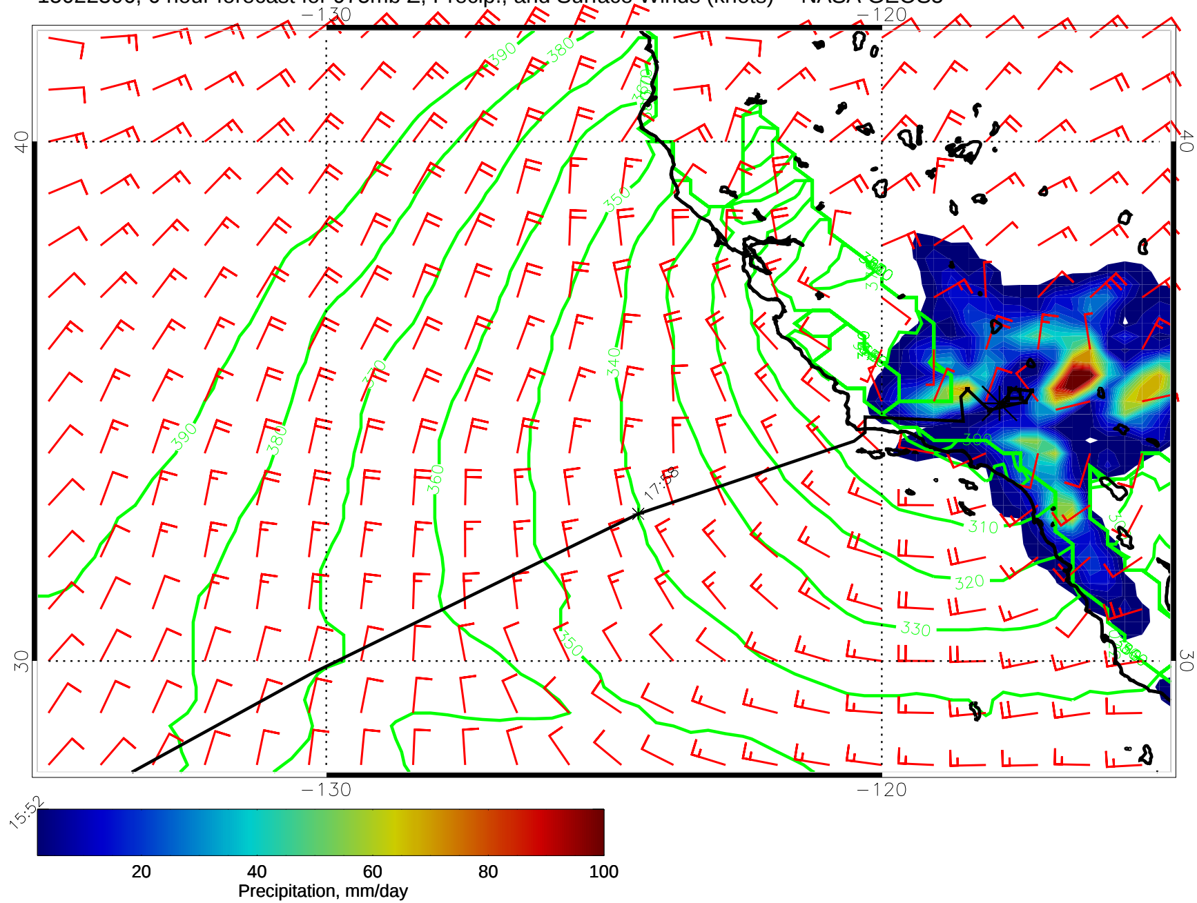
15022306, 6 hour forecast for 975mb Z, Precip., and Surface Winds (knots) -- NASA GEOS5
