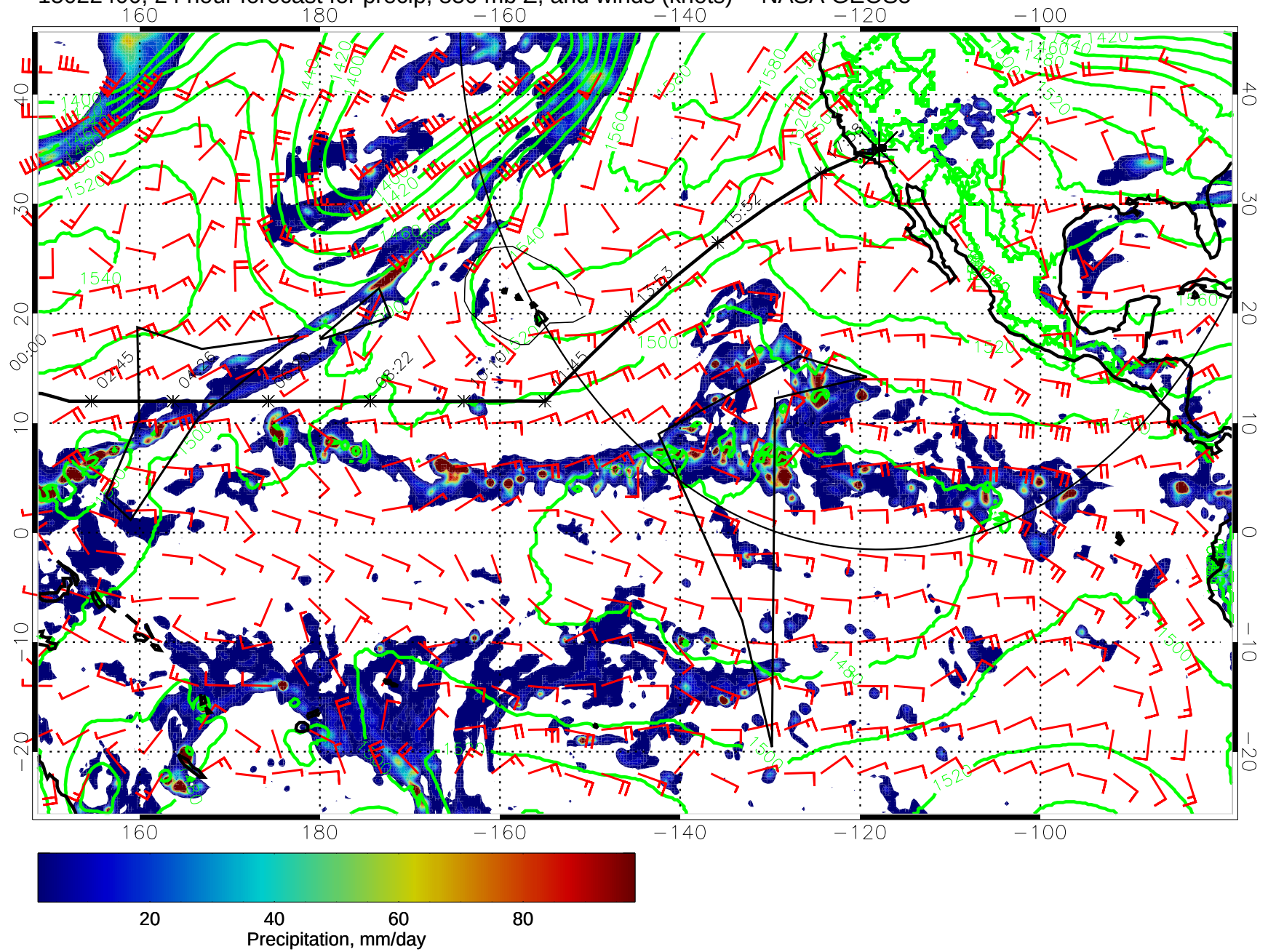
15022400, 24 hour forecast for precip, 850 mb Z, and winds (knots) -- NASA GEOS5
