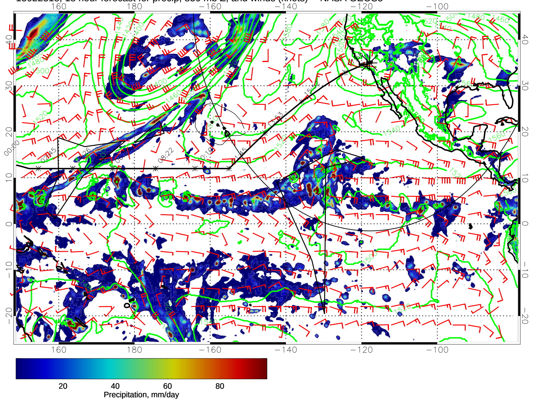
15022318, 18 hour forecast for precip, 850 mb Z, and winds (knots) -- NASA GEOS5
