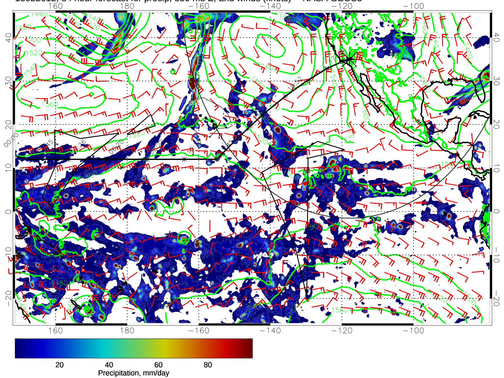
15022612, 84 hour forecast for precip, 850 mb Z, and winds (knots) -- NASA GEOS5
