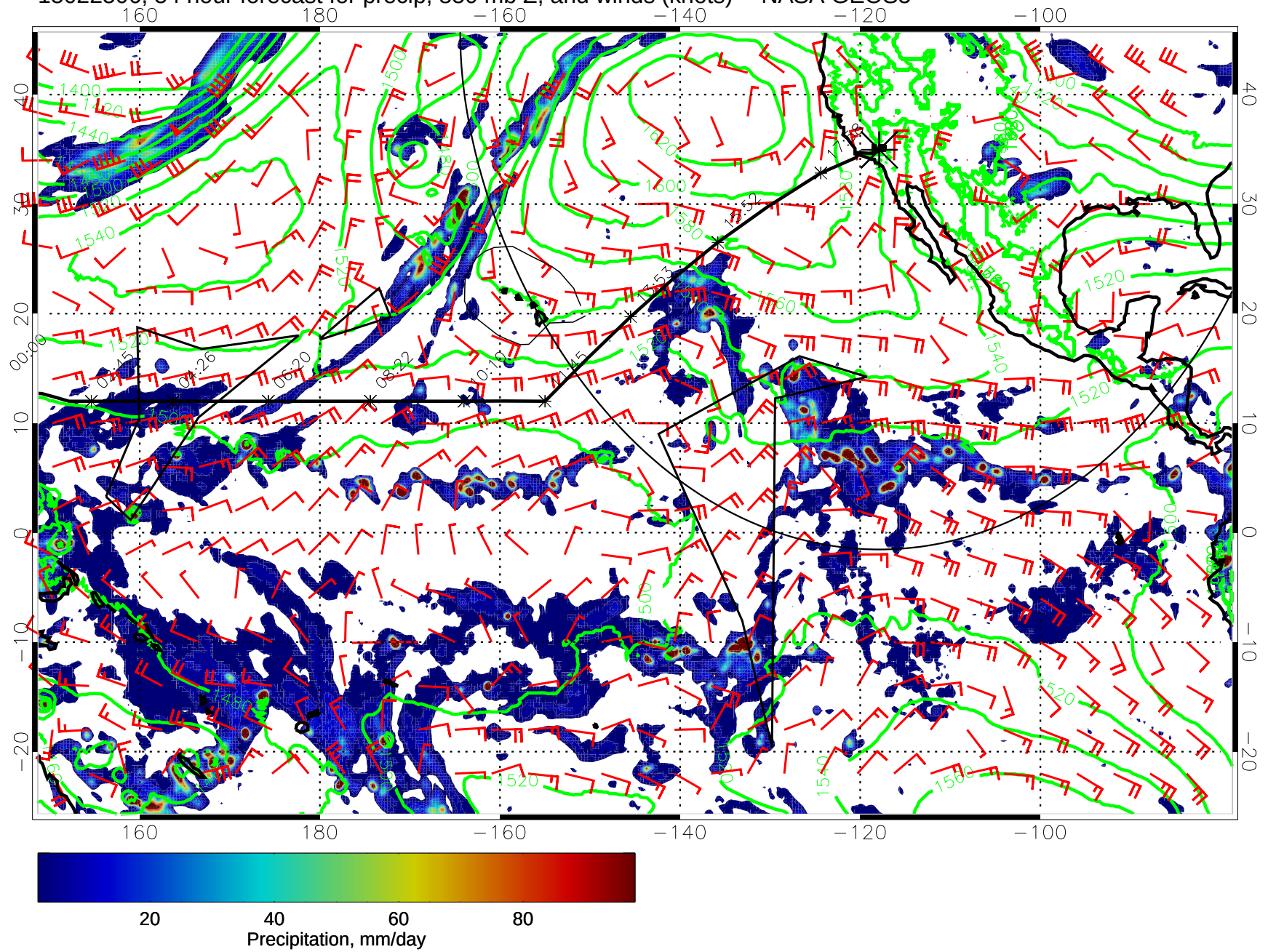
15022506, 54 hour forecast for precip, 850 mb Z, and winds (knots) -- NASA GEOS5
