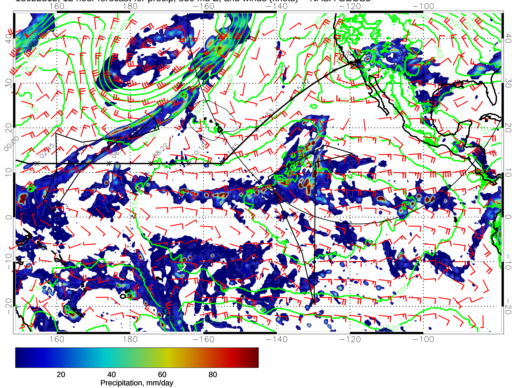
15022312, 12 hour forecast for precip, 850 mb Z, and winds (knots) -- NASA GEOS5
