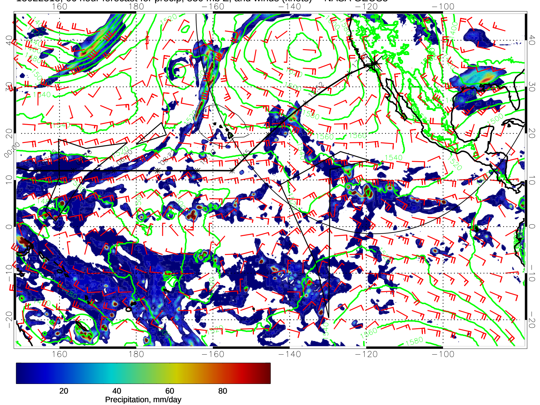
15022518, 66 hour forecast for precip, 850 mb Z, and winds (knots) -- NASA GEOS5
