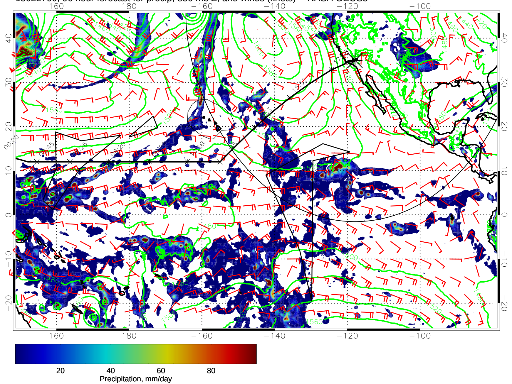
15022700, 96 hour forecast for precip, 850 mb Z, and winds (knots) -- NASA GEOS5
