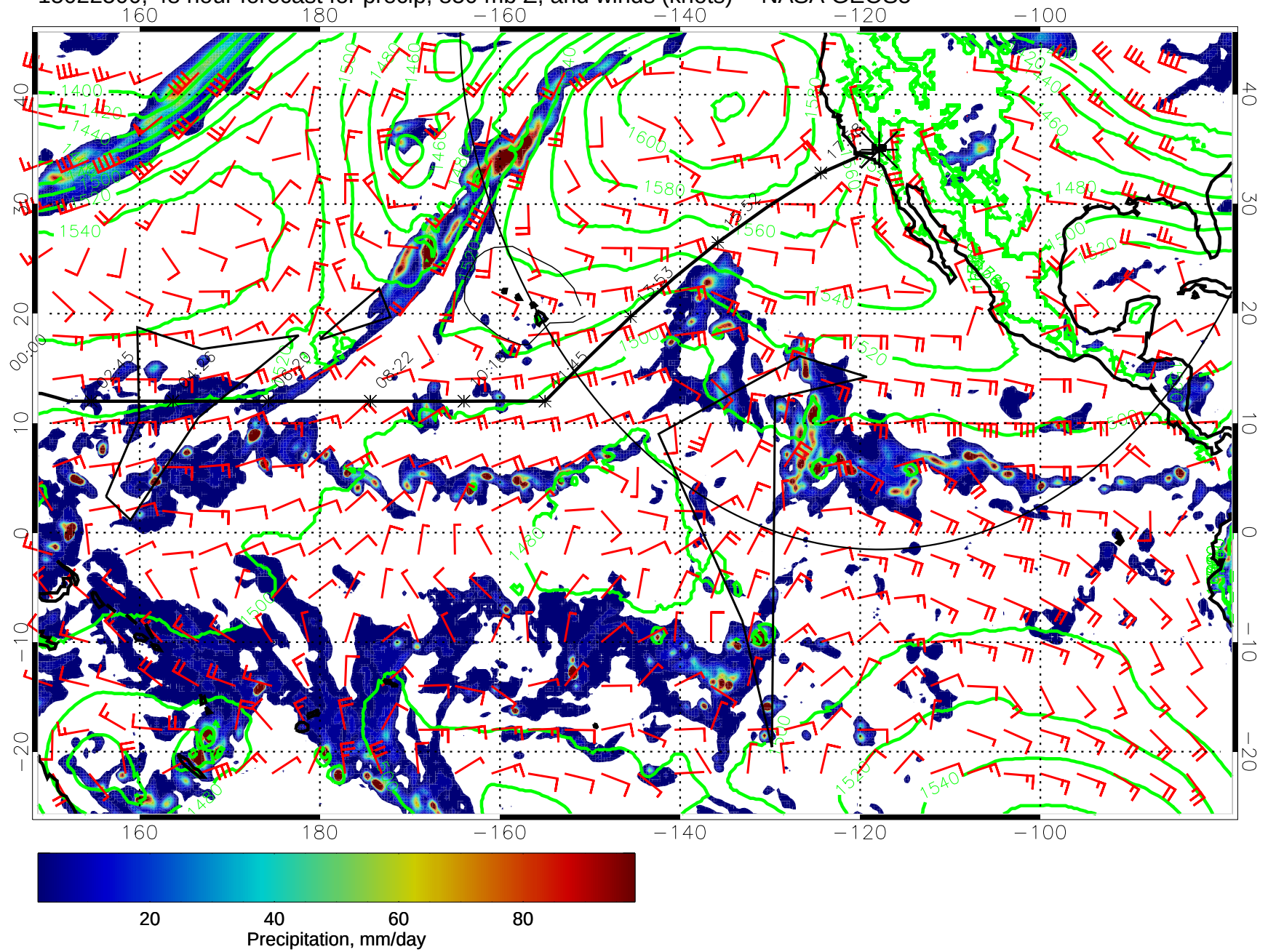
15022500, 48 hour forecast for precip, 850 mb Z, and winds (knots) -- NASA GEOS5
