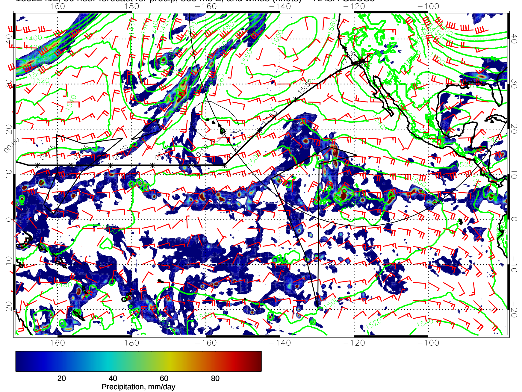
15022412, 36 hour forecast for precip, 850 mb Z, and winds (knots) -- NASA GEOS5
