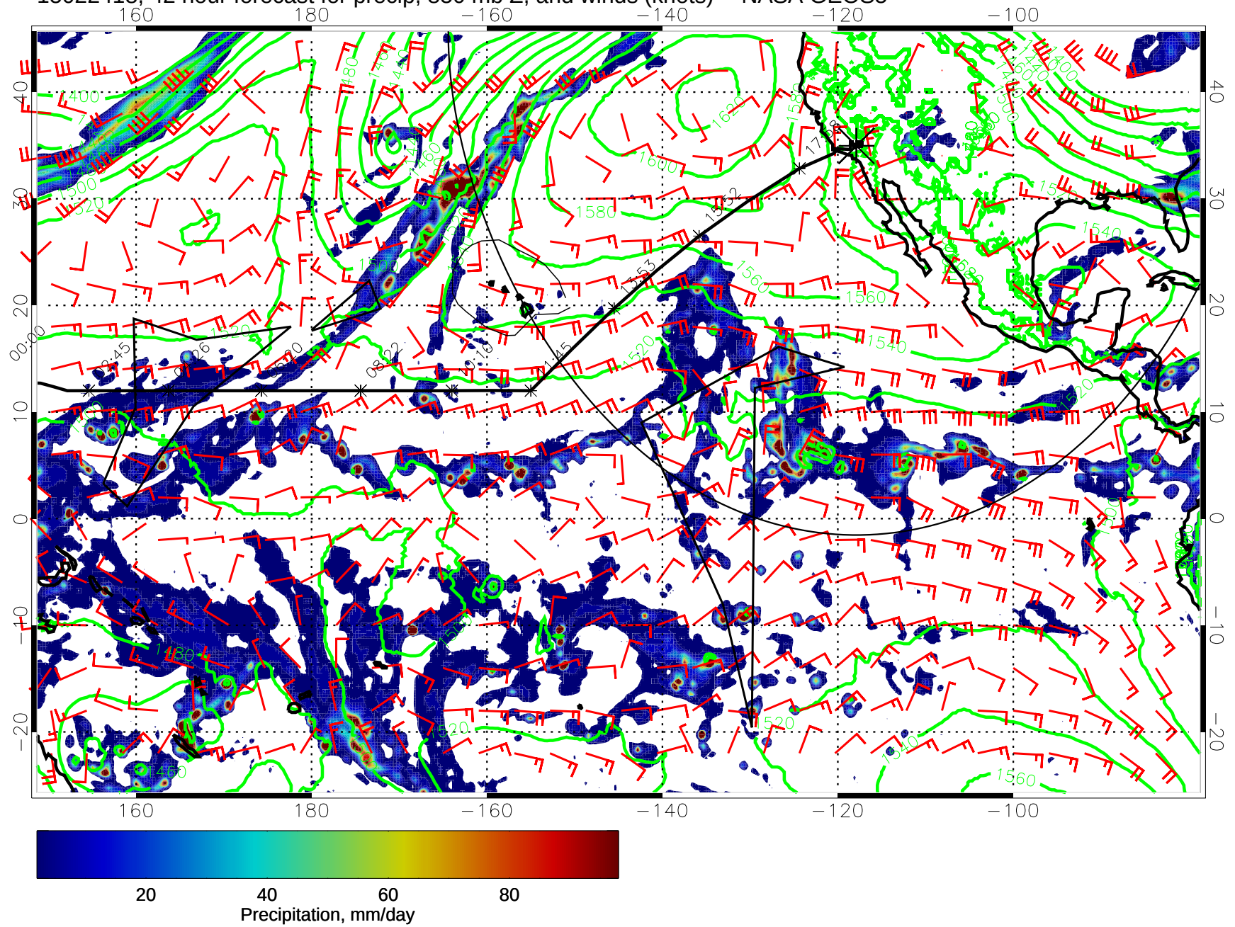
15022418, 42 hour forecast for precip, 850 mb Z, and winds (knots) -- NASA GEOS5
