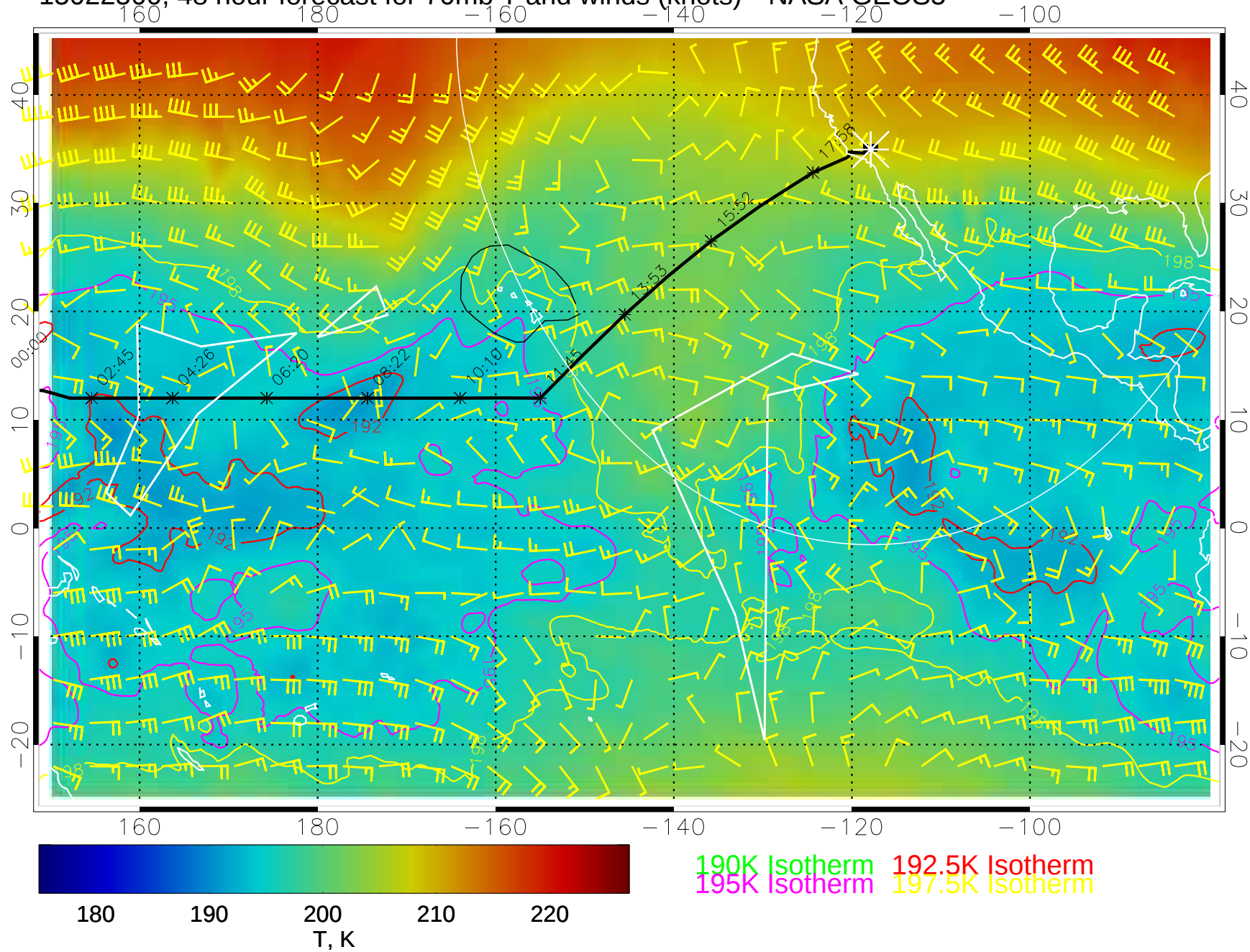
15022500, 48 hour forecast for 70mb T and winds (knots)-- NASA GEOS5
