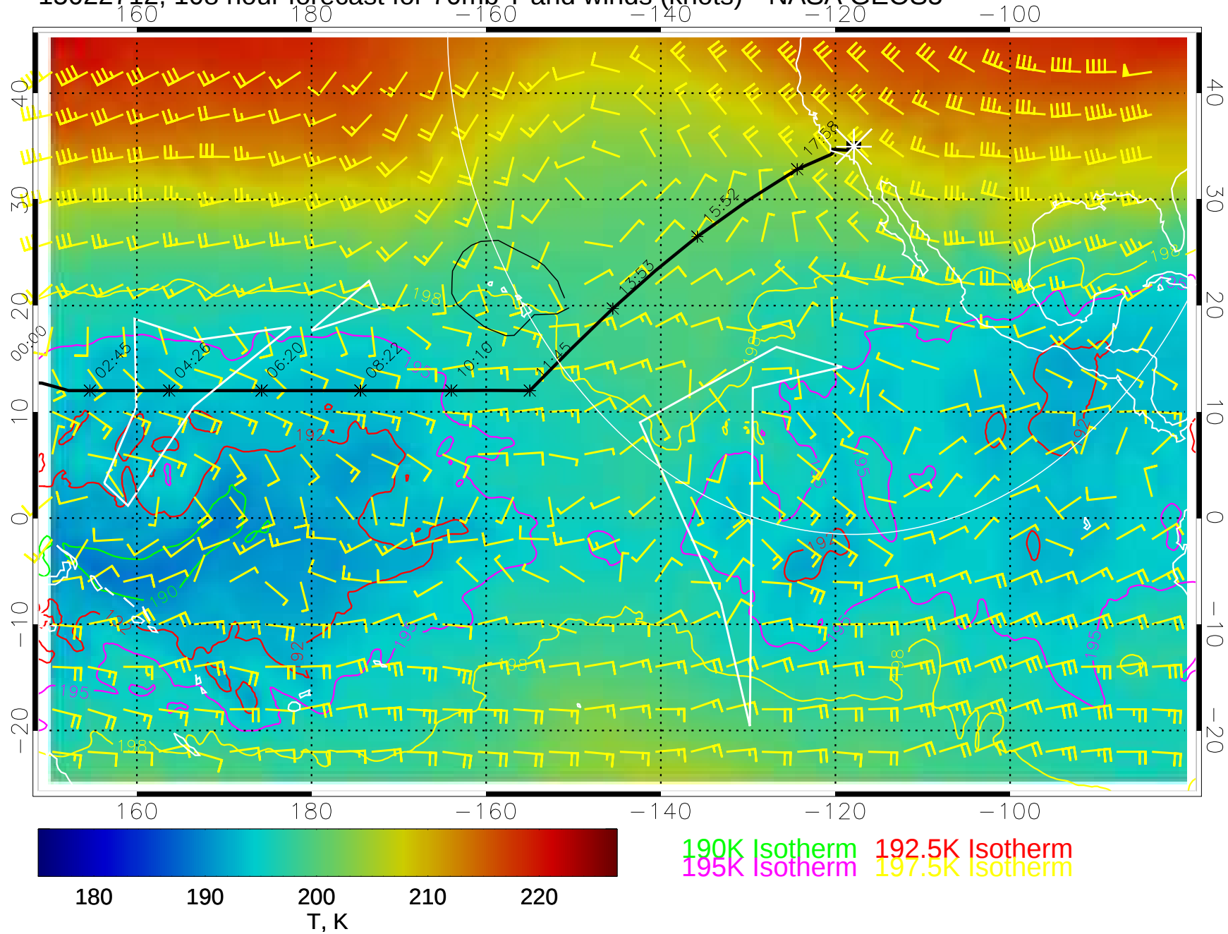
15022712, 108 hour forecast for 70mb T and winds (knots)-- NASA GEOS5
