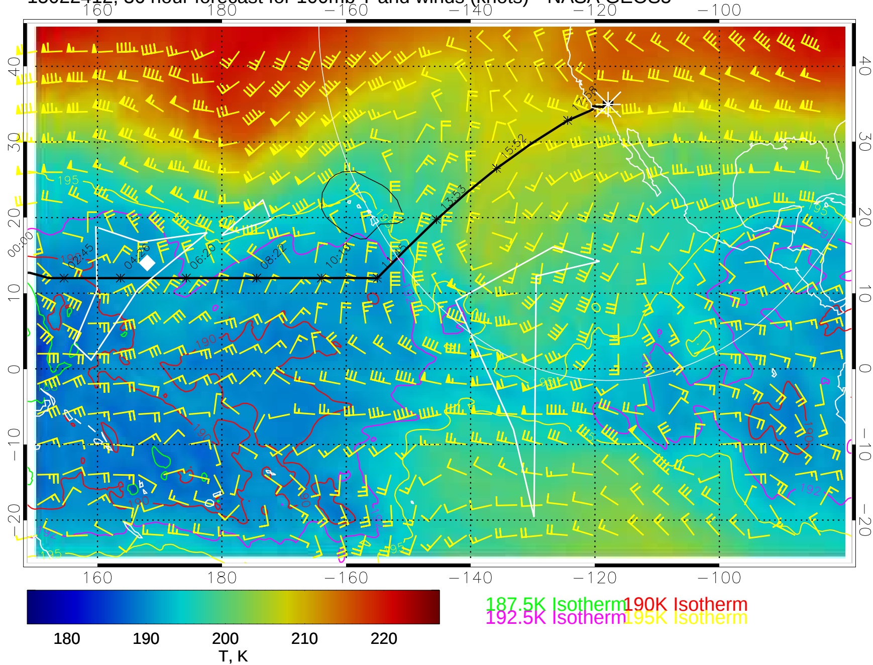
15022412, 36 hour forecast for 100mb T and winds (knots)-- NASA GEOS5
