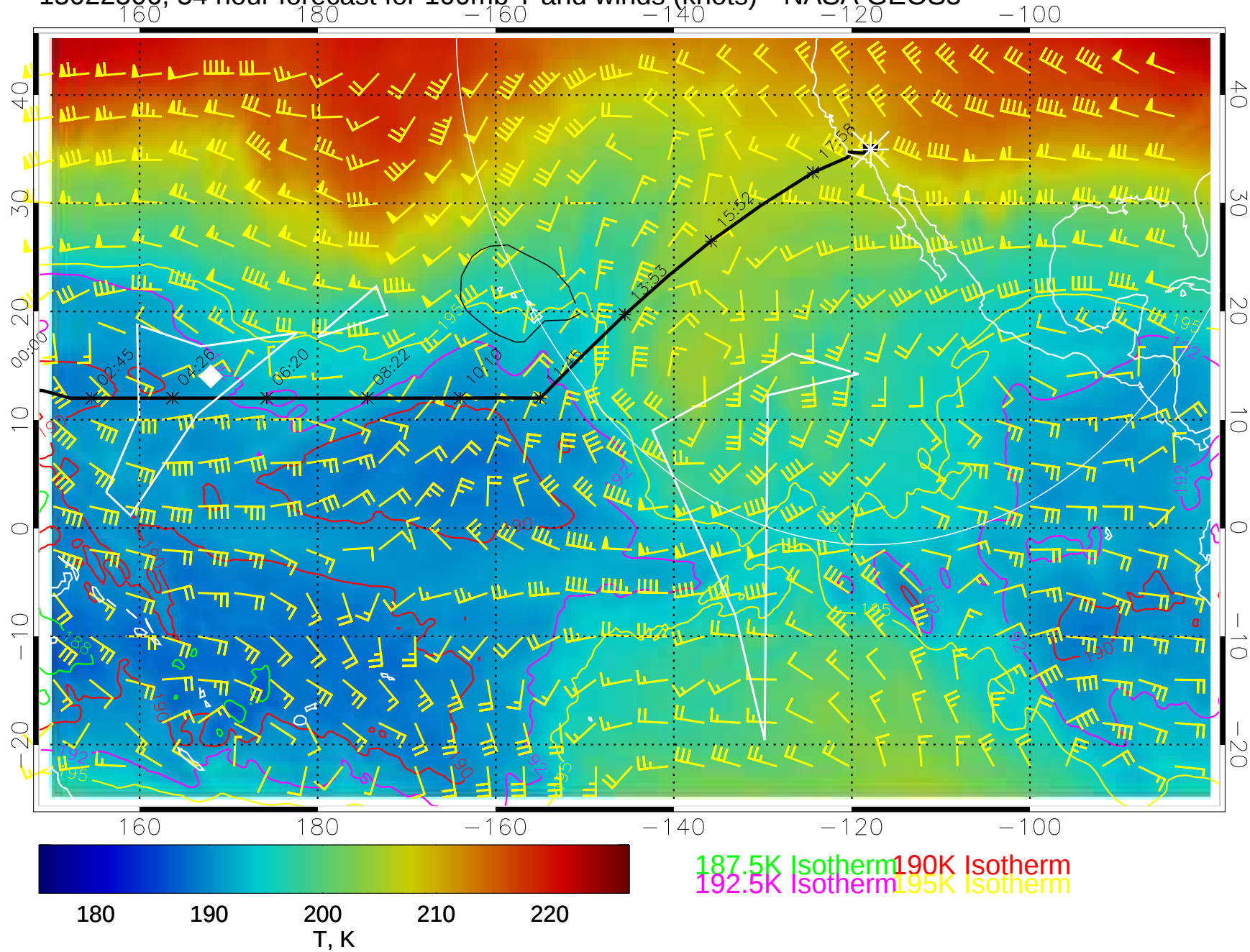
15022506, 54 hour forecast for 100mb T and winds (knots)-- NASA GEOS5
