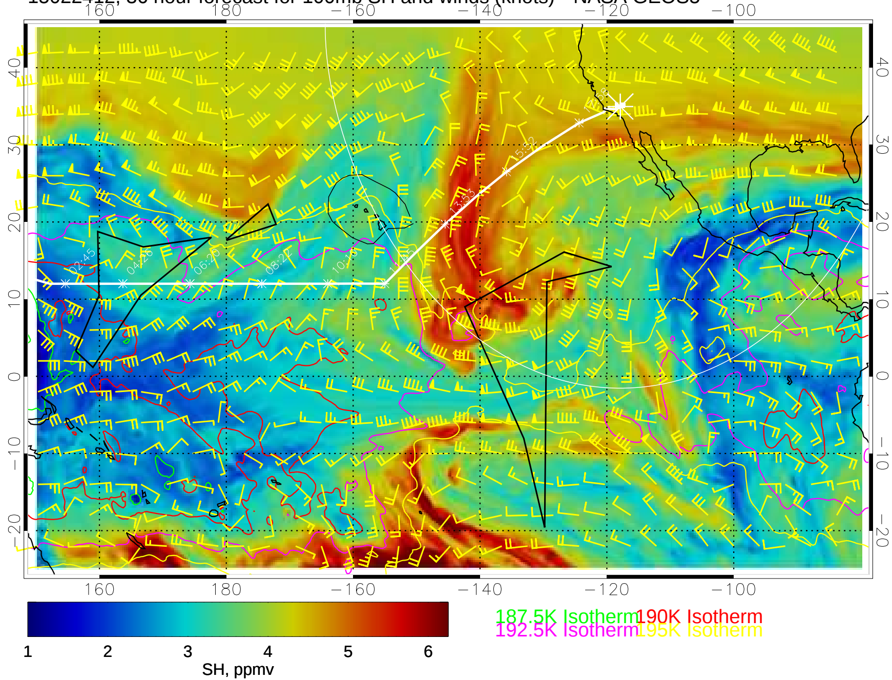
15022412, 36 hour forecast for 100mb SH and winds (knots)-- NASA GEOS5
