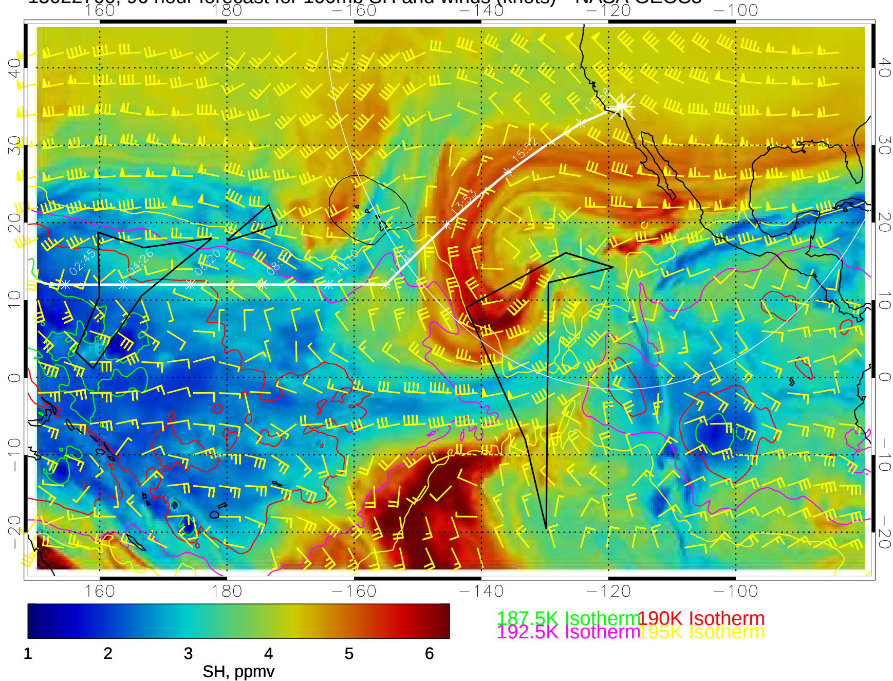
15022700, 96 hour forecast for 100mb SH and winds (knots)-- NASA GEOS5
