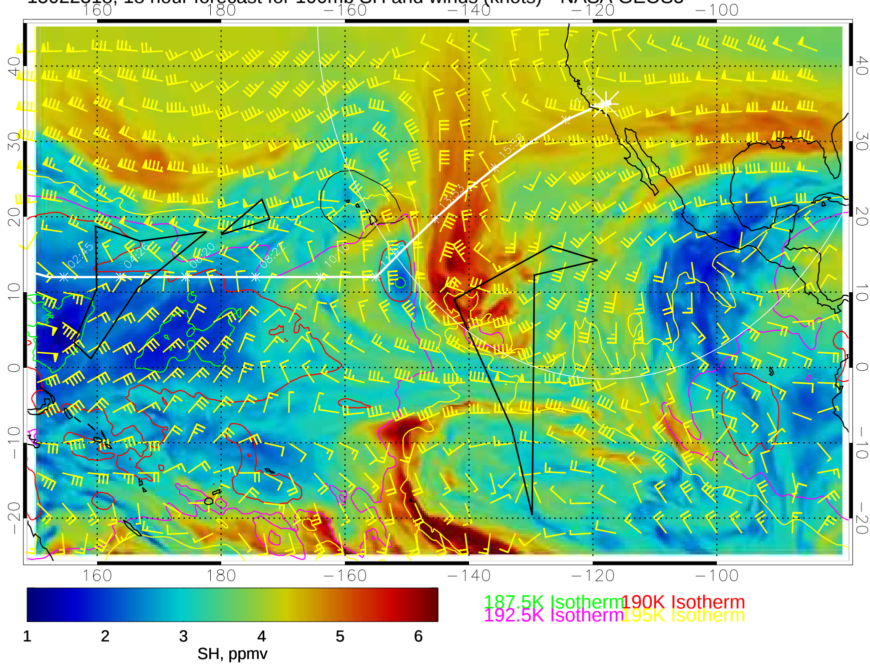
15022318, 18 hour forecast for 100mb SH and winds (knots)-- NASA GEOS5
