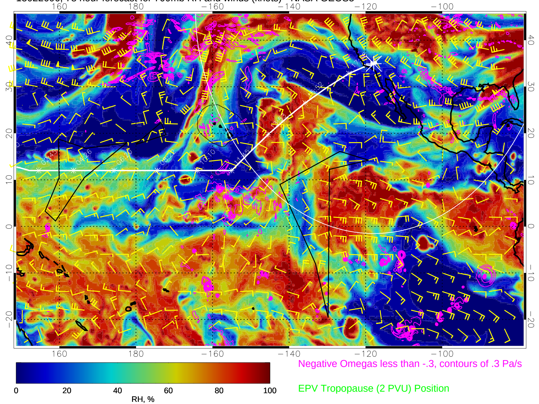
15022606, 78 hour forecast for 700mb RH and winds (knots) - NASA GEOS5
