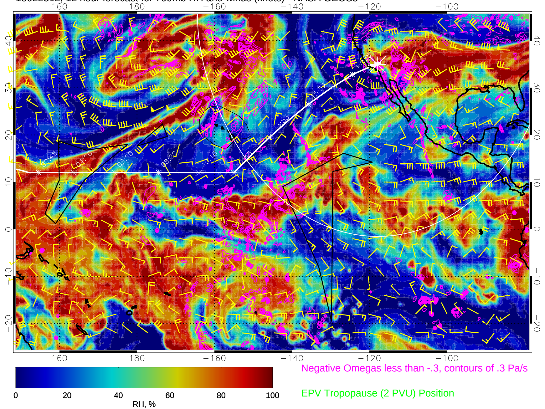
15022312, 12 hour forecast for 700mb RH and winds (knots) - NASA GEOS5
