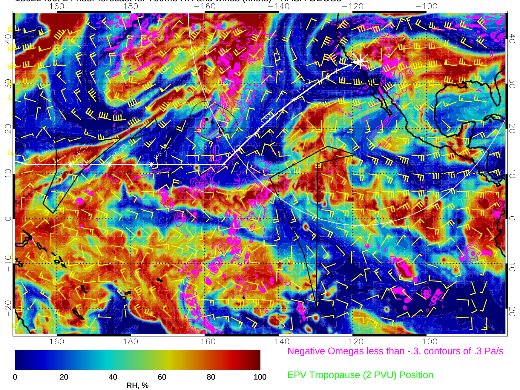
15022400, 24 hour forecast for 700mb RH and winds (knots) - NASA GEOS5
