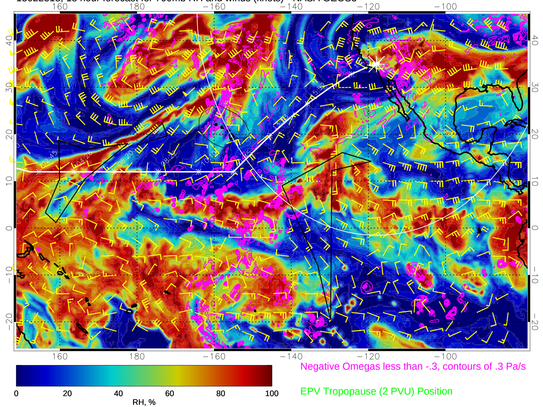
15022318, 18 hour forecast for 700mb RH and winds (knots) - NASA GEOS5
