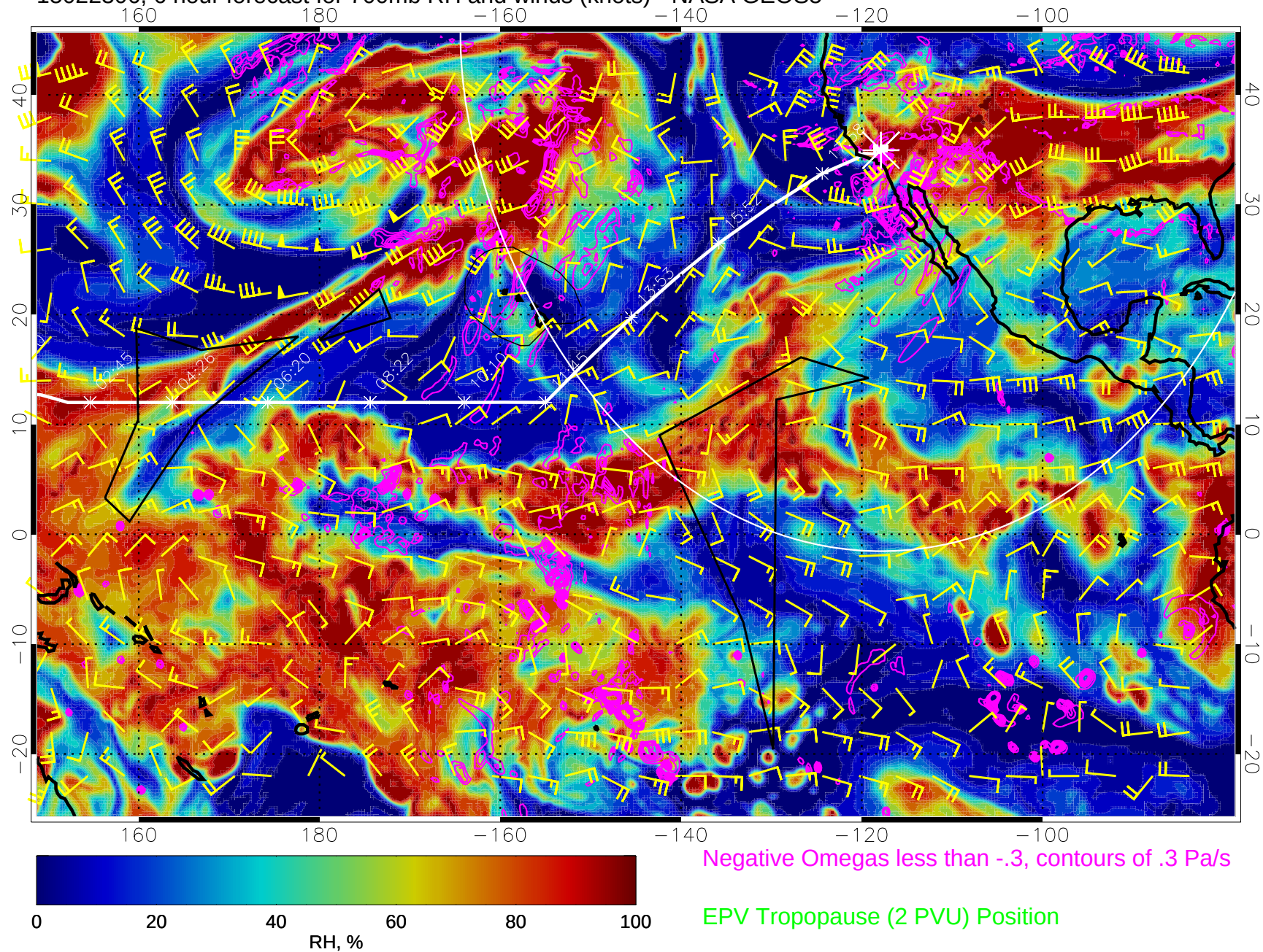
15022306, 6 hour forecast for 700mb RH and winds (knots) - NASA GEOS5
