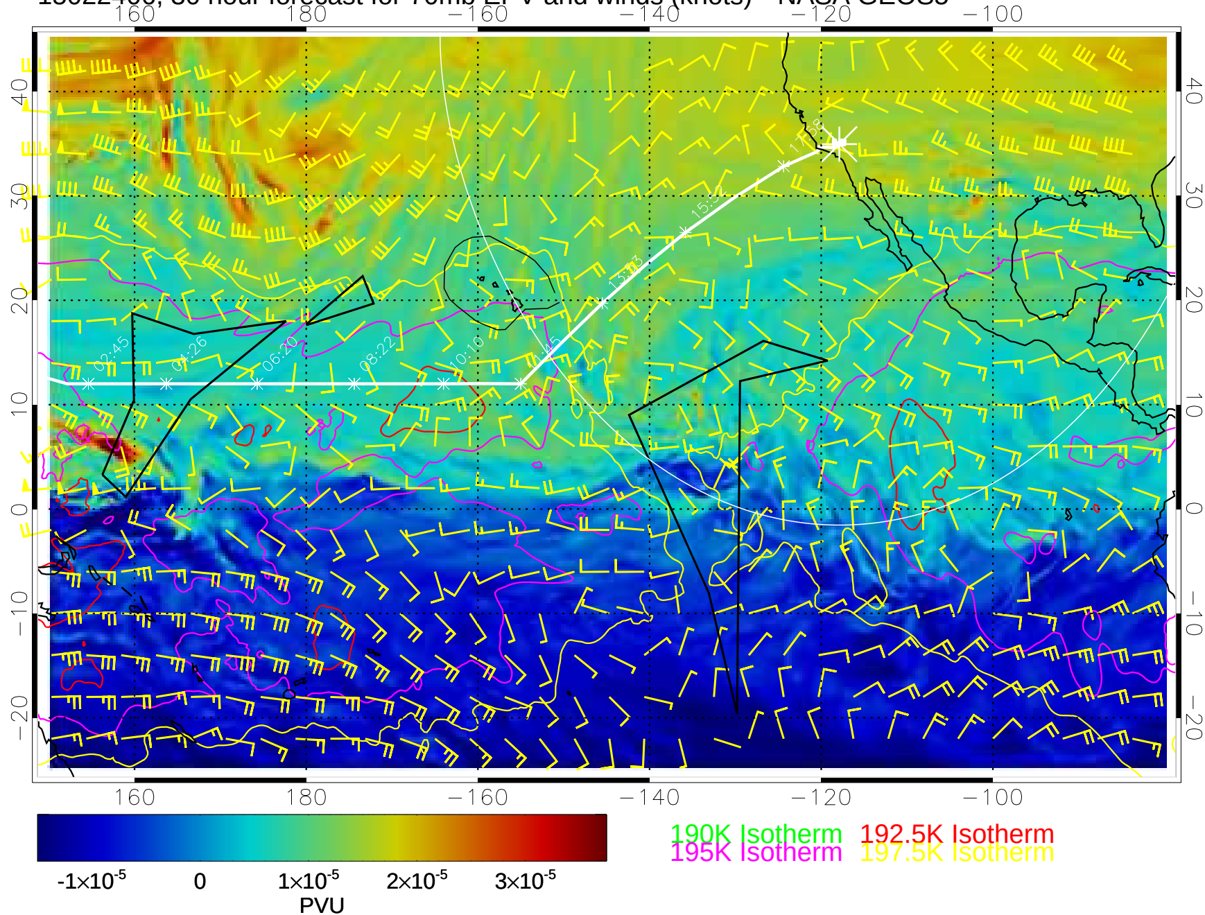
15022406, 30 hour forecast for 70mb EPV and winds (knots)-- NASA GEOS5
