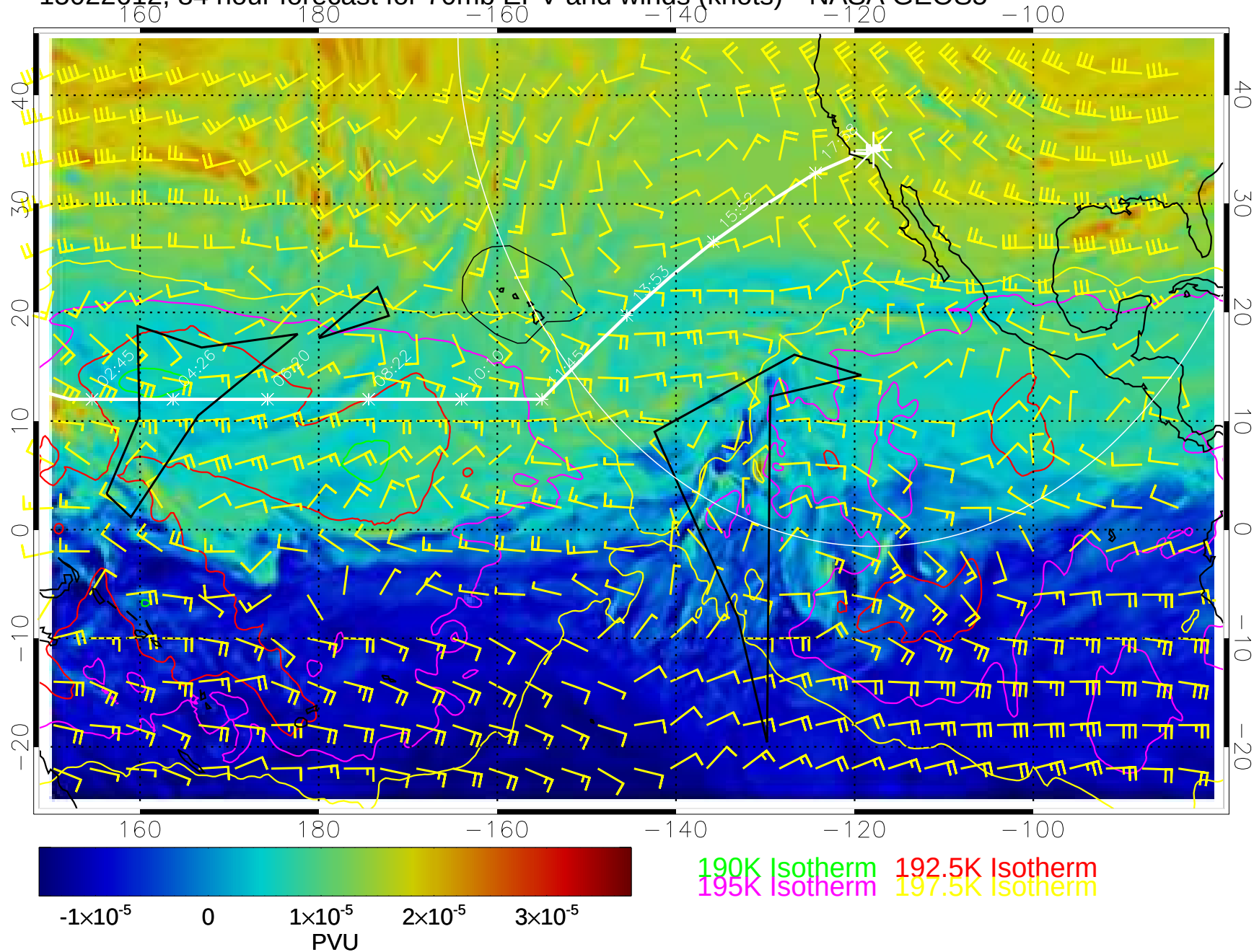
15022612, 84 hour forecast for 70mb EPV and winds (knots)-- NASA GEOS5
