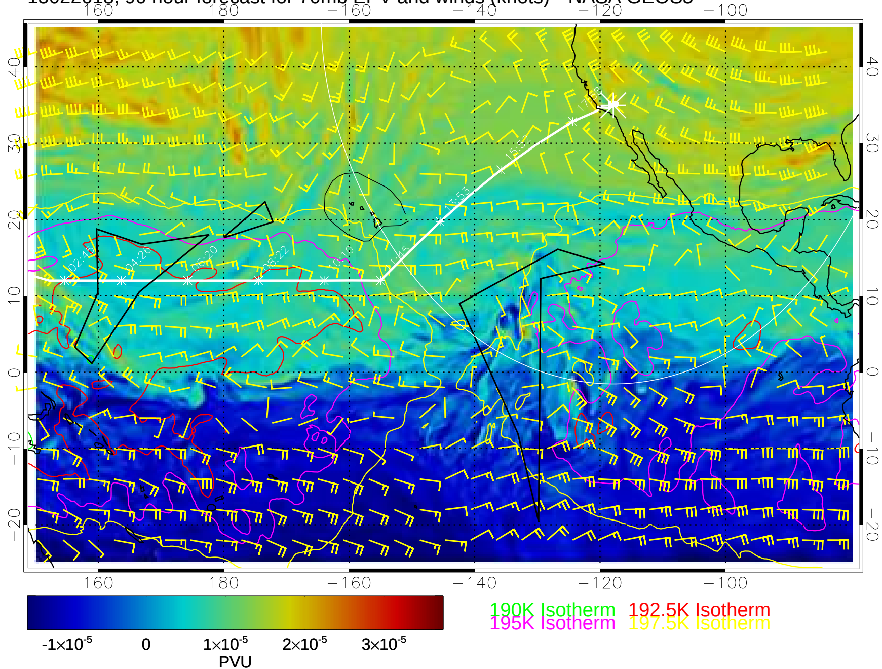
15022618, 90 hour forecast for 70mb EPV and winds (knots)-- NASA GEOS5
