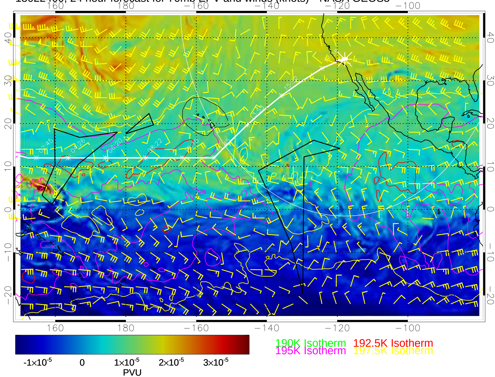
15022400, 24 hour forecast for 70mb EPV and winds (knots)-- NASA GEOS5
