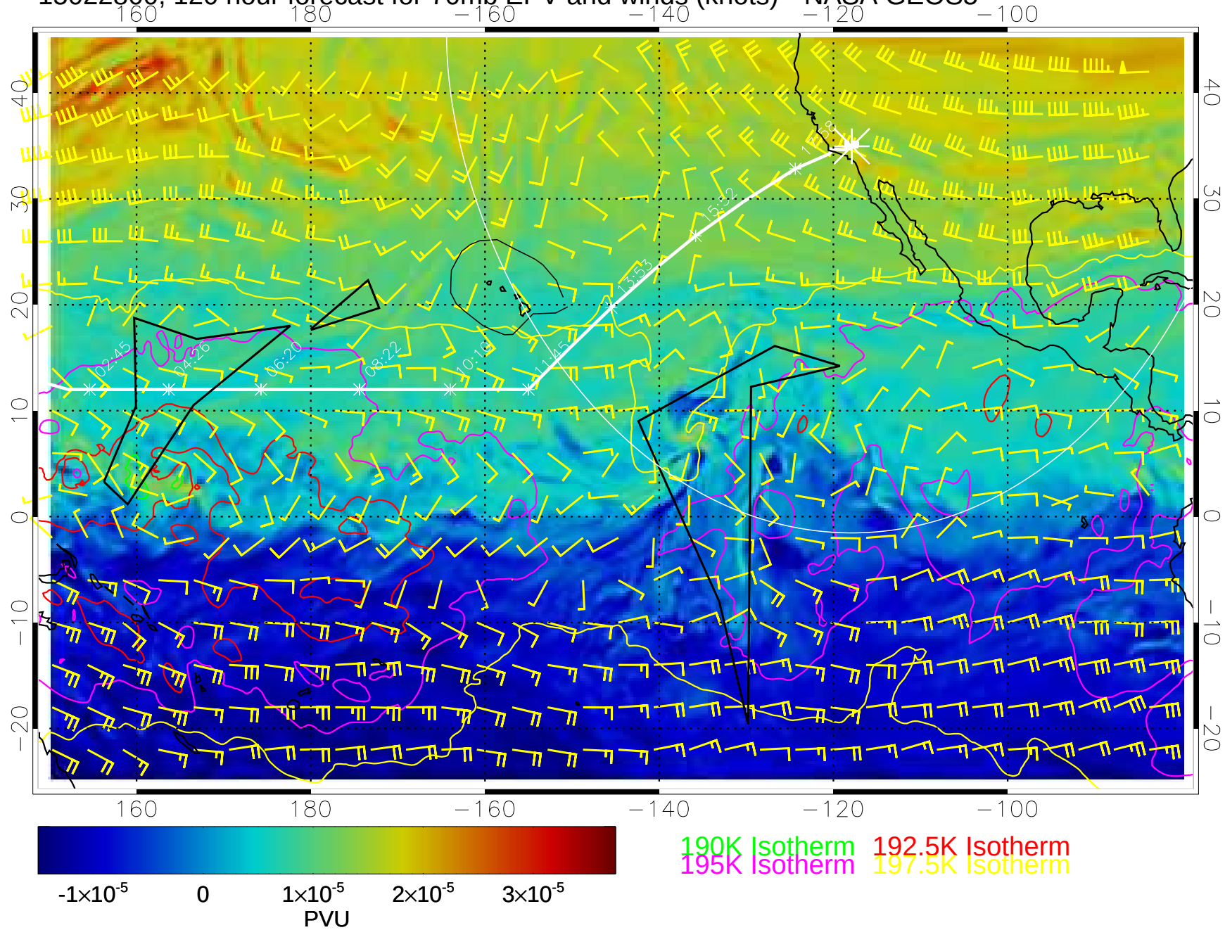
15022800, 120 hour forecast for 70mb EPV and winds (knots)-- NASA GEOS5
