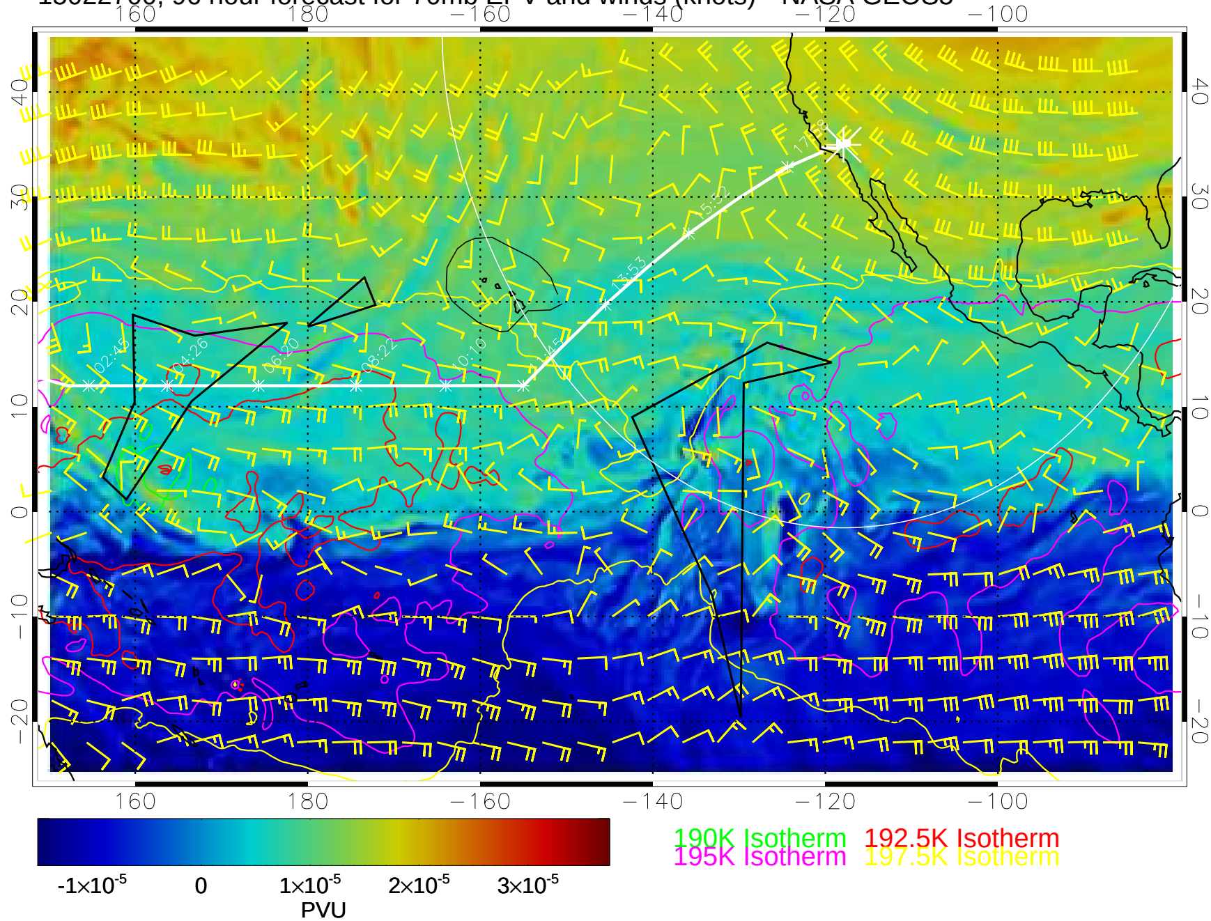
15022700, 96 hour forecast for 70mb EPV and winds (knots)-- NASA GEOS5
