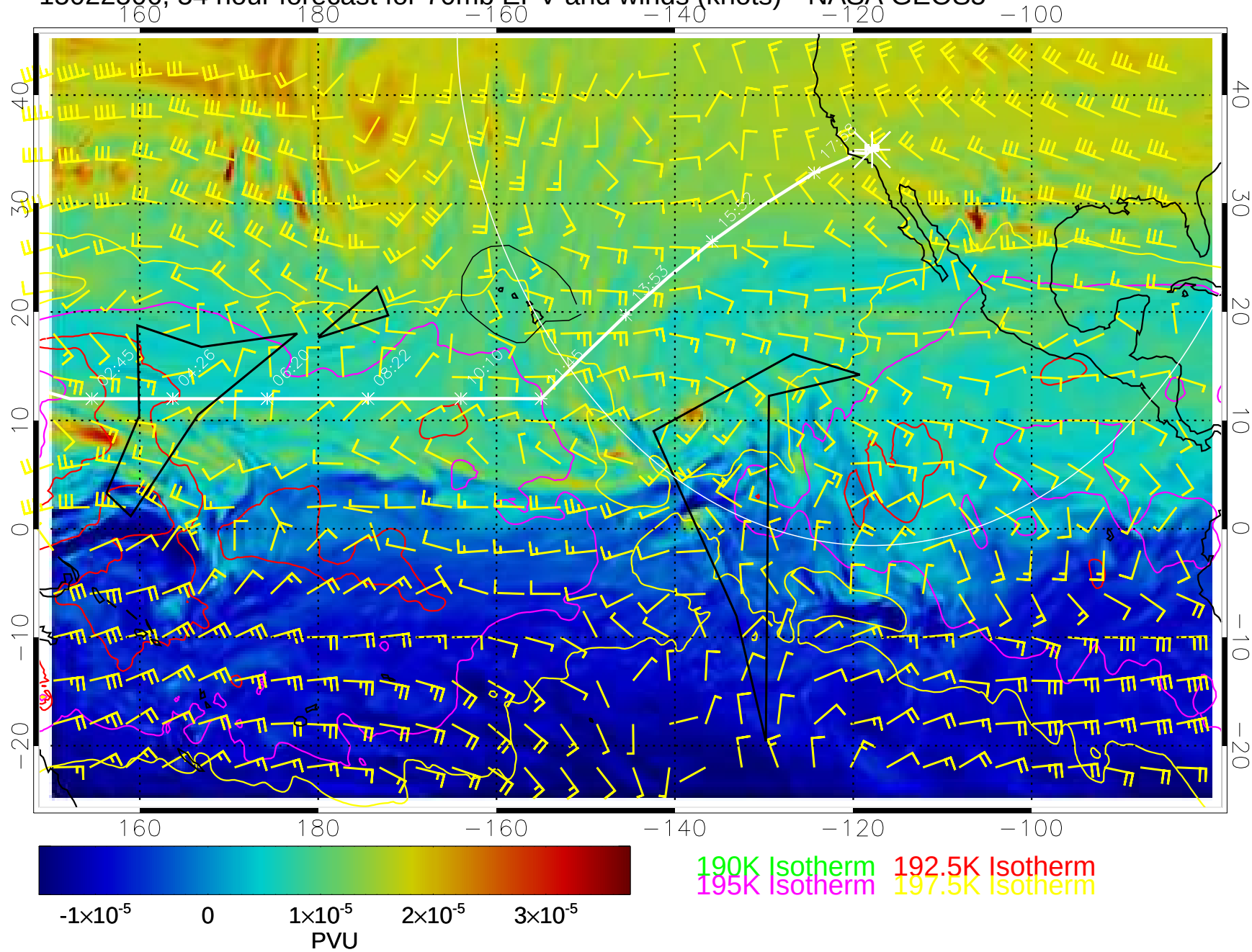
15022506, 54 hour forecast for 70mb EPV and winds (knots)-- NASA GEOS5
