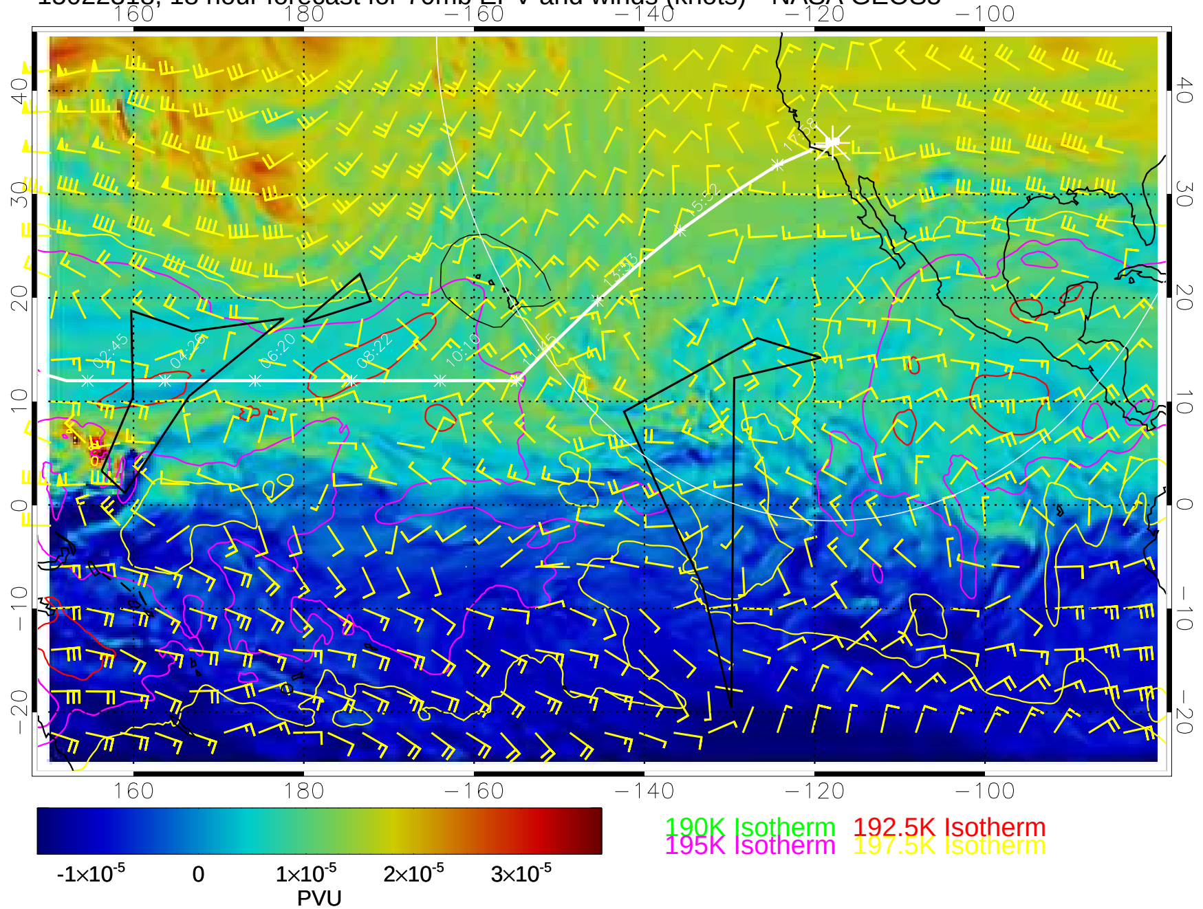
15022318, 18 hour forecast for 70mb EPV and winds (knots)-- NASA GEOS5
