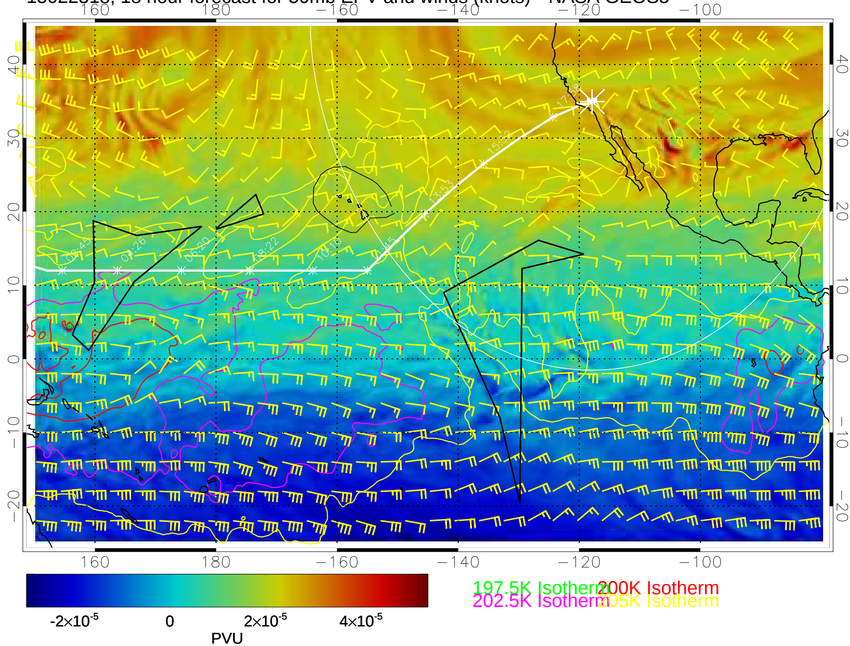
15022318, 18 hour forecast for 50mb EPV and winds (knots)-- NASA GEOS5
