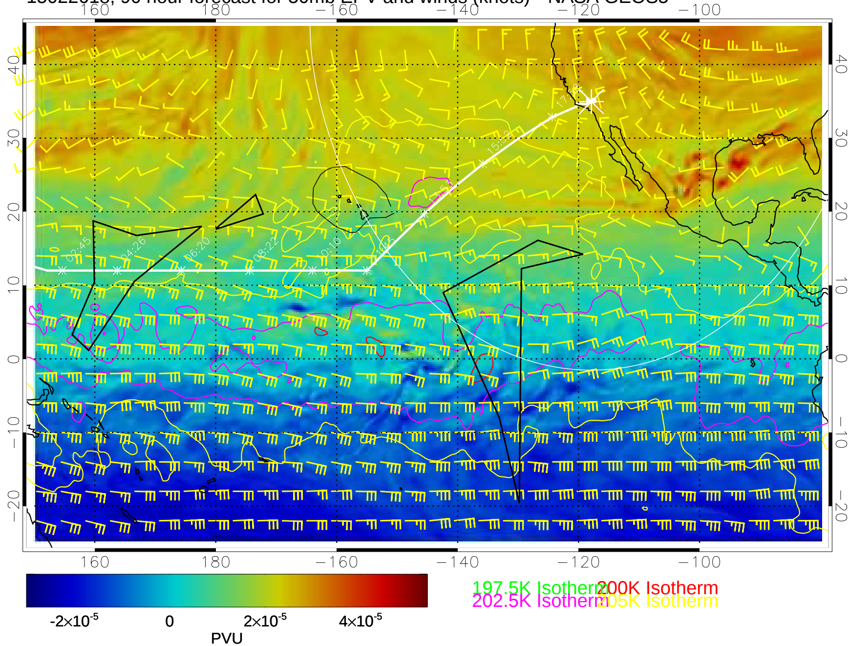
15022618, 90 hour forecast for 50mb EPV and winds (knots)-- NASA GEOS5
