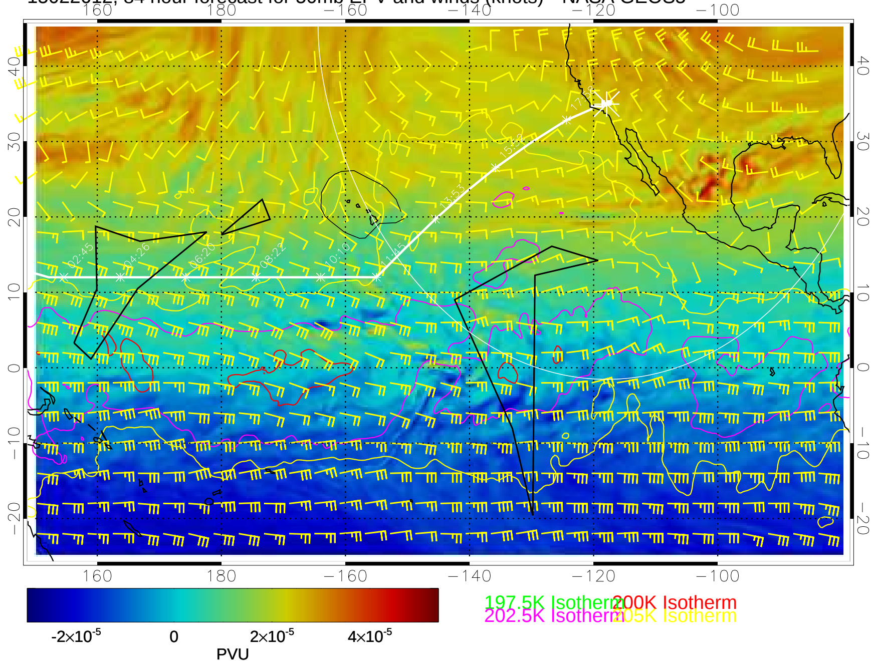
15022612, 84 hour forecast for 50mb EPV and winds (knots)-- NASA GEOS5
