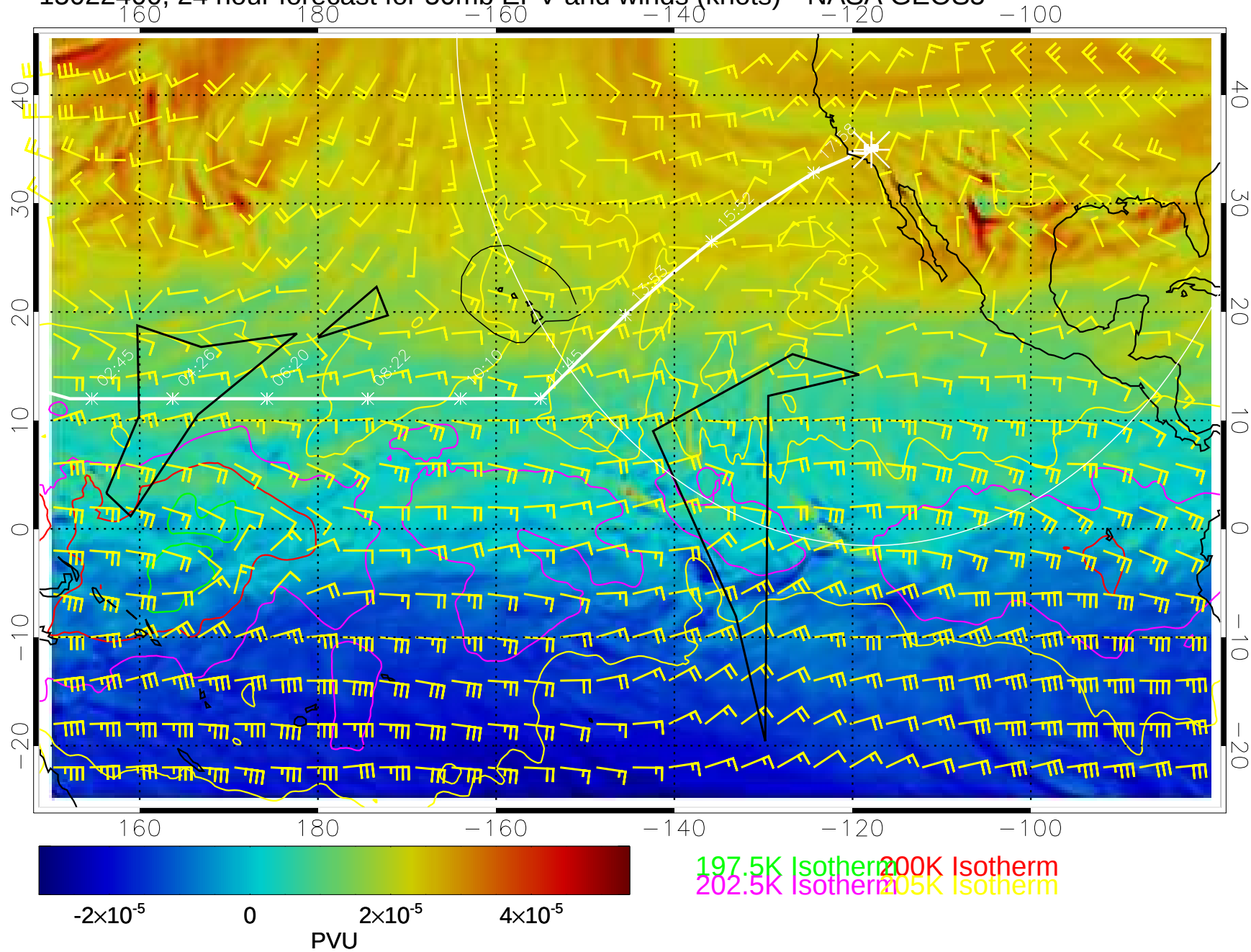
15022400, 24 hour forecast for 50mb EPV and winds (knots)-- NASA GEOS5
