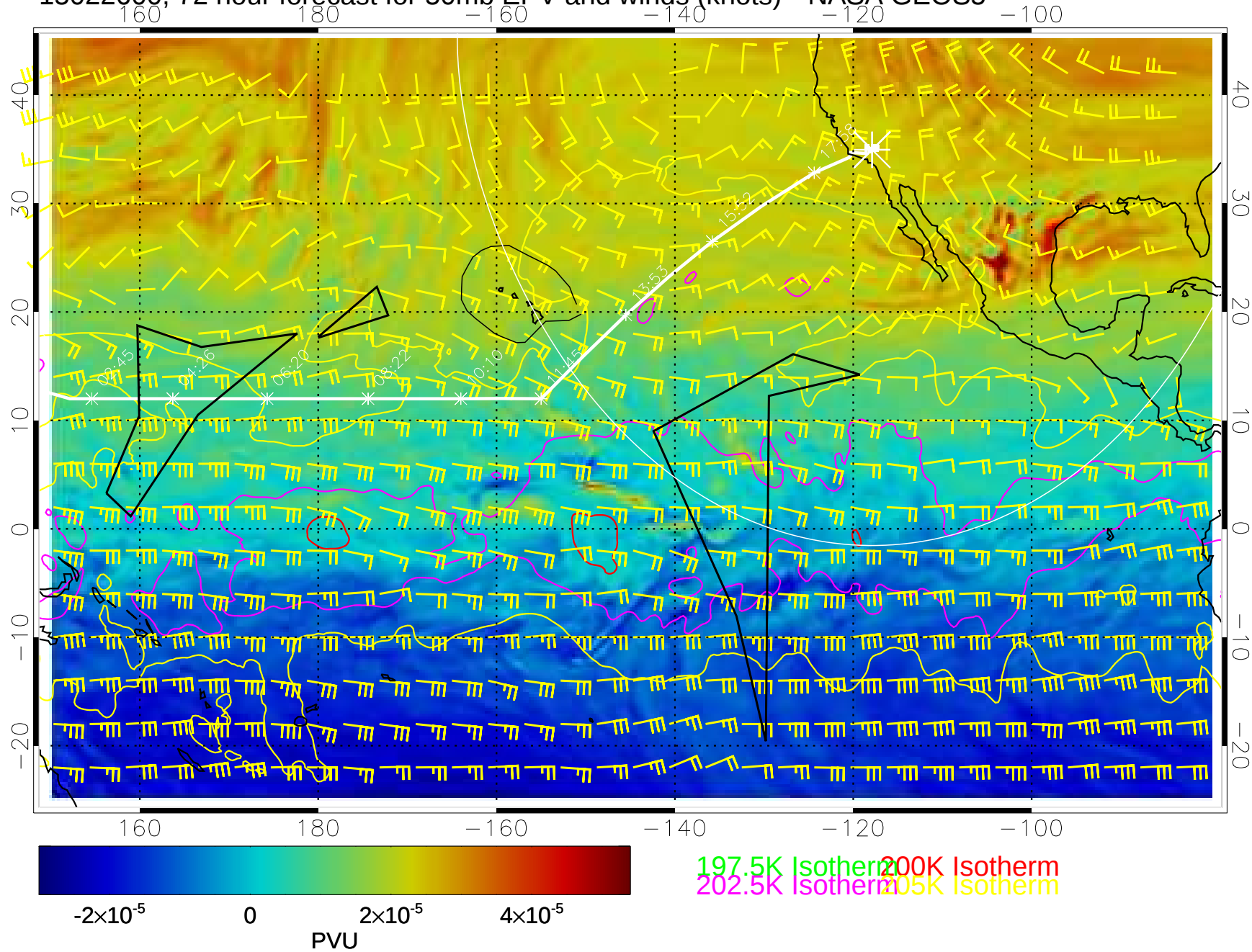
15022600, 72 hour forecast for 50mb EPV and winds (knots)-- NASA GEOS5
