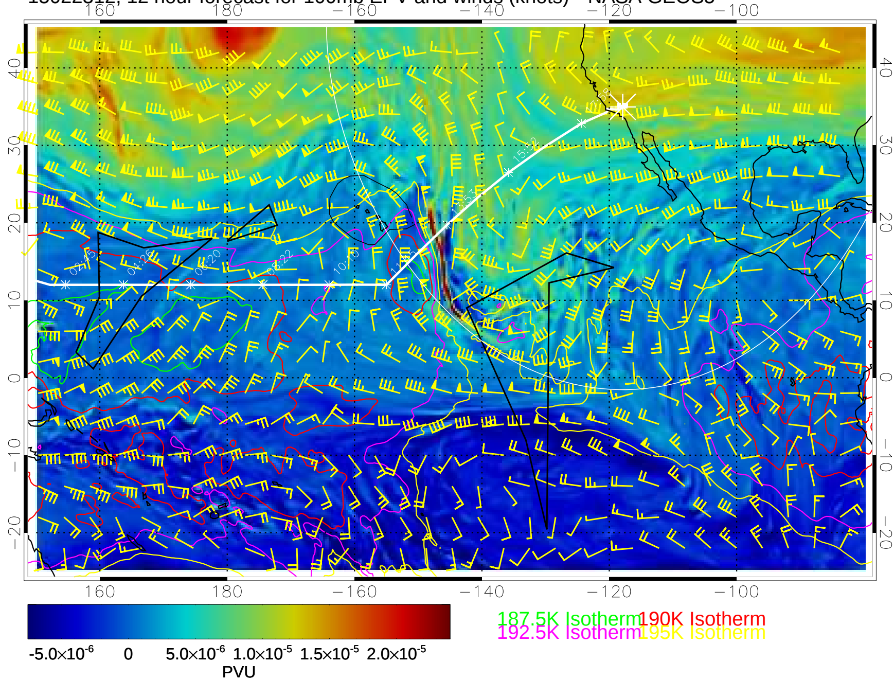
15022312, 12 hour forecast for 100mb EPV and winds (knots)-- NASA GEOS5
