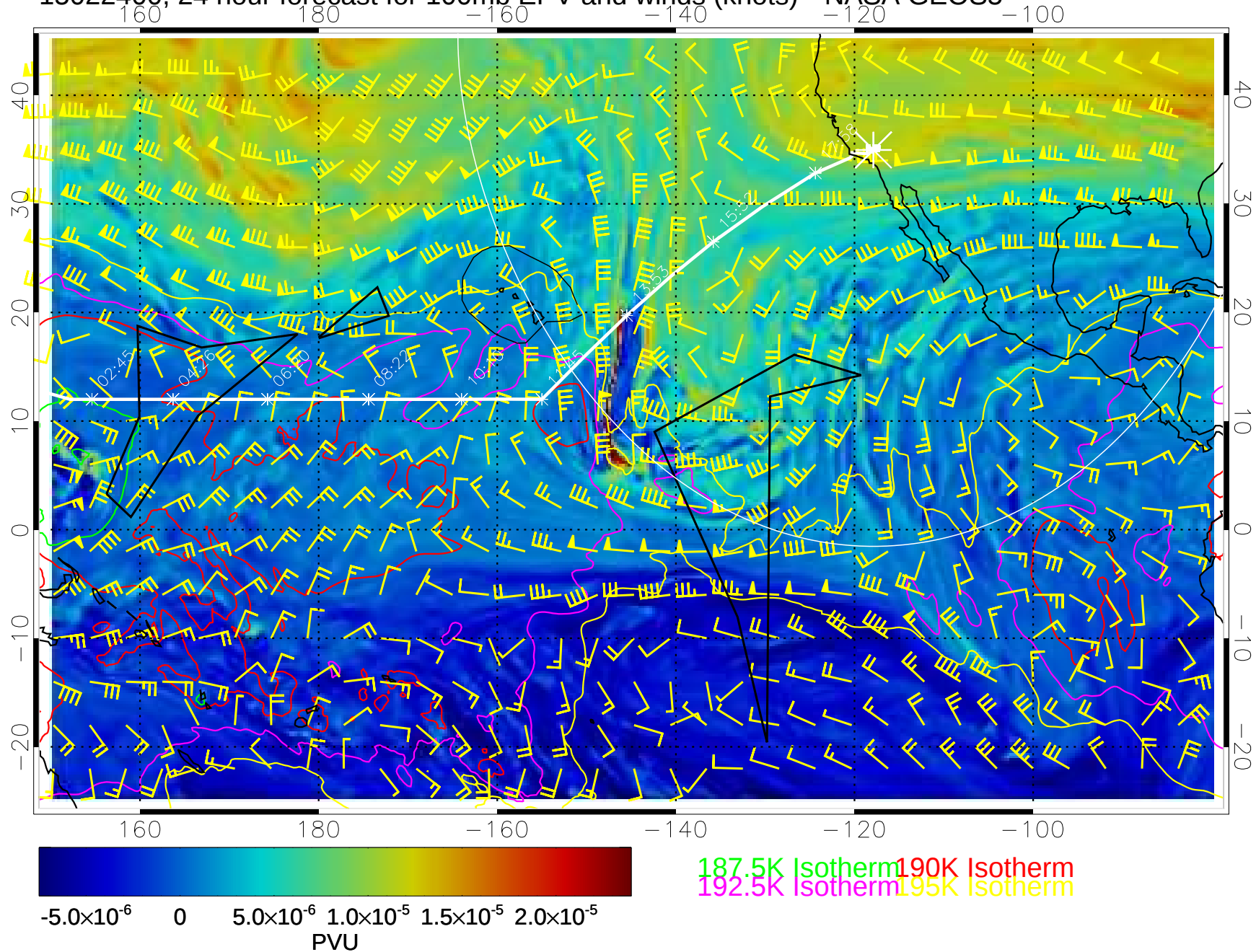
15022400, 24 hour forecast for 100mb EPV and winds (knots)-- NASA GEOS5
